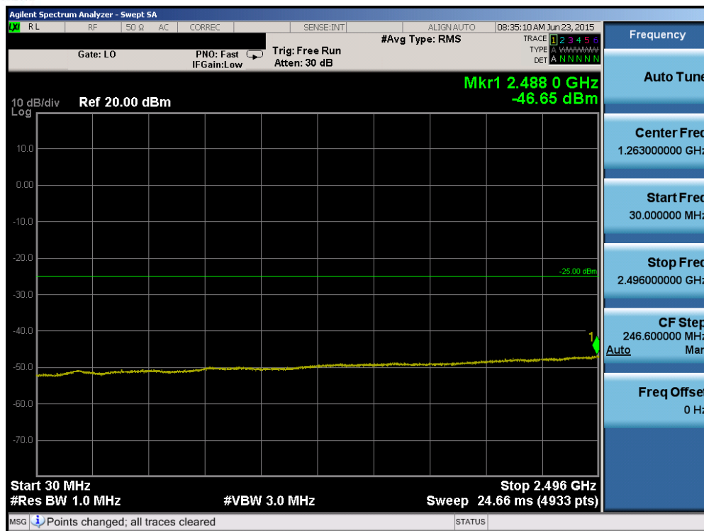
Plot 6-65. Conducted Spurious Plot (Band 41 – 10.0MHz QPSK – RB Size 1, RB Offset 0 – Mid Channel)
