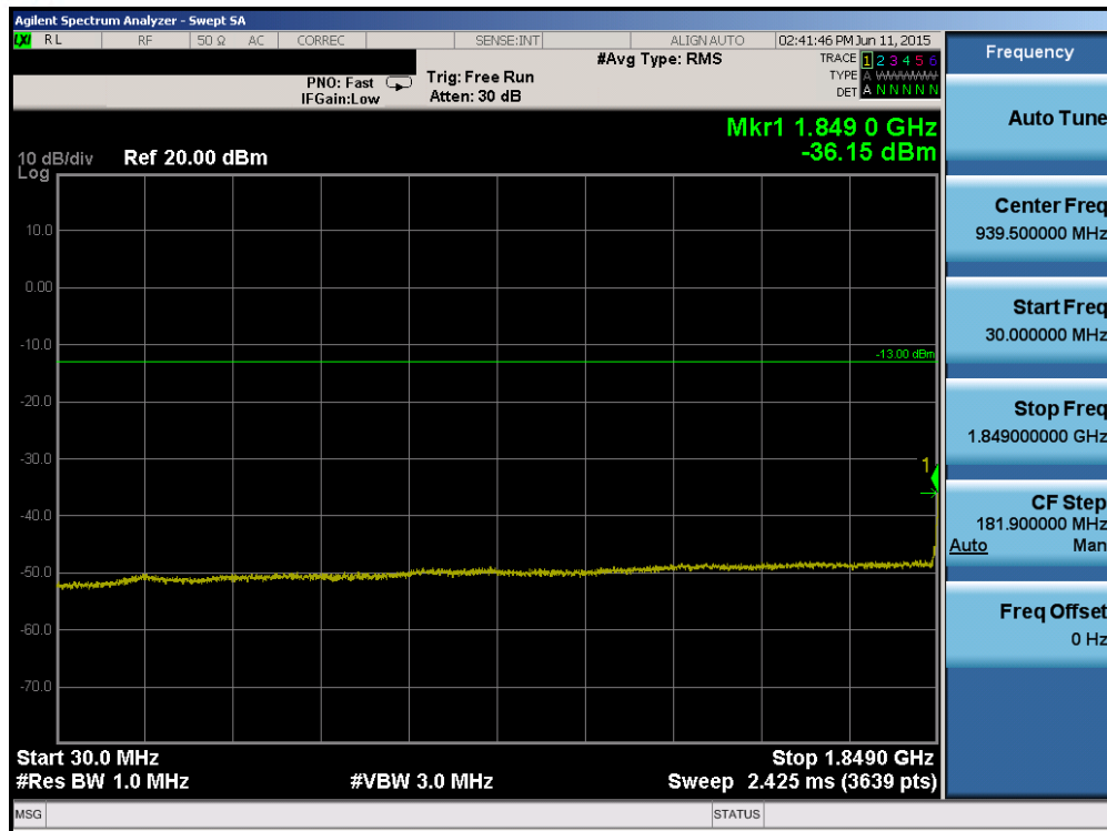
Plot 6-53. Conducted Spurious Plot (Band 2 – 5.0MHz QPSK – RB Size 1, RB Offset 0 – Low Channel)
