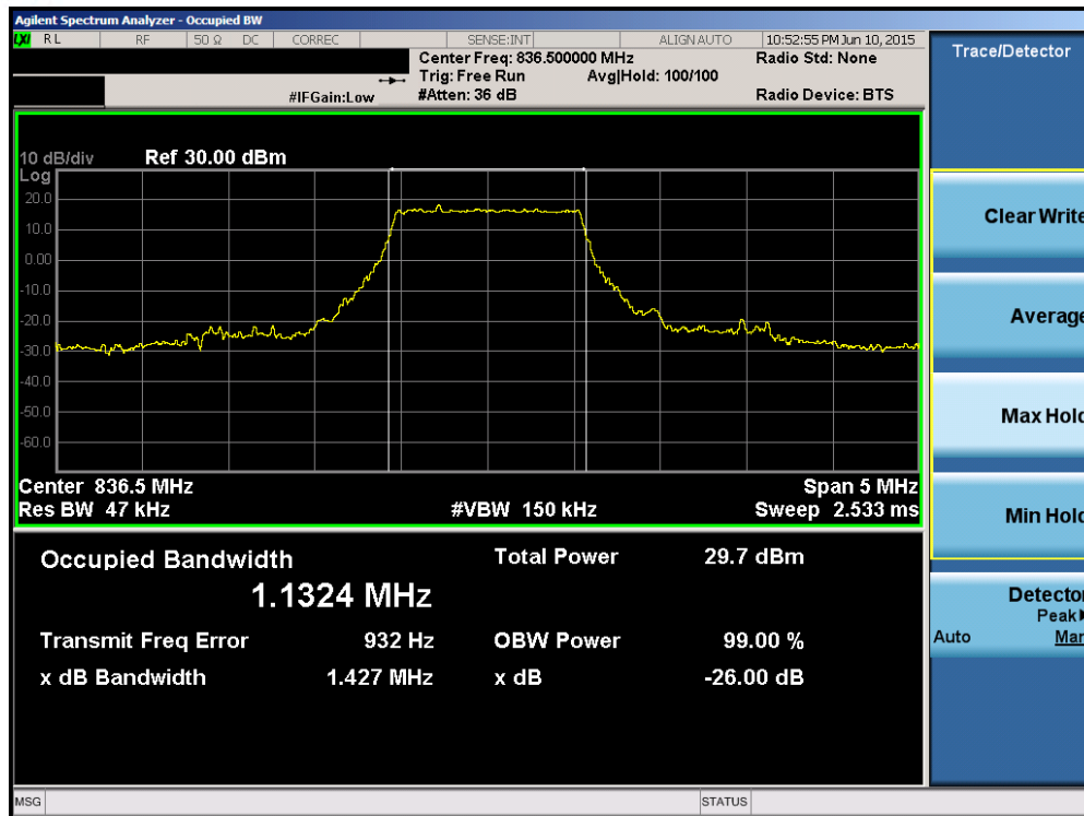
Plot 6-5. Occupied Bandwidth Plot (Band 5/26 – 1.4MHz QPSK – RB Size 6)
