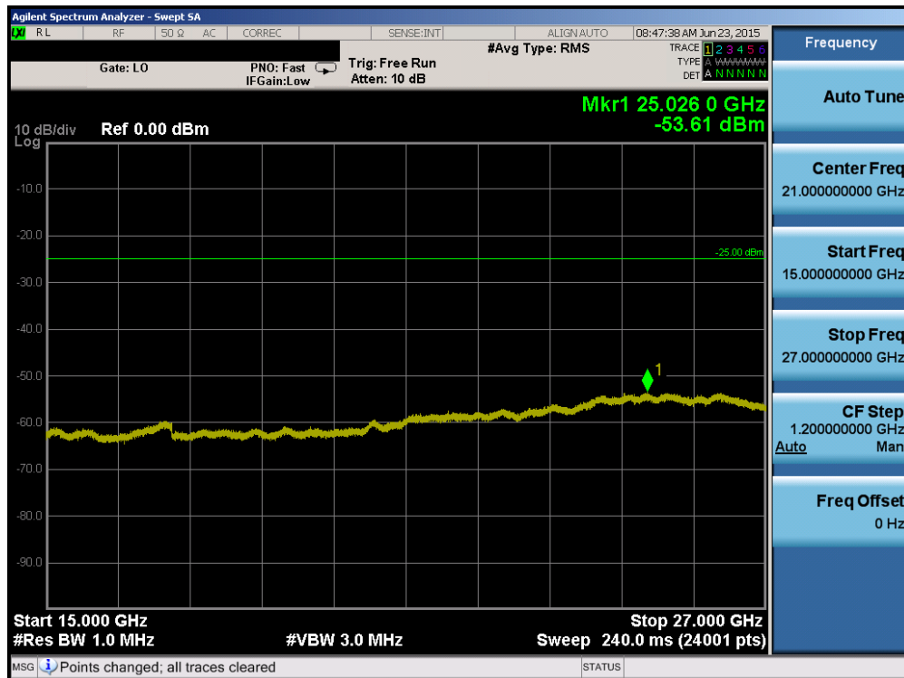
Plot 6-70. Conducted Spurious Plot (Band 41 – 10.0MHz QPSK – RB Size 1, RB Offset 0 – High Channel)
