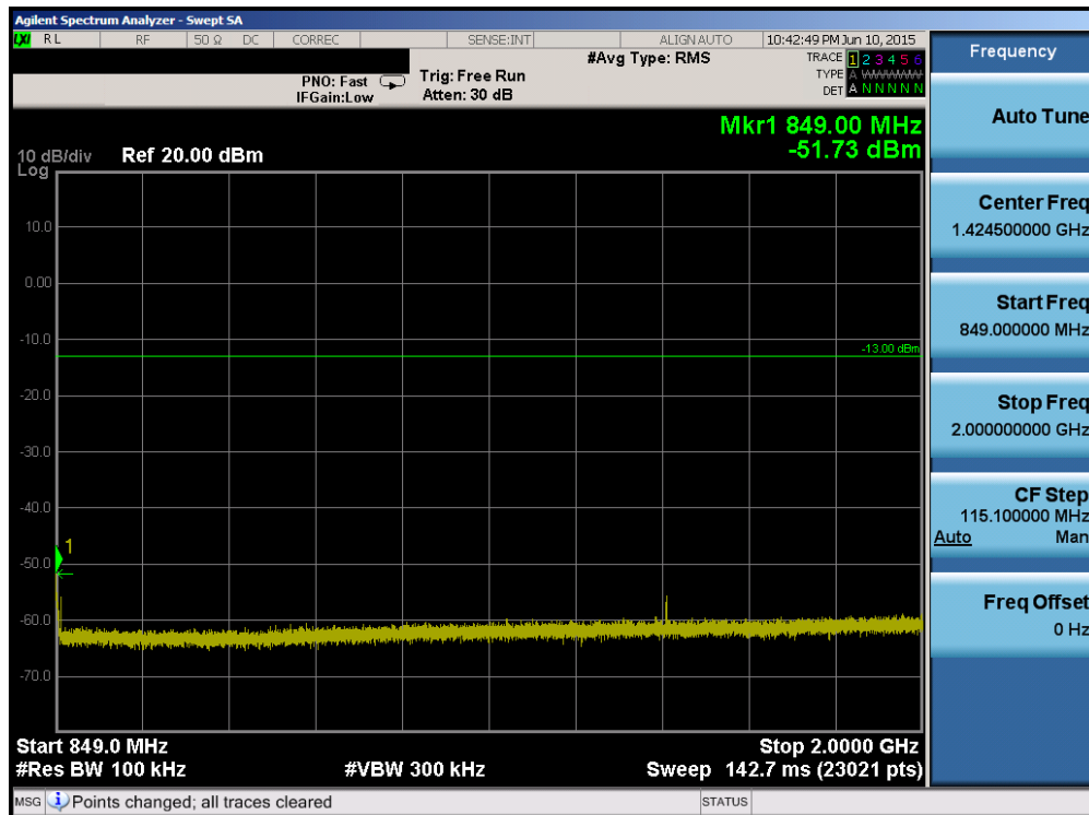
Plot 6-48. Conducted Spurious Plot (Band 26 – 15.0MHz QPSK – RB Size 1, RB Offset 0 – Mid Channel)
