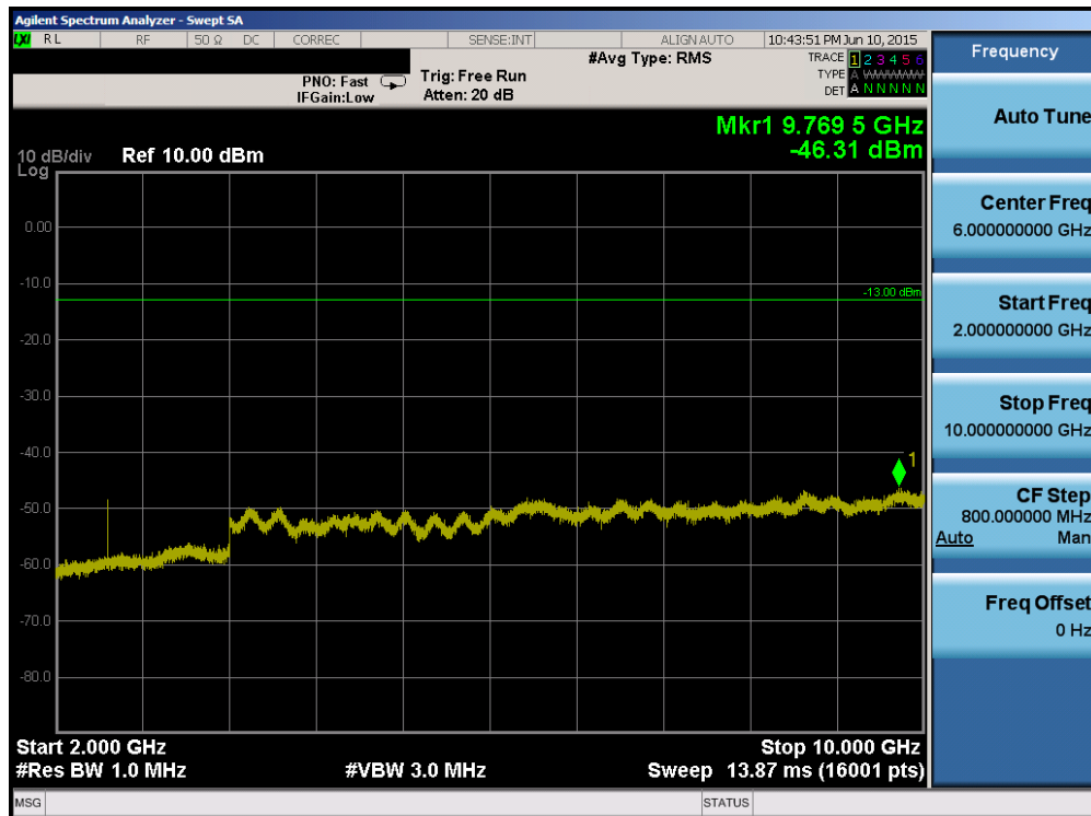
Plot 6-46. Conducted Spurious Plot (Band 26 – 15.0MHz QPSK – RB Size 1, RB Offset 0 – Low Channel)
