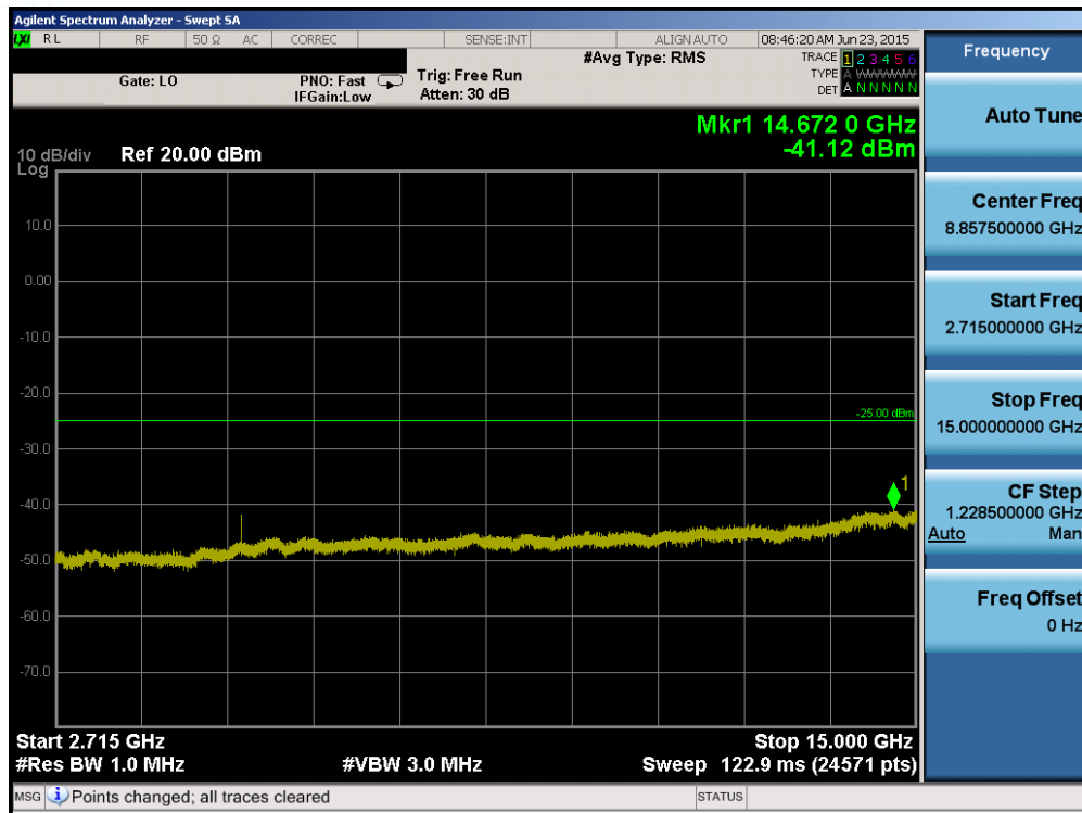
Plot 6-69. Conducted Spurious Plot (Band 41 – 10.0MHz QPSK – RB Size 1, RB Offset 0 – High Channel)
