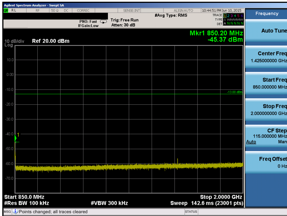
Plot 6-51. Conducted Spurious Plot (Band 26 – 15.0MHz QPSK – RB Size 1, RB Offset 0 – High Channel)
