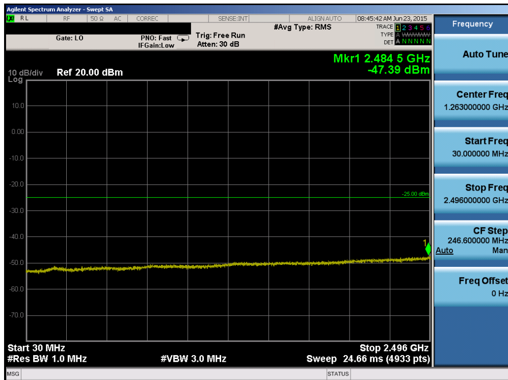
Plot 6-68. Conducted Spurious Plot (Band 41 – 10.0MHz QPSK – RB Size 1, RB Offset 0 – High Channel)
