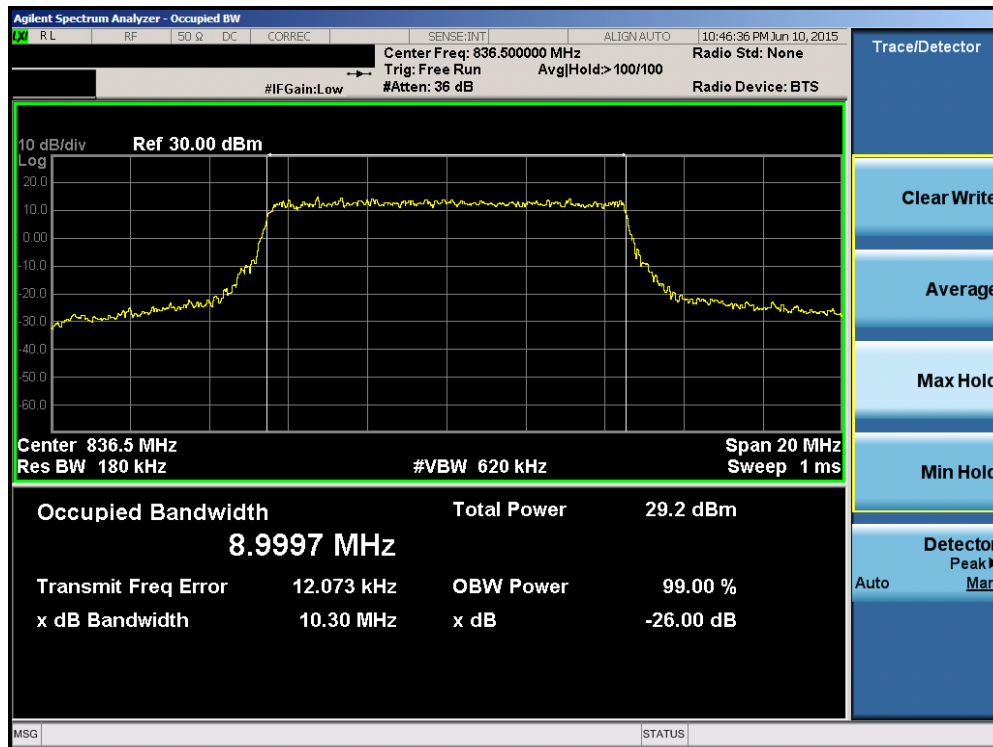
Plot 6-11. Occupied Bandwidth Plot (Band 5/26 – 10.0MHz QPSK – RB Size 50)
