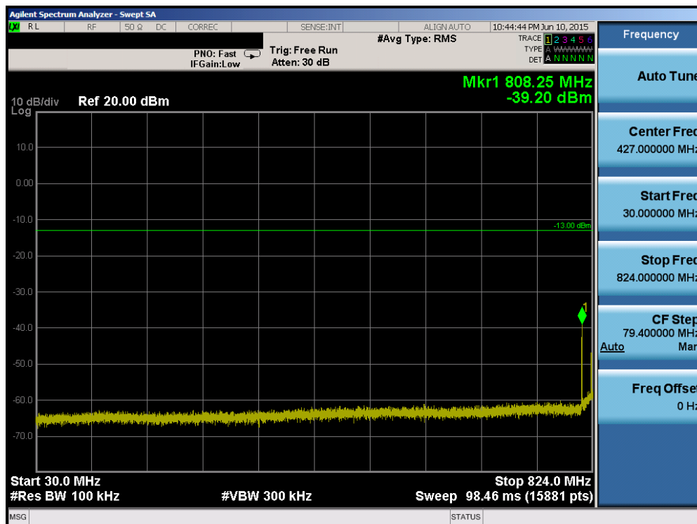
Plot 6-50. Conducted Spurious Plot (Band 26 – 15.0MHz QPSK – RB Size 1, RB Offset 0 – High Channel)
