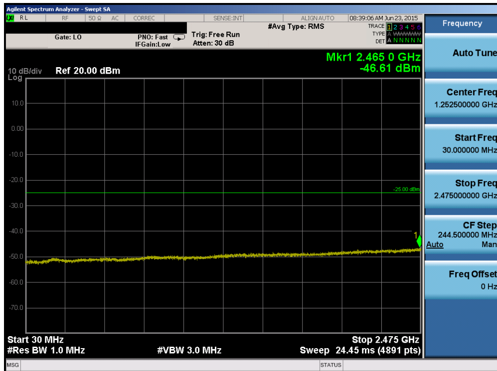
Plot 6-62. Conducted Spurious Plot (Band 41 – 10.0MHz QPSK – RB Size 1, RB Offset 0– Low Channel)
