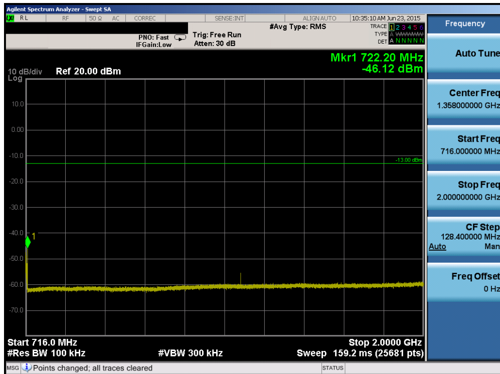
Plot 6-36. Conducted Spurious Plot (Band 17 – 10.0MHz QPSK – RB Size 1, RB Offset 0 – Low Channel)
