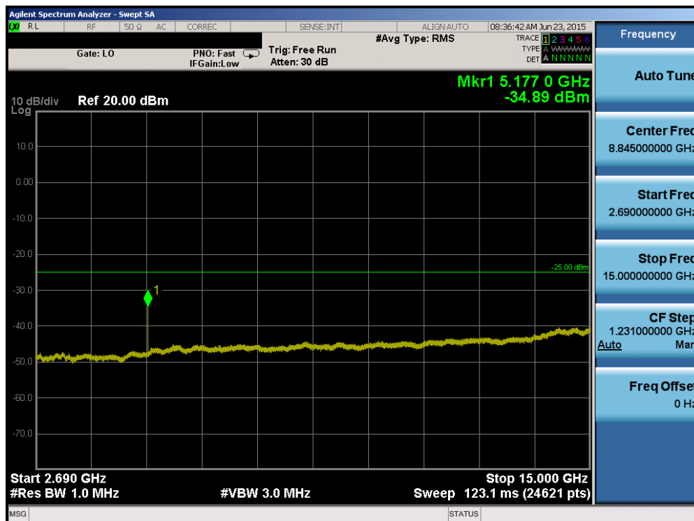
Plot 6-66. Conducted Spurious Plot (Band 41 – 10.0MHz QPSK – RB Size 1, RB Offset 0 – Mid Channel)
