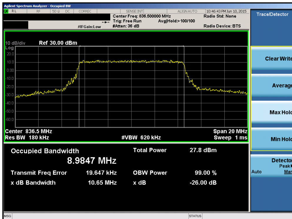
Plot 6-12. Occupied Bandwidth Plot (Band 5/26 – 10.0MHz 16-QAM – RB Size 50)
