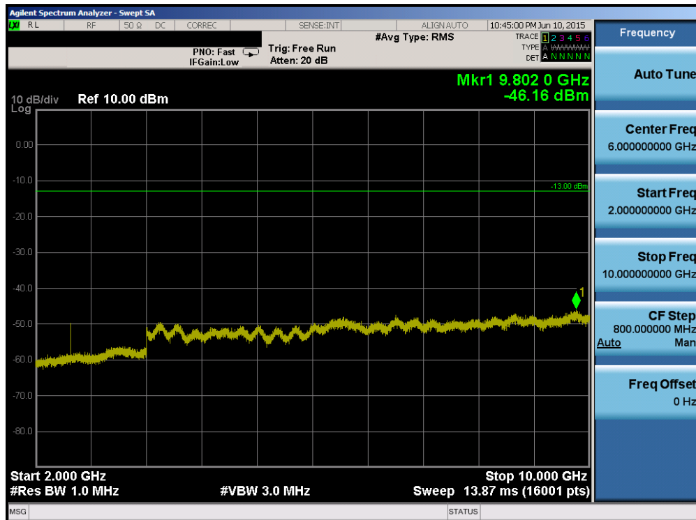
Plot 6-52. Conducted Spurious Plot (Band 26 – 15.0MHz QPSK – RB Size 1, RB Offset 0 – High Channel)
