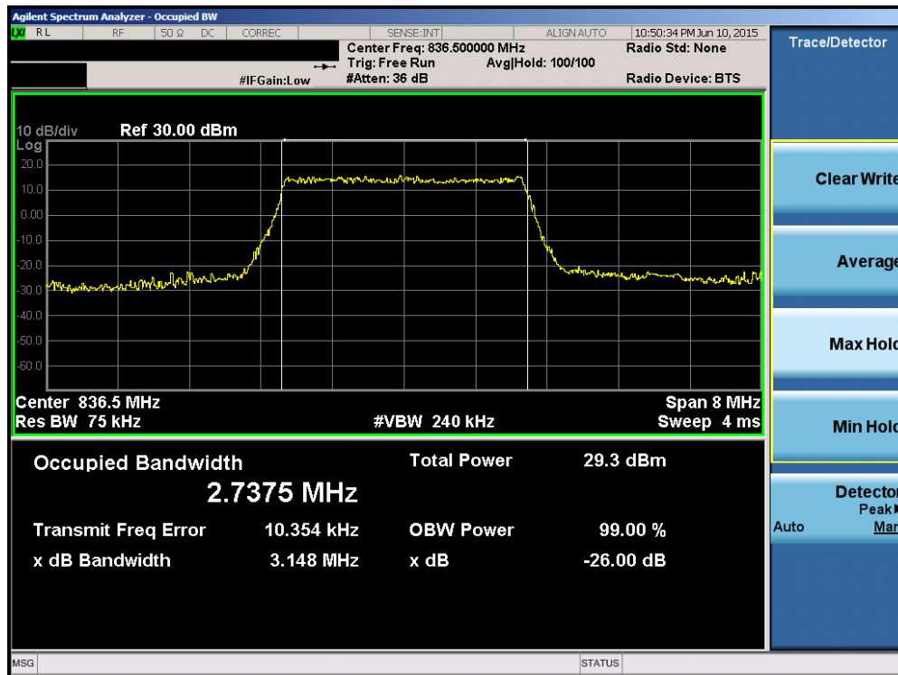
Plot 6-7. Occupied Bandwidth Plot (Band 5/26 – 3.0MHz QPSK – RB Size 15)
