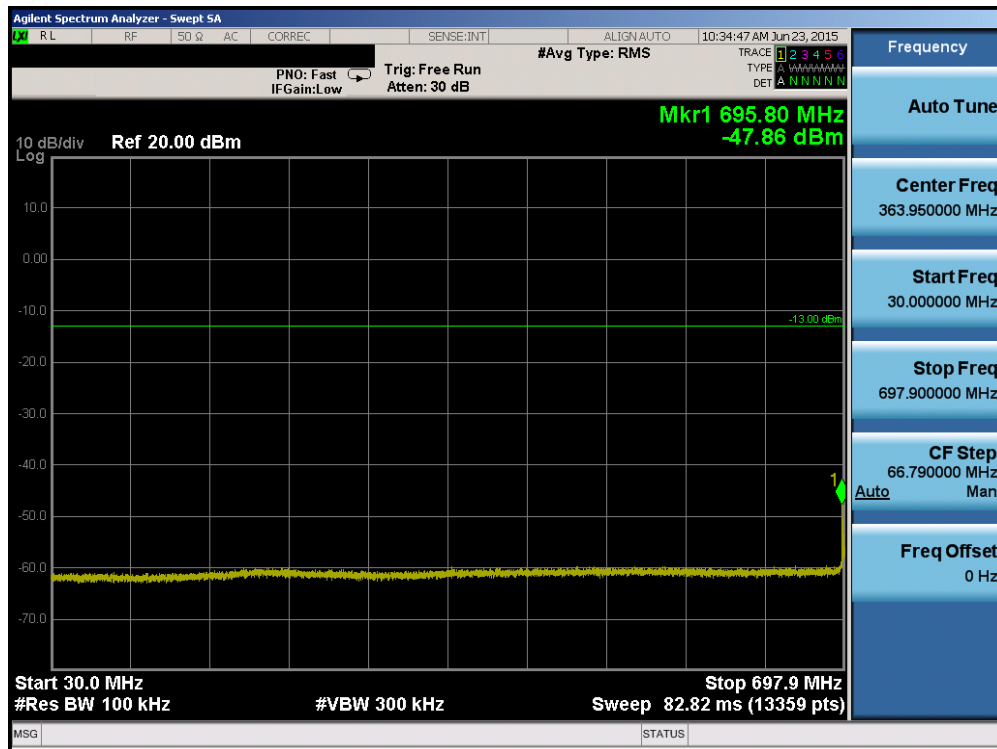
Plot 6-35. Conducted Spurious Plot (Band 17 – 10.0MHz QPSK – RB Size 1, RB Offset 0– Low Channel)
