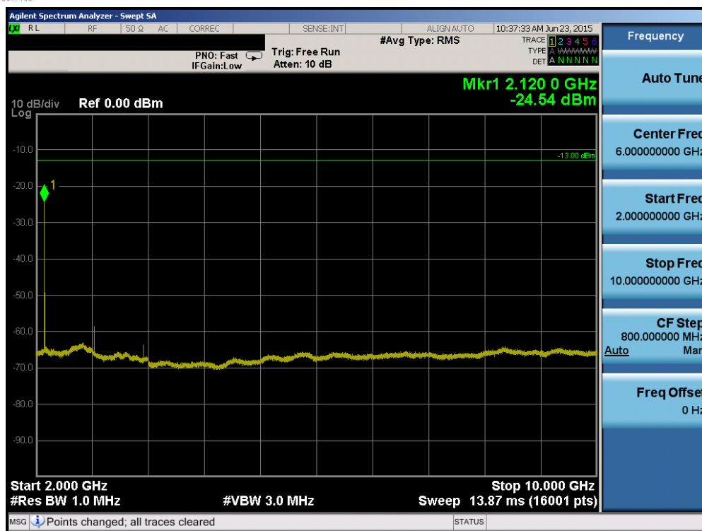
Plot 6-43. Conducted Spurious Plot (Band 17 – 10.0MHz QPSK – RB Size 1, RB Offset 0 – High Channel)
