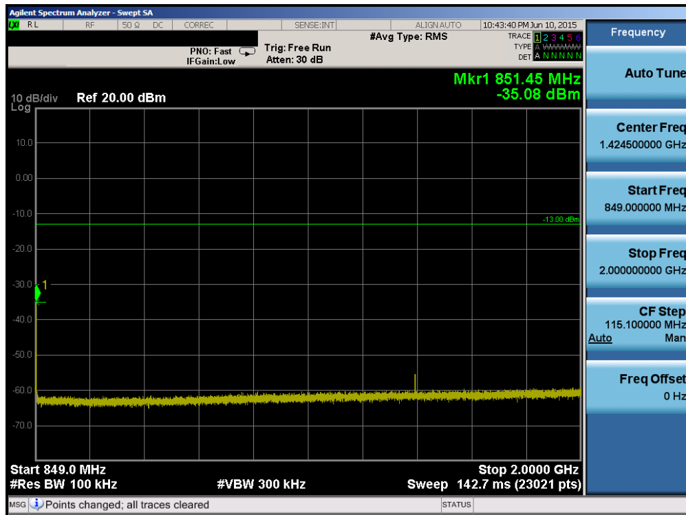
Plot 6-45. Conducted Spurious Plot (Band 26 – 15.0MHz QPSK – RB Size 1, RB Offset 0 – Low Channel)
