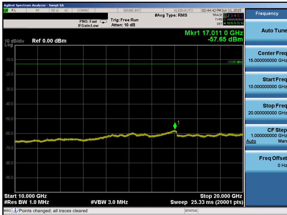
Plot 6-61. Conducted Spurious Plot (Band 2 – 5.0MHz QPSK – RB Size 1, RB Offset 0 – High Channel)
