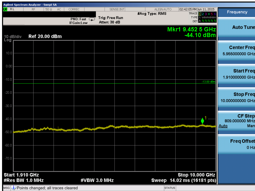
Plot 6-54. Conducted Spurious Plot (Band 2 – 5.0MHz QPSK – RB Size 1, RB Offset 0 – Low Channel)
