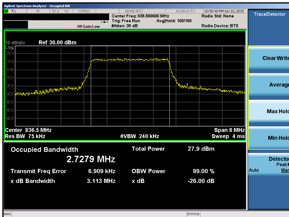
Plot 6-8. Occupied Bandwidth Plot (Band 5/26 – 3.0MHz 16-QAM – RB Size 15)
