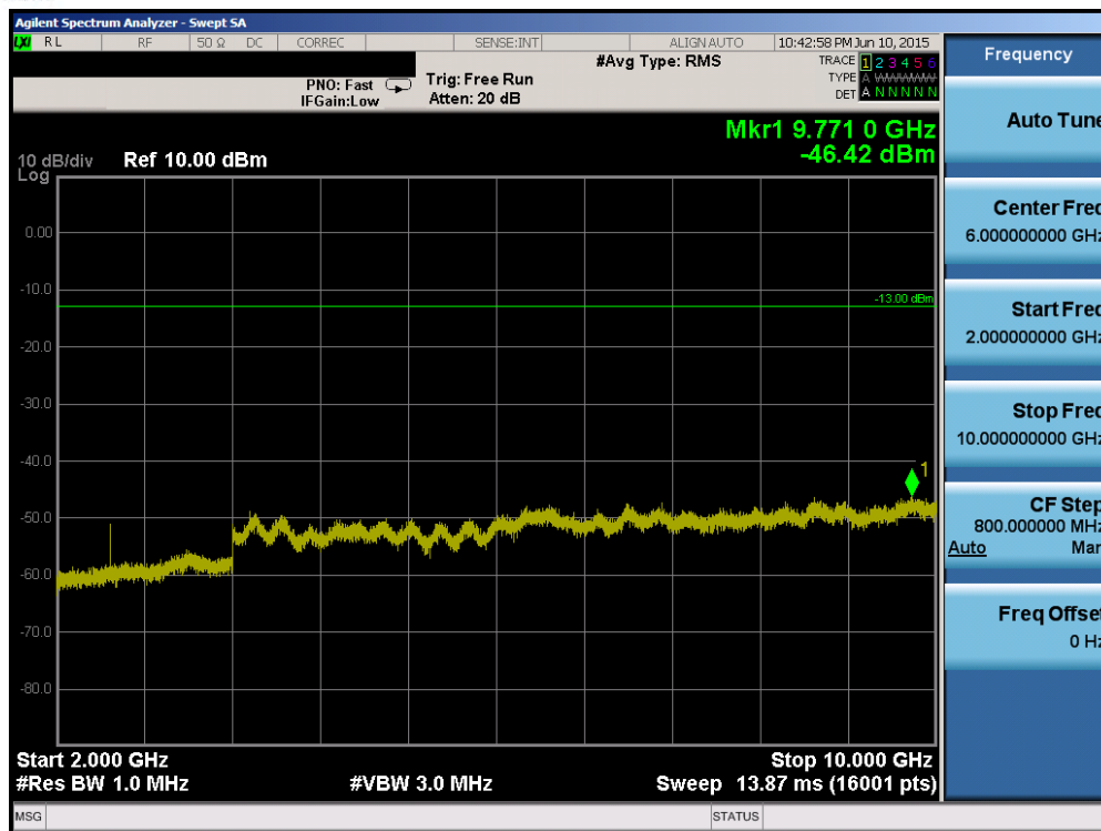
Plot 6-49. Conducted Spurious Plot (Band 26 – 15.0MHz QPSK – RB Size 1, RB Offset 0 – Mid Channel)
