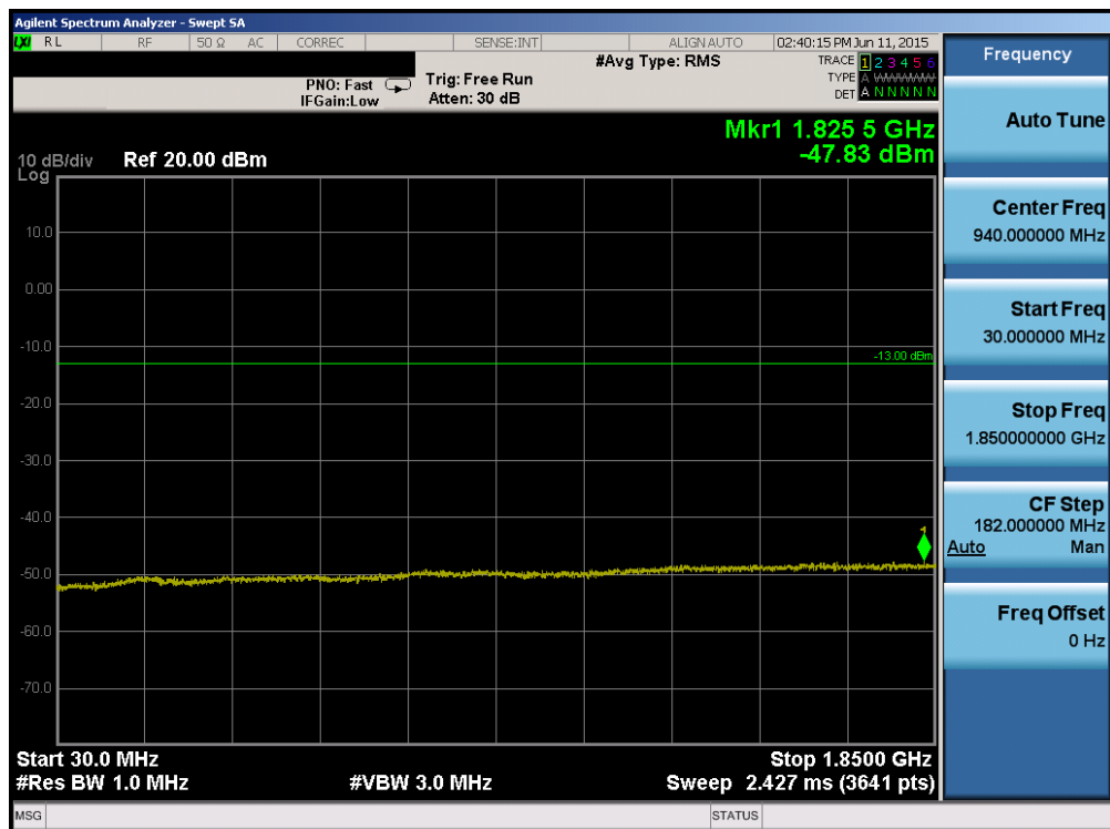
Plot 6-56. Conducted Spurious Plot (Band 2 – 5.0MHz QPSK – RB Size 1, RB Offset 0 – Mid Channel)
