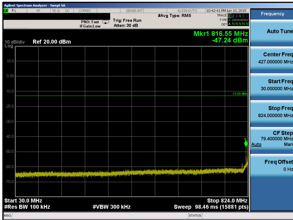
Plot 6-47. Conducted Spurious Plot (Band 26 – 15.0MHz QPSK – RB Size 1, RB Offset 0 – Mid Channel)
