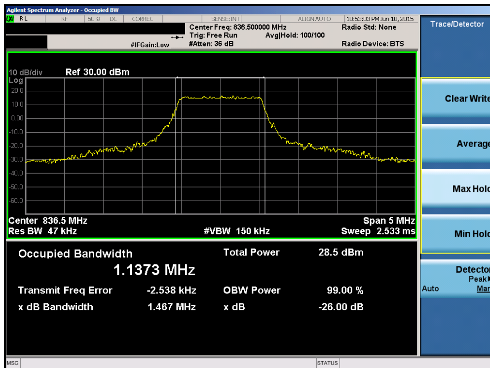
Plot 6-6. Occupied Bandwidth Plot (Band 5/26 – 1.4MHz 16-QAM – RB Size 6)
