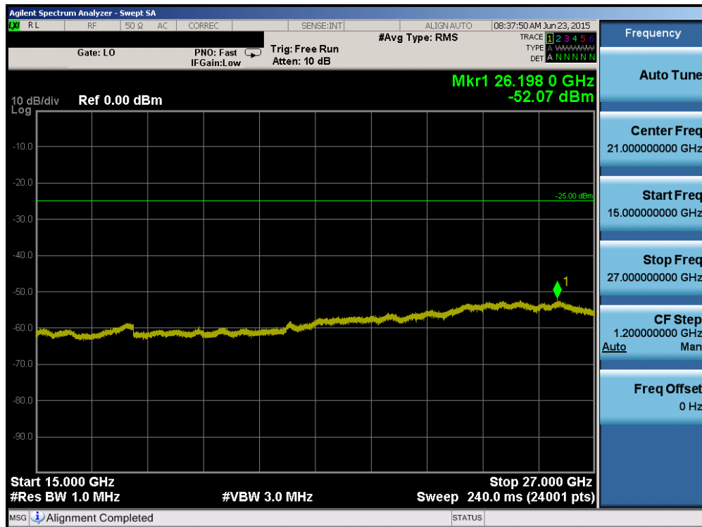
Plot 6-67. Conducted Spurious Plot (Band 41 – 10.0MHz QPSK – RB Size 1, RB Offset 0 – Mid Channel)
