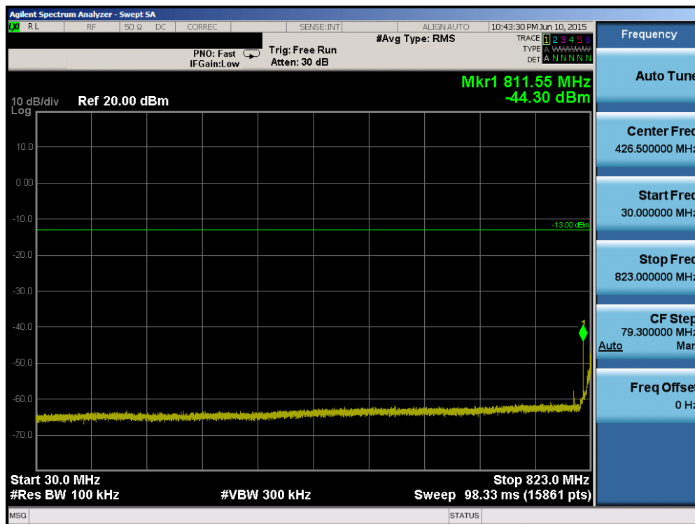
Plot 6-44. Conducted Spurious Plot (Band 26 – 15.0MHz QPSK – RB Size 1, RB Offset 0 – Low Channel)
