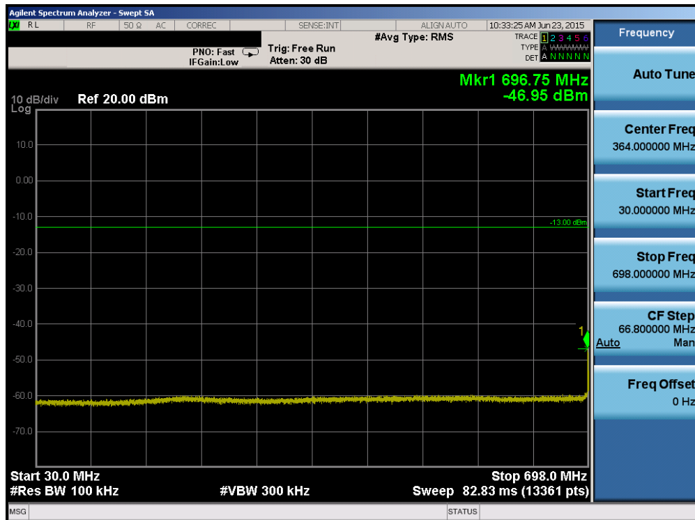
Plot 6-38. Conducted Spurious Plot (Band 17 – 10.0MHz QPSK – RB Size 1, RB Offset 0 – Mid Channel)
