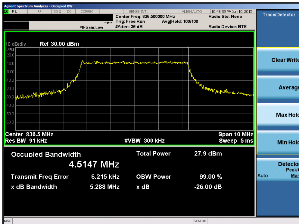
Plot 6-10. Occupied Bandwidth Plot (Band 5/26 – 5.0MHz 16-QAM – RB Size 25)
