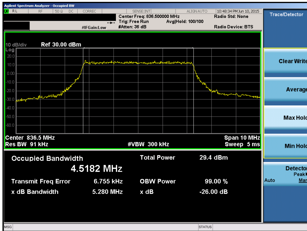
Plot 6-9. Occupied Bandwidth Plot (Band 5/26 – 5.0MHz QPSK – RB Size 25)
