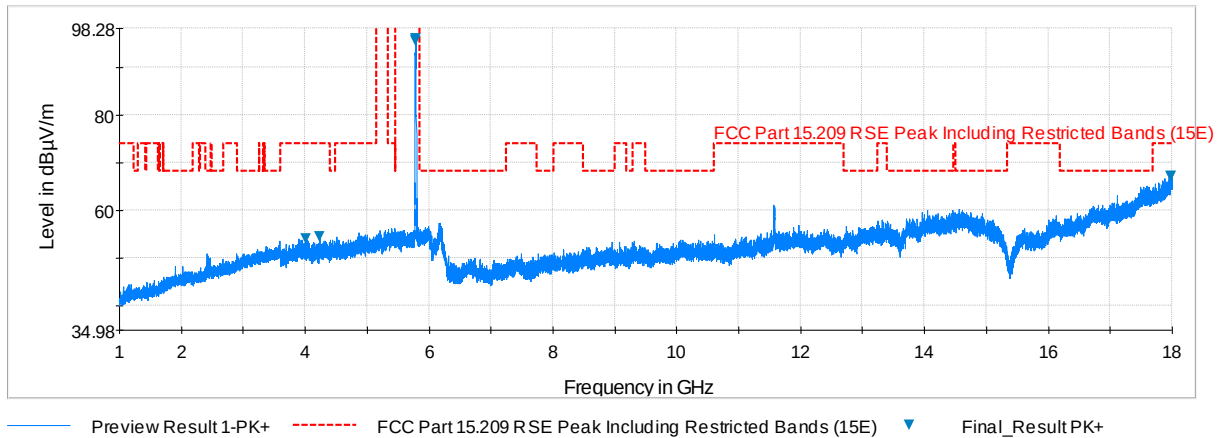
Plot 6-170. Radiated Spurious Plot above 1GHz (802.11a – U3 Ch. 157, Ant. Pol. V)
