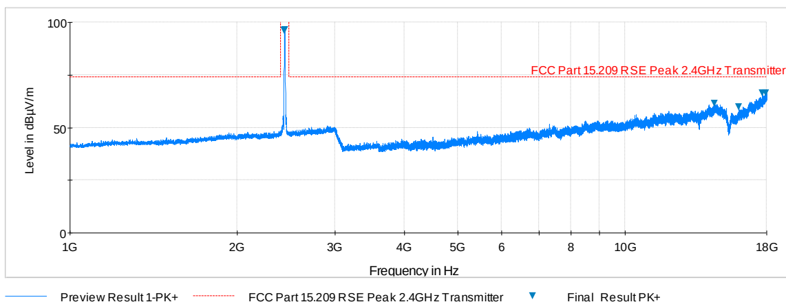
Plot 6-83. Radiated Spurious Plot above 1GHz (802.11b – Ch. 6, Ant. Pol. H)
