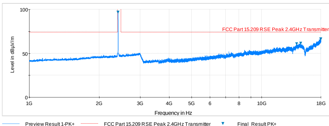
Plot 6-82. Radiated Spurious Plot above 1GHz (802.11b – Ch. 1, Ant. Pol. V)
