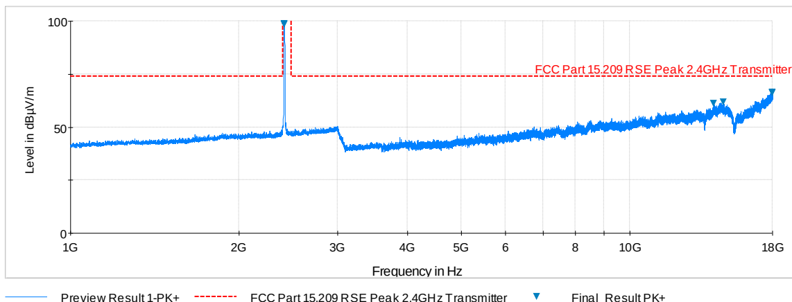
Plot 6-81. Radiated Spurious Plot above 1GHz (802.11b – Ch. 1, Ant. Pol. H)
