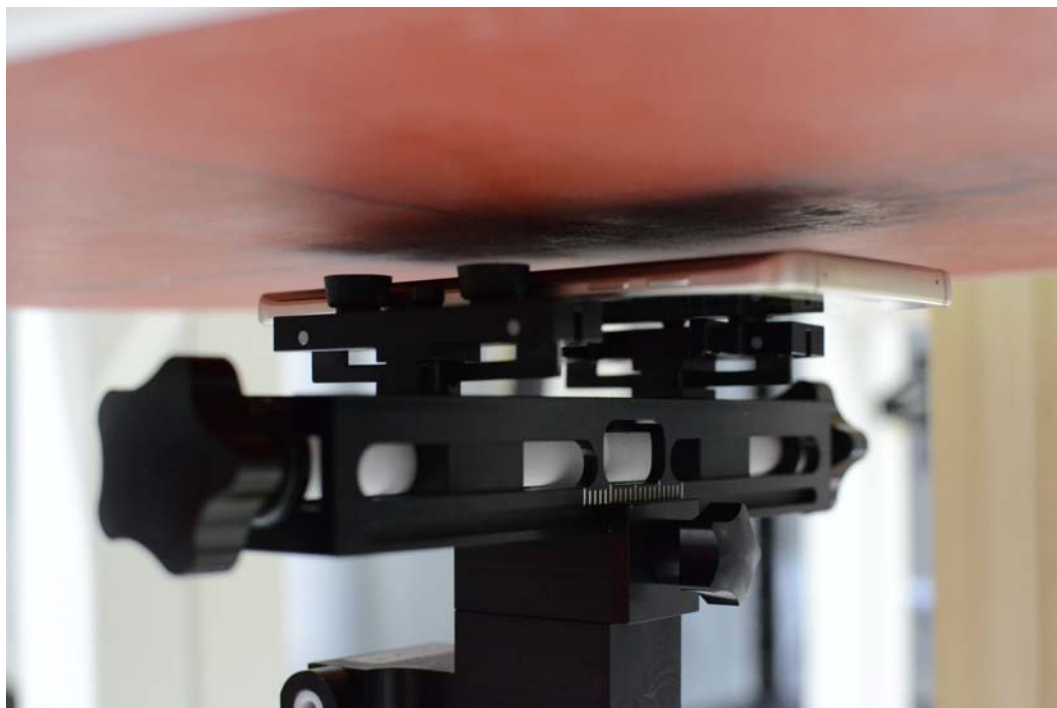
SAR Test Setup Photo 6– Back Side at 1.0 cm (Body-worn and Hotspot)
