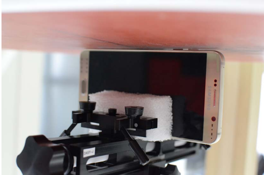
SAR Test Setup Photo 13– Left Edge at 0.0 cm (Extremity)
