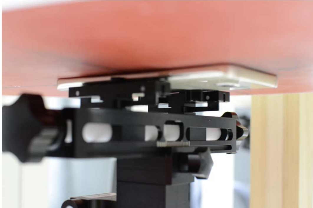
SAR Test Setup Photo 7— Front Side at 0.0 cm (Extremity)
