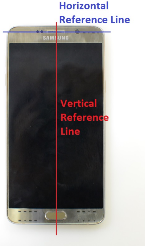
SAR Test Setup Photo 15– DUT Reference Lines
