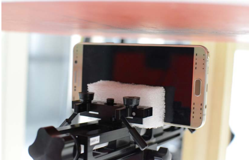
SAR Test Setup Photo 12– Right Edge at 1.0 cm (Hotspot)
