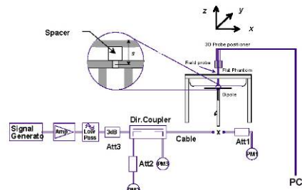
Figure 9 System Verification Setup Diagram
