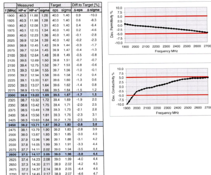
Figure 21 2.4 GHz Head Tissue Equivalent Matter
