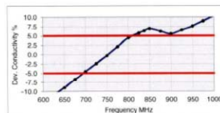
Figure 18 750MHz Body Tissue Equivalent Matter
