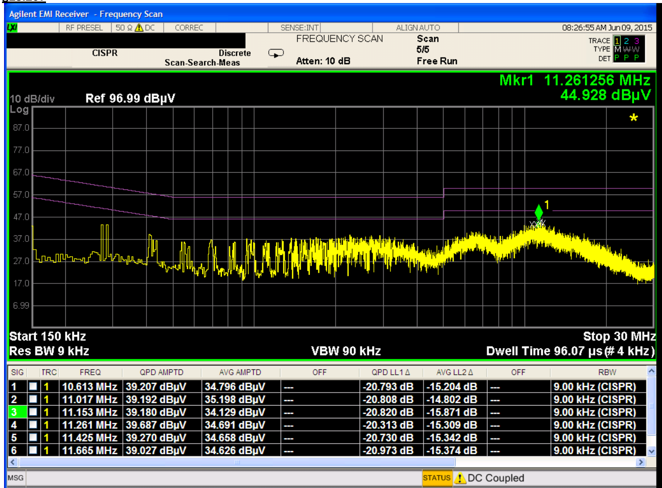
Plot 6-7. Line-Conducted Test Plot (N)
