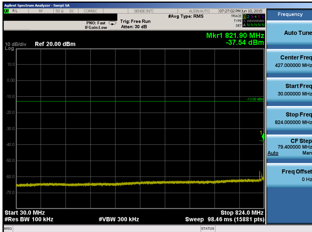
Plot 6-66. Conducted Spurious Plot (Band 26 – 15.0MHz QPSK – RB Size 1, RB Offset 0 – High Channel)
