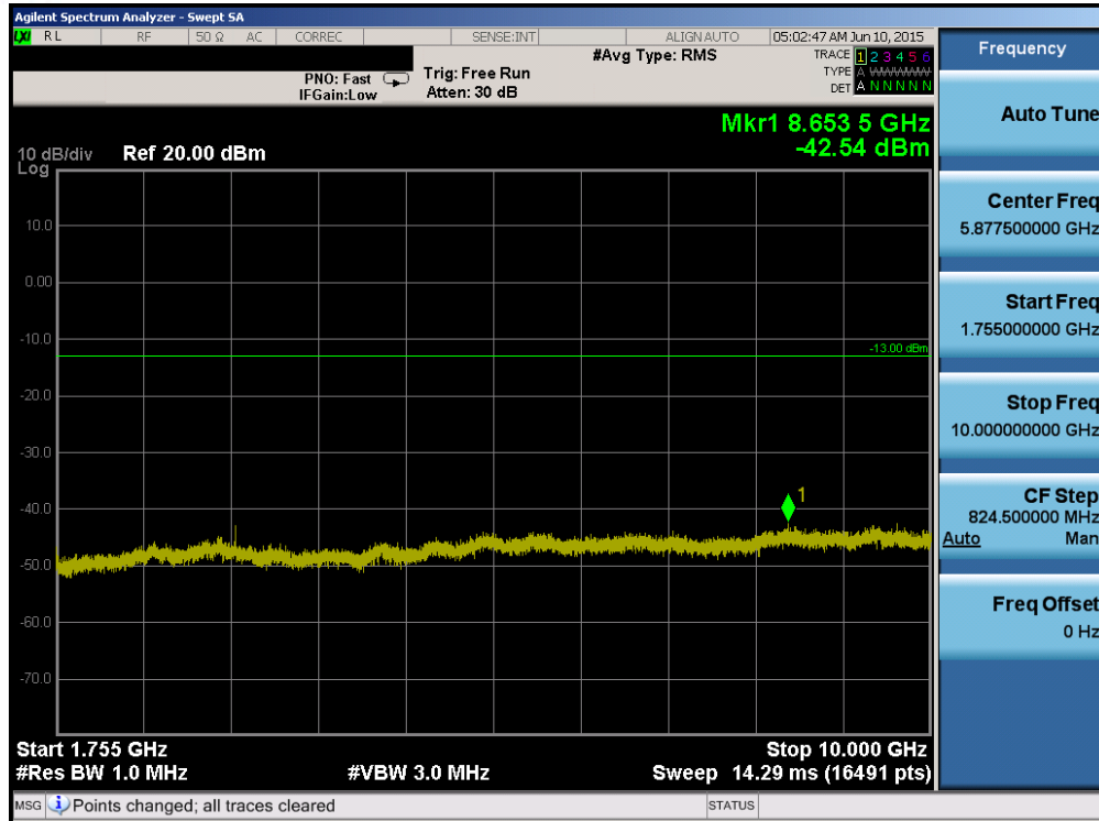
Plot 6-73. Conducted Spurious Plot (Band 4 – 20.0MHz QPSK – RB Size 1, RB Offset 0 – Mid Channel)
