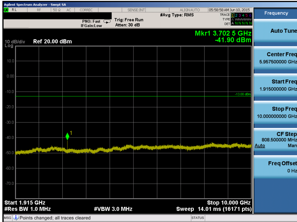
Plot 6-79. Conducted Spurious Plot (Band 25 - 20.0MHz QPSK - RB Size 1, RB Offset 0 - Low Channel)
