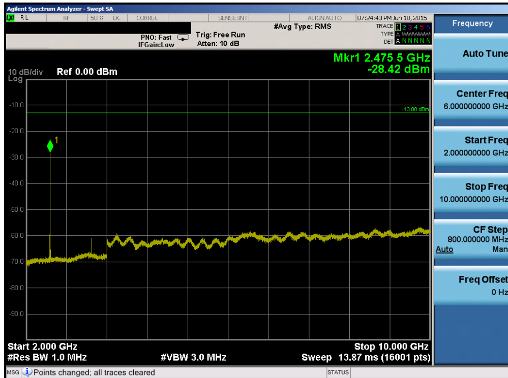
Plot 6-62. Conducted Spurious Plot (Band 26 – 15.0MHz QPSK – RB Size 1, RB Offset 0 – Low Channel)
