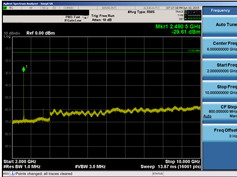
Plot 6-65. Conducted Spurious Plot (Band 26 – 15.0MHz QPSK – RB Size 1, RB Offset 0 – Mid Channel)
