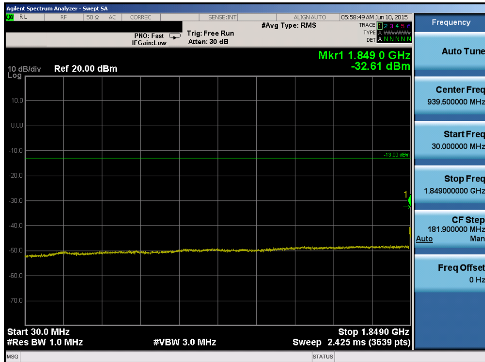
Plot 6-78. Conducted Spurious Plot (Band 25 – 20.0MHz QPSK – RB Size 1, RB Offset 0 – Low Channel)
