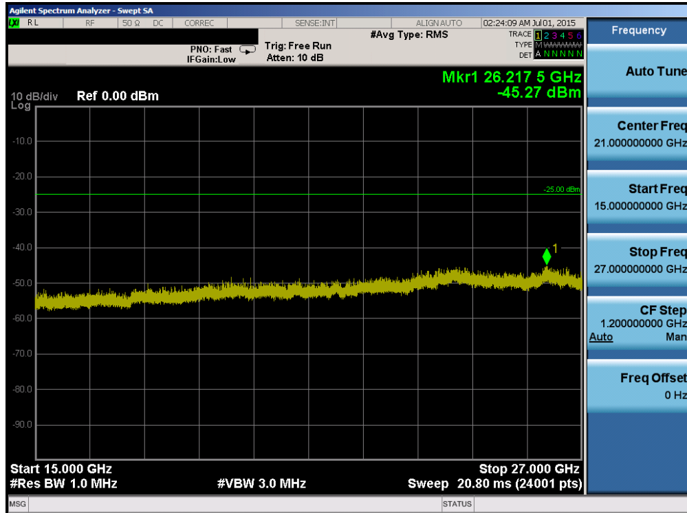
Plot 6-89. Conducted Spurious Plot (Band 41 – 20.0MHz QPSK – RB Size 1, RB Offset 0 – Low Channel)
