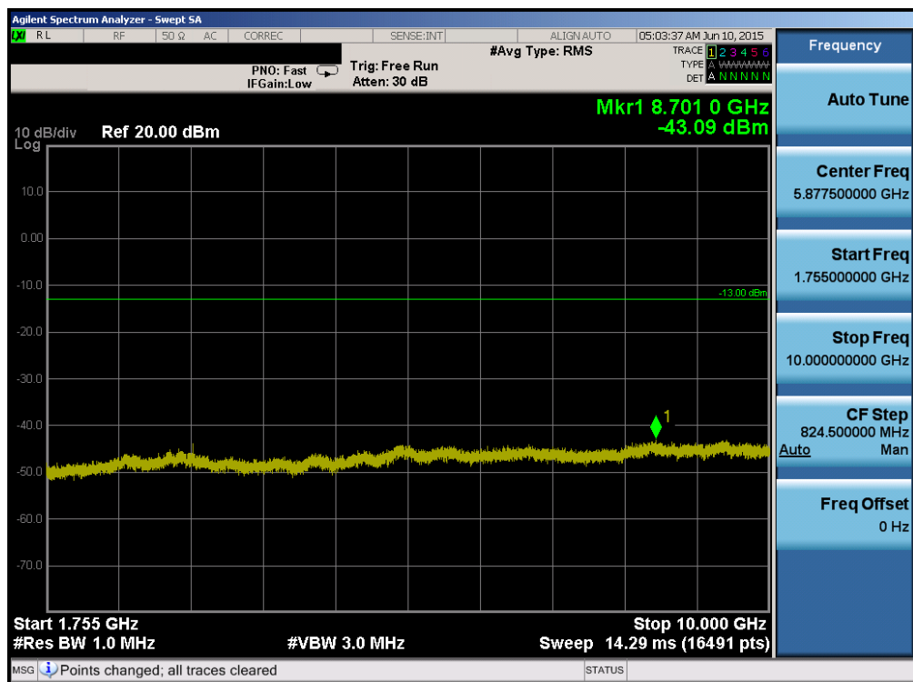
Plot 6-70. Conducted Spurious Plot (Band 4 – 20.0MHz QPSK – RB Size 1, RB Offset 0 – Low Channel)
