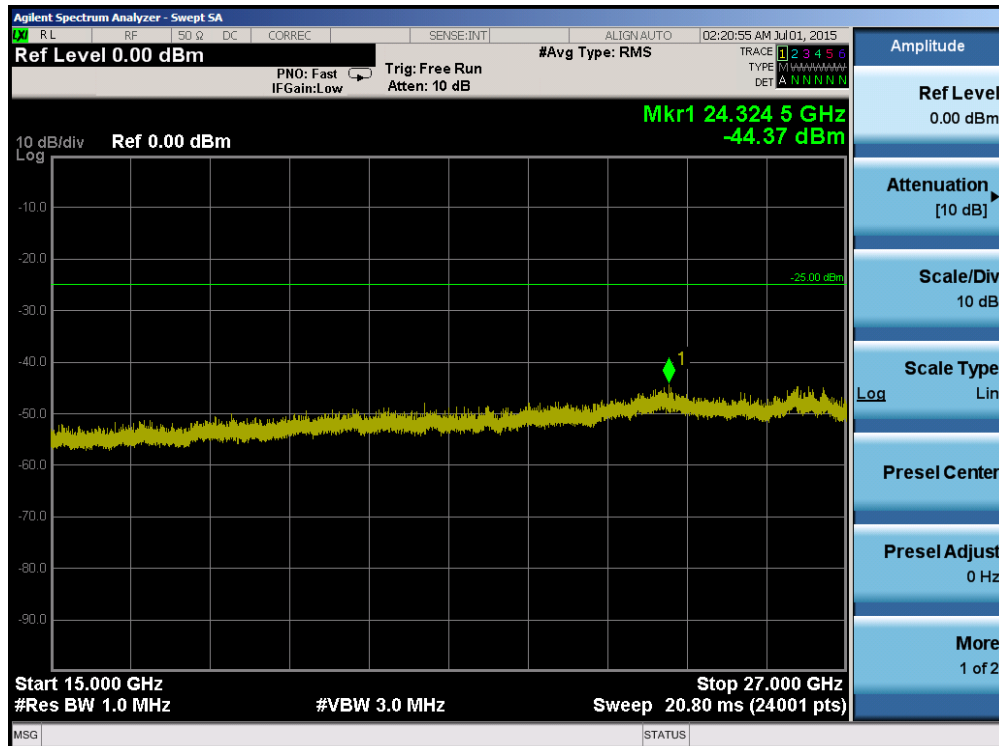
Plot 6-92. Conducted Spurious Plot (Band 41 – 20.0MHz QPSK – RB Size 1, RB Offset 0 – Mid Channel)
