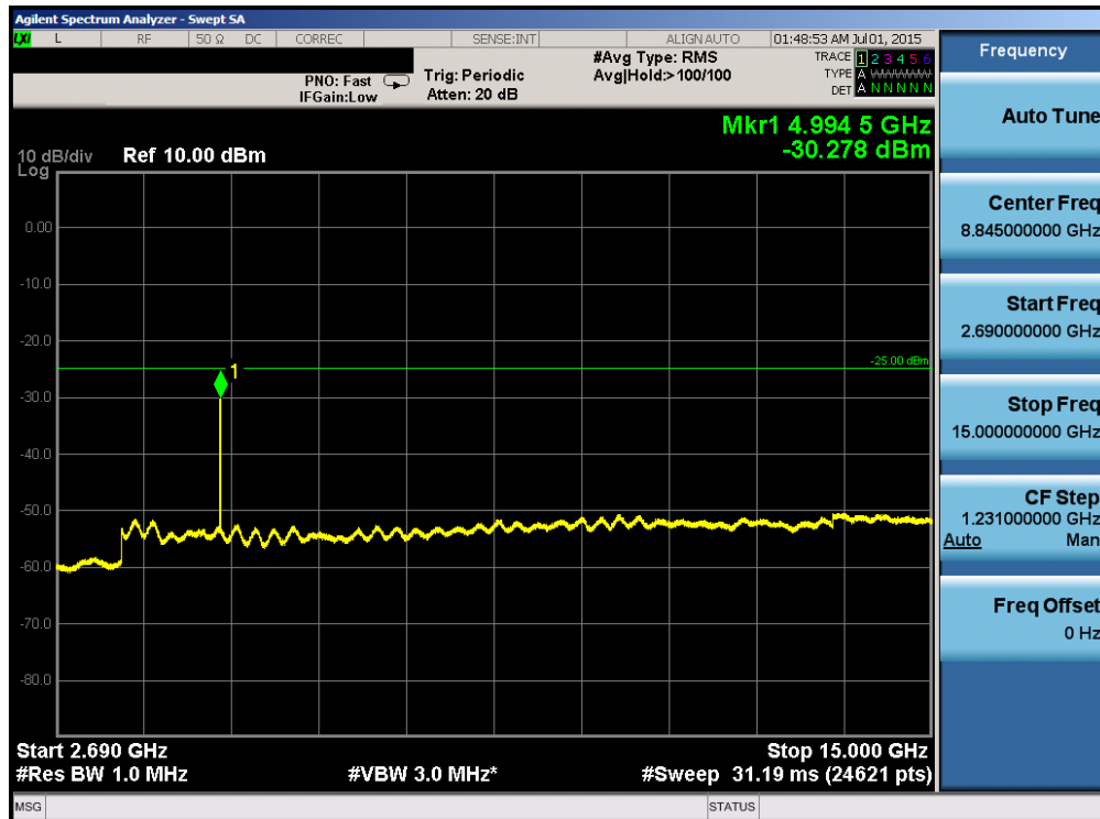
Plot 6-88. Conducted Spurious Plot (Band 41 – 20.0MHz QPSK – RB Size 1, RB Offset 0 – Low Channel)
