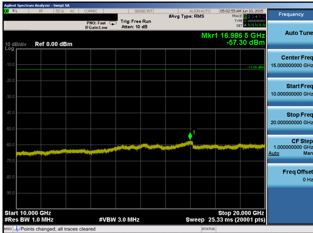
Plot 6-74. Conducted Spurious Plot (Band 4 – 20.0MHz QPSK – RB Size 1, RB Offset 0 – Mid Channel)
