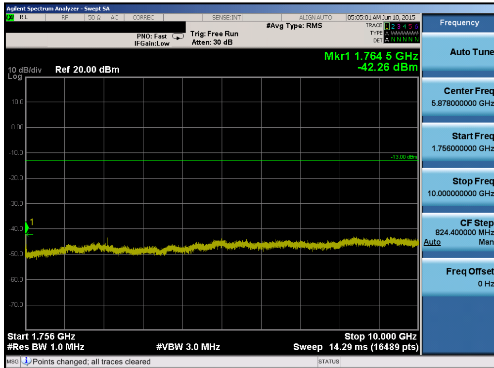
Plot 6-76. Conducted Spurious Plot (Band 4 – 20.0MHz QPSK – RB Size 1, RB Offset 0 – High Channel)
