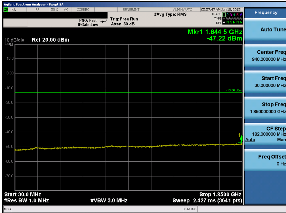
Plot 6-81. Conducted Spurious Plot (Band 25 – 20.0MHz QPSK – RB Size 1, RB Offset 0 – Mid Channel)
