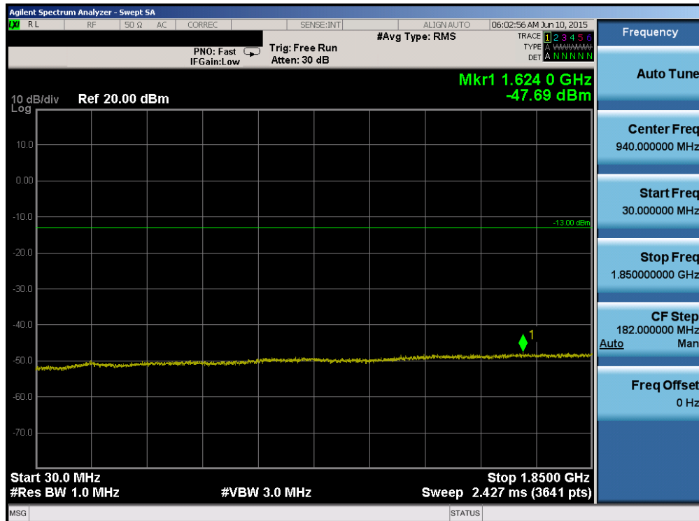
Plot 6-84. Conducted Spurious Plot (Band 25 – 20.0MHz QPSK – RB Size 1, RB Offset 0 – High Channel)
