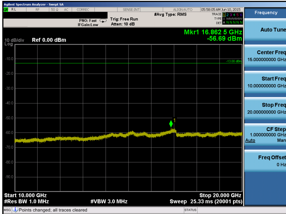
Plot 6-83. Conducted Spurious Plot (Band 25 – 20.0MHz QPSK – RB Size 1, RB Offset 0 – Mid Channel)
