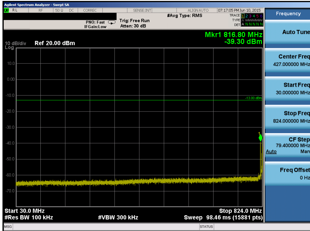
Plot 6-63. Conducted Spurious Plot (Band 26 – 15.0MHz QPSK – RB Size 1, RB Offset 0 – Mid Channel)
