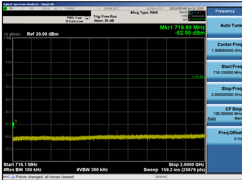
Plot 6-58. Conducted Spurious Plot (Band 12 – 10.0MHz QPSK – RB Size 1, RB Offset 0 – High Channel)
