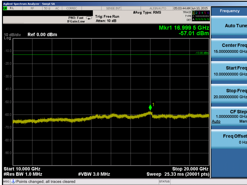
Plot 6-71. Conducted Spurious Plot (Band 4 – 20.0MHz QPSK – RB Size 1, RB Offset 0 – Low Channel)
