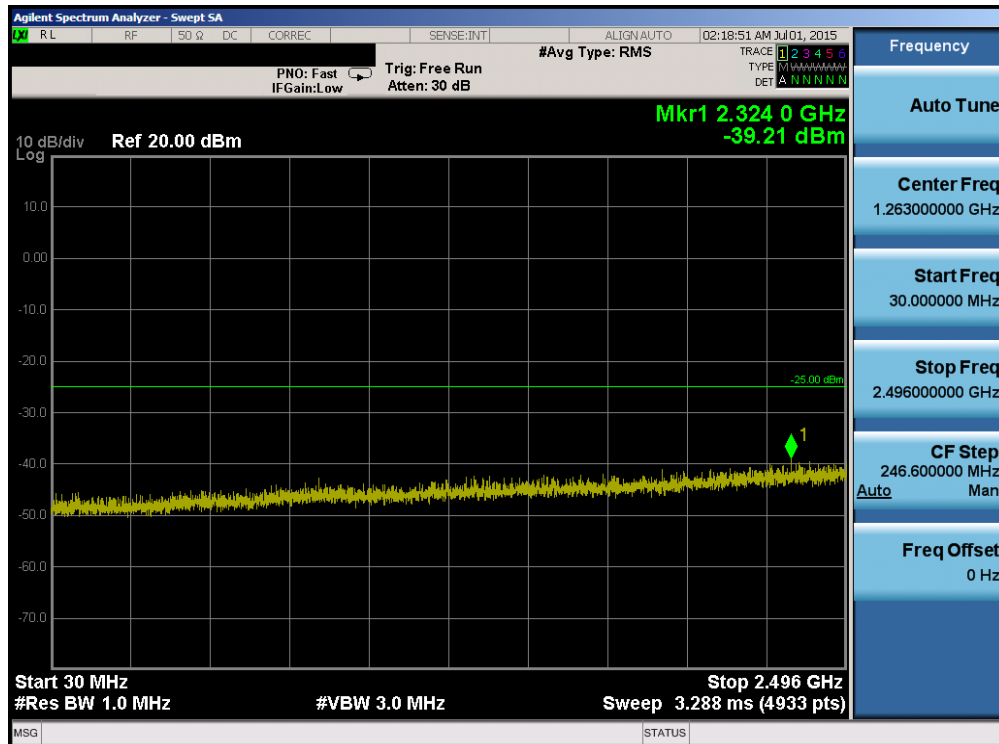
Plot 6-90. Conducted Spurious Plot (Band 41 – 20.0MHz QPSK – RB Size 1, RB Offset 0 – Mid Channel)
