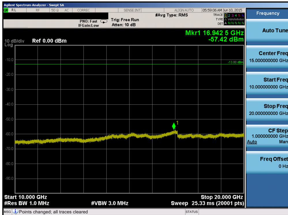
Plot 6-80. Conducted Spurious Plot (Band 25 - 20.0MHz QPSK - RB Size 1, RB Offset 0 - Low Channel)
