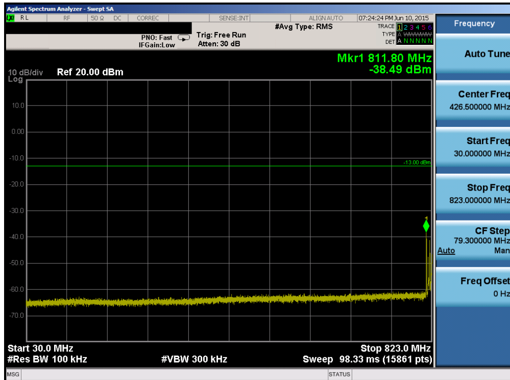
Plot 6-60. Conducted Spurious Plot (Band 26 – 15.0MHz QPSK – RB Size 1, RB Offset 0 – Low Channel)
