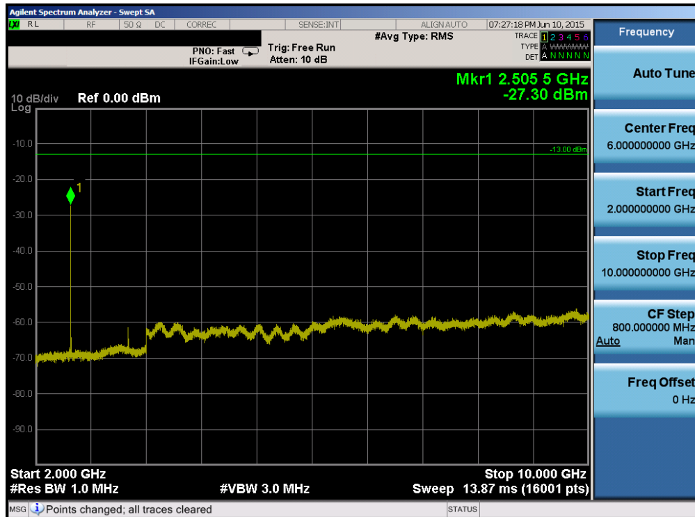
Plot 6-68. Conducted Spurious Plot (Band 26 – 15.0MHz QPSK – RB Size 1, RB Offset 0 – High Channel)
