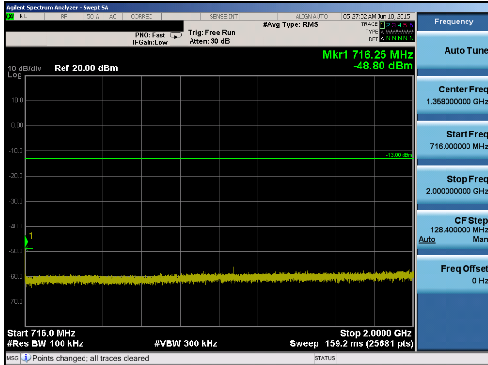
Plot 6-55. Conducted Spurious Plot (Band 12 – 10.0MHz QPSK – RB Size 1, RB Offset 0 – Mid Channel)
