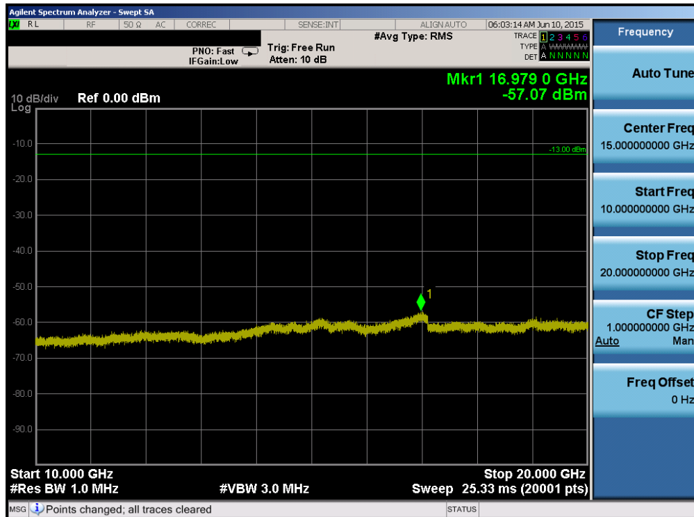
Plot 6-86. Conducted Spurious Plot (Band 25 – 20.0MHz QPSK – RB Size 1, RB Offset 0 – High Channel)
