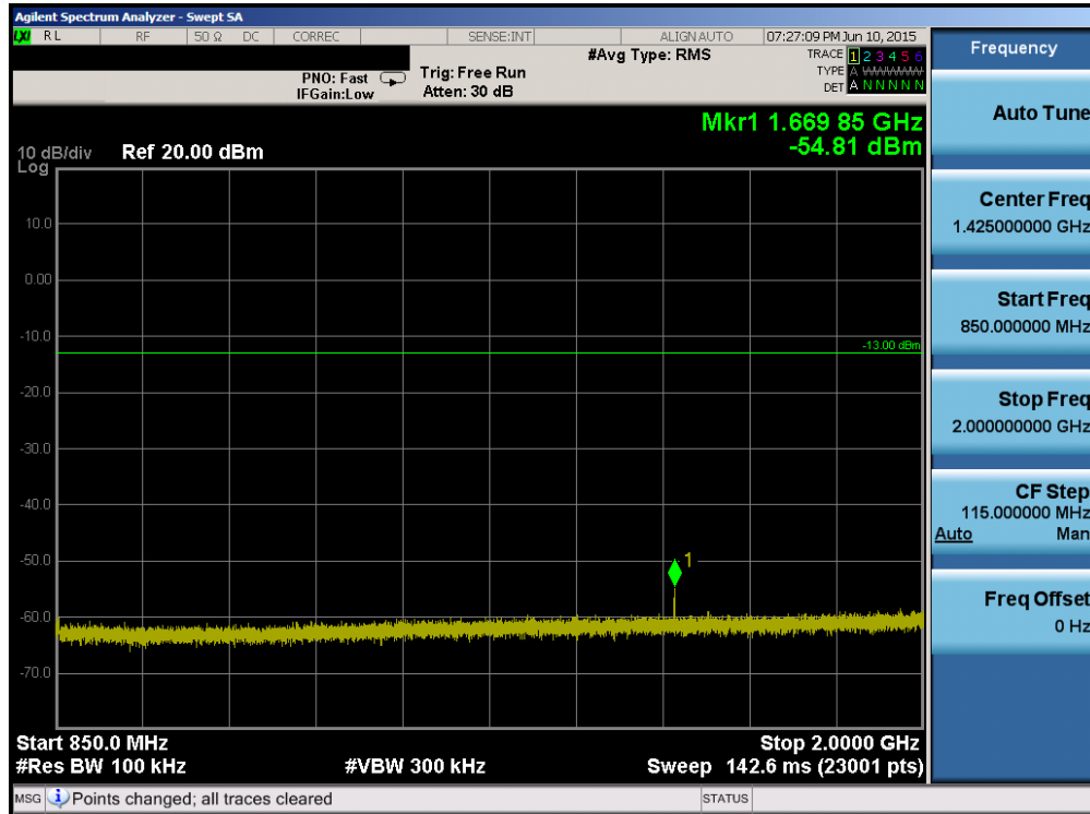
Plot 6-67. Conducted Spurious Plot (Band 26 – 15.0MHz QPSK – RB Size 1, RB Offset 0 – High Channel)
