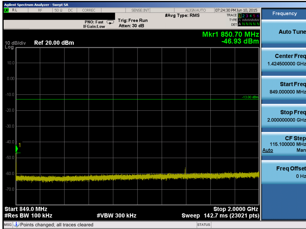
Plot 6-61. Conducted Spurious Plot (Band 26 – 15.0MHz QPSK – RB Size 1, RB Offset 0 – Low Channel)
