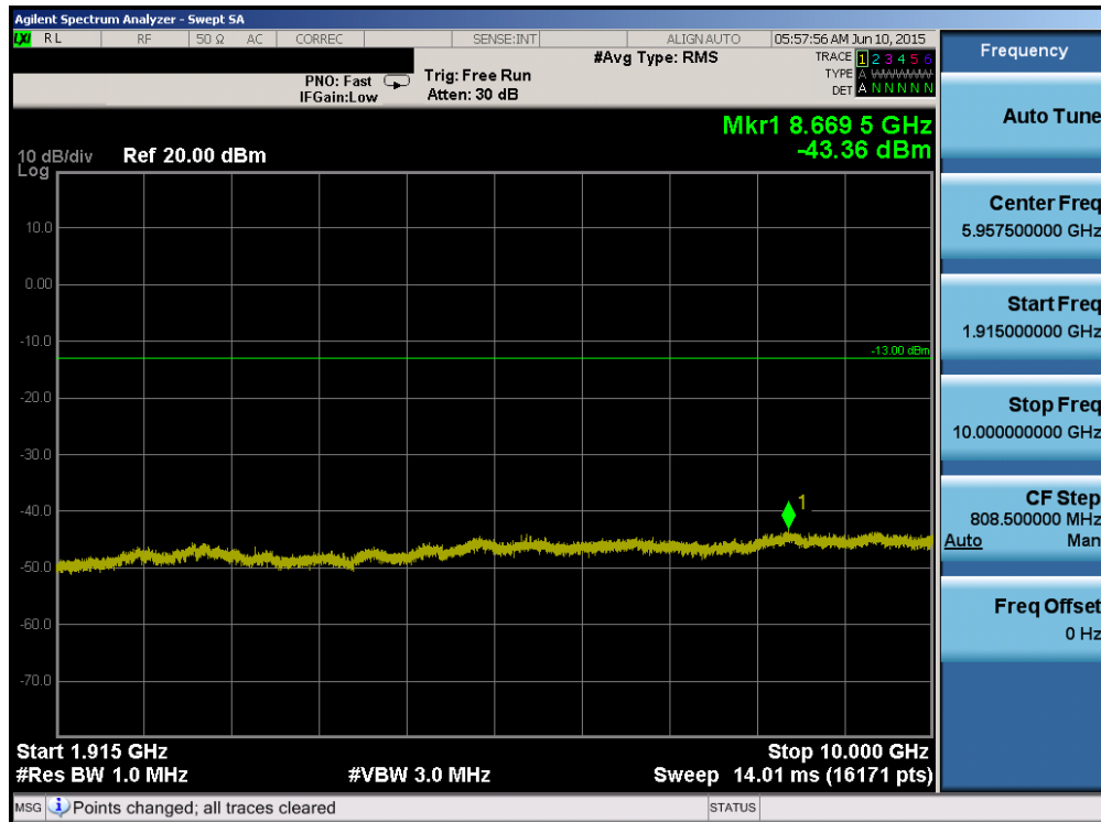
Plot 6-82. Conducted Spurious Plot (Band 25 – 20.0MHz QPSK – RB Size 1, RB Offset 0 – Mid Channel)
