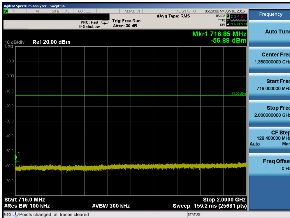
Plot 6-52. Conducted Spurious Plot (Band 12 – 10.0MHz QPSK – RB Size 1, RB Offset 0 – Low Channel)
