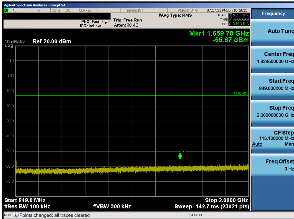
Plot 6-64. Conducted Spurious Plot (Band 26 – 15.0MHz QPSK – RB Size 1, RB Offset 0 – Mid Channel)
