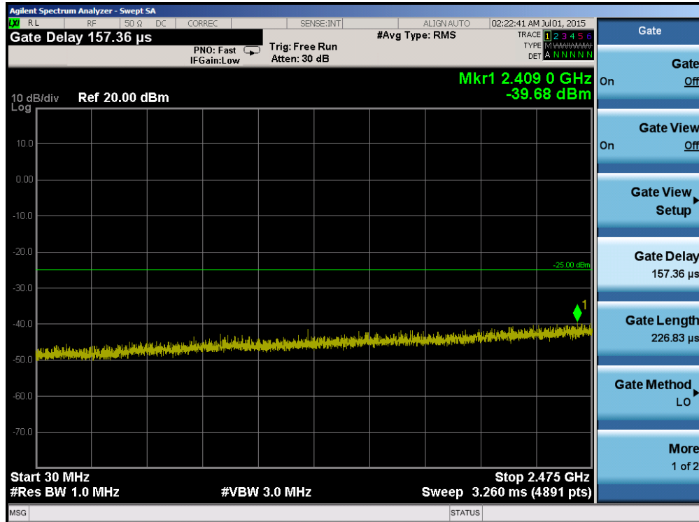
Plot 6-87. Conducted Spurious Plot (Band 41 – 20.0MHz QPSK – RB Size 1, RB Offset 0– Low Channel)
