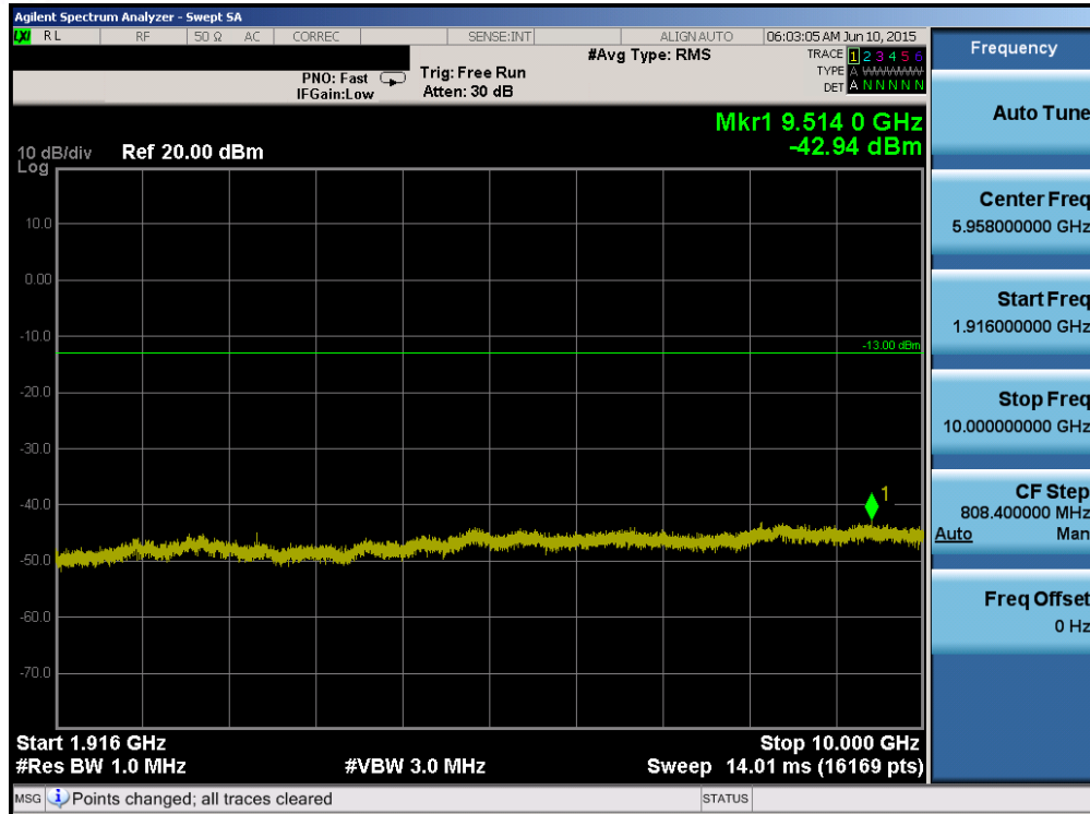
Plot 6-85. Conducted Spurious Plot (Band 25 – 20.0MHz QPSK – RB Size 1, RB Offset 0 – High Channel)
