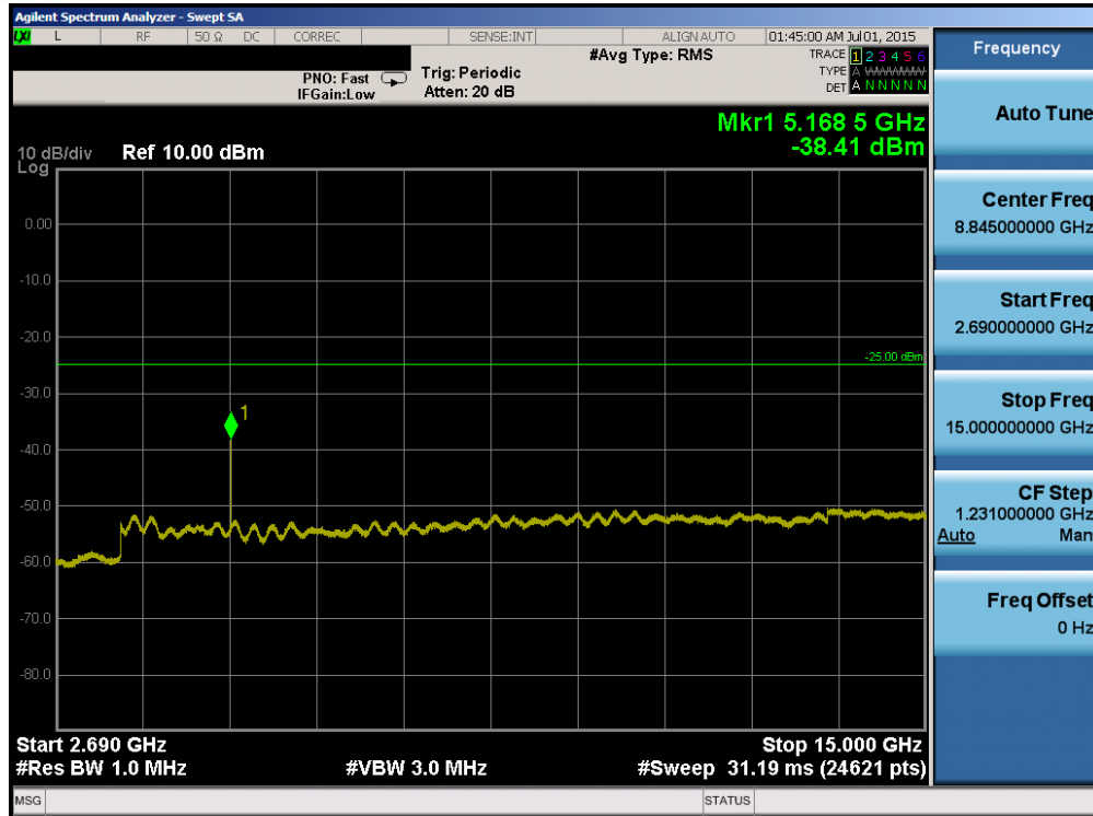
Plot 6-91. Conducted Spurious Plot (Band 41 – 20.0MHz QPSK – RB Size 1, RB Offset 0 – Mid Channel)
