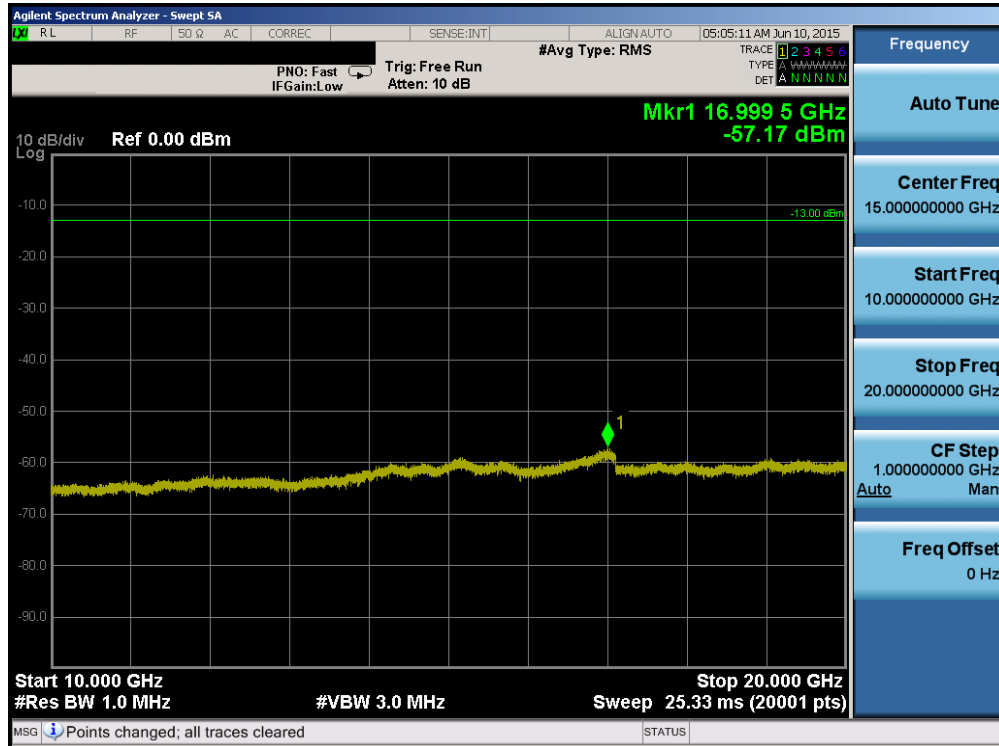
Plot 6-77. Conducted Spurious Plot (Band 4 – 20.0MHz QPSK – RB Size 1, RB Offset 0 – High Channel)
