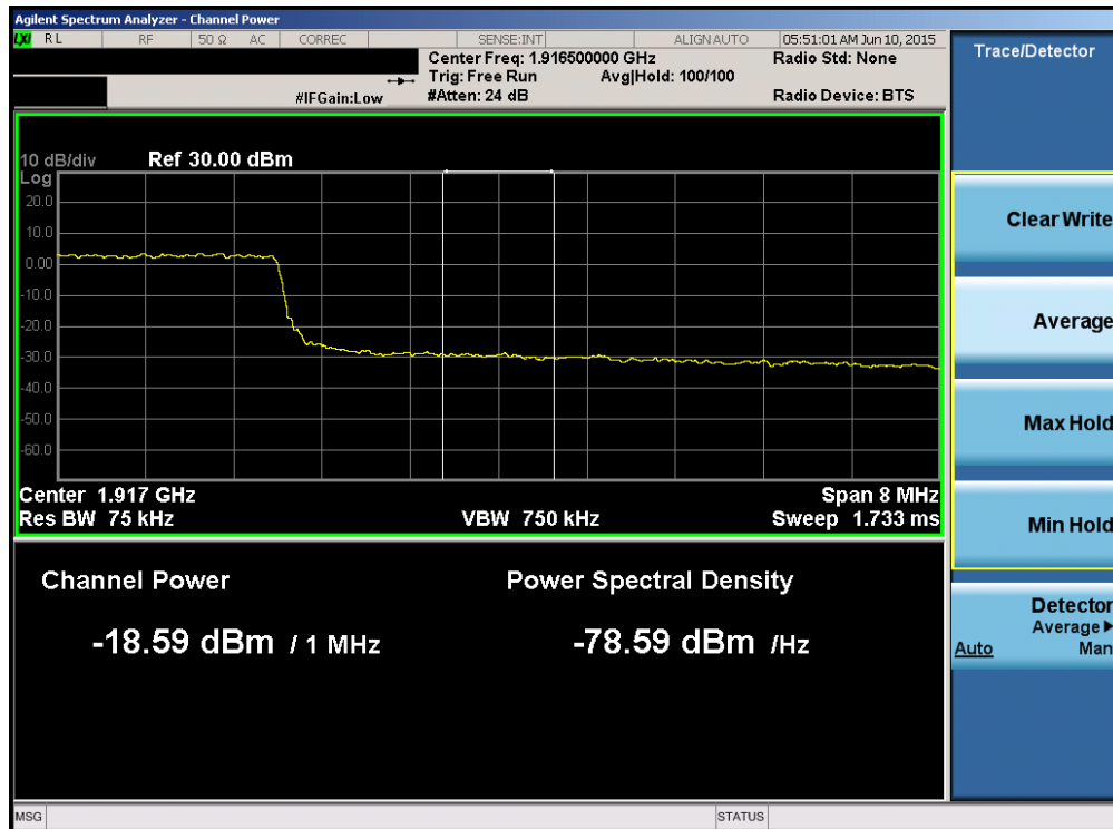
Plot 6-164. Upper Extended Band Edge Plot (Band 25 – 10.0MHz QPSK – RB Size 50)
