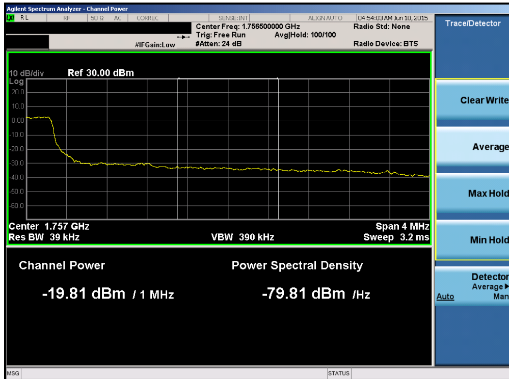
Plot 6-136. Upper Extended Band Edge Plot (Band 4 – 5.0MHz QPSK – RB Size 25)
