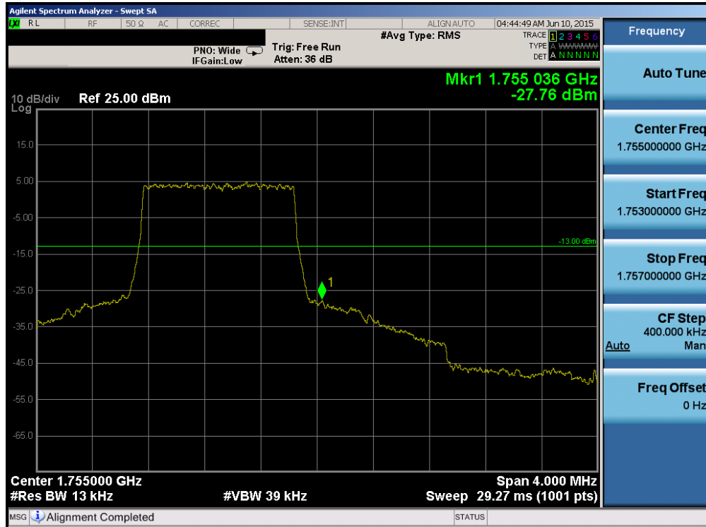
Plot 6-127. Upper Band Edge Plot (Band 4 – 1.4MHz QPSK – RB Size 6)
