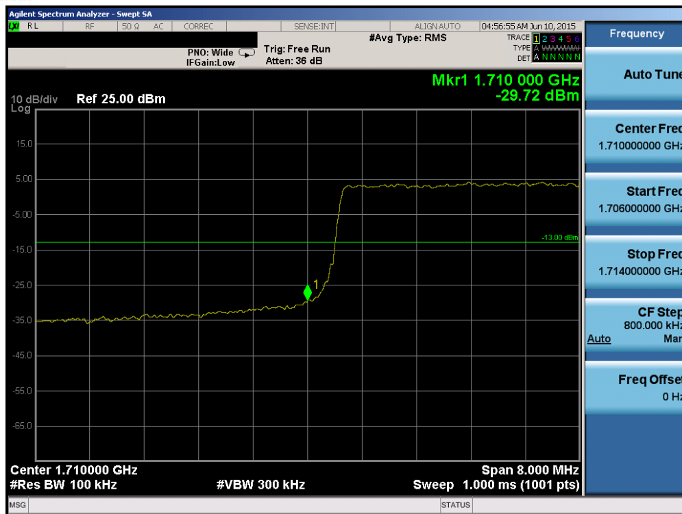
Plot 6-137. Lower Band Edge Plot (Band 4 – 10.0MHz QPSK – RB Size 50)
