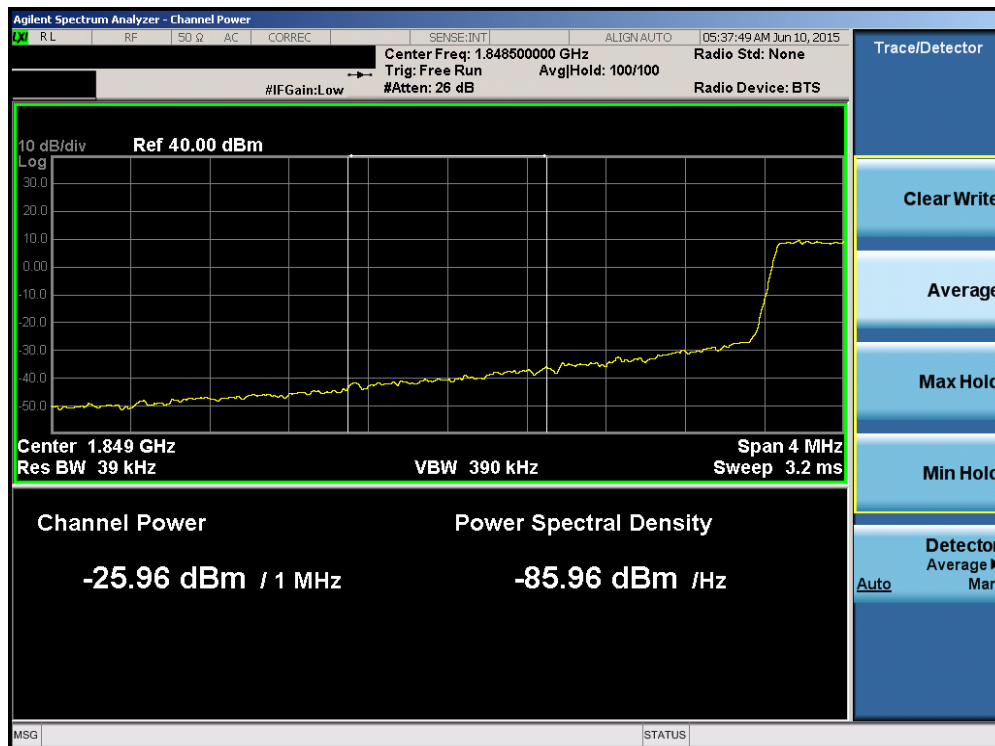
Plot 6-150. Lower Extended Band Edge Plot (Band 25 – 1.4MHz QPSK – RB Size 6)
