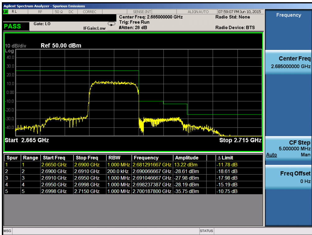
Plot 6-176. Upper Band Edge Plot (Band 41 – 10.0MHz QPSK – RB Size 50)
