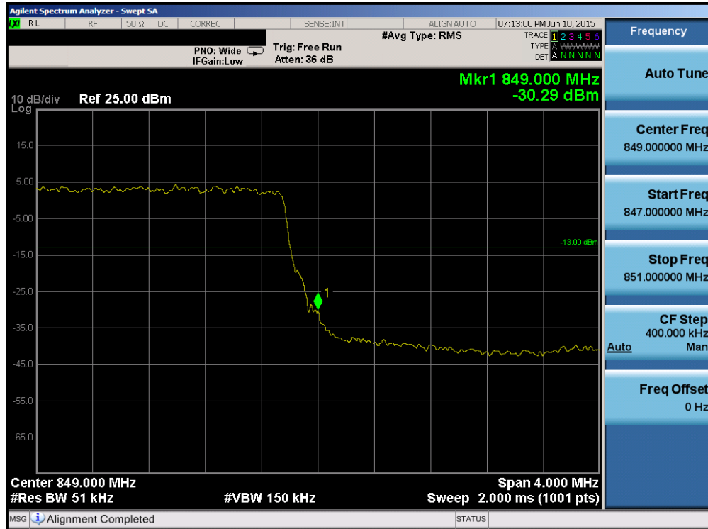
Plot 6-119. Upper Band Edge Plot (Band 26 – 5.0MHz QPSK – RB Size 25)
