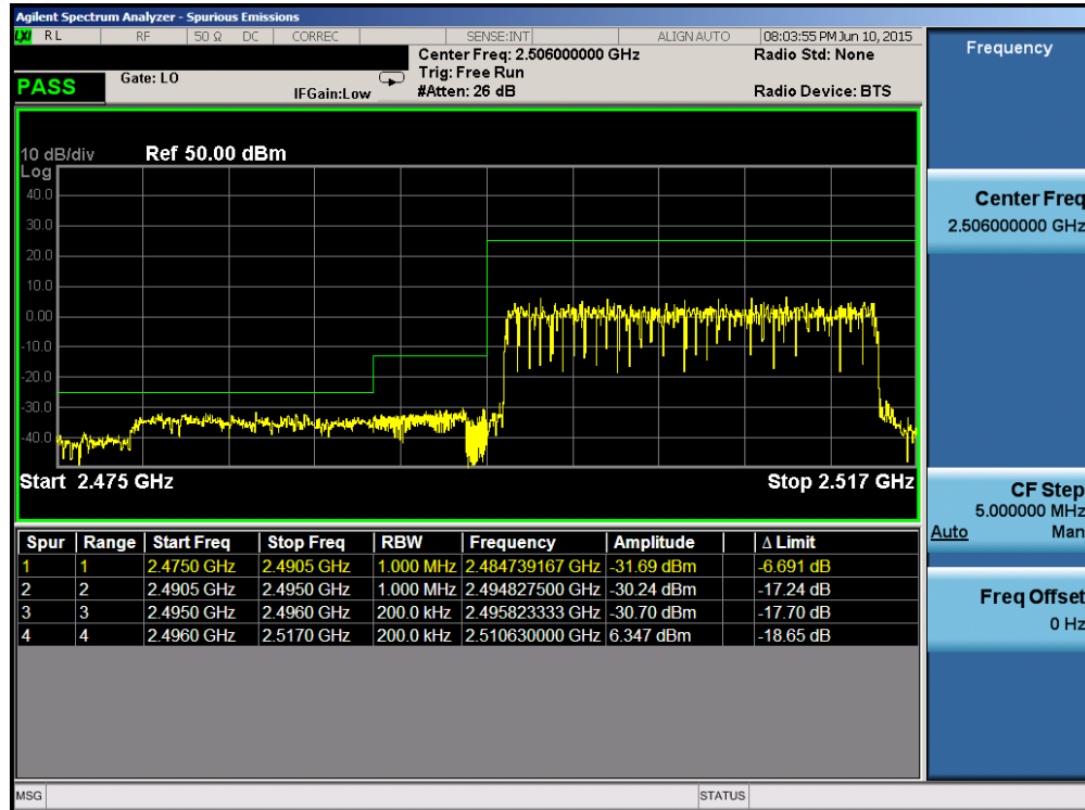
Plot 6-179. Lower Band Edge Plot (Band 41 – 20.0MHz QPSK – RB Size 100)
