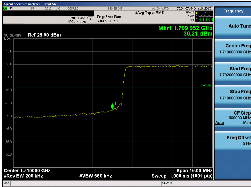
Plot 6-145. Lower Band Edge Plot (Band 4 – 20.0MHz QPSK – RB Size 100)
