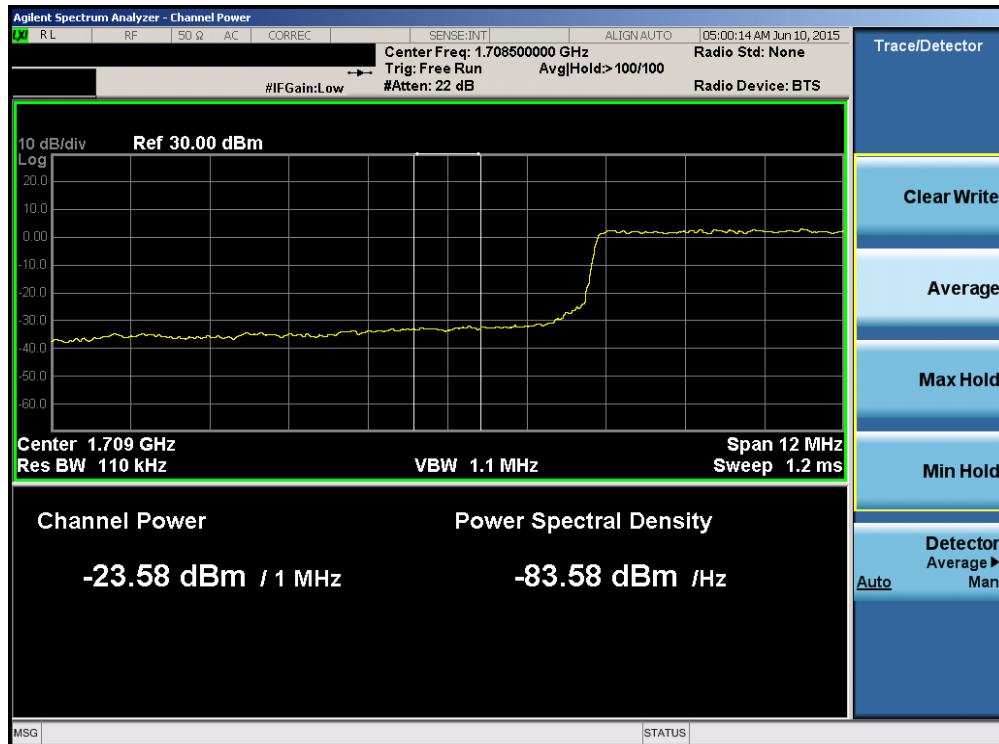
Plot 6-142. Lower Extended Band Edge Plot (Band 4 – 15.0MHz QPSK – RB Size 75)
