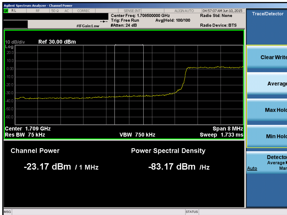
Plot 6-138. Lower Extended Band Edge Plot (Band 4 – 10.0MHz QPSK – RB Size 50)
