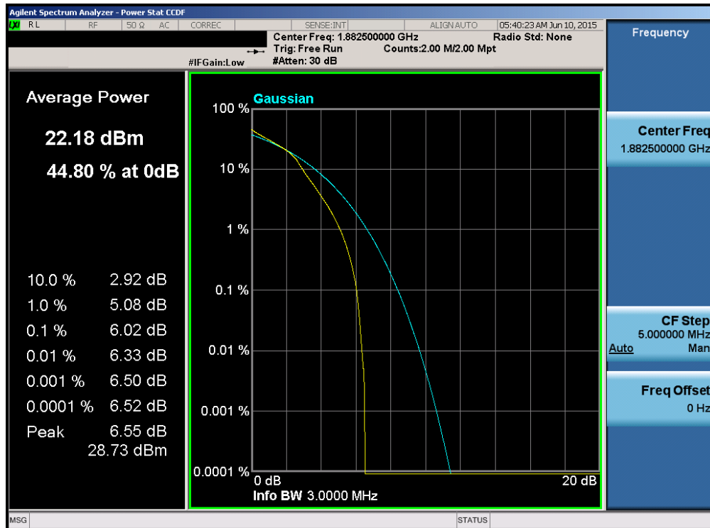
Plot 6-184. PAR Plot (Band 25 – 3.0MHz 16-QAM – RB Size 15)
