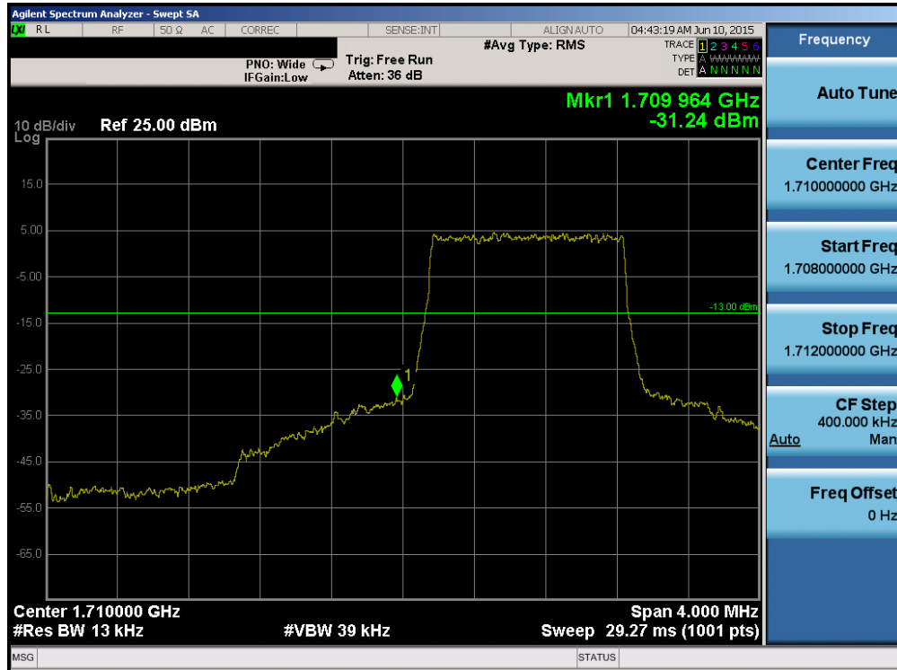
Plot 6-125. Lower Band Edge Plot (Band 4 – 1.4MHz QPSK – RB Size 6)
