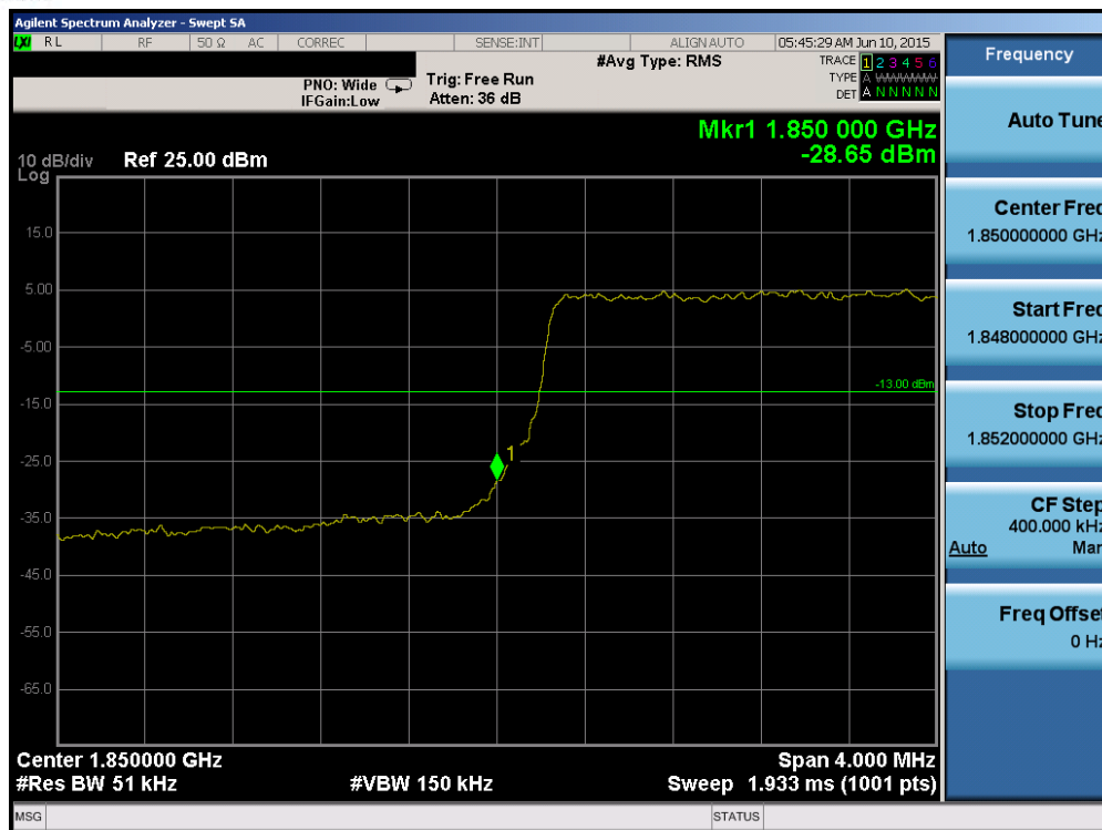
Plot 6-157. Lower Band Edge Plot (Band 25 – 5.0MHz QPSK – RB Size 25)
