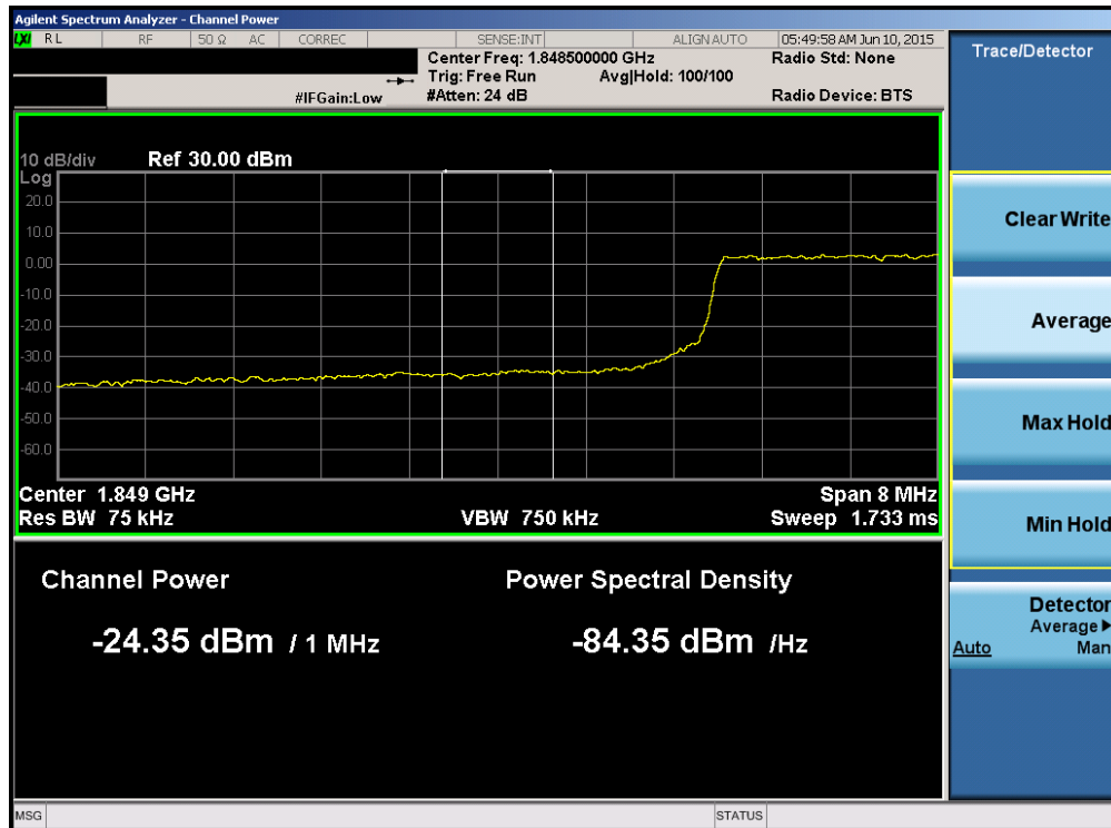
Plot 6-162. Lower Extended Band Edge Plot (Band 25 – 10.0MHz QPSK – RB Size 50)
