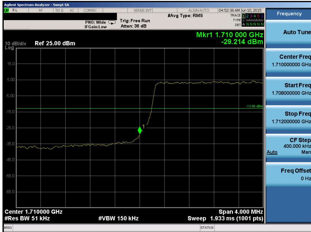
Plot 6-133. Lower Band Edge Plot (Band 4 – 5.0MHz QPSK – RB Size 25)
