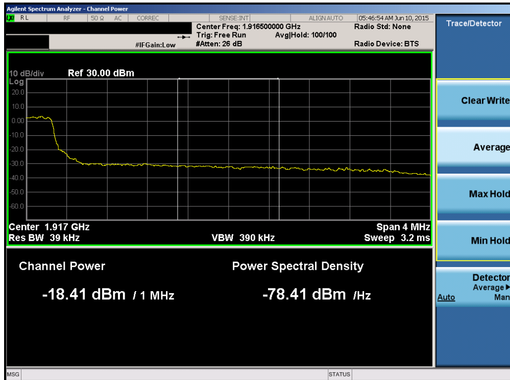
Plot 6-160. Upper Extended Band Edge Plot (Band 25 – 5.0MHz QPSK – RB Size 25)
