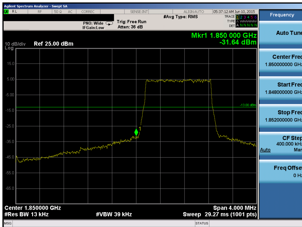
Plot 6-149. Lower Band Edge Plot (Band 25 – 1.4MHz QPSK – RB Size 6)
