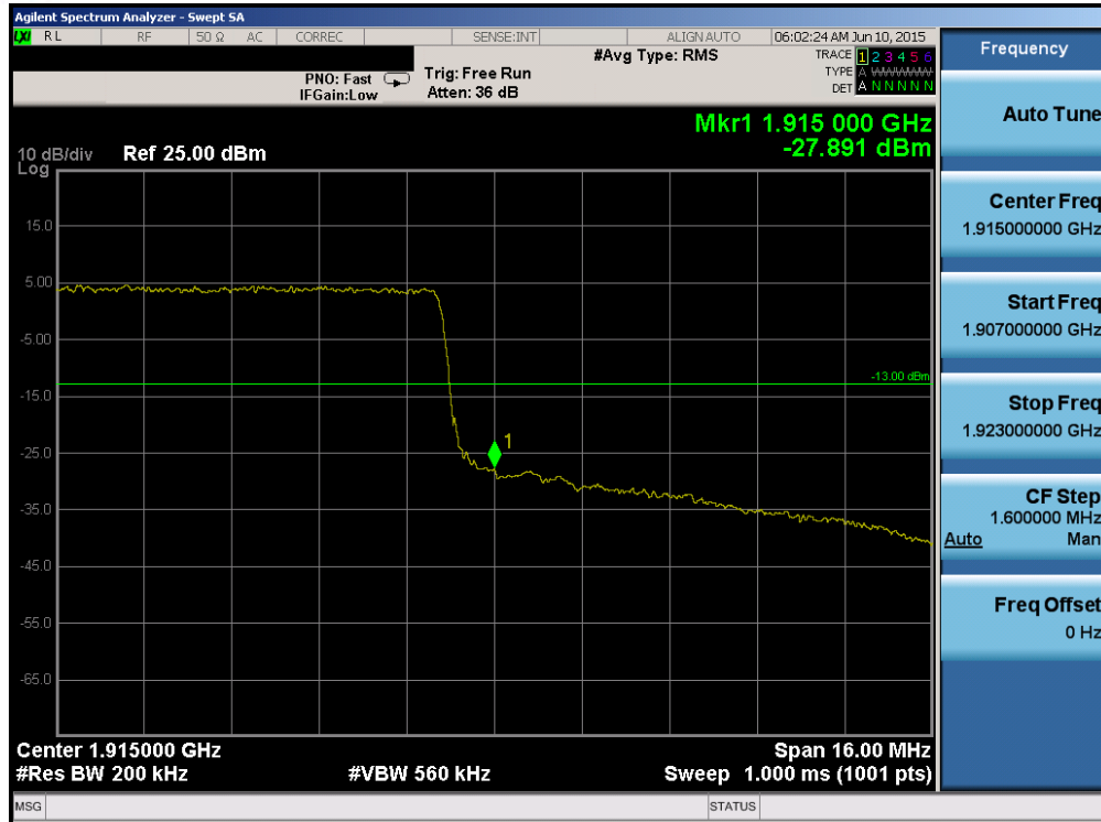
Plot 6-171. Upper Band Edge Plot (Band 25 – 20.0MHz QPSK – RB Size 100)
