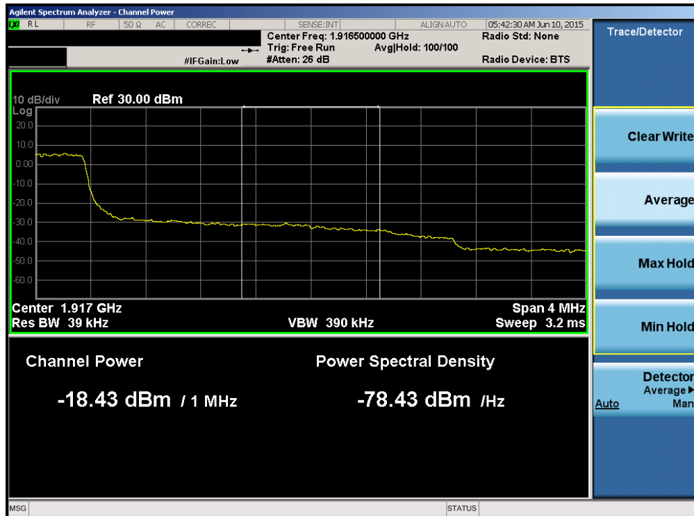
Plot 6-156. Upper Extended Band Edge Plot (Band 25 – 3.0MHz QPSK – RB Size 15)
