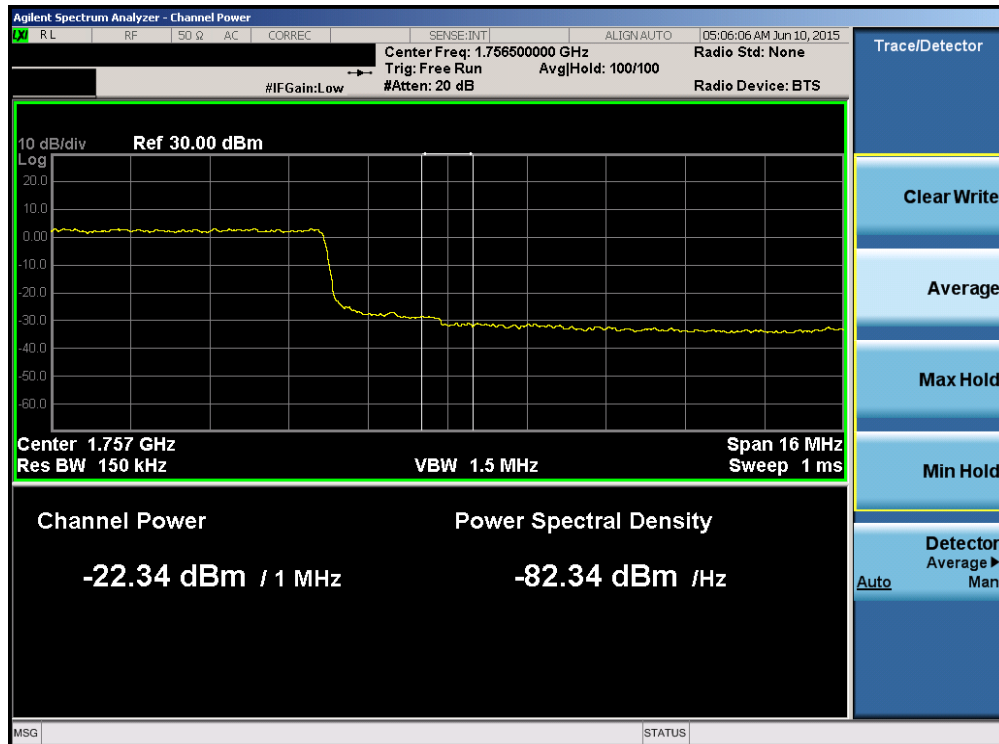
Plot 6-148. Upper Extended Band Edge Plot (Band 4 – 20.0MHz QPSK – RB Size 100)
