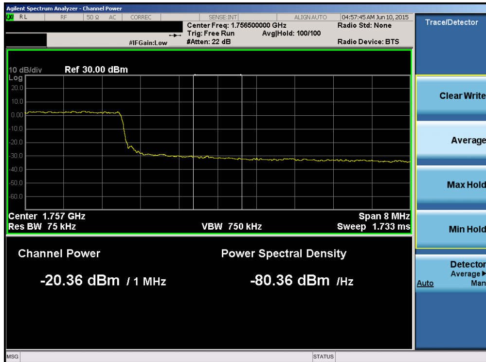
Plot 6-140. Upper Extended Band Edge Plot (Band 4 – 10.0MHz QPSK – RB Size 50)
