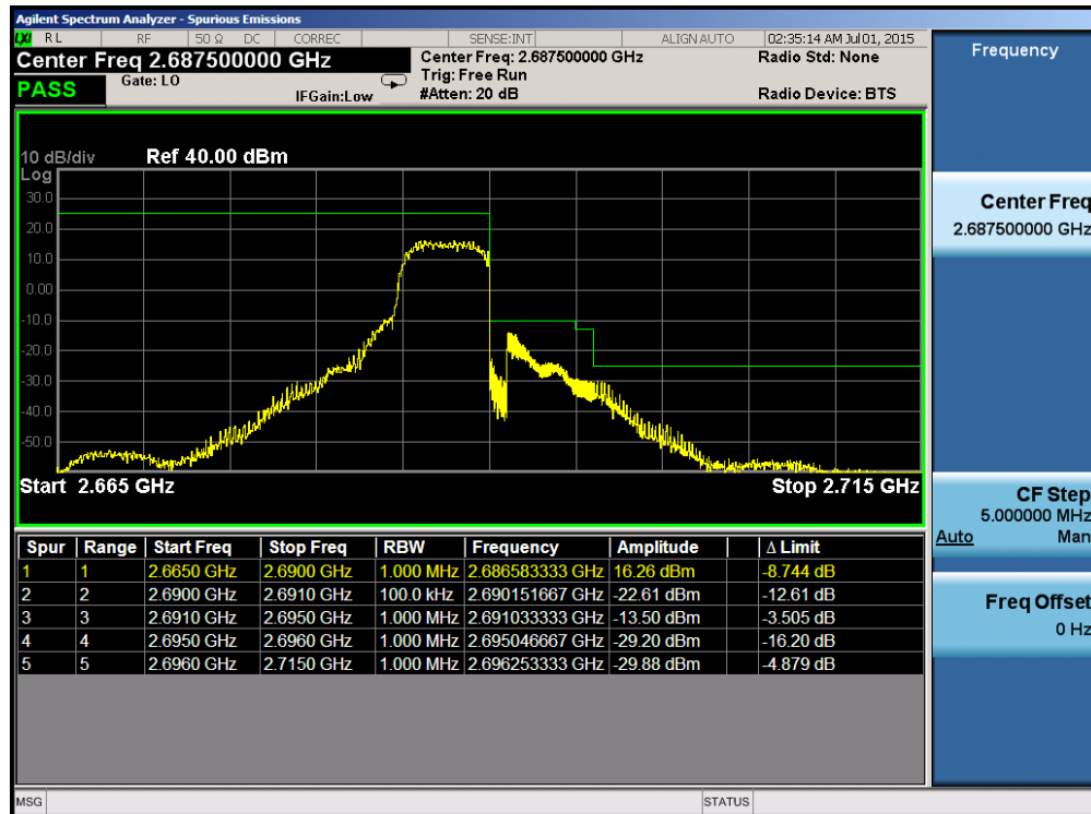
Plot 6-174. Upper Band Edge Plot (Band 41 – 5.0MHz QPSK – RB Size 25)
