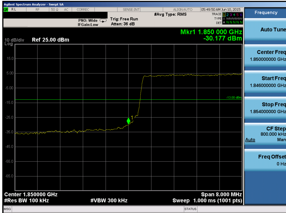
Plot 6-161. Lower Band Edge Plot (Band 25 – 10.0MHz QPSK – RB Size 50)
