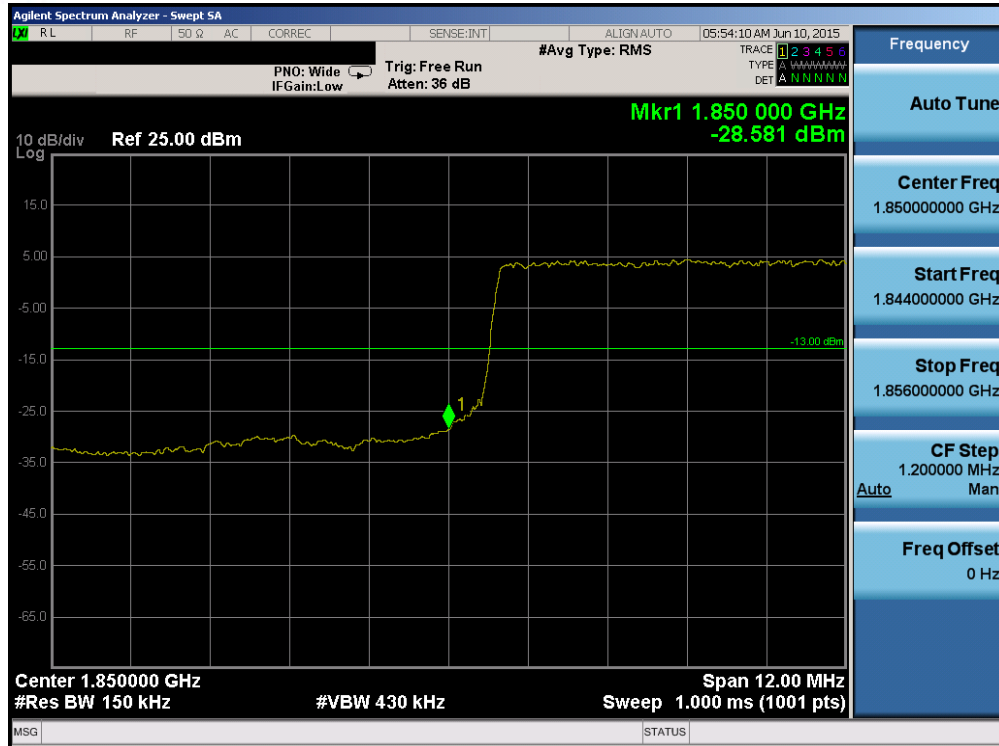
Plot 6-165. Lower Band Edge Plot (Band 25 – 15.0MHz QPSK – RB Size 75)
