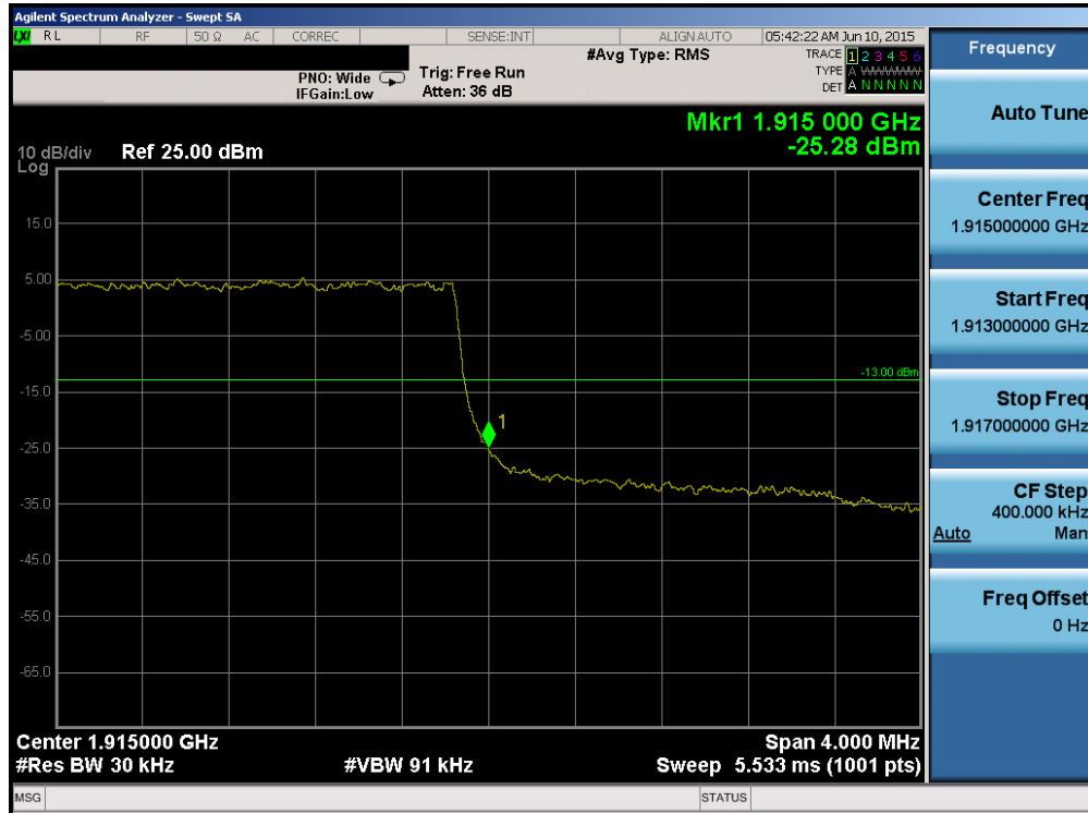
Plot 6-155. Upper Band Edge Plot (Band 25 – 3.0MHz QPSK – RB Size 15)
