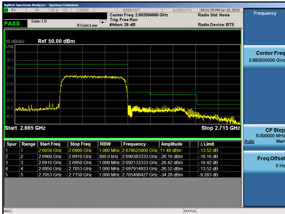
Plot 6-178. Upper Band Edge Plot (Band 41 – 15.0MHz QPSK – RB Size 75)
