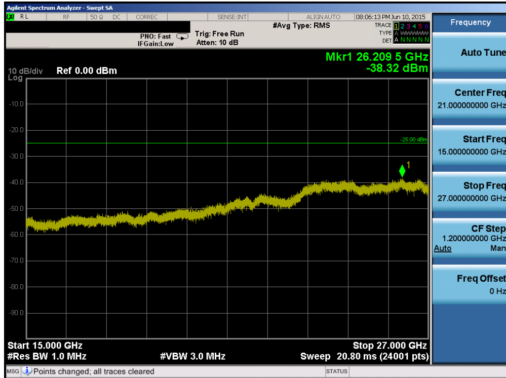
Plot 6-95. Conducted Spurious Plot (Band 41 – 20.0MHz QPSK – RB Size 1, RB Offset 0 – High Channel)
