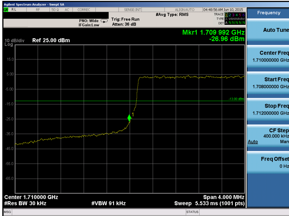
Plot 6-129. Lower Band Edge Plot (Band 4 – 3.0MHz QPSK – RB Size 15)
