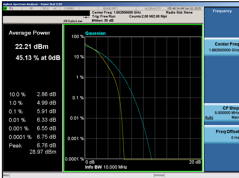
Plot 6-188. PAR Plot (Band 25 – 10.0MHz 16-QAM – RB Size 50)
