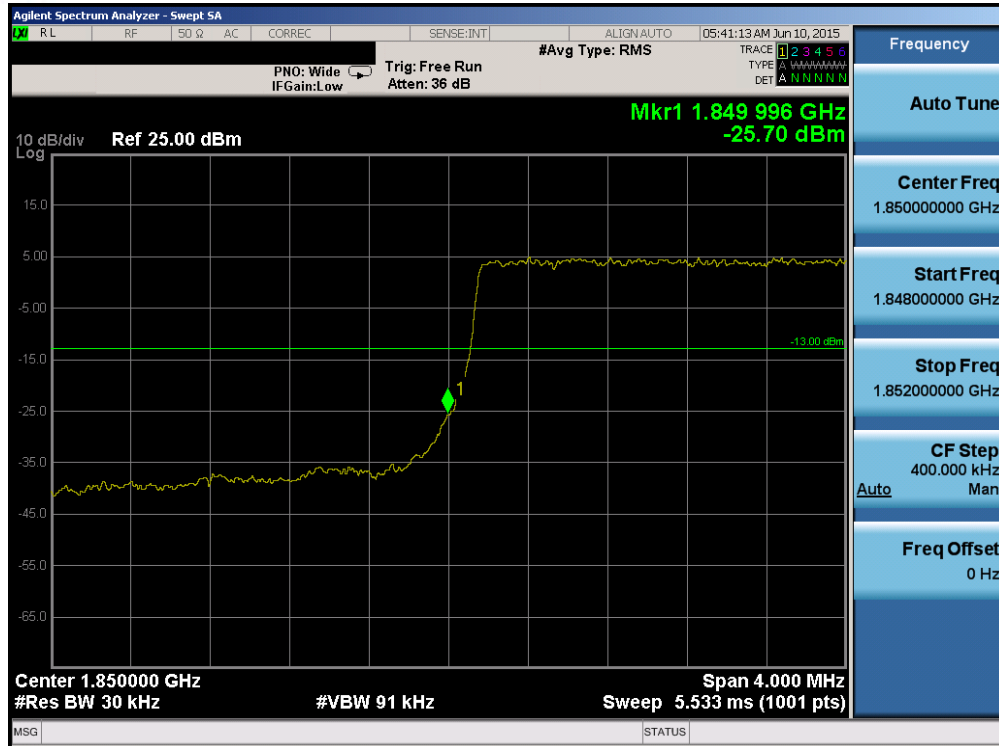
Plot 6-153. Lower Band Edge Plot (Band 25 – 3.0MHz QPSK – RB Size 15)
