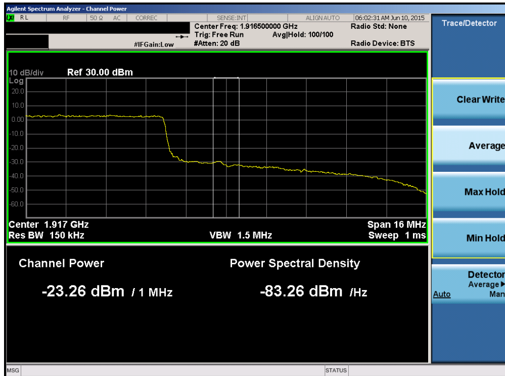
Plot 6-172. Upper Extended Band Edge Plot (Band 25 – 20.0MHz QPSK – RB Size 100)
