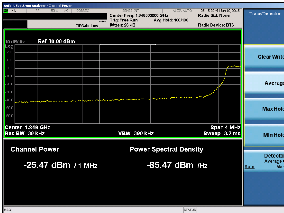
Plot 6-158. Lower Extended Band Edge Plot (Band 25 – 5.0MHz QPSK – RB Size 25)
