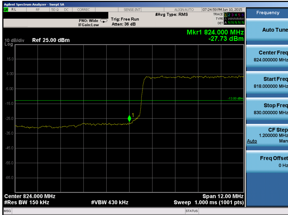
Plot 6-123. Lower Band Edge Plot (Band 26 – 15.0MHz QPSK – RB Size 75)
