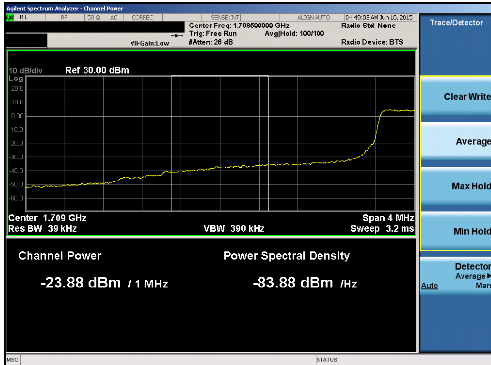
Plot 6-130. Lower Extended Band Edge Plot (Band 4 – 3.0MHz QPSK – RB Size 15)
