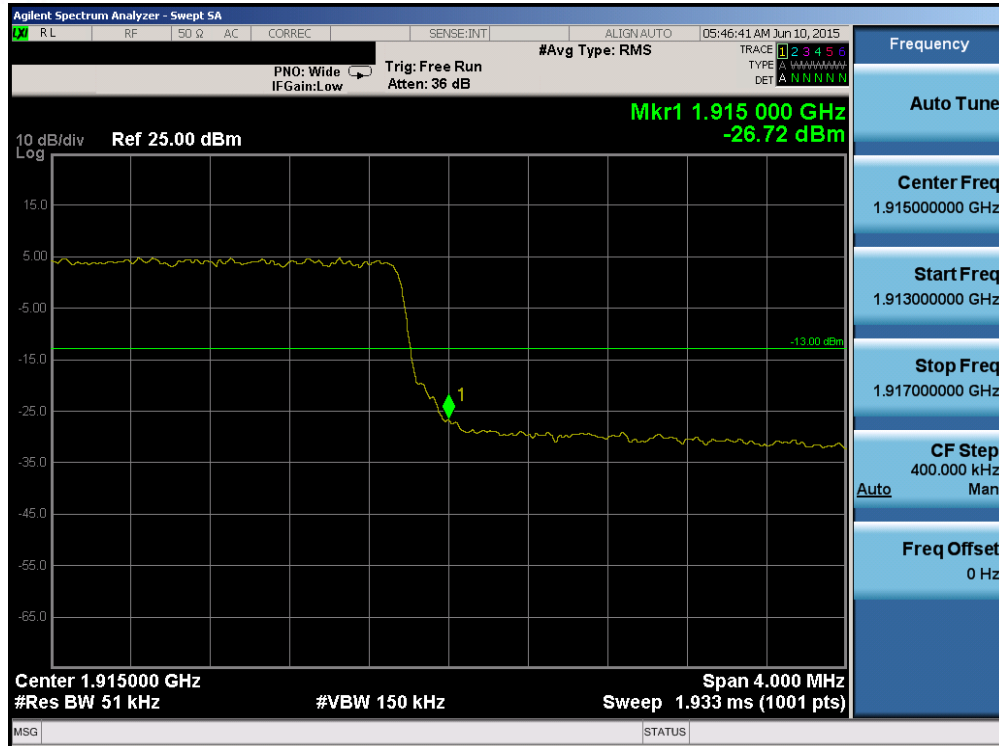
Plot 6-159. Upper Band Edge Plot (Band 25 – 5.0MHz QPSK – RB Size 25)
