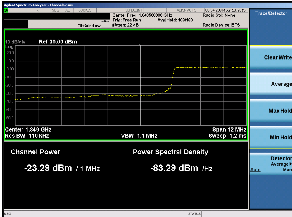
Plot 6-166. Lower Extended Band Edge Plot (Band 25 – 15.0MHz QPSK – RB Size 75)
