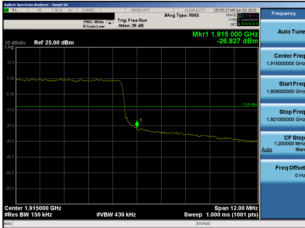
Plot 6-167. Upper Band Edge Plot (Band 25 – 15.0MHz QPSK – RB Size 75)
