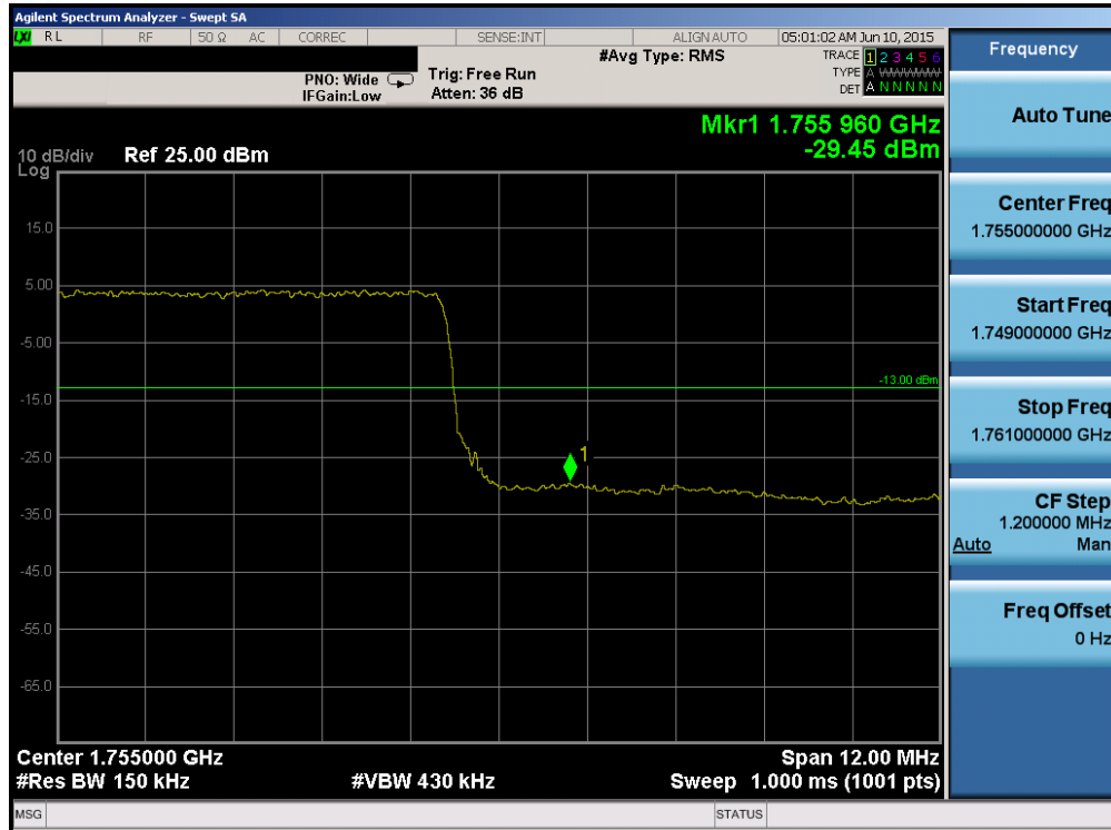
Plot 6-143. Upper Band Edge Plot (Band 4 – 15.0MHz QPSK – RB Size 75)
