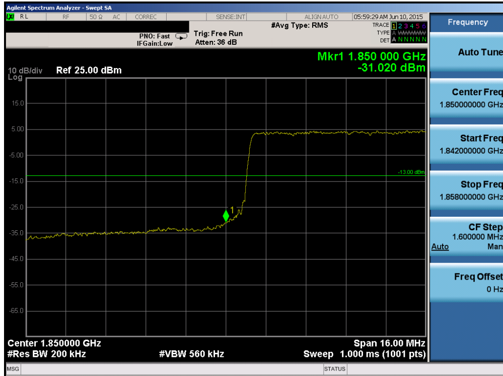
Plot 6-169. Lower Band Edge Plot (Band 25 – 20.0MHz QPSK – RB Size 100)
