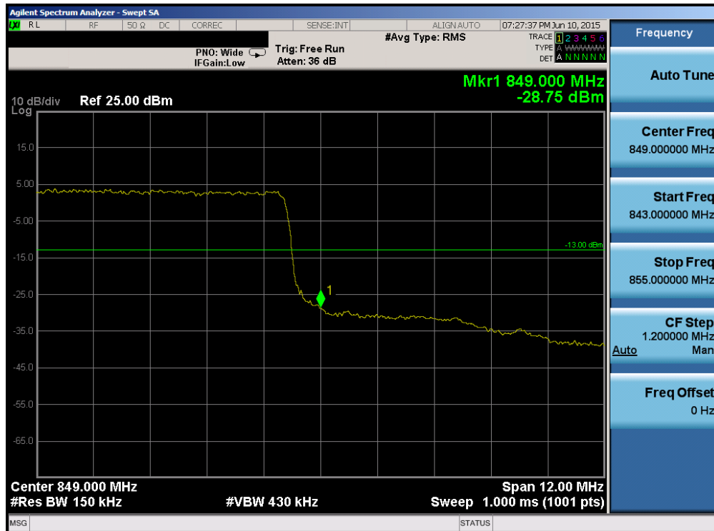
Plot 6-124. Upper Band Edge Plot (Band 26 – 15.0MHz QPSK – RB Size 75)
