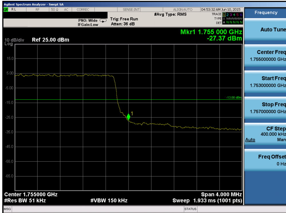
Plot 6-135. Upper Band Edge Plot (Band 4 – 5.0MHz QPSK – RB Size 25)
