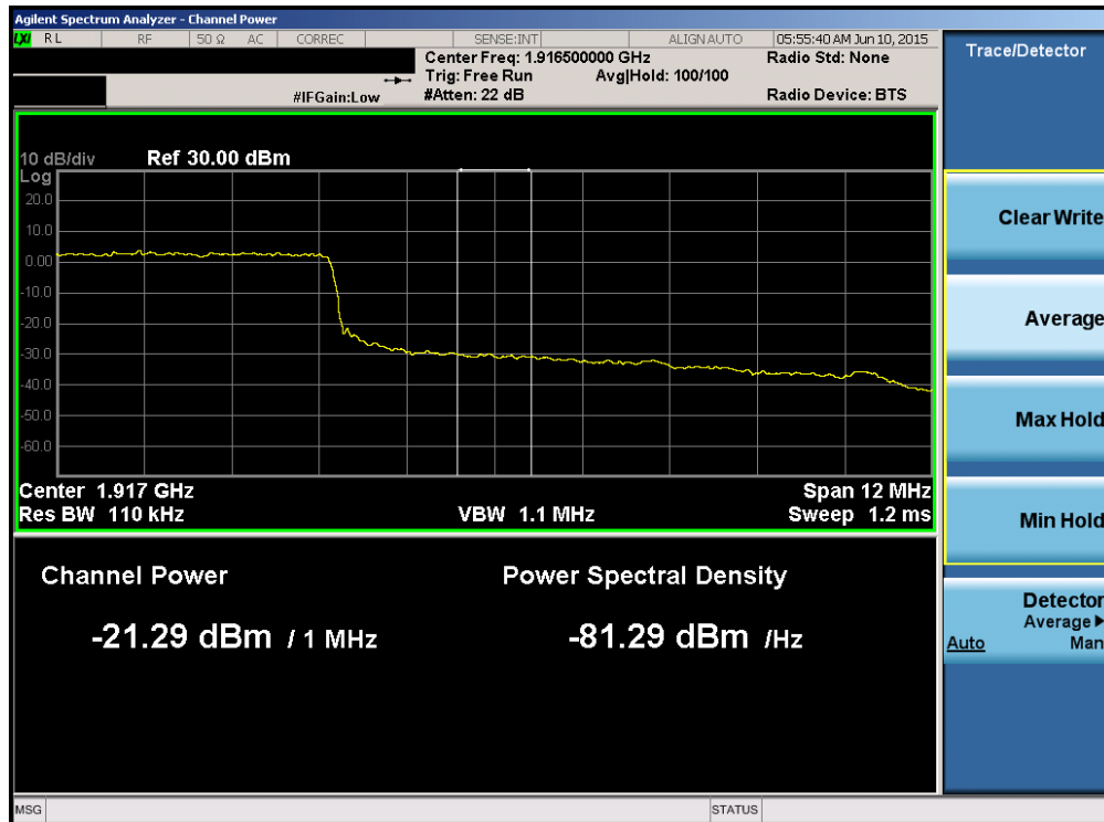
Plot 6-168. Upper Extended Band Edge Plot (Band 25 – 15.0MHz QPSK – RB Size 75)
