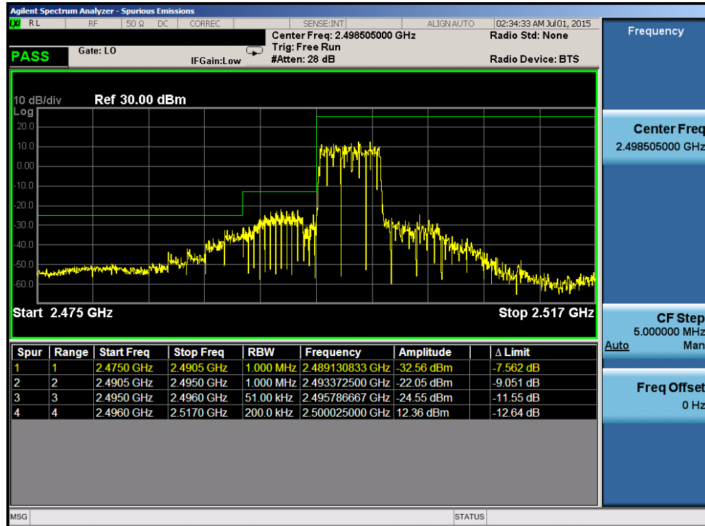
Plot 6-173. Lower Band Edge Plot (Band 41 – 5.0MHz QPSK – RB Size 25)
