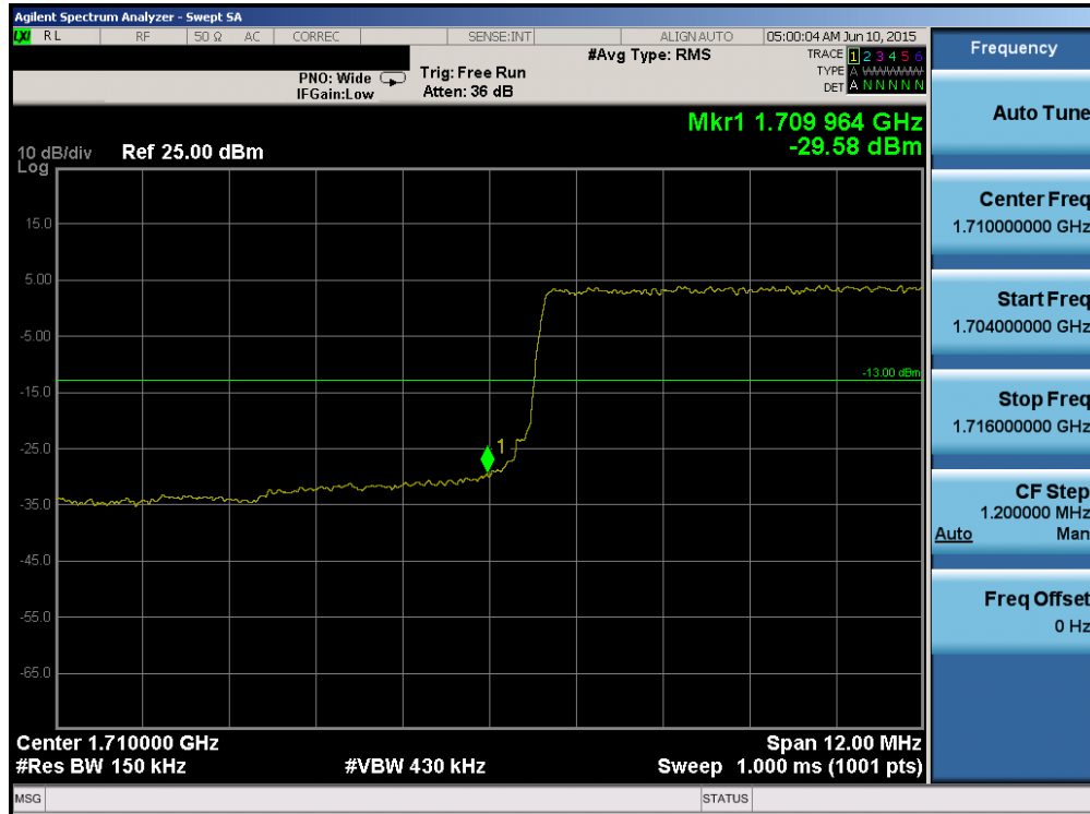
Plot 6-141. Lower Band Edge Plot (Band 4 – 15.0MHz QPSK – RB Size 75)
