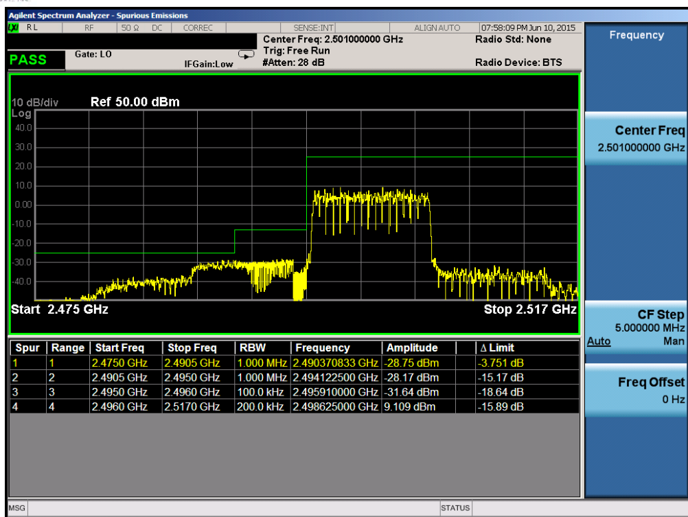
Plot 6-175. Lower Band Edge Plot (Band 41 – 10.0MHz QPSK – RB Size 50)
