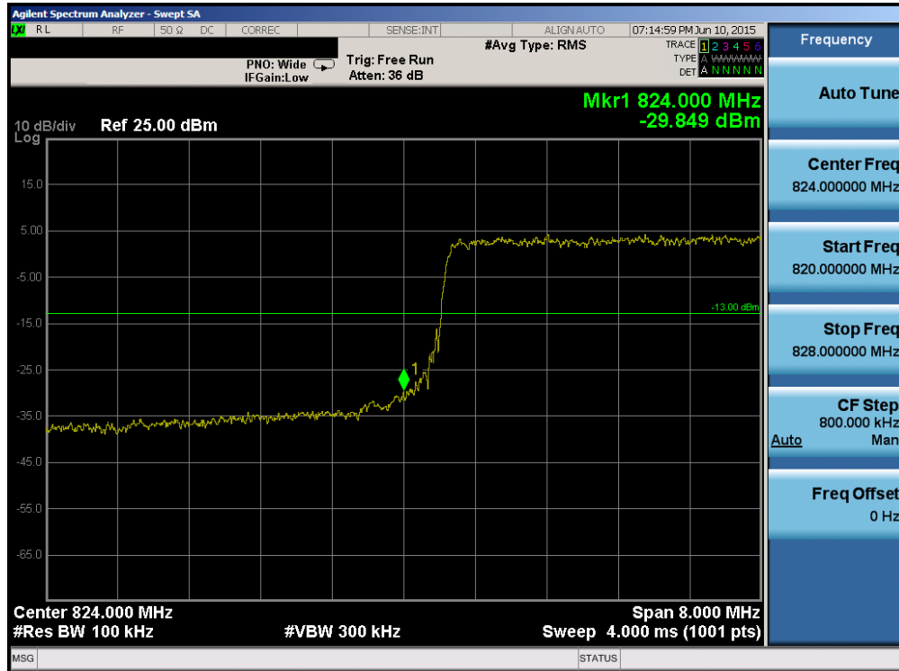
Plot 6-121. Lower Band Edge Plot (Band 26 – 10.0MHz QPSK – RB Size 50)
