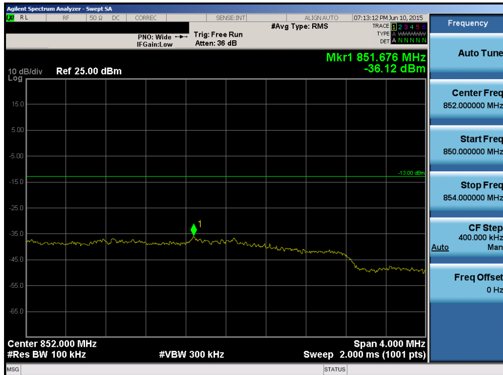
Plot 6-120. Upper Extended Band Edge Plot (Band 26 – 5.0MHz QPSK – RB Size 25)
