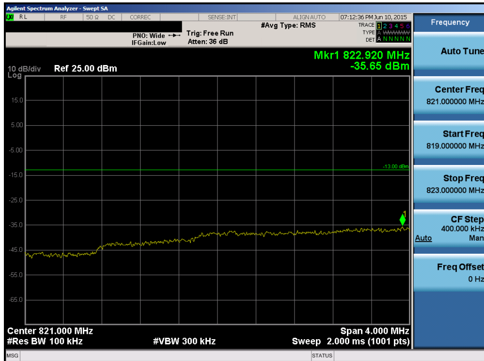
Plot 6-118. Lower Extended Band Edge Plot (Band 26 – 5.0MHz QPSK – RB Size 25)
