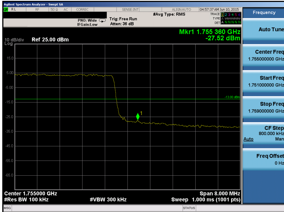
Plot 6-139. Upper Band Edge Plot (Band 4 – 10.0MHz QPSK – RB Size 50)
