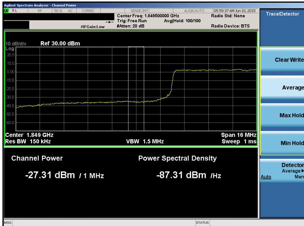
Plot 6-170. Lower Extended Band Edge Plot (Band 25 – 20.0MHz QPSK – RB Size 100)
