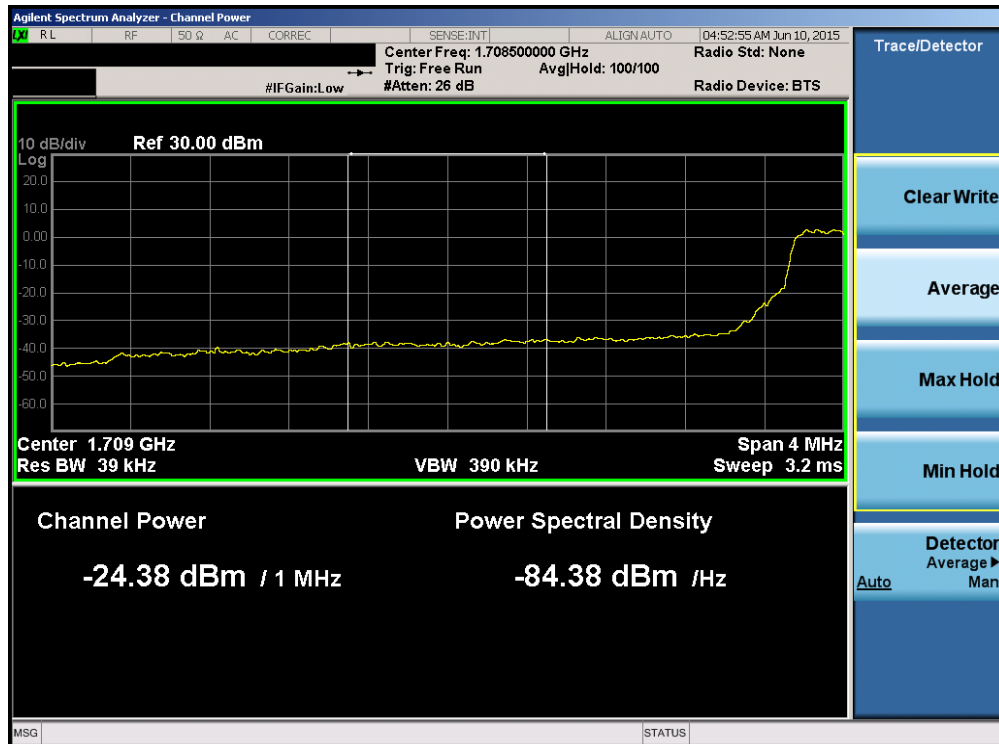
Plot 6-134. Lower Extended Band Edge Plot (Band 4 – 5.0MHz QPSK – RB Size 25)
