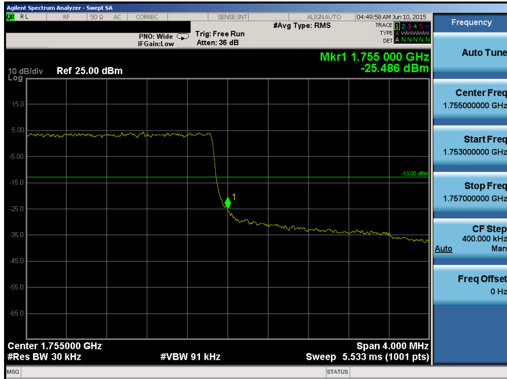
Plot 6-131. Upper Band Edge Plot (Band 4 – 3.0MHz QPSK – RB Size 15)
