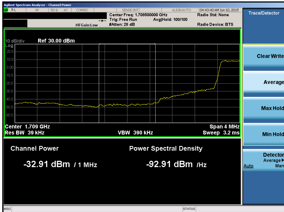
Plot 6-126. Lower Extended Band Edge Plot (Band 4 – 1.4MHz QPSK – RB Size 6)
