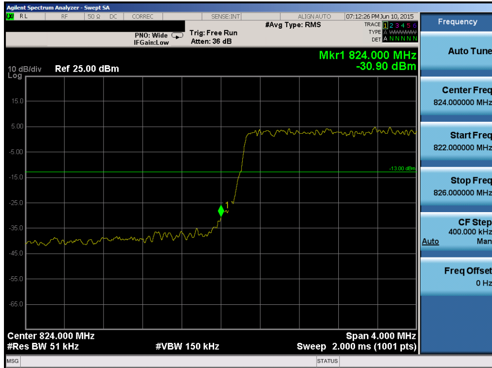
Plot 6-117. Lower Band Edge Plot (Band 26 – 5.0MHz QPSK – RB Size 25)
