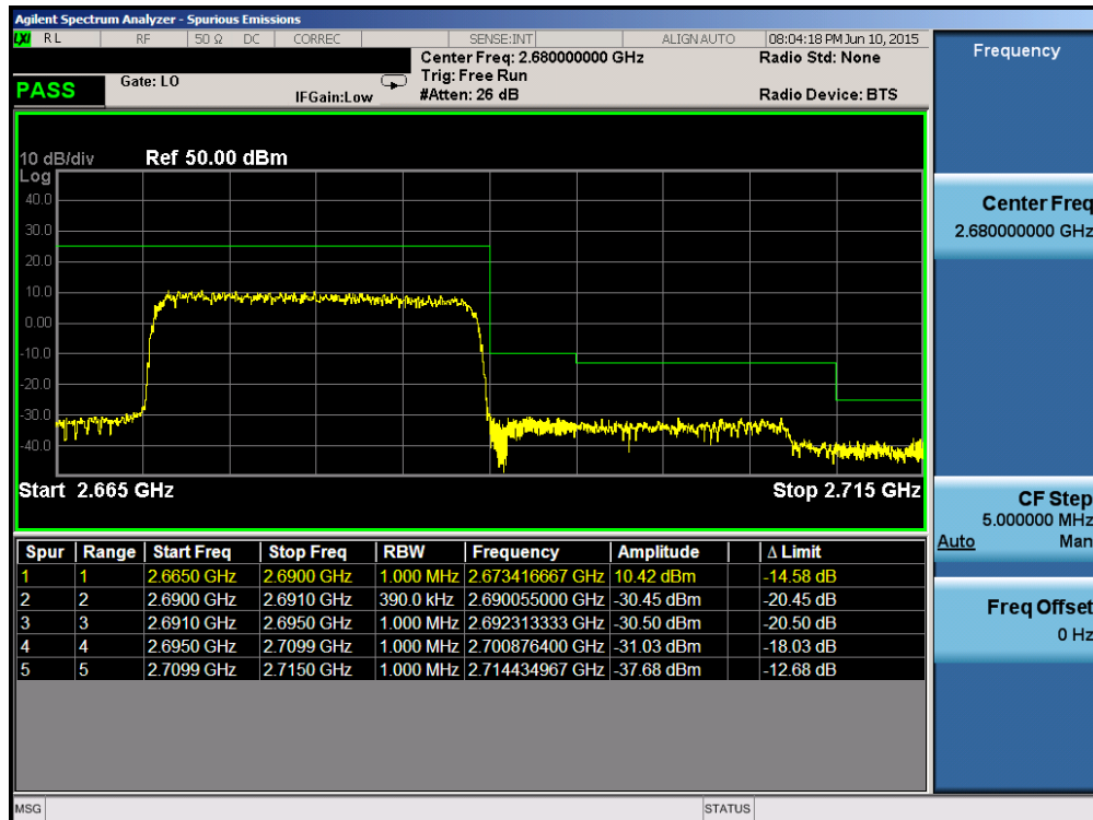
Plot 6-180. Upper Band Edge Plot (Band 41 – 20.0MHz QPSK – RB Size 100)
