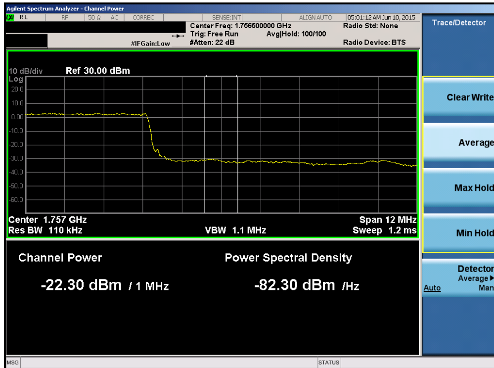
Plot 6-144. Upper Extended Band Edge Plot (Band 4 – 15.0MHz QPSK – RB Size 75)
