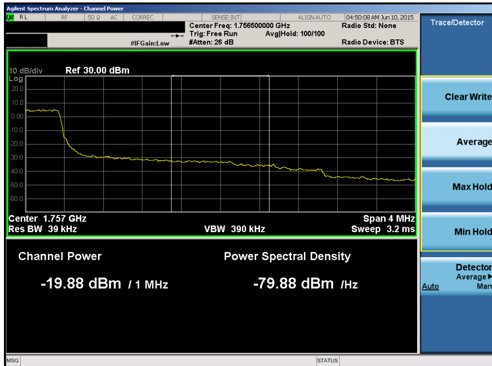
Plot 6-132. Upper Extended Band Edge Plot (Band 4 – 3.0MHz QPSK – RB Size 15)
