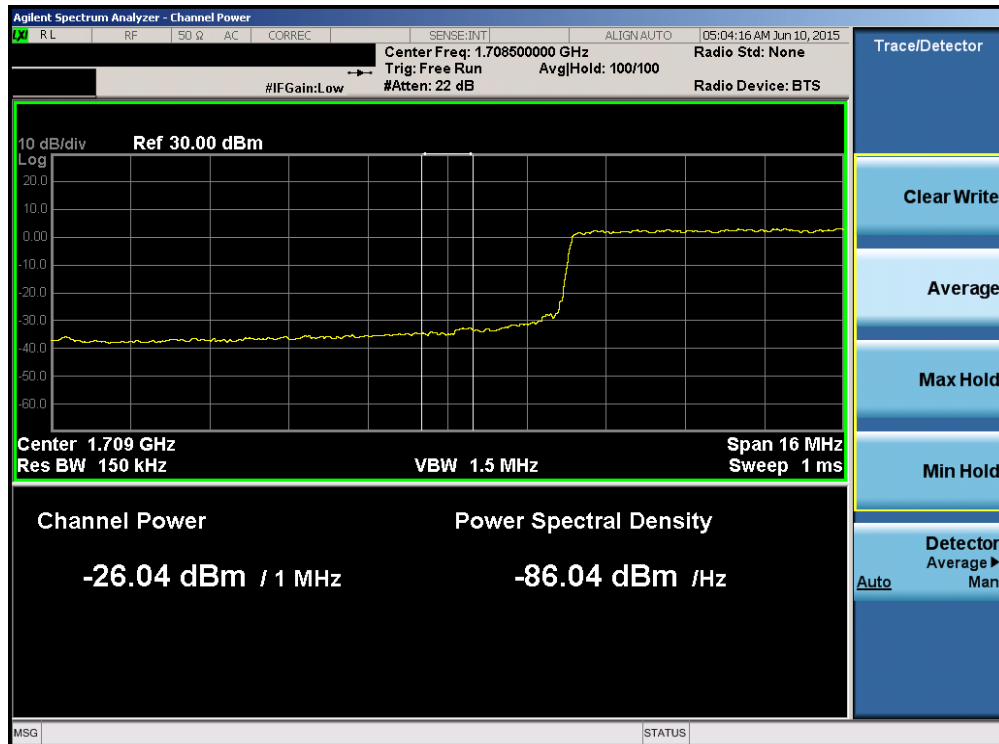
Plot 6-146. Lower Extended Band Edge Plot (Band 4 – 20.0MHz QPSK – RB Size 100)
