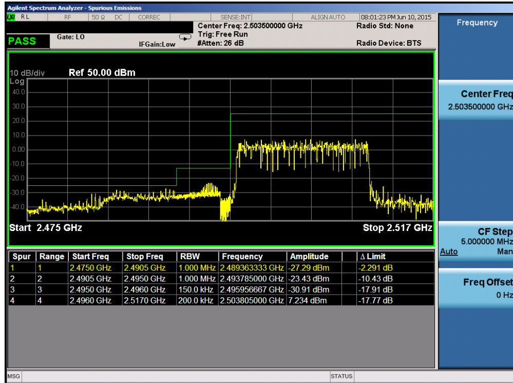
Plot 6-177. Lower Band Edge Plot (Band 41 – 15.0MHz QPSK – RB Size 75)
