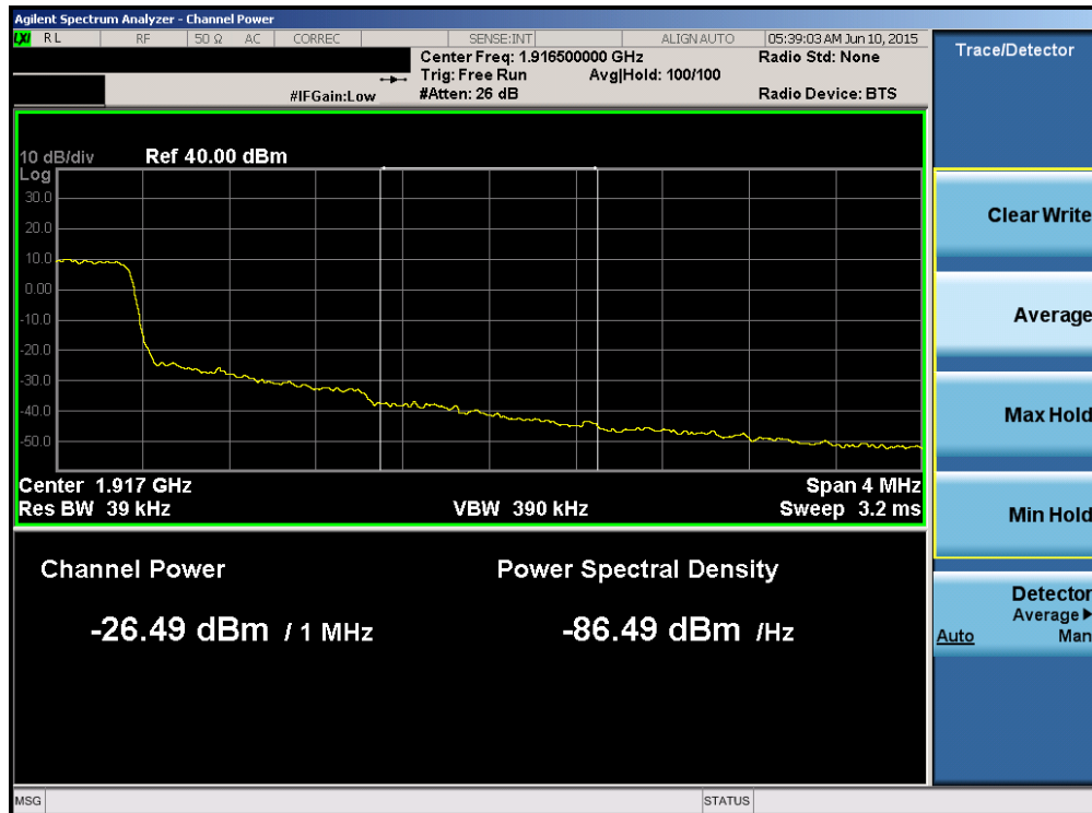
Plot 6-152. Upper Extended Band Edge Plot (Band 25 – 1.4MHz QPSK – RB Size 6)
