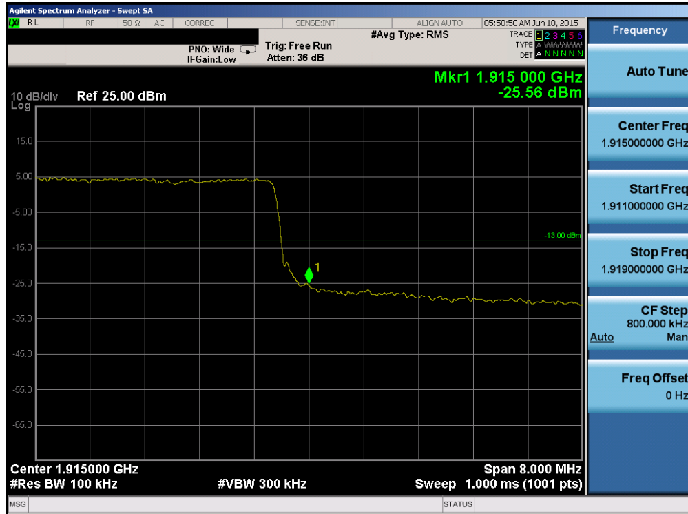
Plot 6-163. Upper Band Edge Plot (Band 25 – 10.0MHz QPSK – RB Size 50)
