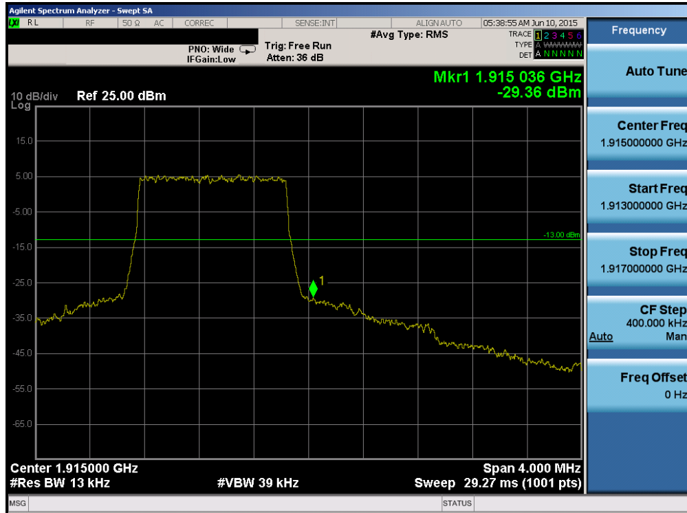
Plot 6-151. Upper Band Edge Plot (Band 25 – 1.4MHz QPSK – RB Size 6)
