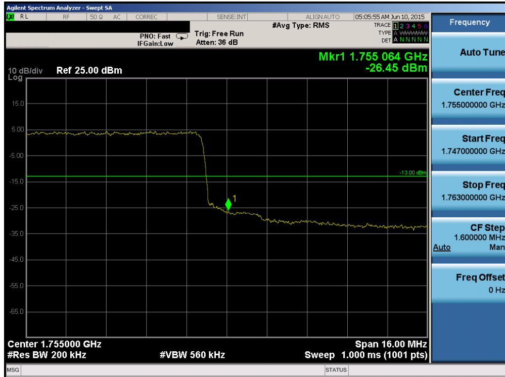
Plot 6-147. Upper Band Edge Plot (Band 4 – 20.0MHz QPSK – RB Size 100)
