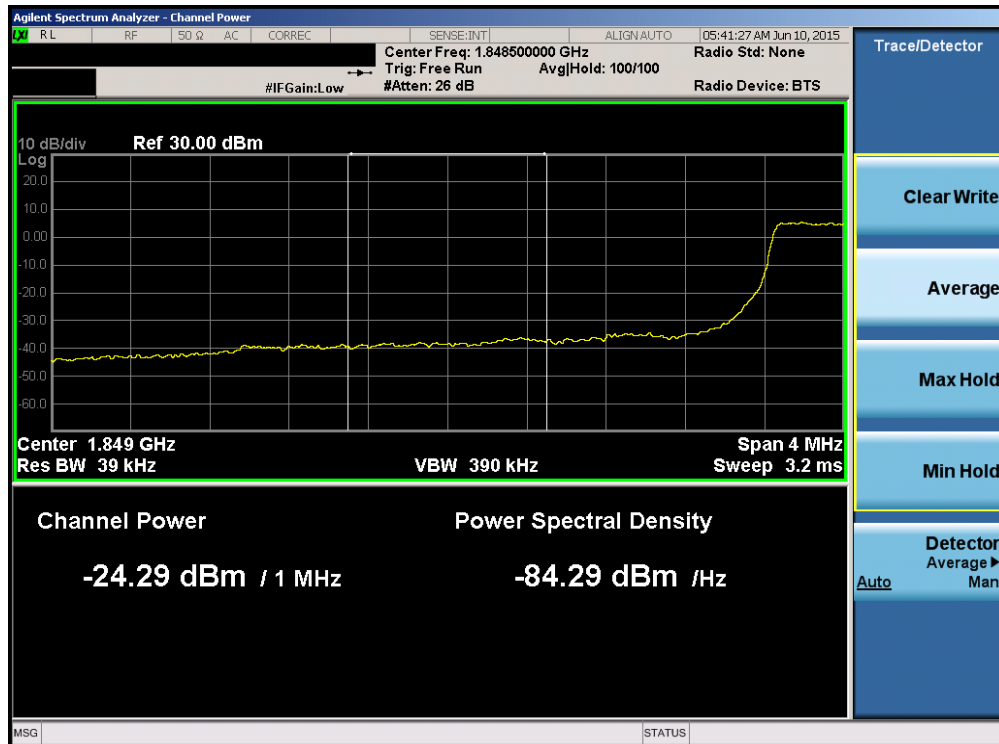
Plot 6-154. Lower Extended Band Edge Plot (Band 25 – 3.0MHz QPSK – RB Size 15)
