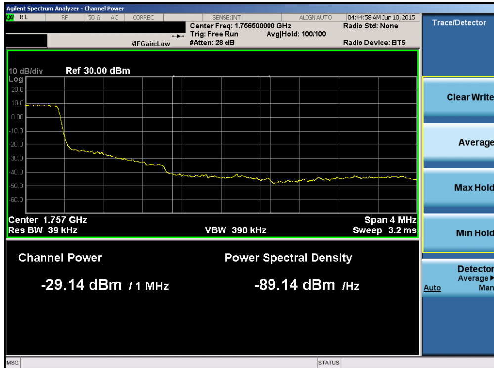
Plot 6-128. Upper Extended Band Edge Plot (Band 4 – 1.4MHz QPSK – RB Size 6)
