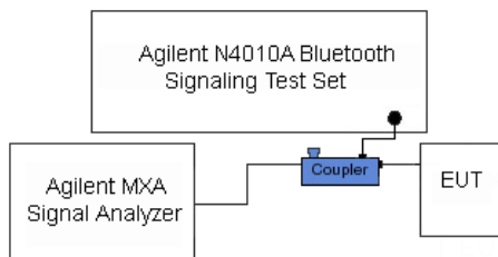
Figure 6-7. Test Instrument & Measurement Setup
