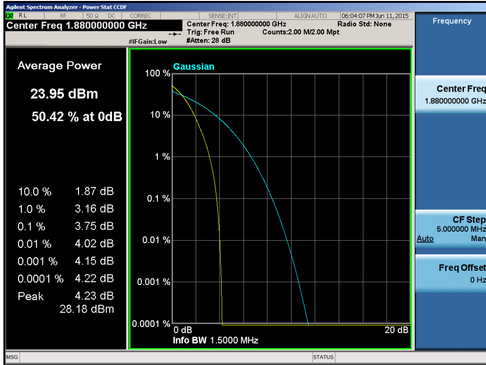
Plot 6-83. Peak-Average Ratio Plot (PCS CDMA Mode – Ch. 600)
