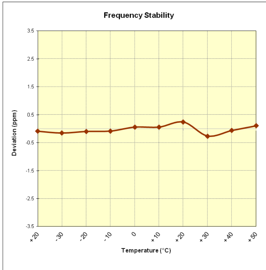
Figure 6-11. Frequency Stability Graph (PCS CDMA Mode – Ch. 600)
