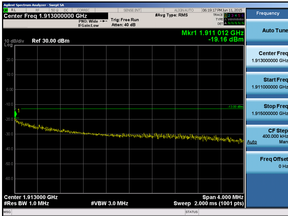
Plot 6-74. 4MHz Span Plot (PCS CDMA Mode – Ch. 1175)
