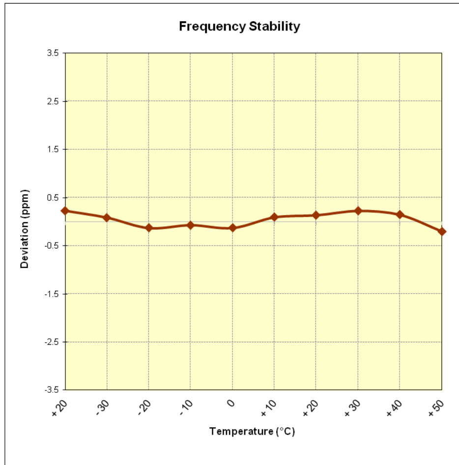
Figure 6-12. Frequency Stability Graph (PCS WCDMA Mode – Ch. 9400)
