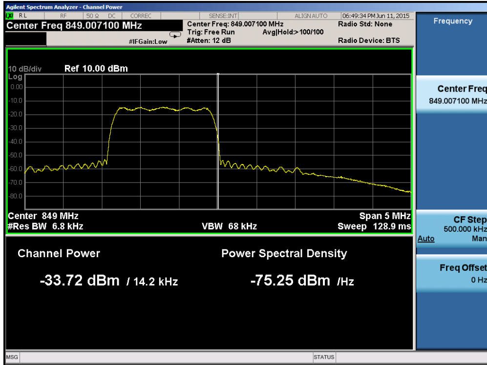
Plot 6-69. Band Edge Plot (Cellular CDMA Mode – Ch. 777)
