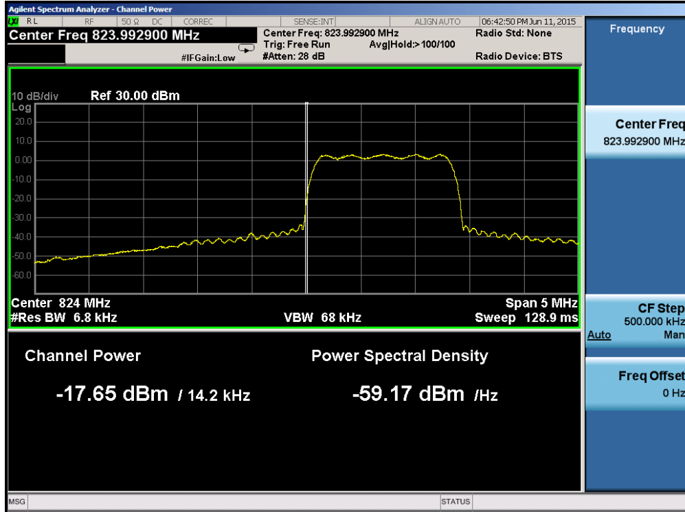
Plot 6-67. Band Edge Plot (Cellular CDMA Mode – Ch. 1013)
