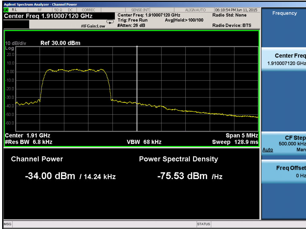
Plot 6-73. Band Edge Plot (PCS CDMA Mode – Ch. 1175)
