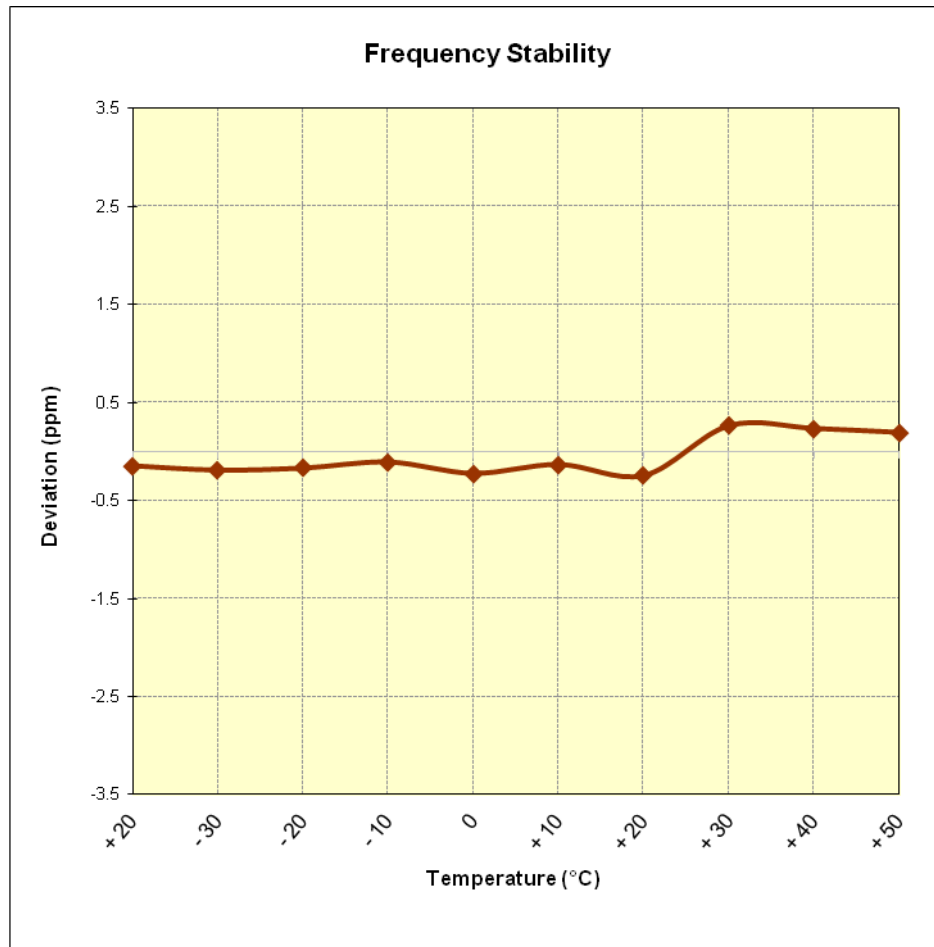
Figure 6-10. Frequency Stability Graph (PCS GSM Mode – Ch. 661)
