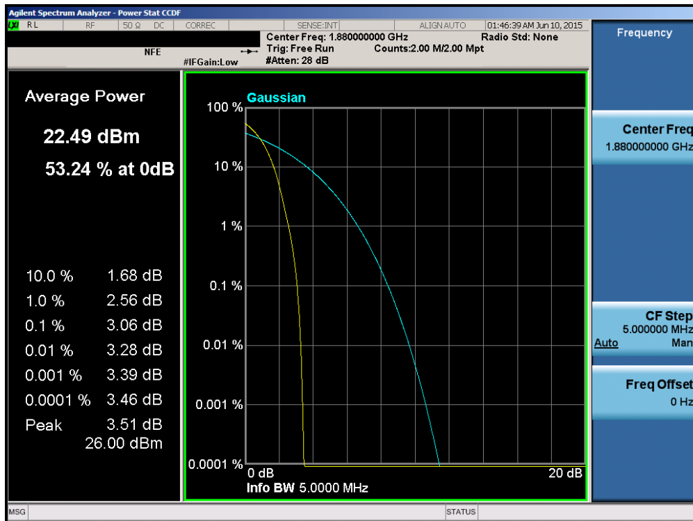
Plot 6-84. Peak-Average Ratio Plot (PCS WCDMA Mode – Ch. 9400)
