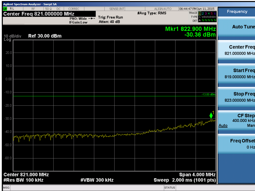
Plot 6-68. 4MHz Span Plot (Cellular CDMA Mode – Ch. 1013)
