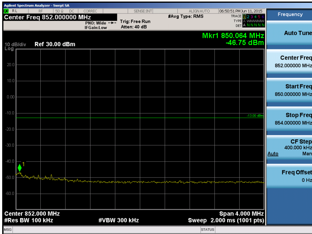
Plot 6-70. 4MHz Span Plot (Cellular CDMA Mode – Ch. 777)
