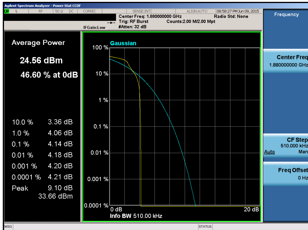
Plot 6-82. Peak-Average Ratio Plot (EDGE1900 Mode – Ch. 661)
