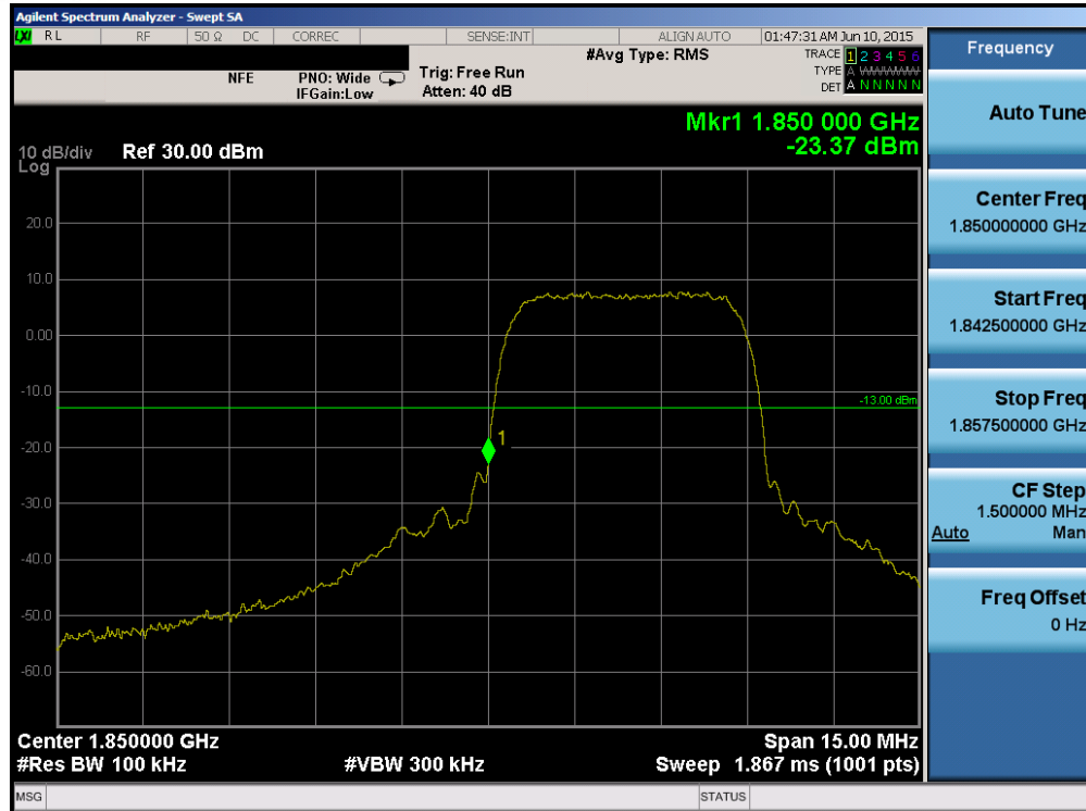
Plot 6-77. Band Edge Plot (PCS WCDMA Mode – Ch. 9262)
