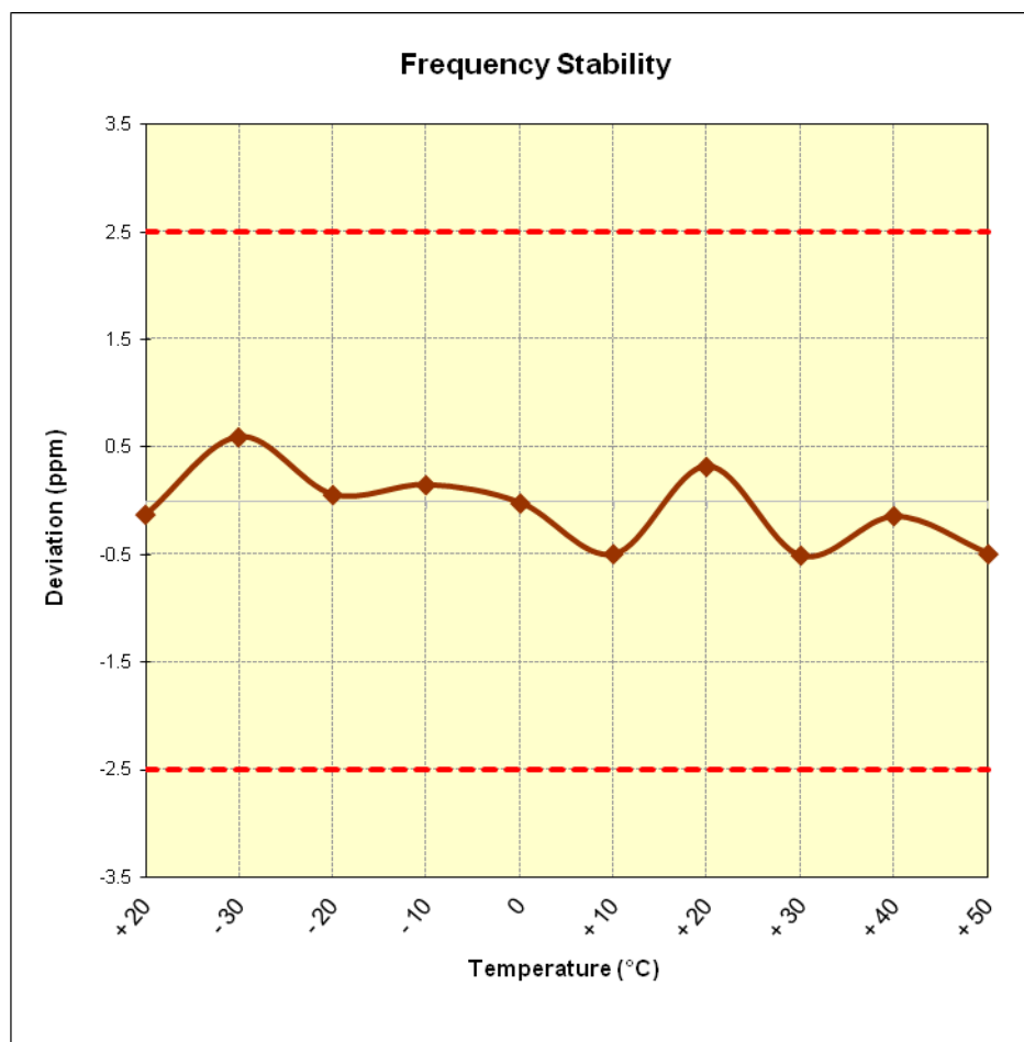
Figure 6-8. Frequency Stability Graph (Cellular CDMA Mode – Ch. 384)
