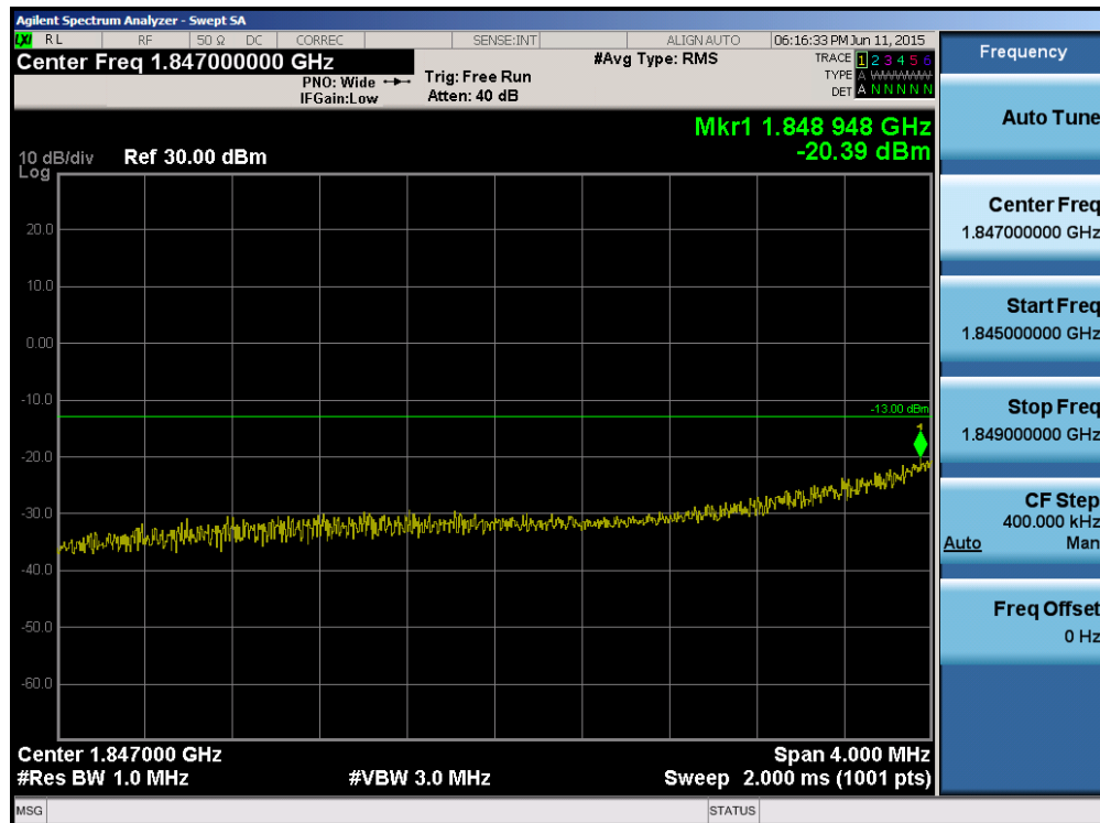
Plot 6-72. 4MHz Span Plot (PCS CDMA Mode – Ch. 25)
