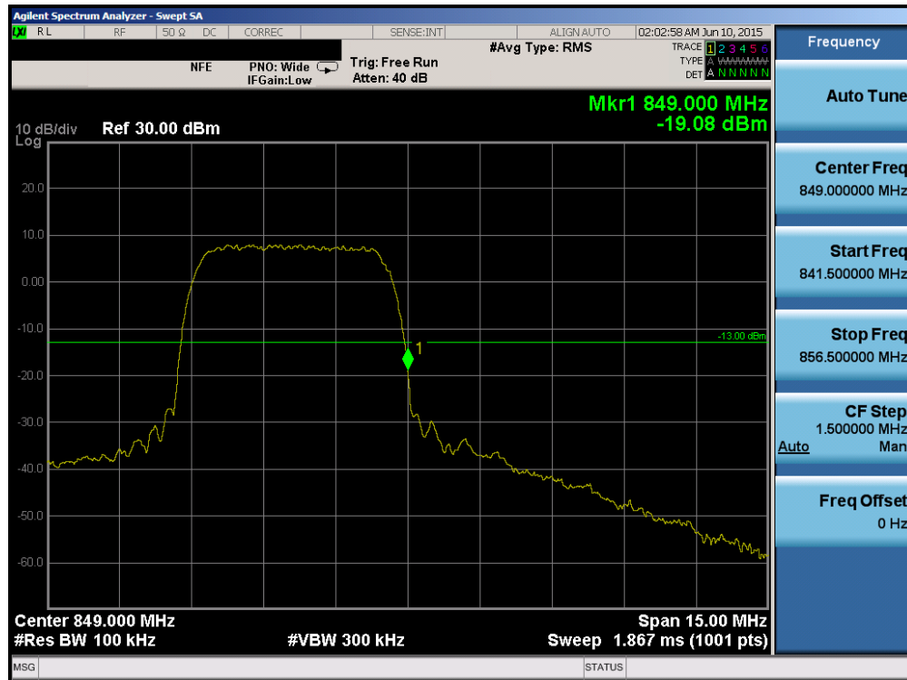
Plot 6-76. Band Edge Plot (Cellular WCDMA Mode – Ch. 4233)
