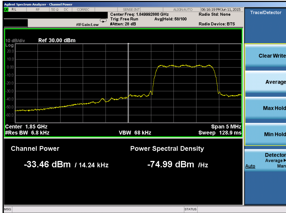
Plot 6-71. Band Edge Plot (PCS CDMA Mode – Ch. 25)
