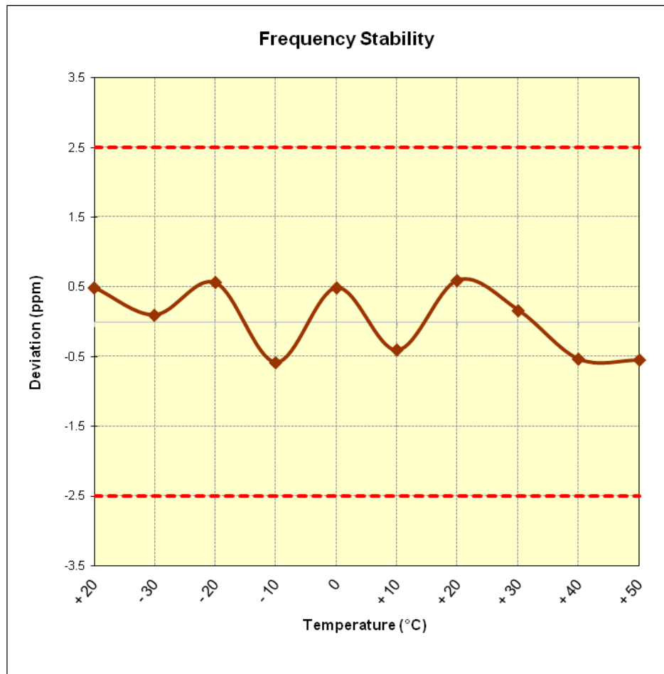
Figure 6-9. Frequency Stability Graph (Cellular WCDMA Mode – Ch. 4183)
