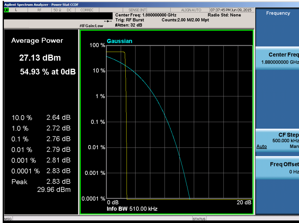
Plot 6-81. Peak-Average Ratio Plot (PCS GSM Mode – Ch. 661)
