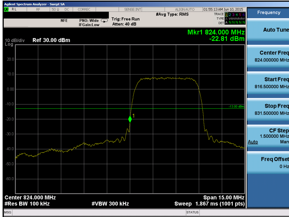
Plot 6-75. Band Edge Plot (Cellular WCDMA Mode – Ch. 4132)
