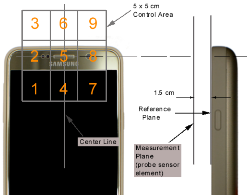
Figure 15-3 5x5 Scan grid above WD
