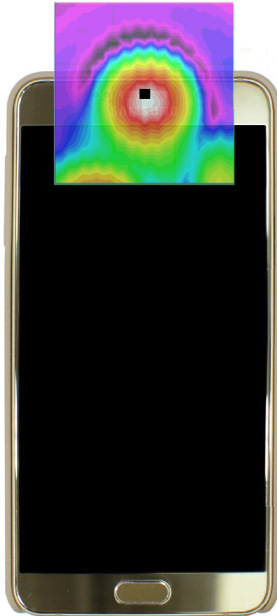
Figure 12-3 Axial T-coil Scan Overlay Magnetic Field Distributions
