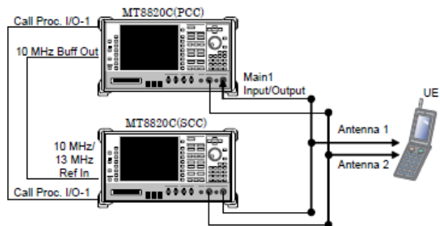
Figure 9-4 Power Measurement Setup
