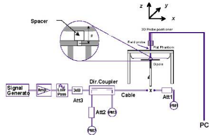
Figure 6 System Verification Setup Diagram
