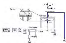
Figure 9 System Verification Setup Diagram
