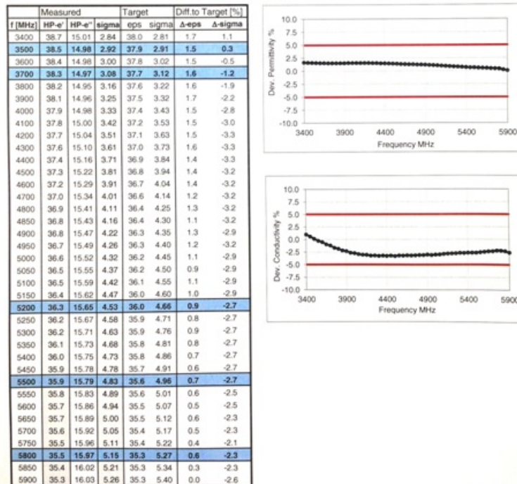
Figure D-7 5GHz Head Tissue Equivalent Matter
