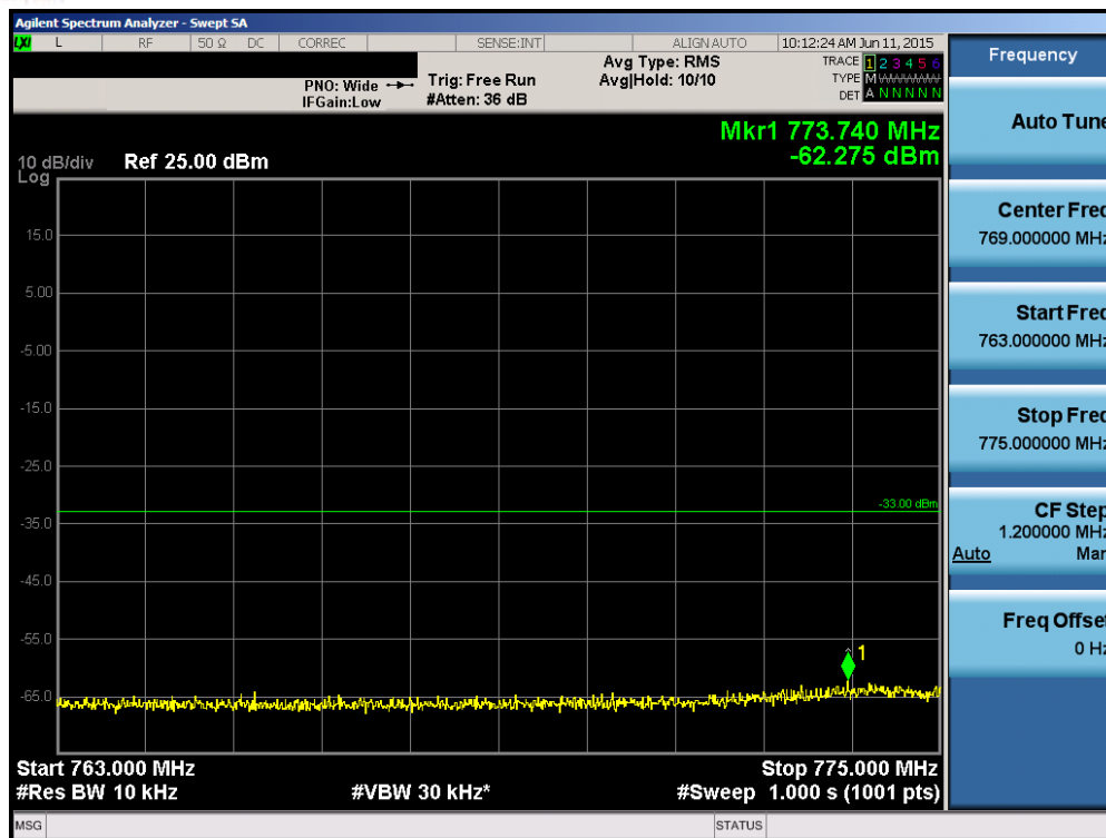
Plot 6-109. Lower Emission Mask Edge Plot (Band 13 – 10.0MHz QPSK – RB Size 50)
