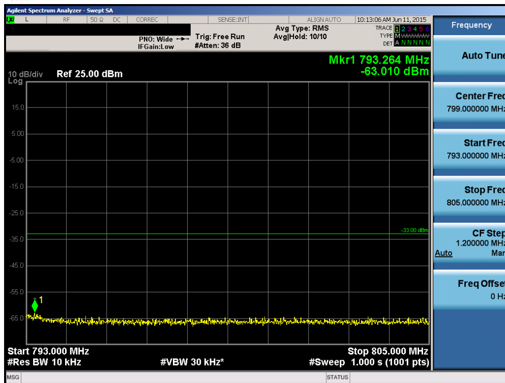
Plot 6-111. Upper Emission Mask Edge Plot (Band 13 – 10.0MHz QPSK – RB Size 50)
