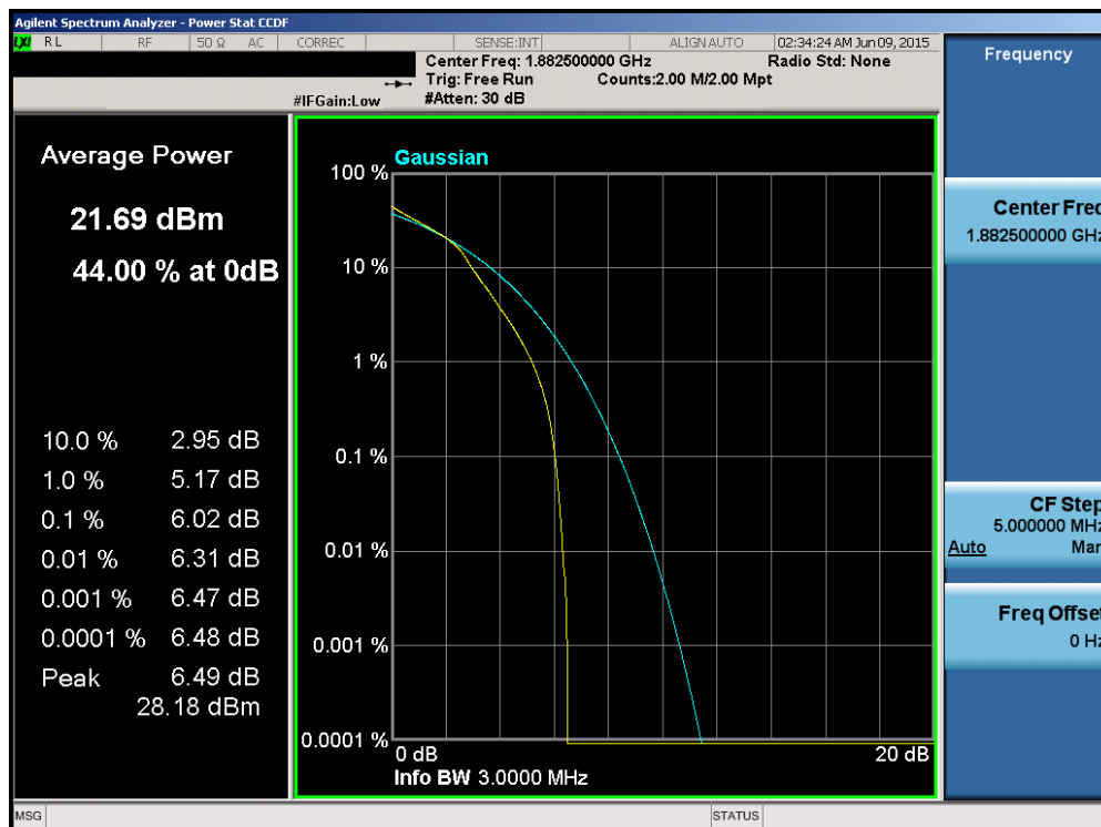
Plot 6-177. PAR Plot (Band 2/25 – 3.0MHz 16-QAM – RB Size 15)
