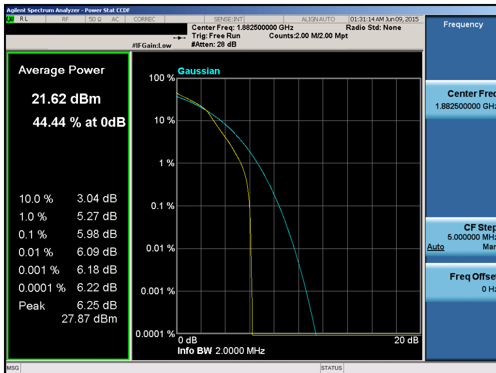
Plot 6-175. PAR Plot (Band 2/25 – 1.4MHz 16-QAM – RB Size 6)
