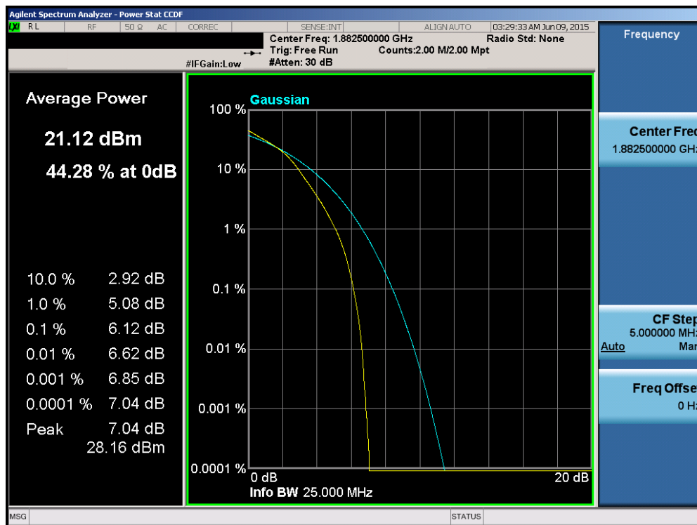
Plot 6-185. PAR Plot (Band 2/25 – 20.0MHz 16-QAM – RB Size 100)
