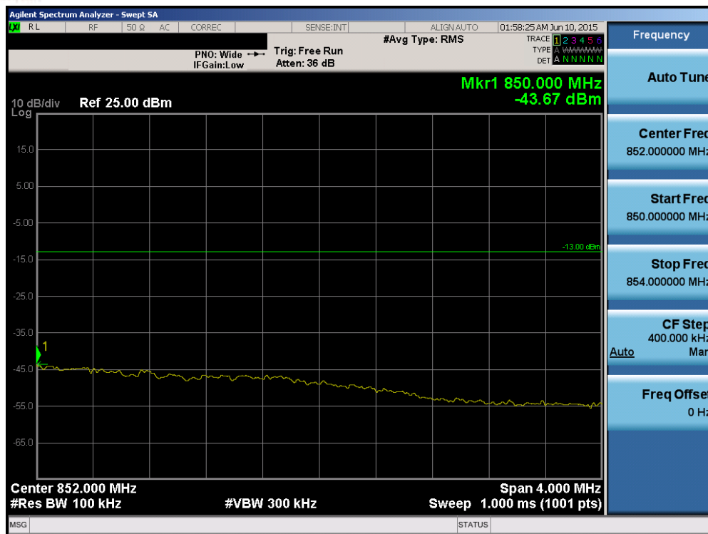
Plot 6-115. Upper Extended Band Edge Plot (Band 5 – 1.4MHz QPSK – RB Size 6)
