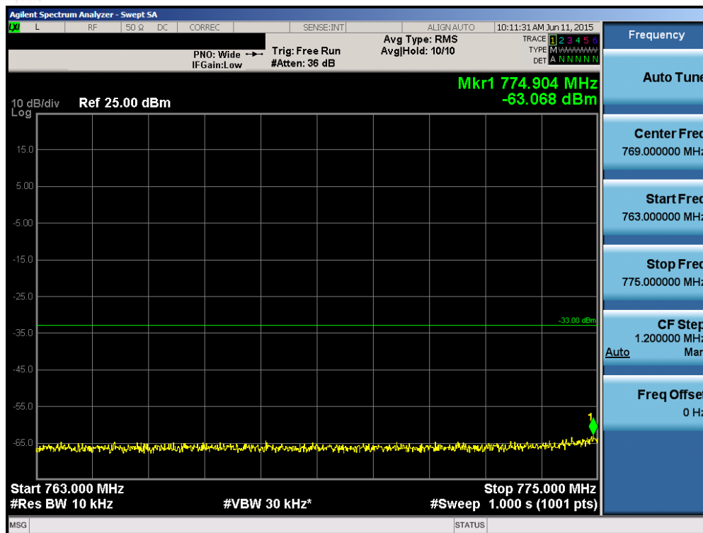
Plot 6-105. Lower Emission Mask Edge Plot (Band 13 – 5.0MHz QPSK – RB Size 25)
