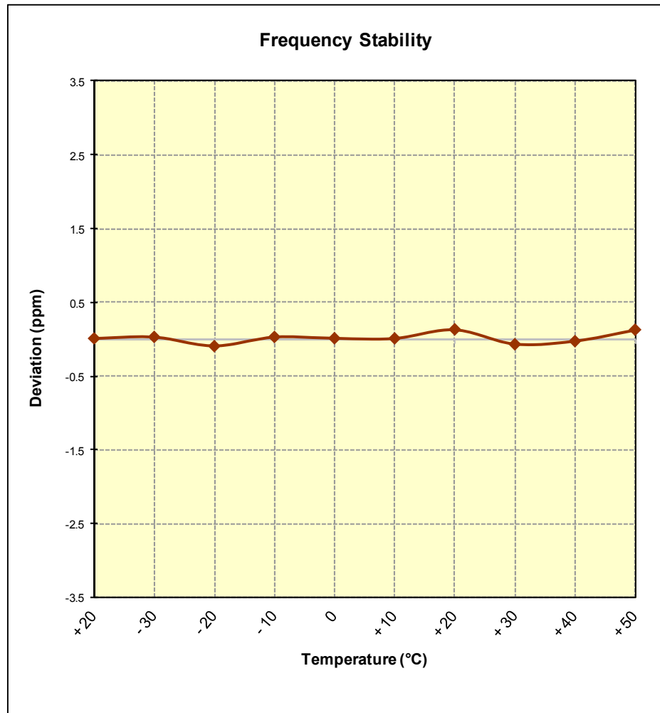
Figure 6-11. Frequency Stability Graph (Band 2/25)
