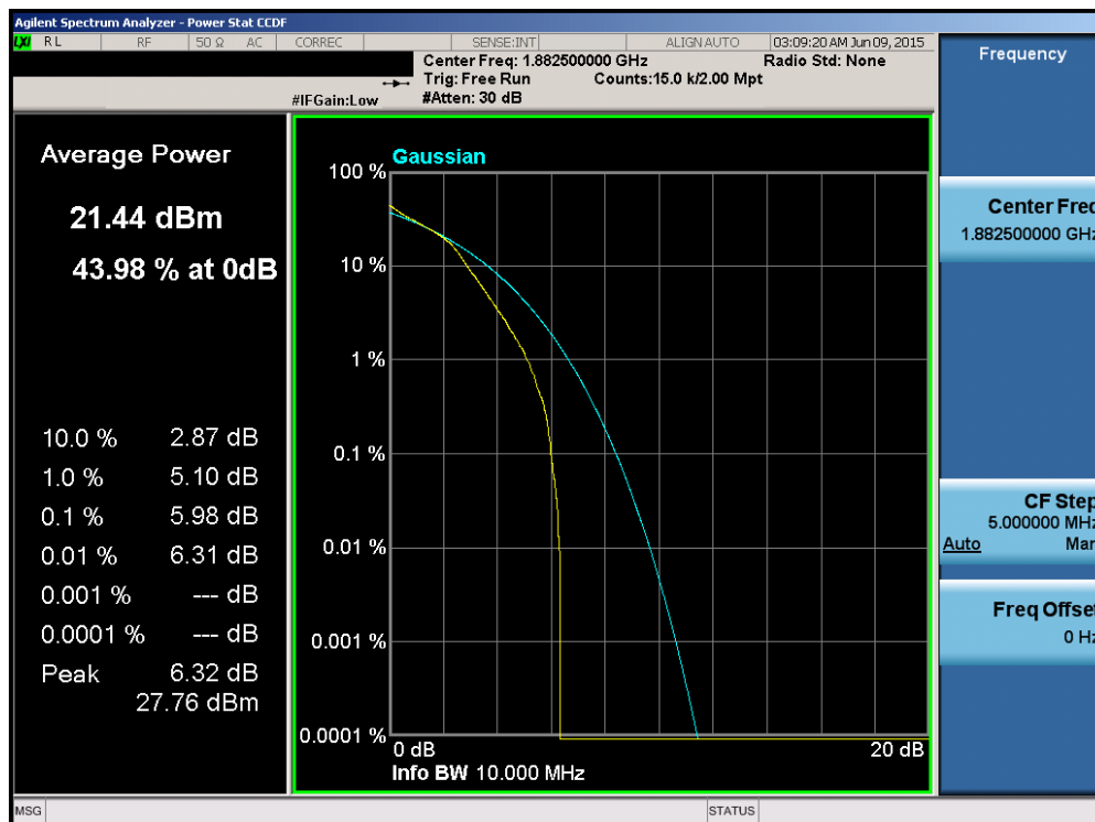
Plot 6-181. PAR Plot (Band 2/25 – 10.0MHz 16-QAM – RB Size 50)
