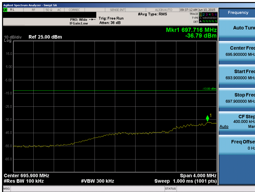
Plot 6-91. Lower Extended Band Edge Plot (Band 12 – 1.4MHz QPSK – RB Size 6)
