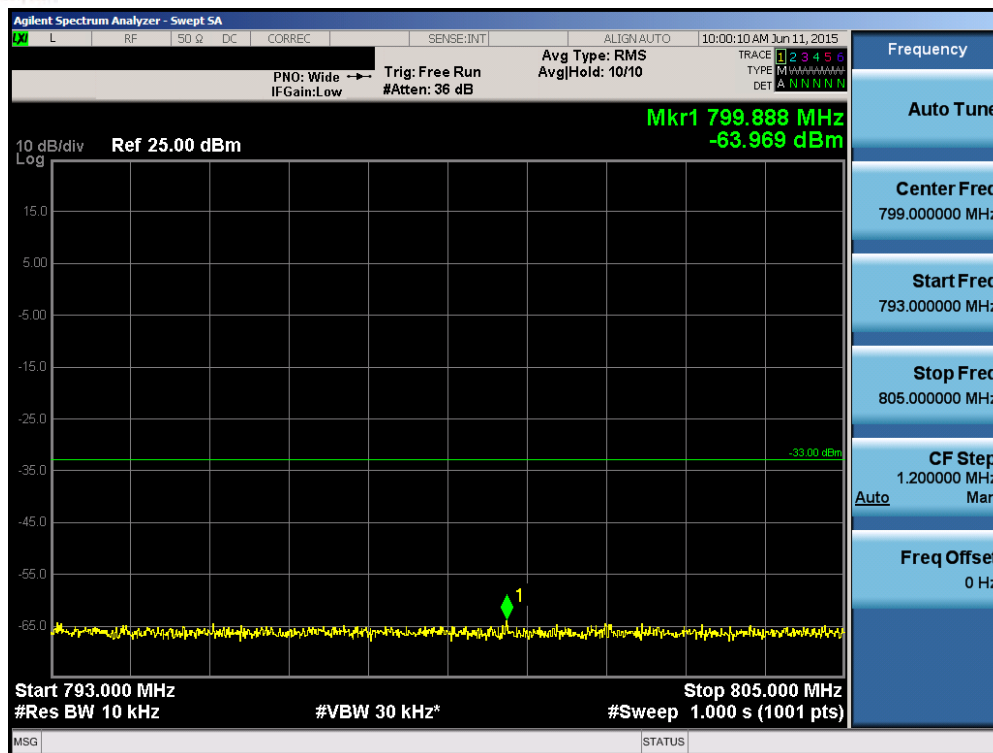
Plot 6-107. Upper Emission Mask Edge Plot (Band 13 – 5.0MHz QPSK – RB Size 25)
