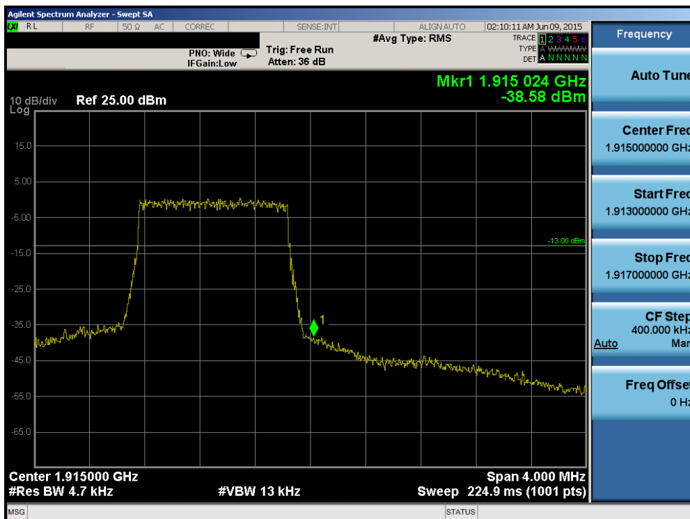
Plot 6-152. Upper Band Edge Plot (Band 2/25 – 1.4MHz QPSK – RB Size 6)
