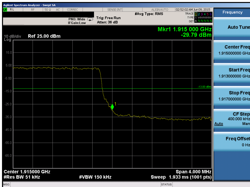
Plot 6-160. Upper Band Edge Plot (Band 2/25 – 5.0MHz QPSK – RB Size 25)
