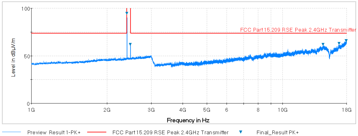
Plot 6-42. Radiated Spurious Plot above 1GHz (BT – Ch. 0, Ant. Pol. H)
