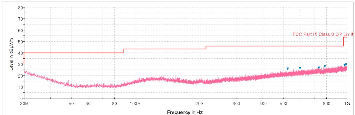
Plot 6-52. Radiated Spurious Plot below 1GHz (Pol. H)
