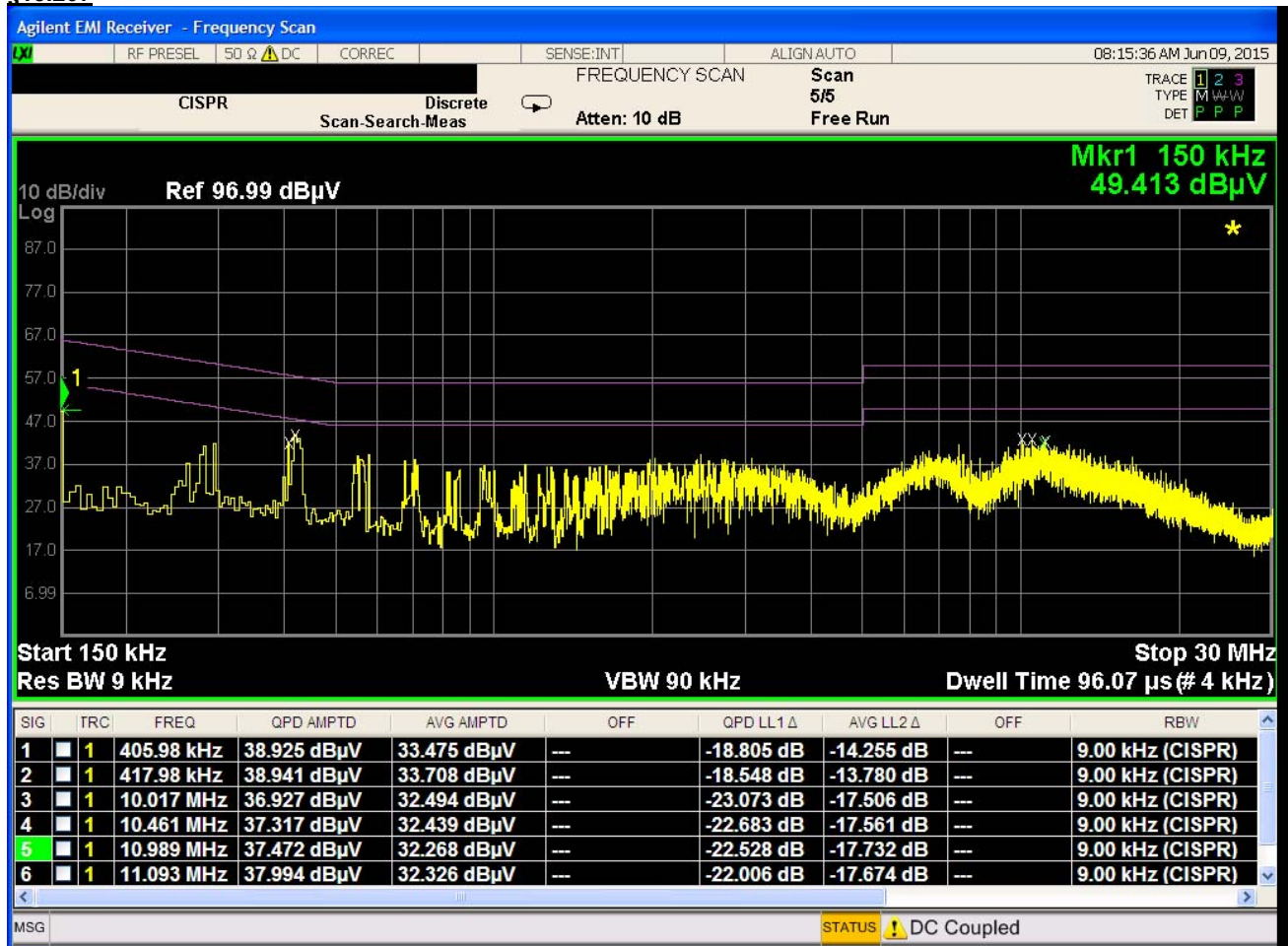
Plot 6-55. Line-Conducted Test Plot (N)
