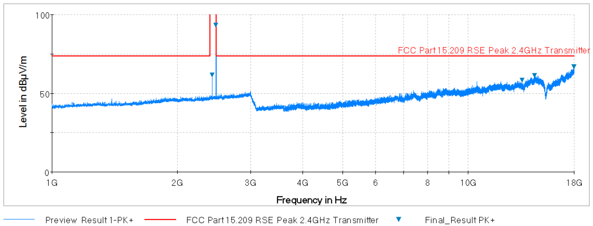
Plot 6-46. Radiated Spurious Plot above 1GHz (BT – Ch. 78, Ant. Pol. H)
