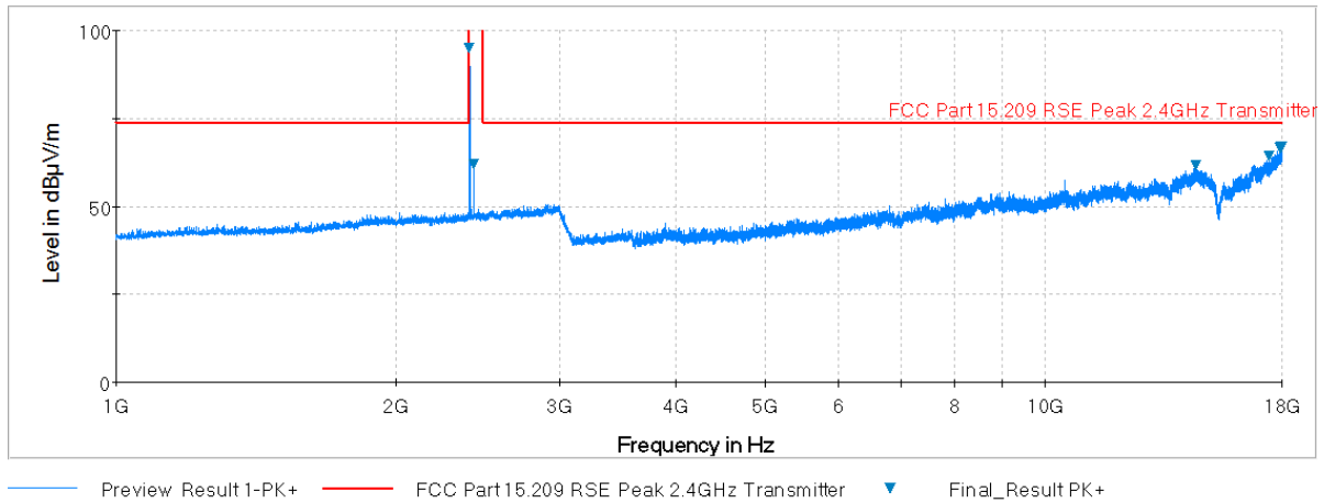
Plot 6-43. Radiated Spurious Plot above 1GHz (BT – Ch. 0, Ant. Pol. V)
