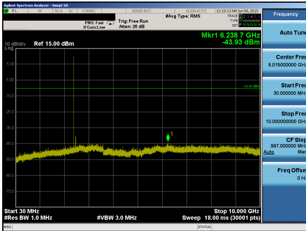
Plot 6-36. Conducted Spurious Plot (Bluetooth, 1Mbps – Ch. 0)
