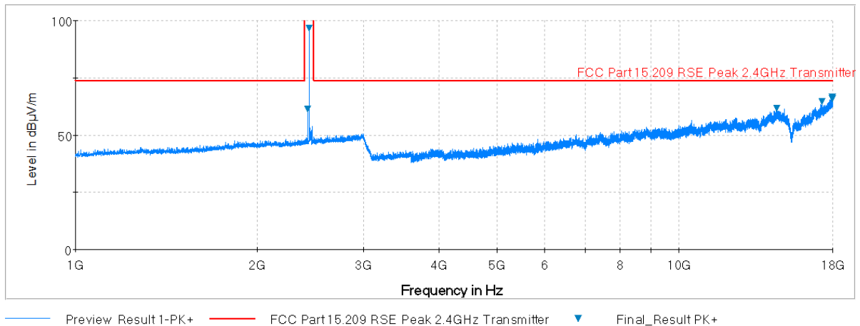
Plot 6-44. Radiated Spurious Plot above 1GHz (BT – Ch. 39, Ant. Pol. H)
