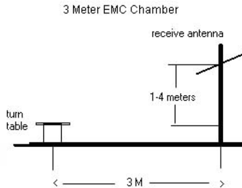
Figure 6-8. Test Instrument & Measurement Setup
