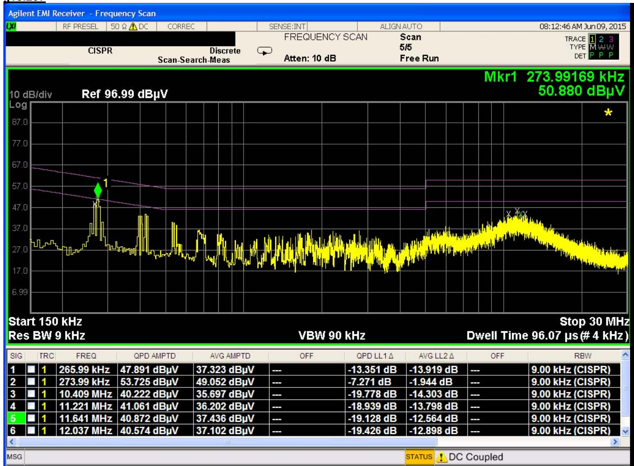
Plot 6-54. Line-Conducted Test Plot (L1)
