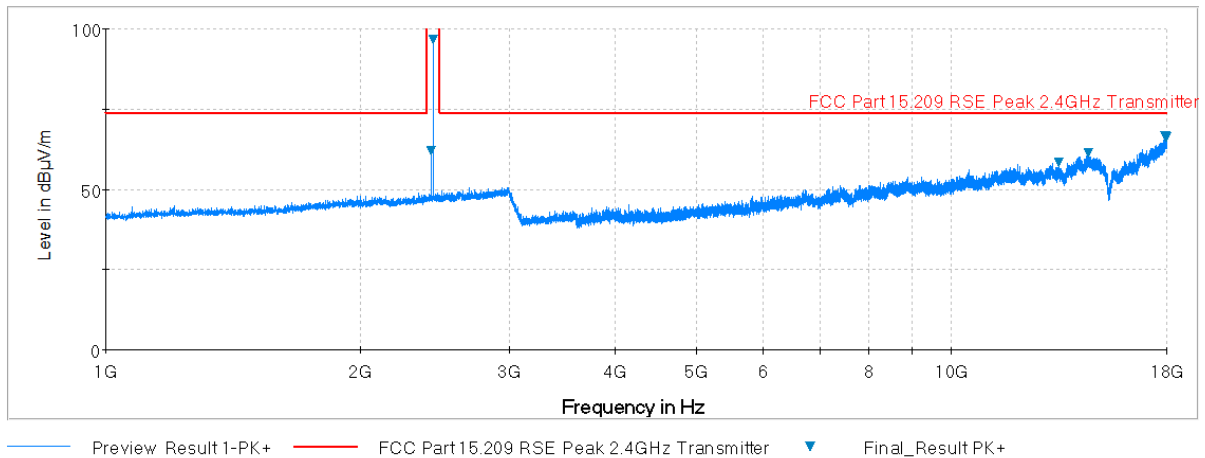
Plot 6-45. Radiated Spurious Plot above 1GHz (BT – Ch. 39, Ant. Pol. V)
