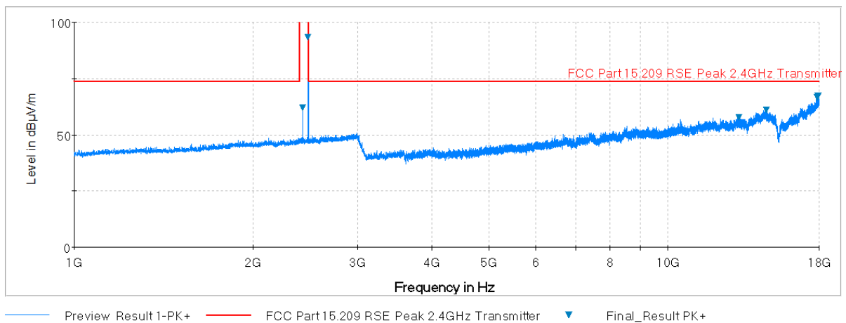
Plot 6-47. Radiated Spurious Plot above 1GHz (BT – Ch. 78, Ant. Pol. V)
