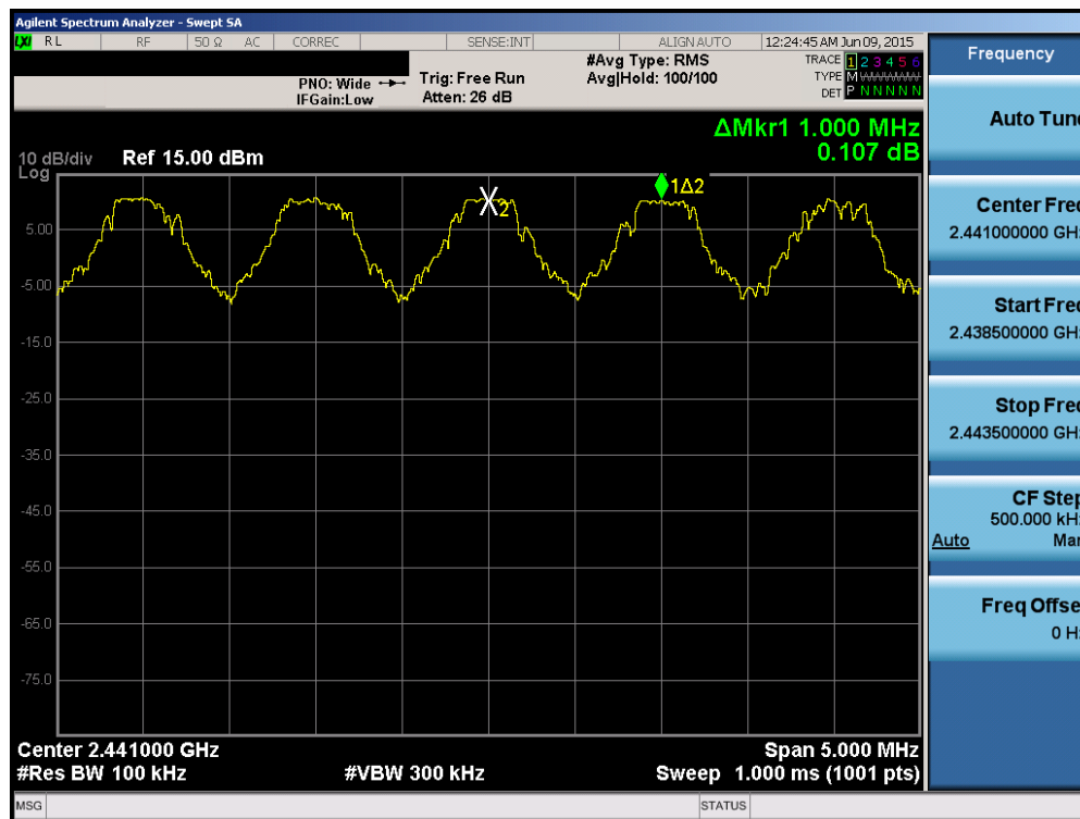
Plot 6-32. Channel Spacing Plot (Bluetooth)
