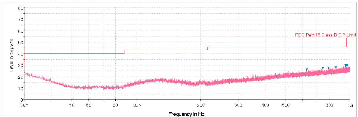
Plot 6-53. Radiated Spurious Plot below 1GHz (Pol. V)
