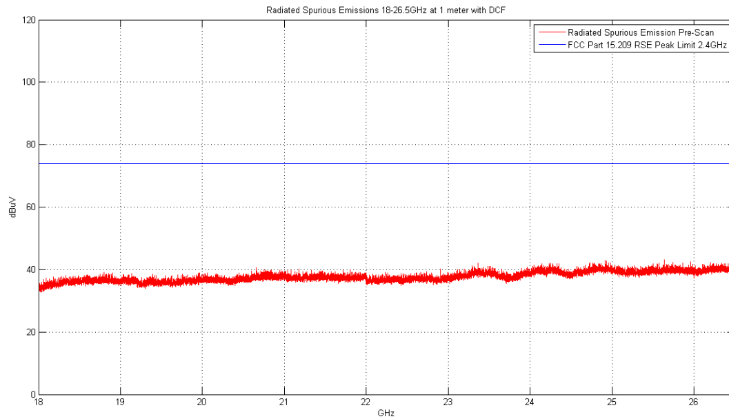
Plot 6-49. Radiated Spurious Plot above 18GHz (Pol. V)
