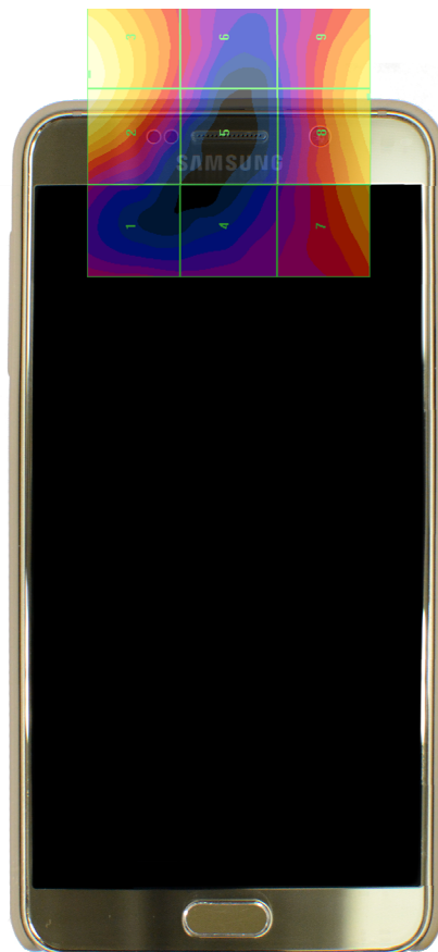
Figure 15-4 E-Field WD Scan overlay
