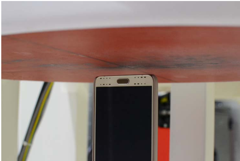
SAR Test Setup Photo 8 – Bottom Edge at 1.0 cm (Hotspot)
