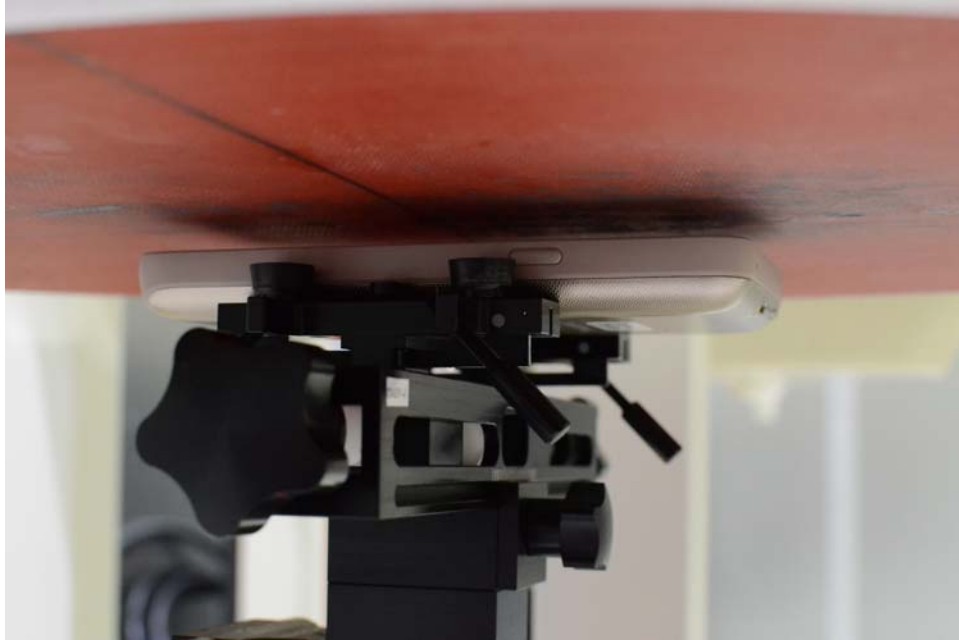
SAR Test Setup Photo 5 - Front Side at 1.0 cm (Hotspot)
