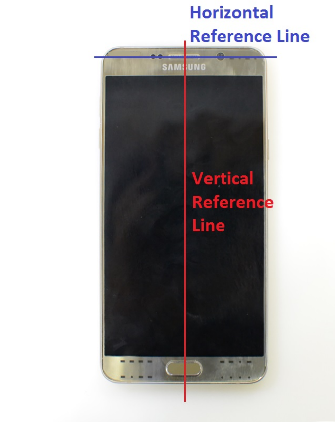
SAR Test Setup Photo 9 – DUT Reference Lines
