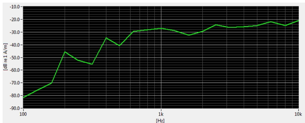
Figure 6-1 Worst-case ABM2 Plot for GSM
