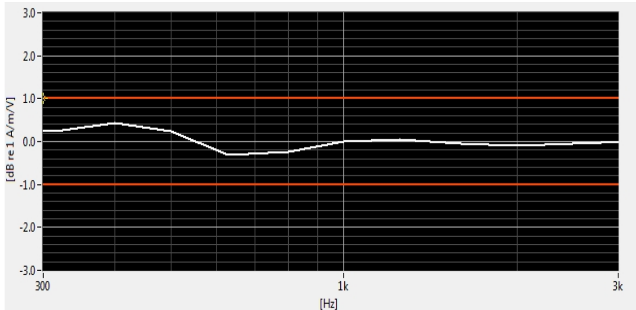
Figure 6-2 Helmholtz Coil Validation for Frequency Response
