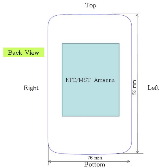
Figure F-2 NFC Antenna Location
