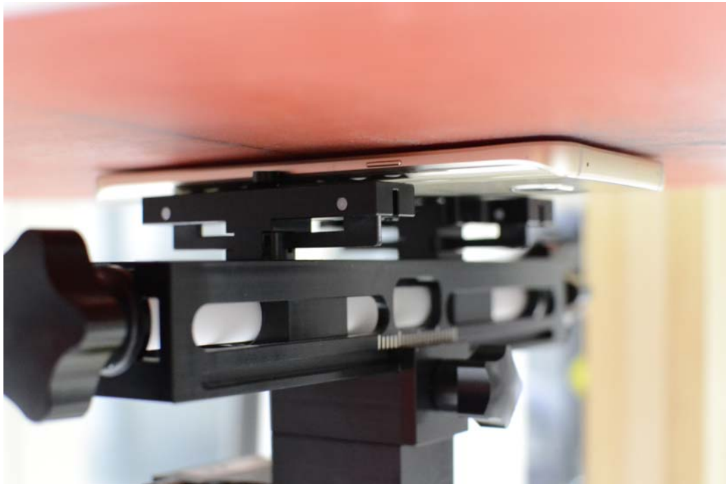
SAR Test Setup Photo 10— Front Side at 0.1 cm (Extremity)
