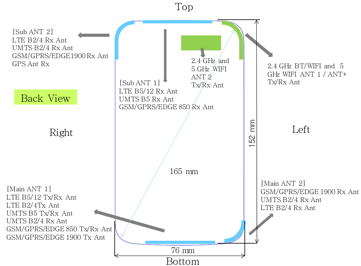
Figure F-1 DUT Antenna Locations
