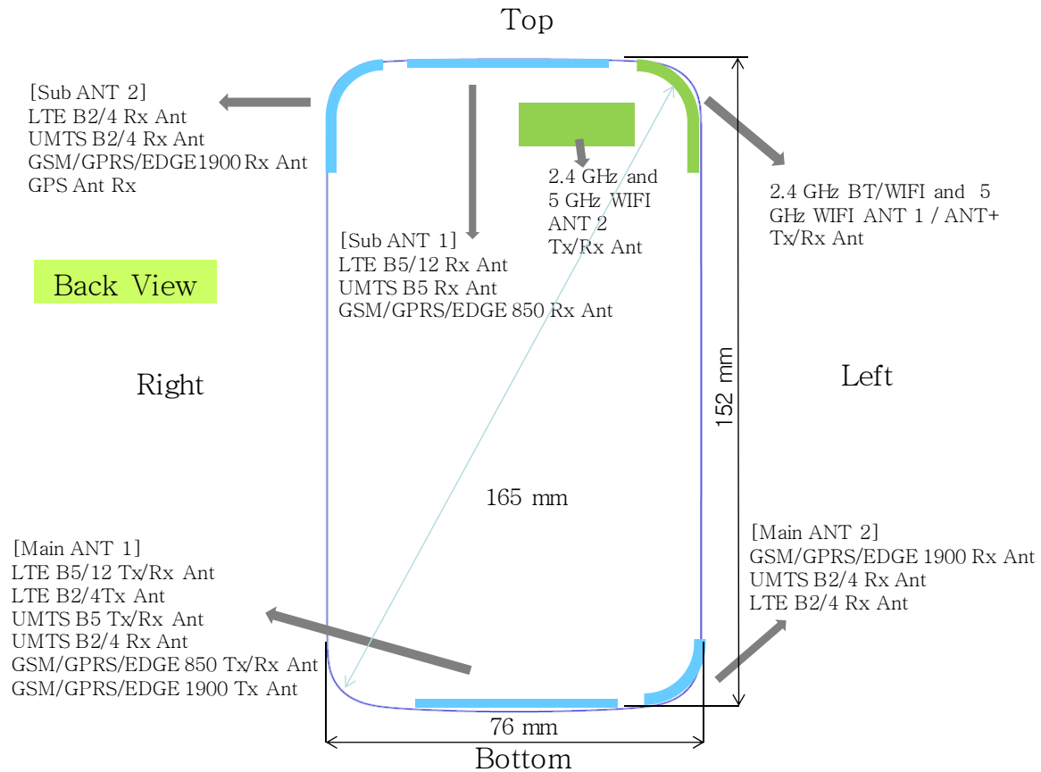
Figure F-1 DUT Antenna Locations
