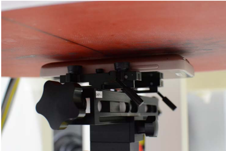
SAR Test Setup Photo 4 – Back Side at 0.4 cm (Phablet)
