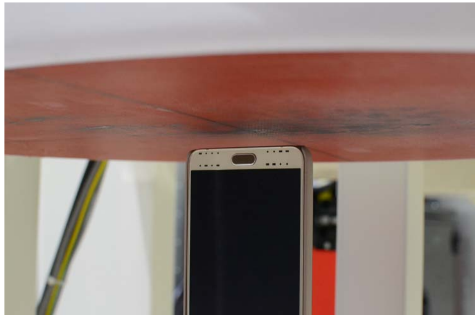
SAR Test Setup Photo 10 – Bottom Edge at 1.0 cm (Hotspot)
