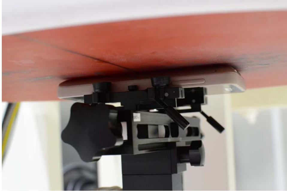
SAR Test Setup Photo 3 – Back Side at 0.0 cm (Phablet)
