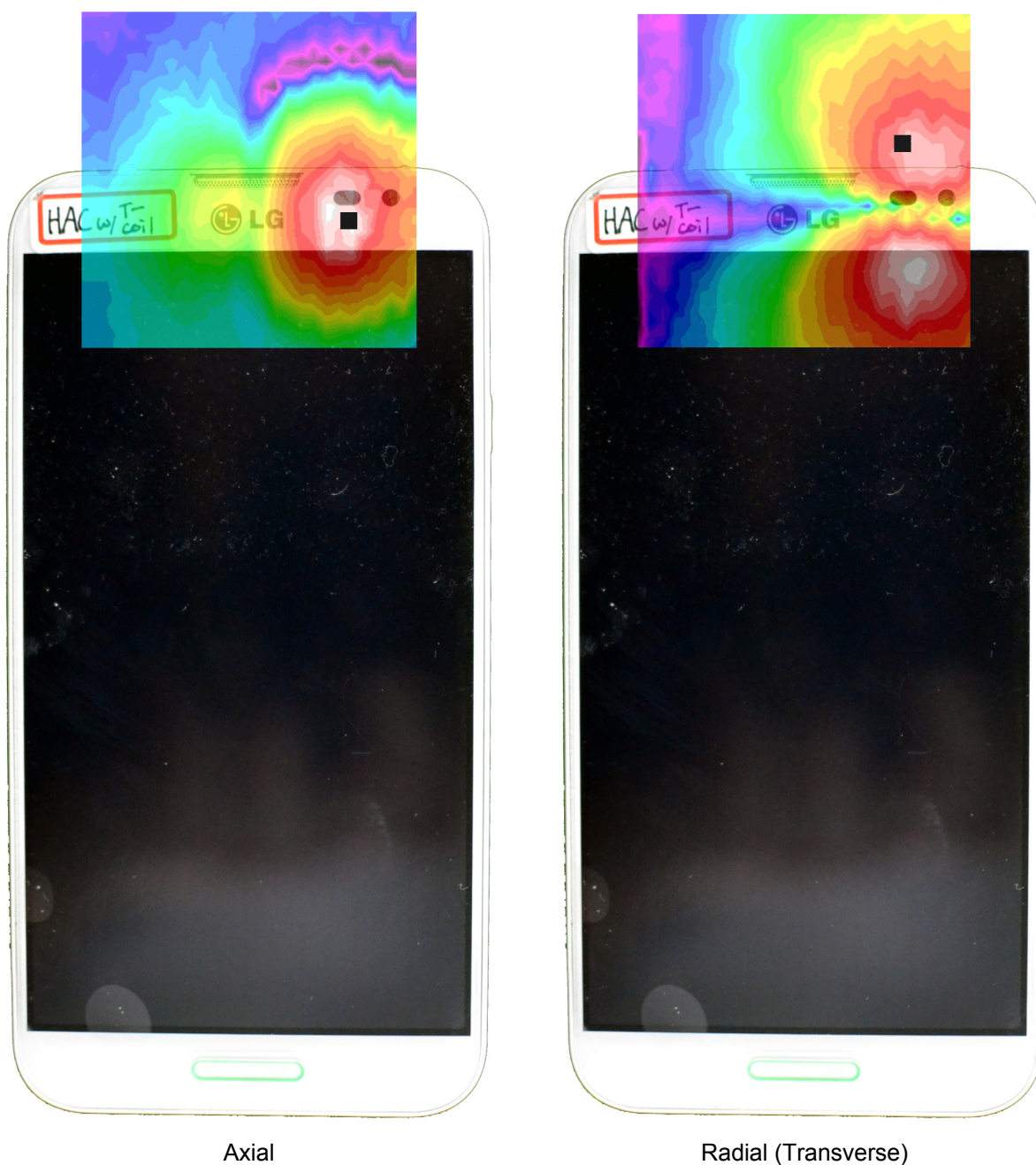
Figure 14-3 T-Coil Scan Overlay Magnetic Field Distributions
