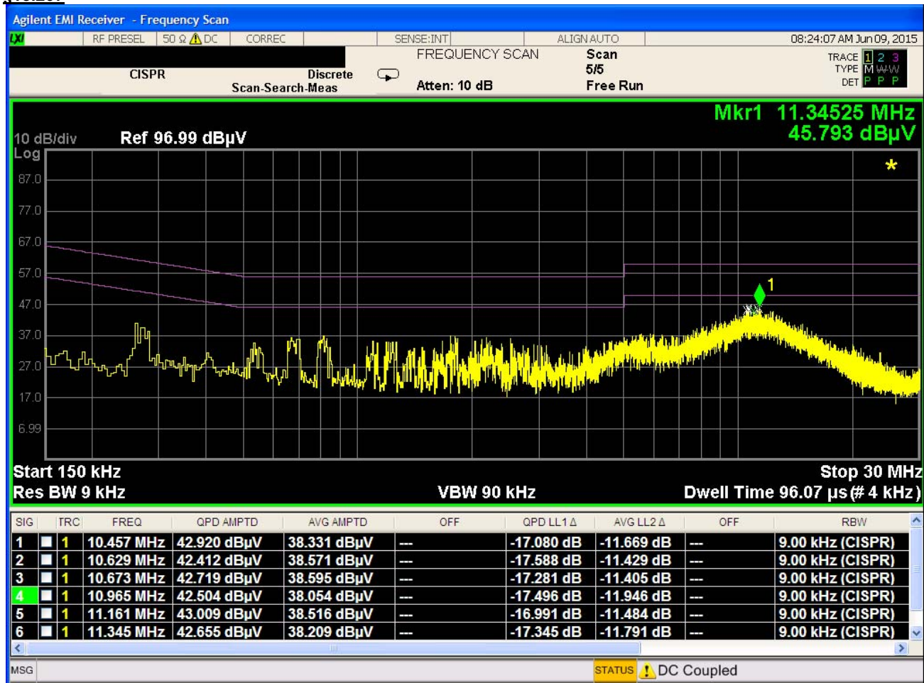
Plot 6-6. Line-Conducted Test Plot (L1)
