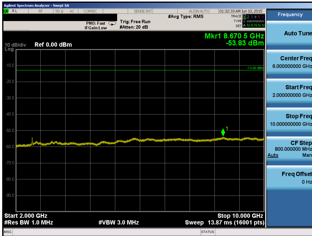
Plot 6-54. Conducted Spurious Plot (Band 5 – 10.0MHz QPSK – RB Size 1, RB Offset 0 – High Channel)
