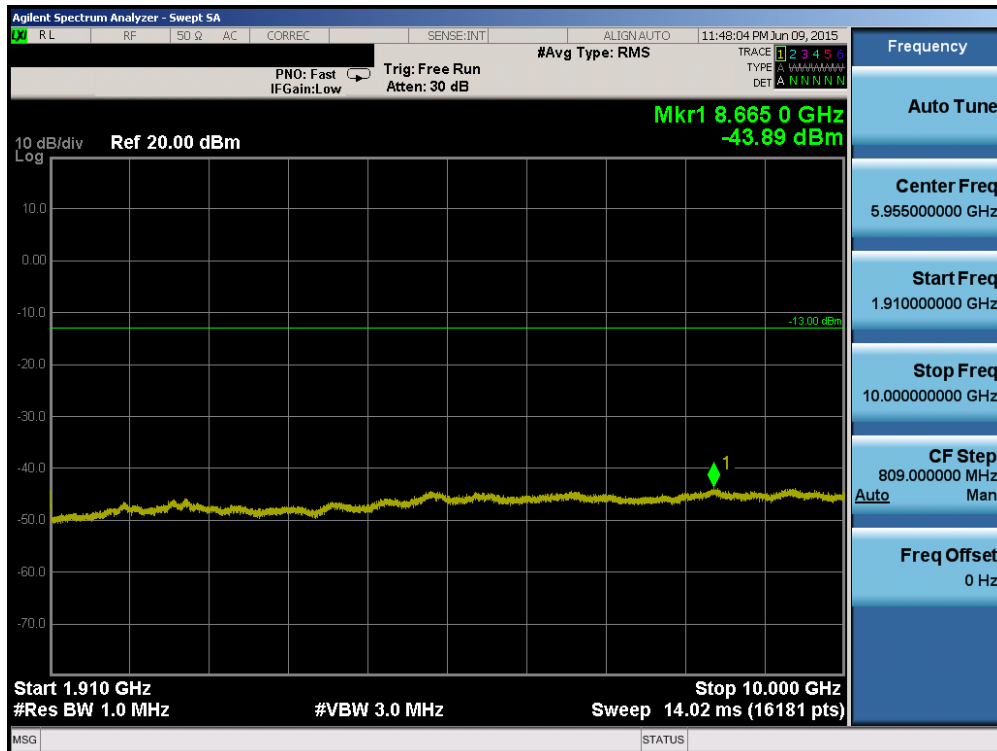
Plot 6-68. Conducted Spurious Plot (Band 2 – 10.0MHz QPSK – RB Size 1, RB Offset 0 – Mid Channel)
