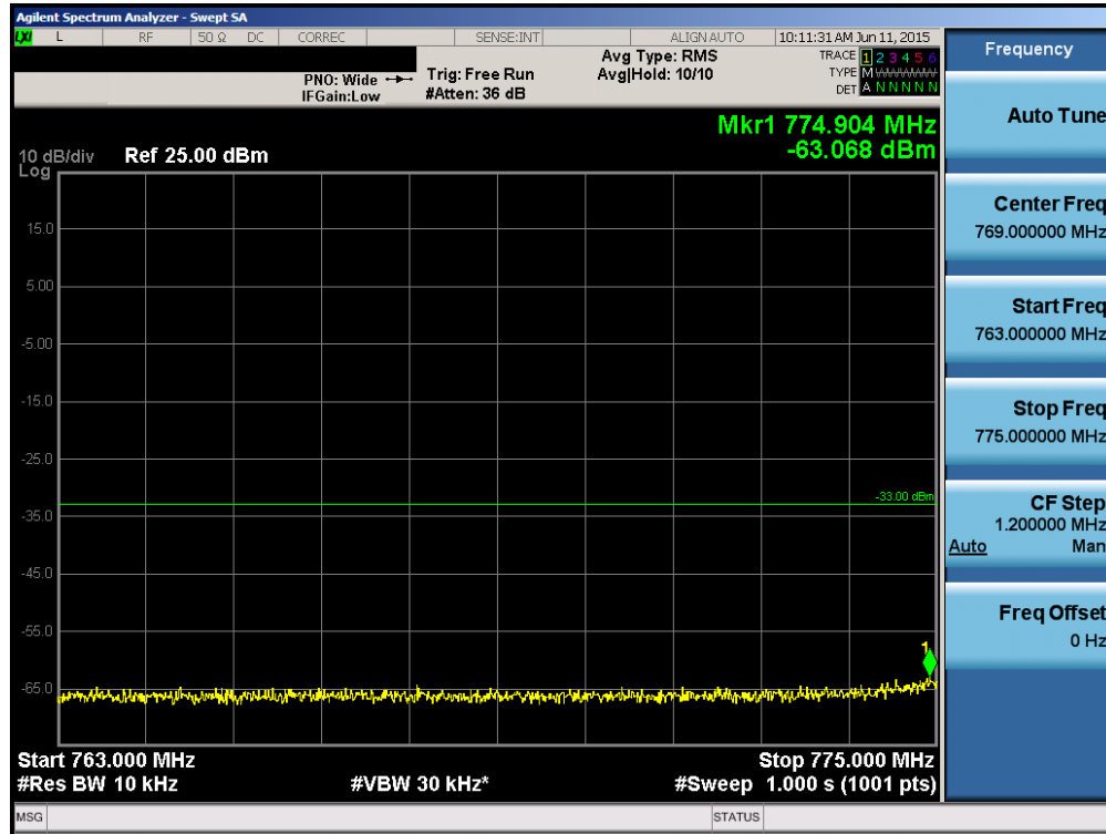
Plot 6-74. Lower Extended Band Edge Plot (Band 13 – 5.0MHz QPSK – RB Size 25)
