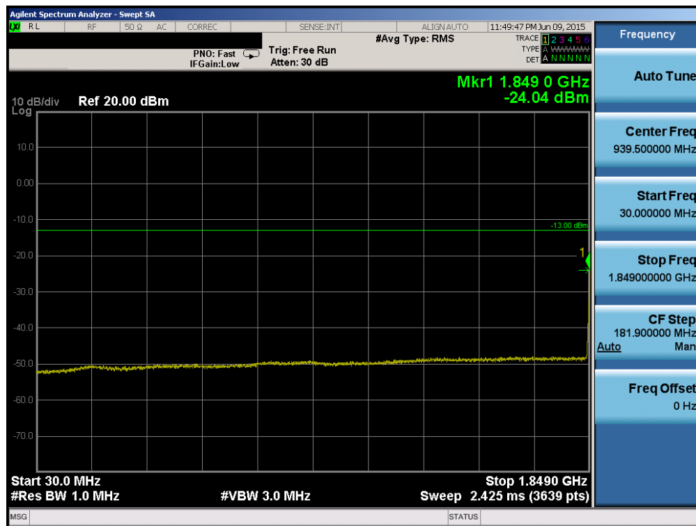
Plot 6-64. Conducted Spurious Plot (Band 2 – 10.0MHz QPSK – RB Size 1, RB Offset 0– Low Channel)
