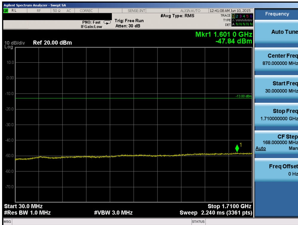
Plot 6-58. Conducted Spurious Plot (Band 4 – 1.4MHz QPSK – RB Size 1, RB Offset 0 – Mid Channel)
