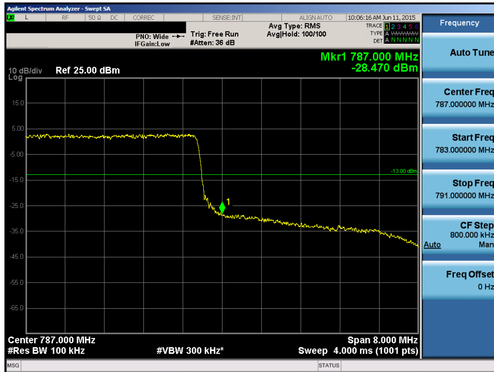
Plot 6-79. Upper Band Edge Plot (Band 13 – 10.0MHz QPSK – RB Size 50)
