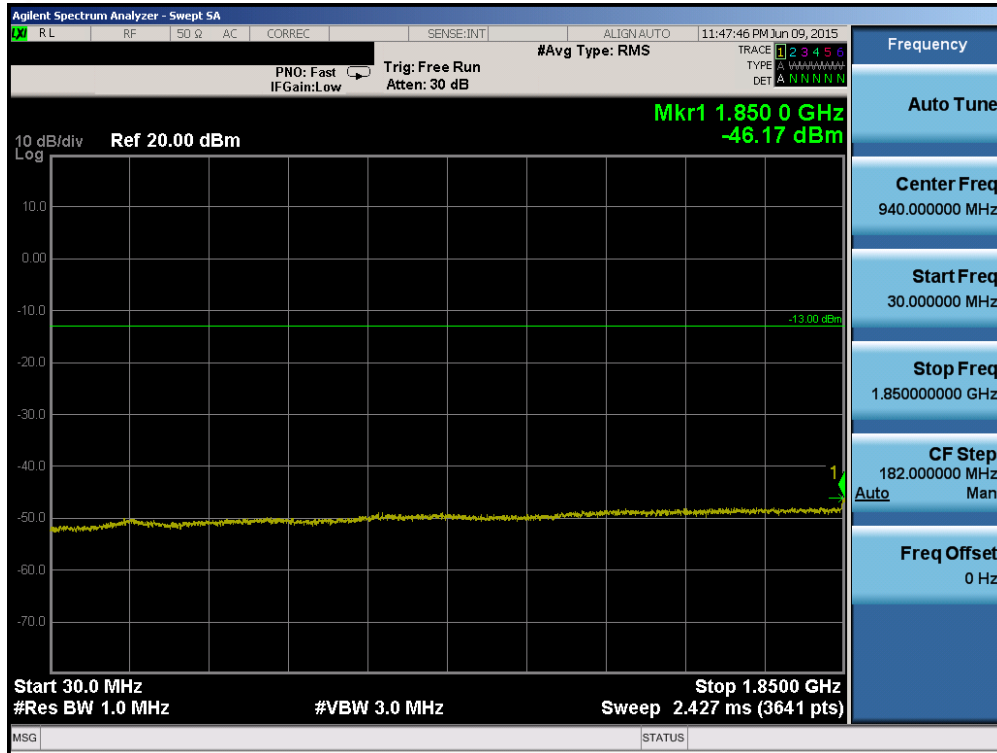
Plot 6-67. Conducted Spurious Plot (Band 2 – 10.0MHz QPSK – RB Size 1, RB Offset 0 – Mid Channel)
