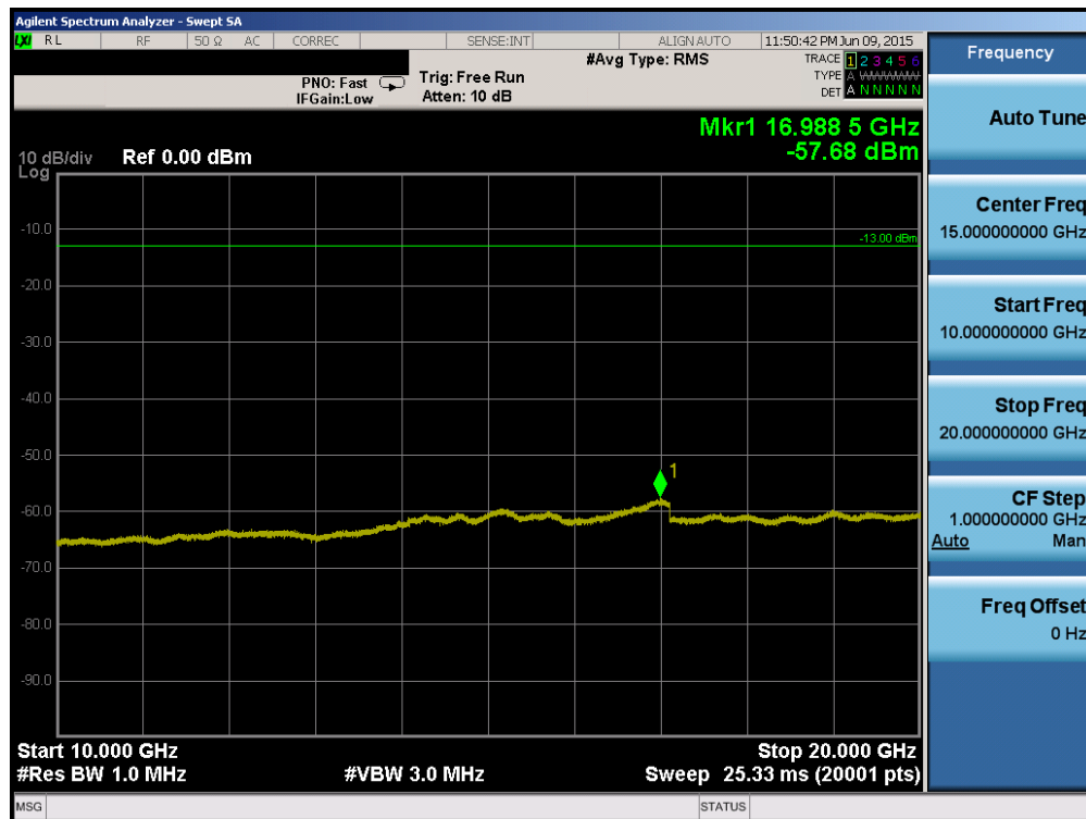
Plot 6-66. Conducted Spurious Plot (Band 2 – 10.0MHz QPSK – RB Size 1, RB Offset 0 – Low Channel)
