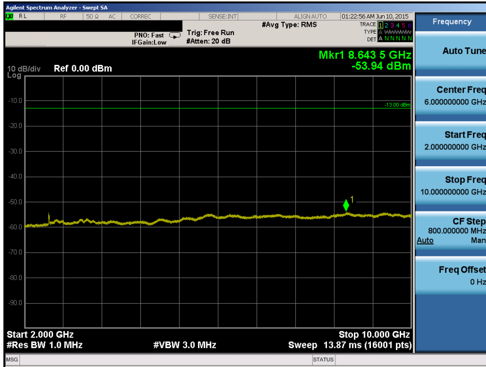
Plot 6-51. Conducted Spurious Plot (Band 5 – 10.0MHz QPSK – RB Size 1, RB Offset 0 – Mid Channel)
