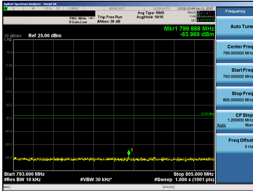
Plot 6-76. Upper Extended Band Edge Plot (Band 13 – 5.0MHz QPSK – RB Size 25)
