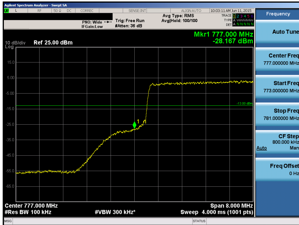
Plot 6-77. Lower Band Edge Plot (Band 13 – 10.0MHz QPSK – RB Size 50)
