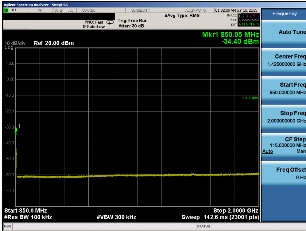
Plot 6-53. Conducted Spurious Plot (Band 5 – 10.0MHz QPSK – RB Size 1, RB Offset 0 – High Channel)
