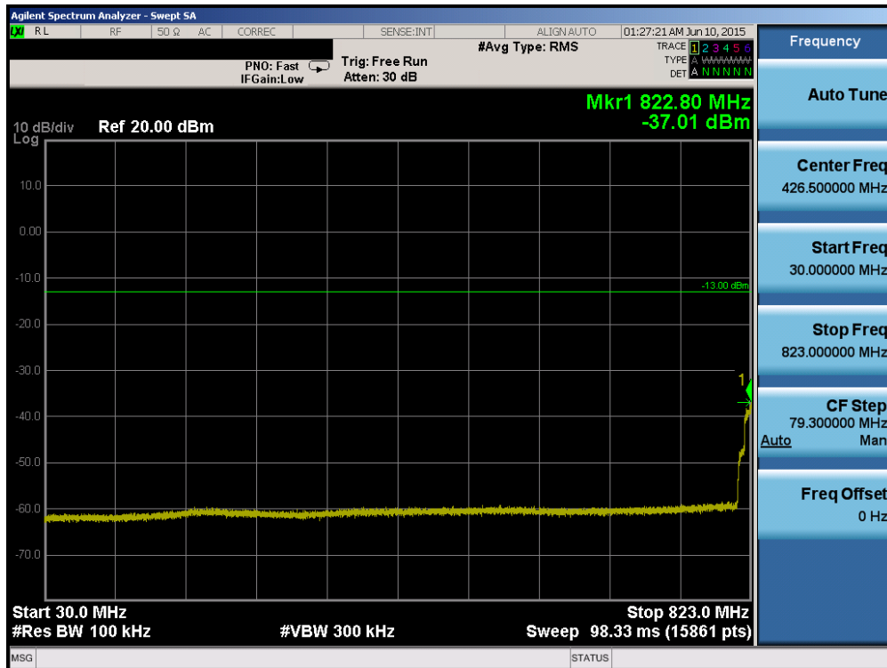
Plot 6-46. Conducted Spurious Plot (Band 5 – 10.0MHz QPSK – RB Size 1, RB Offset 0– Low Channel)
