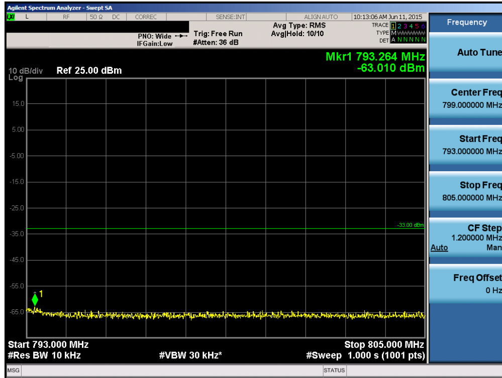
Plot 6-80. Upper Extended Band Edge Plot (Band 13 – 10.0MHz QPSK – RB Size 50)
