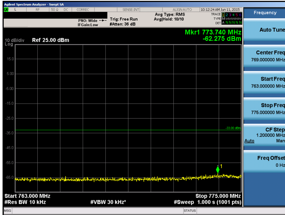
Plot 6-78. Lower Extended Band Edge Plot (Band 13 – 10.0MHz QPSK – RB Size 50)
