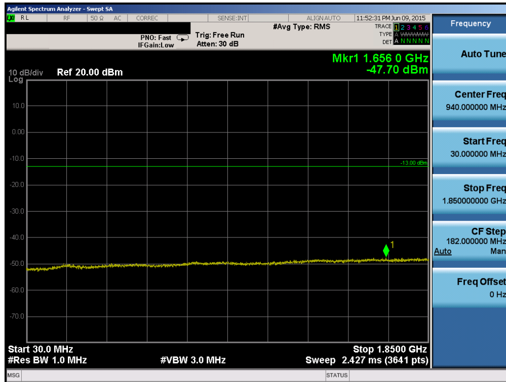
Plot 6-70. Conducted Spurious Plot (Band 2 – 10.0MHz QPSK – RB Size 1, RB Offset 0 – High Channel)
