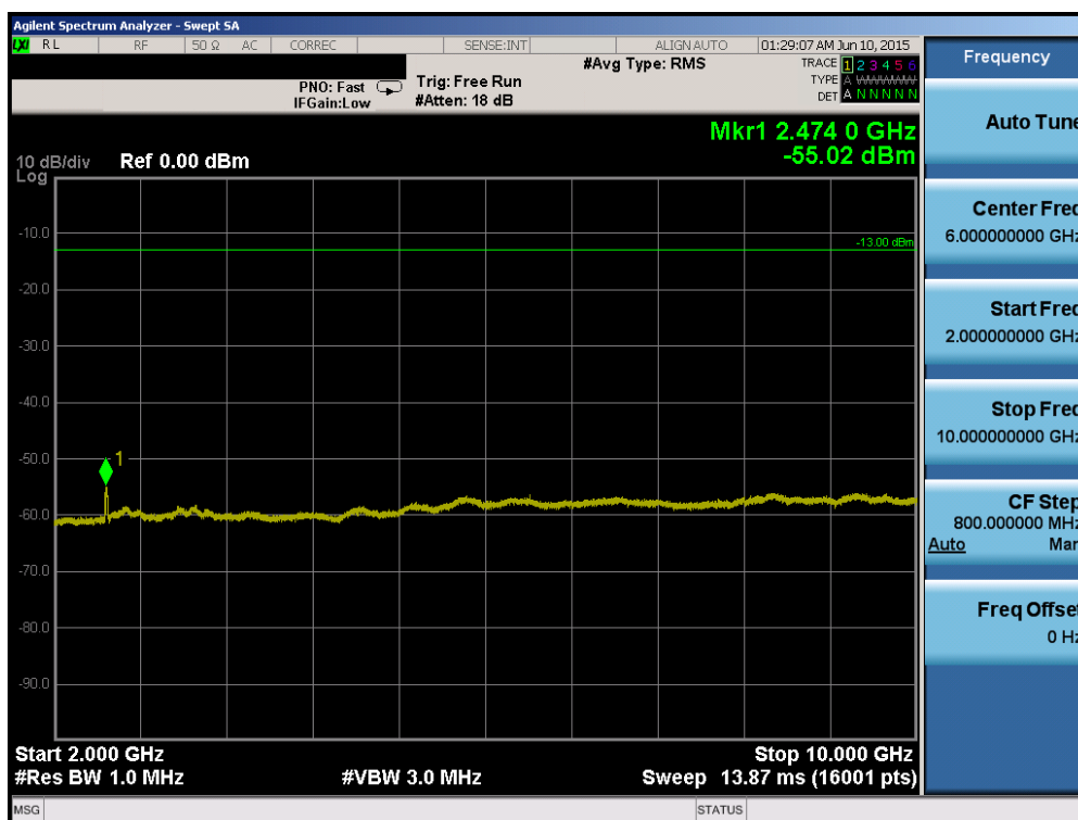
Plot 6-48. Conducted Spurious Plot (Band 5 – 10.0MHz QPSK – RB Size 1, RB Offset 0 – Low Channel)
