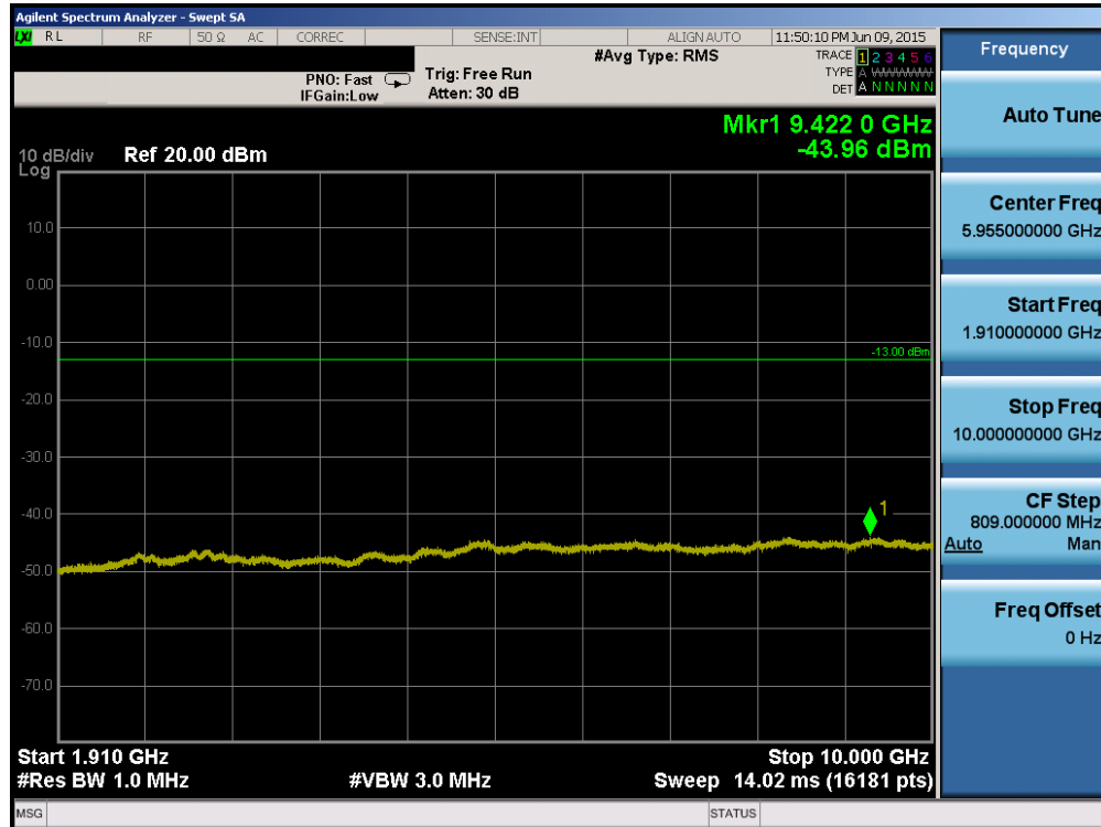
Plot 6-65. Conducted Spurious Plot (Band 2 – 10.0MHz QPSK – RB Size 1, RB Offset 0 – Low Channel)
