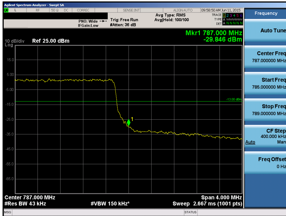
Plot 6-75. Upper Band Edge Plot (Band 13 – 5.0MHz QPSK – RB Size 25)
