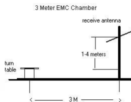
Figure 6-1. Test Instrument & Measurement Setup
