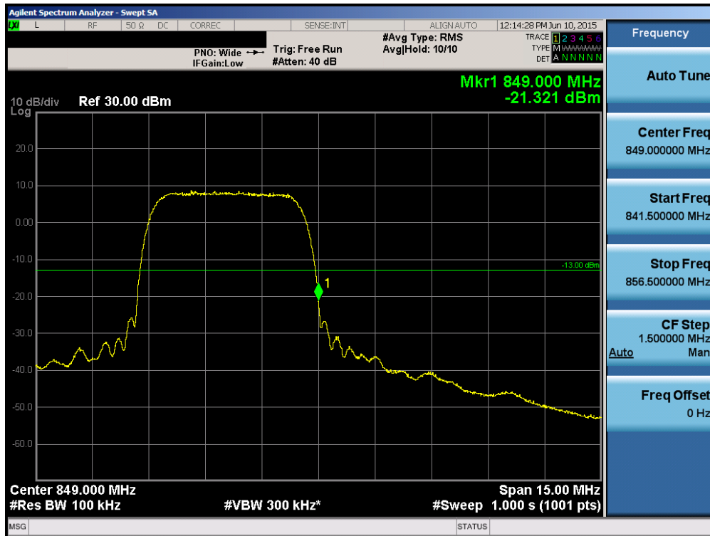
Plot 6-80. Band Edge Plot (Cellular WCDMA Mode – Ch. 4233)
