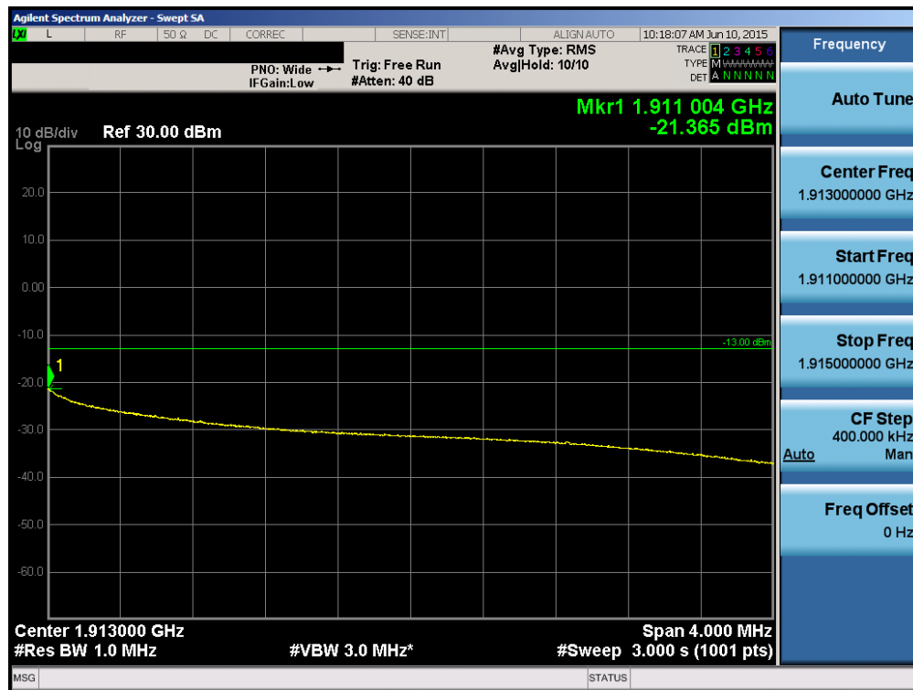
Plot 6-78. 4MHz Span Plot (PCS CDMA Mode – Ch. 1175)
