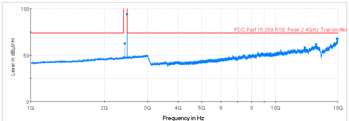
Plot 6-47. Radiated Spurious Plot above 1GHz (BT – Ch. 78, Ant. Pol. V)
