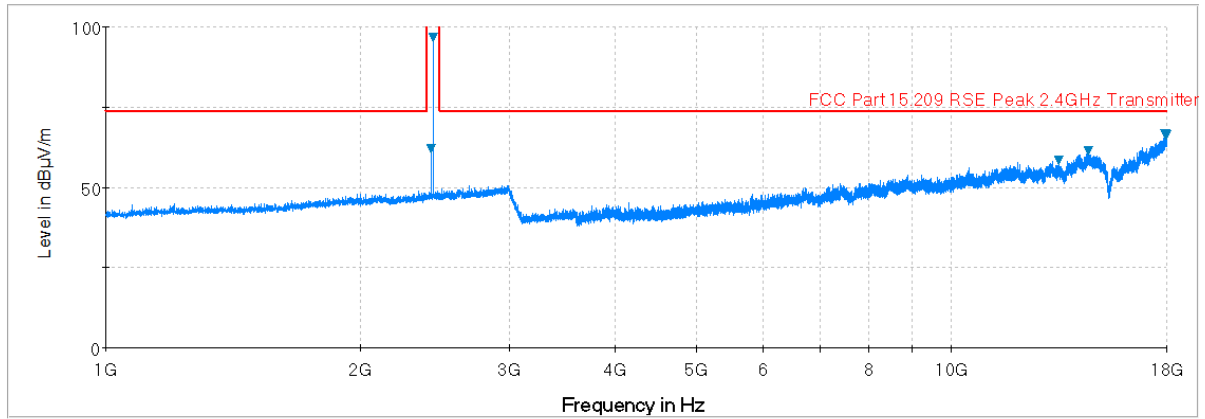
Plot 6-45. Radiated Spurious Plot above 1GHz (BT – Ch. 39, Ant. Pol. V)
