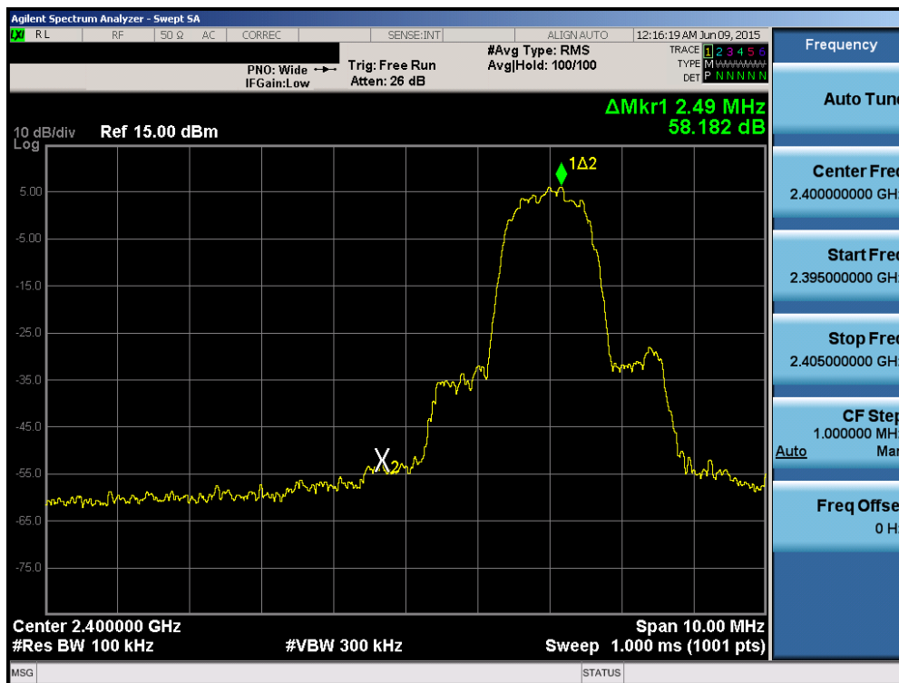
Plot 6-28. Band Edge Plot (Bluetooth with Hopping Disabled, 3 Mbps – Ch. 0)
