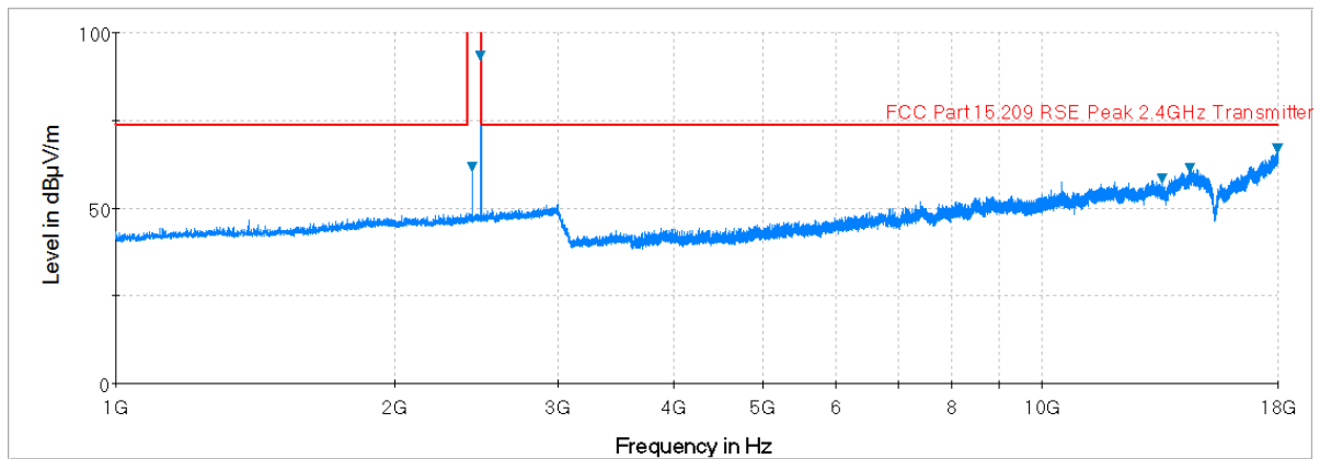
Plot 6-46. Radiated Spurious Plot above 1GHz (BT – Ch. 78, Ant. Pol. H)
