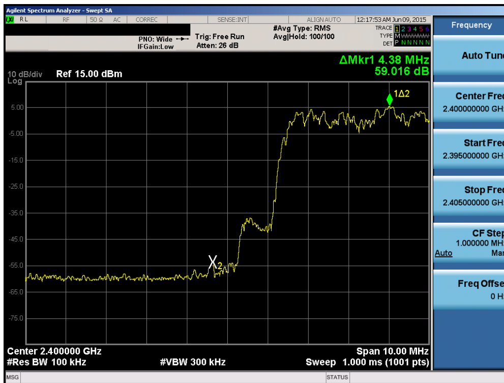
Plot 6-30. Band Edge Plot (Bluetooth with Hopping Enabled, 3 Mbps)
