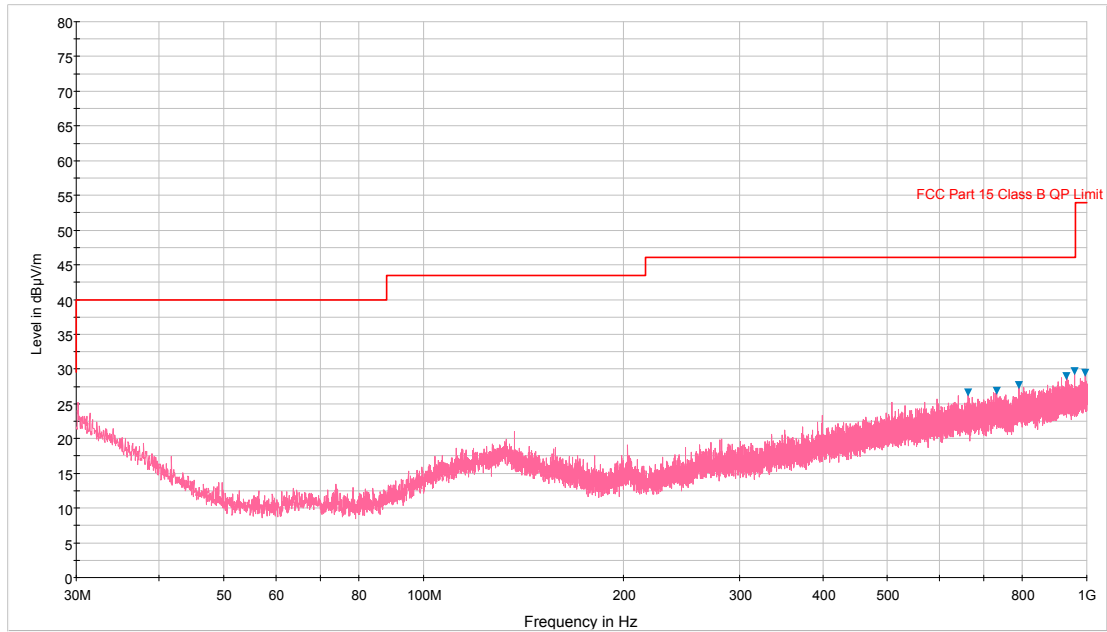
Plot 6-226. Radiated Spurious Plot below 1GHz (5GHz – 2.4GHz, Ant. Pol. V)
