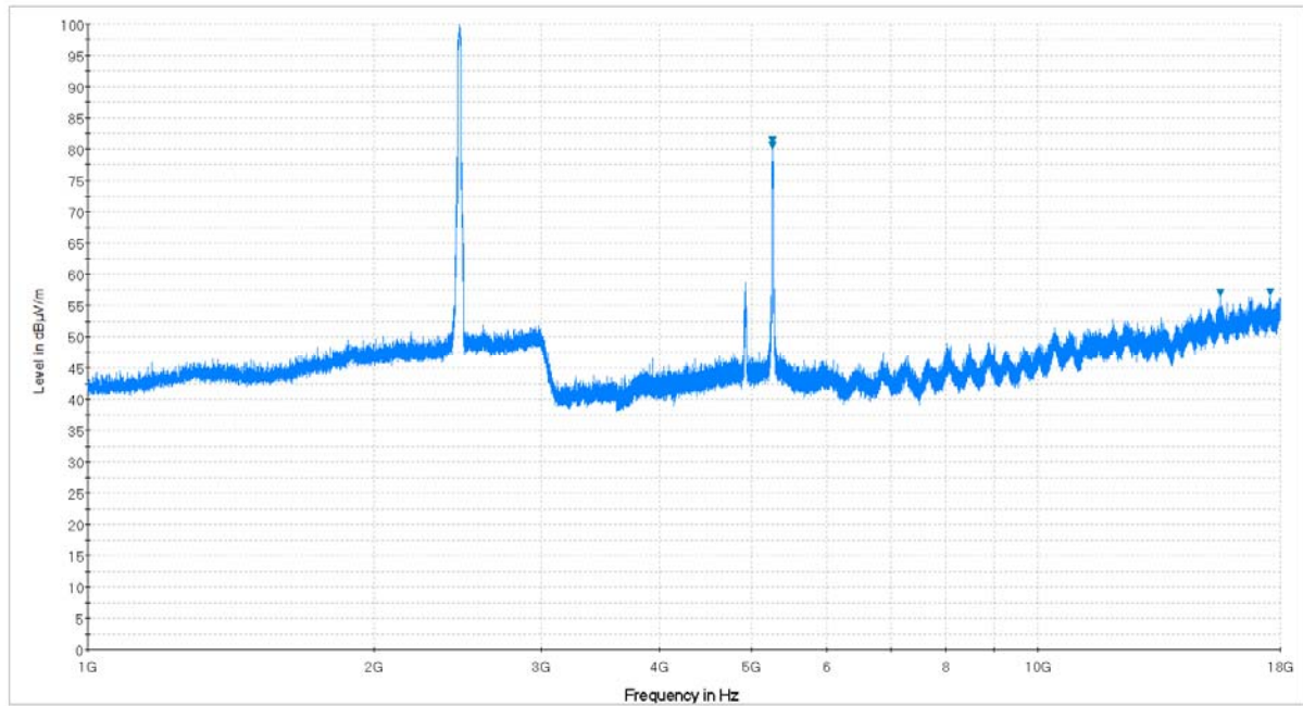
Plot 6-173. Radiated Spurious Plot above 1GHz (2.4GHz [ANT1] – 5GHz [ANT2], Ant. Pol. H)
