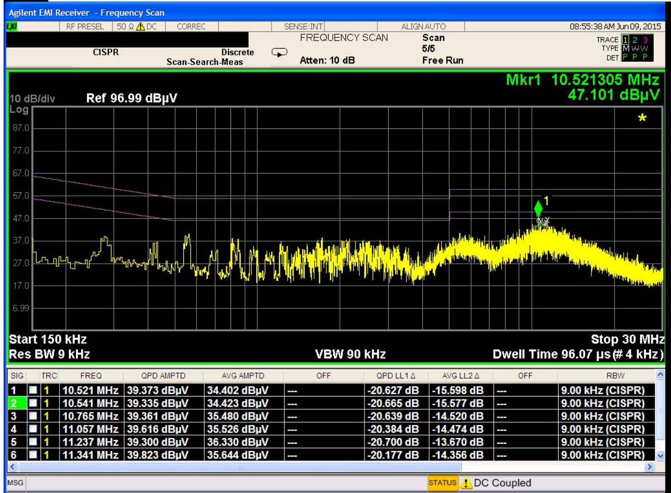
Plot 6-233. Line Conducted Plot with 802.11a UNII Band 3 (L1)
