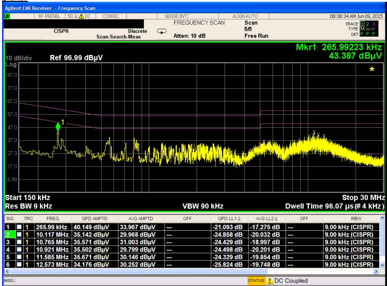
Plot 6-228. Line Conducted Plot with 802.11a UNII Band 1 (N)
