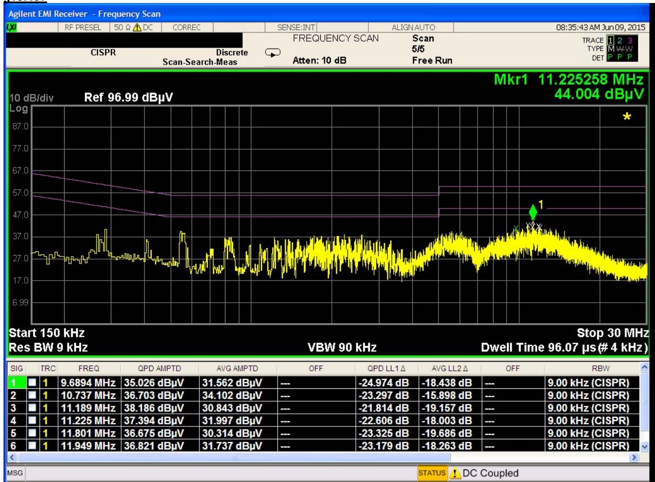
Plot 6-227. Line Conducted Plot with 802.11a UNII Band 1 (L1)
