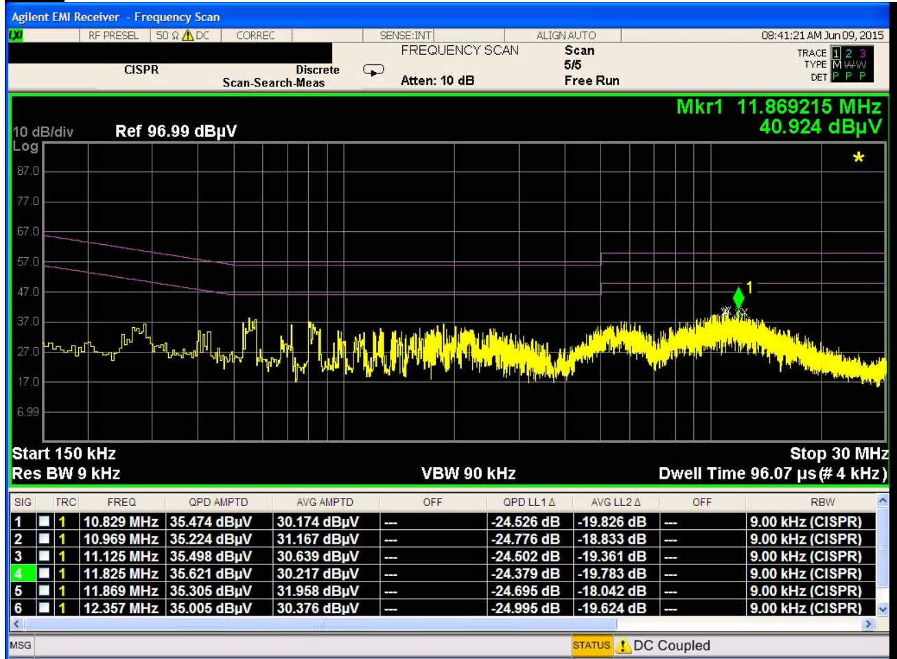
Plot 6-230. Line Conducted Plot with 802.11a UNII Band 2A (N)
