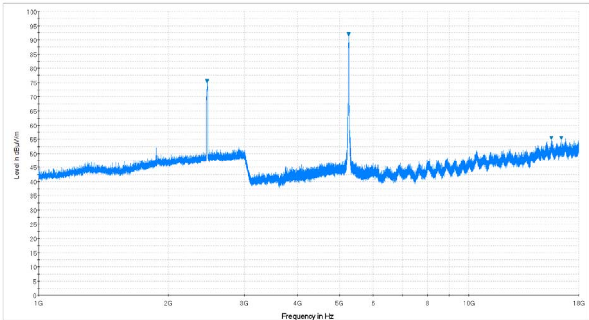
Plot 6-176. Radiated Spurious Plot above 1GHz (5GHz [ANT1] – 2.4GHz [ANT2], Ant. Pol. V)
