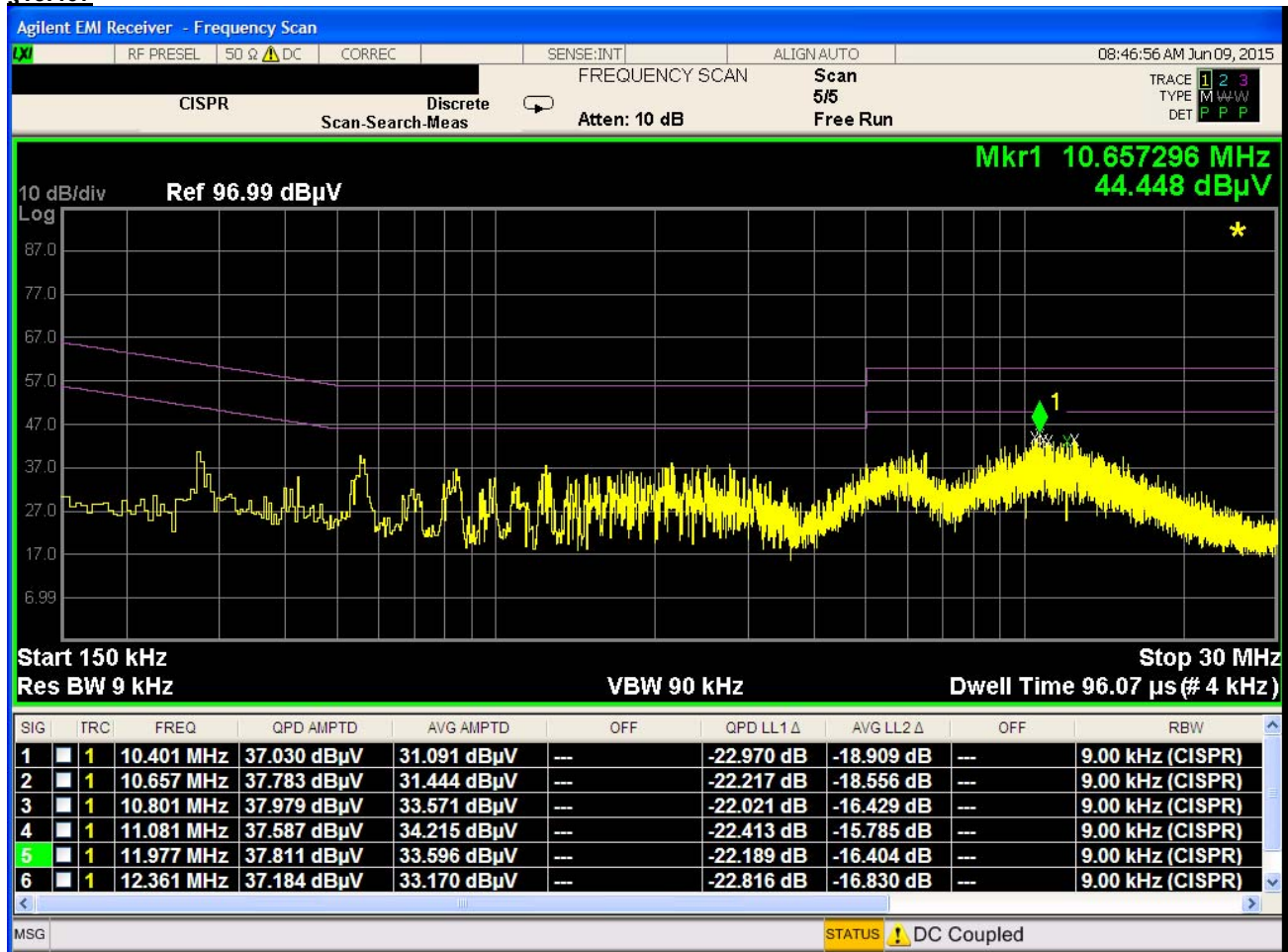
Plot 6-231. Line Conducted Plot with 802.11a UNII Band 2C (L1)
