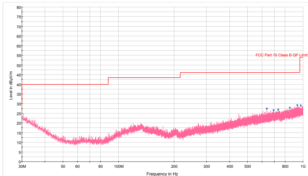
Plot 6-225. Radiated Spurious Plot below 1GHz (5GHz – 2.4GHz, Ant. Pol. H)
