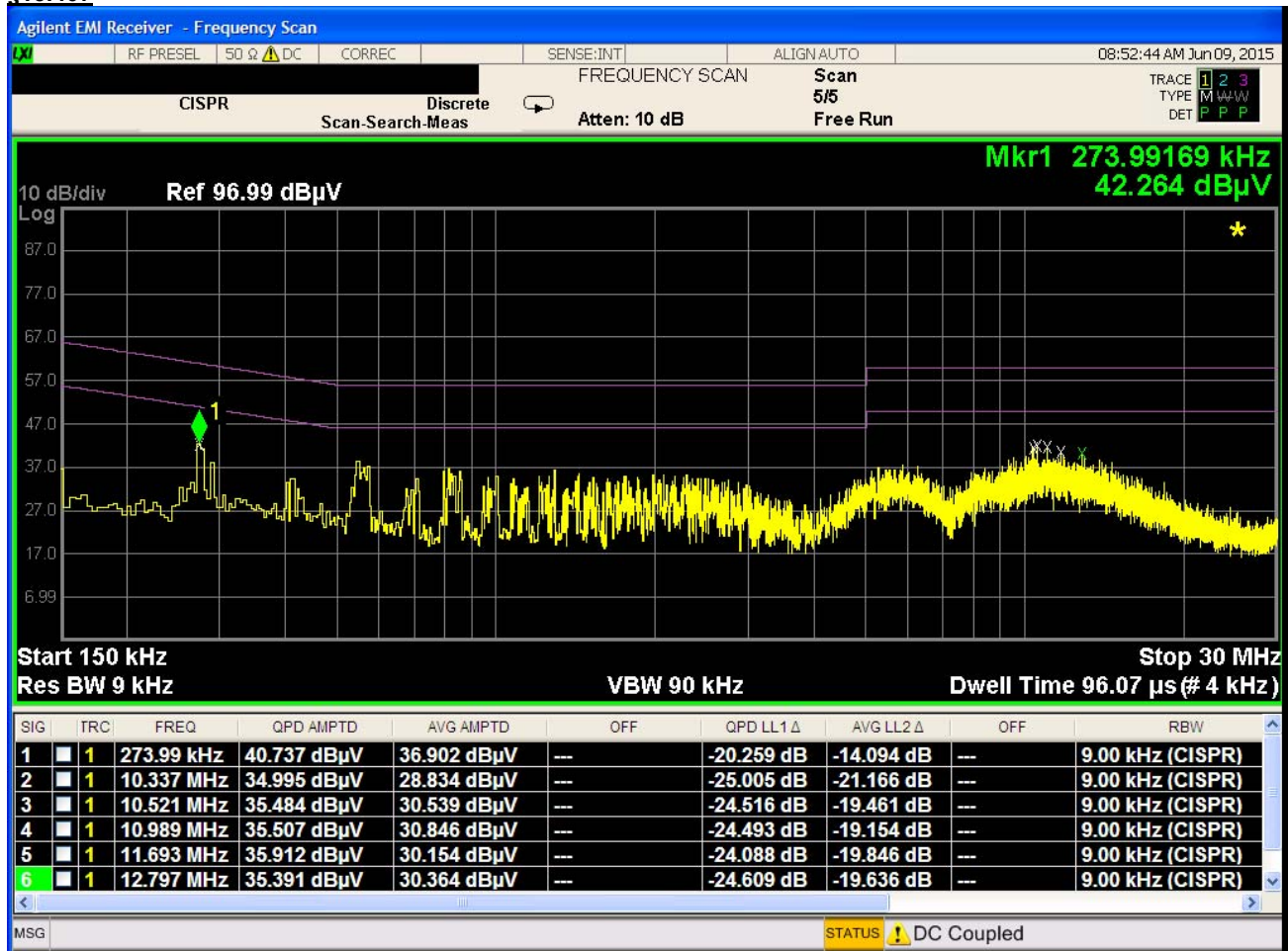
Plot 6-234. Line Conducted Plot with 802.11a UNII Band 3 (N)
