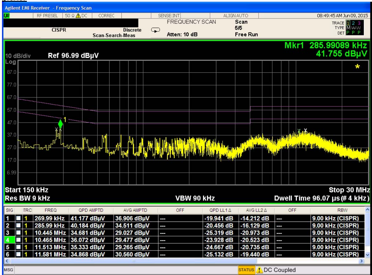
Plot 6-232. Line Conducted Plot with 802.11a UNII Band 2C (N)
