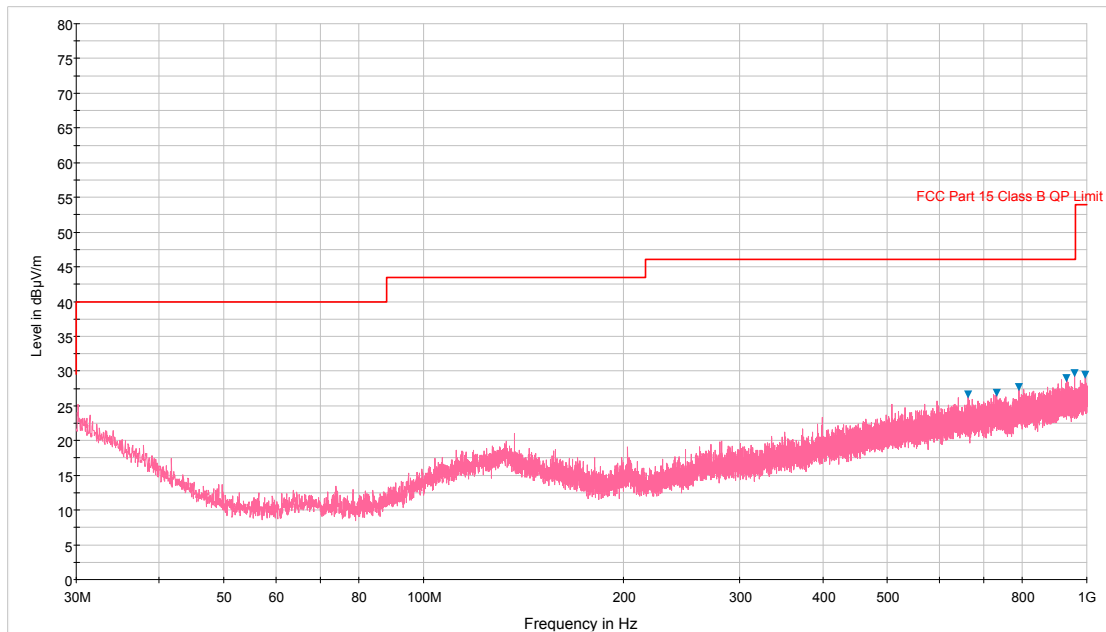
Plot 6-224. Radiated Spurious Plot below 1GHz (2.4GHz – 5 GHz, Ant. Pol. V)
