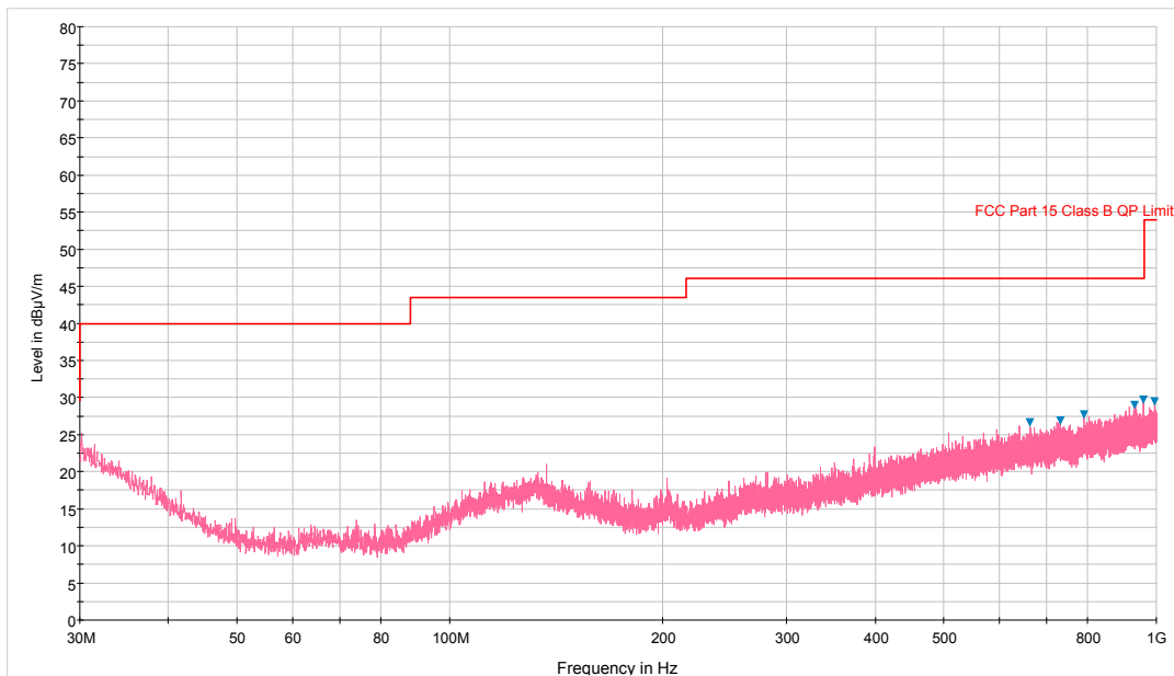
Plot 6-223. Radiated Spurious Plot below 1GHz (2.4GHz – 5 GHz, Ant. Pol. H)
