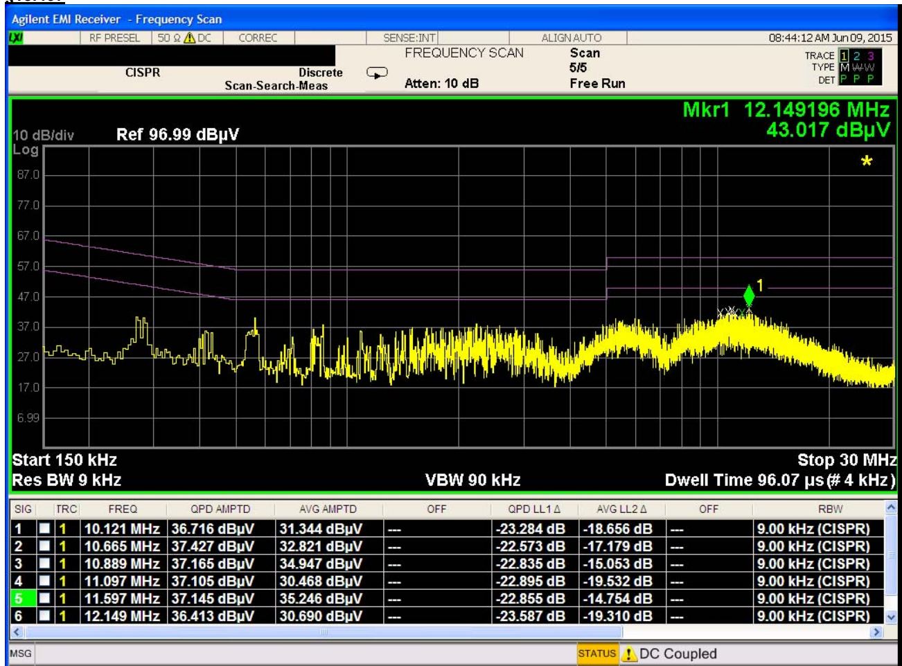
Plot 6-229. Line Conducted Plot with 802.11a UNII Band 2A (L1)
