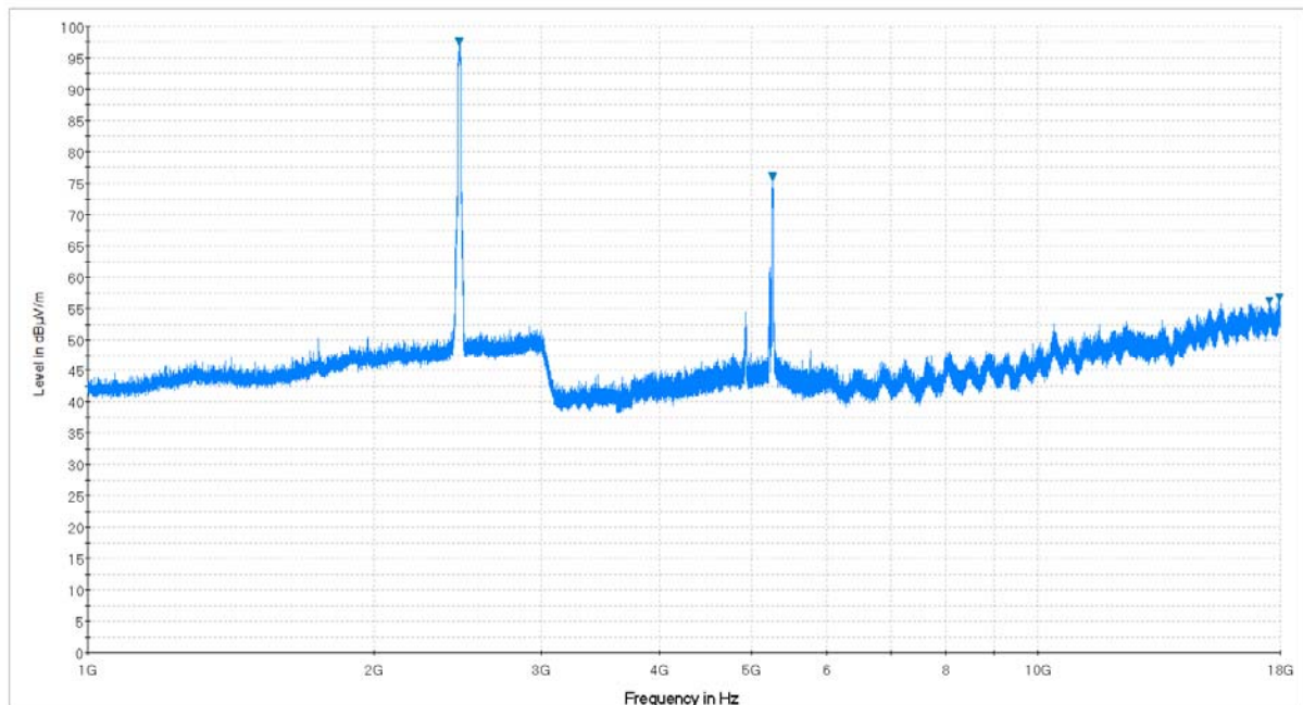
Plot 6-174. Radiated Spurious Plot above 1GHz (2.4GHz [ANT1] – 5GHz [ANT2], Ant. Pol. V)
