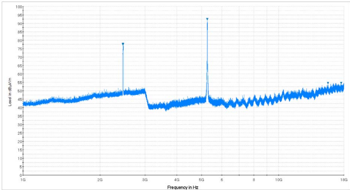
Plot 6-175. Radiated Spurious Plot above 1GHz (5GHz [ANT1] – 2.4GHz [ANT2], Ant. Pol. H)
