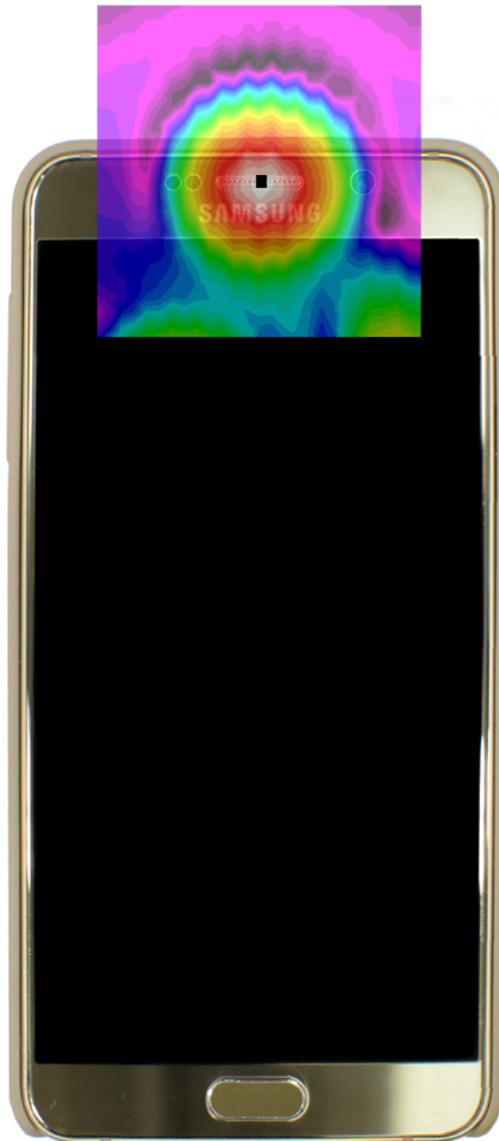
Figure 12-3 Axial T-coil Scan Overlay Magnetic Field Distributions
