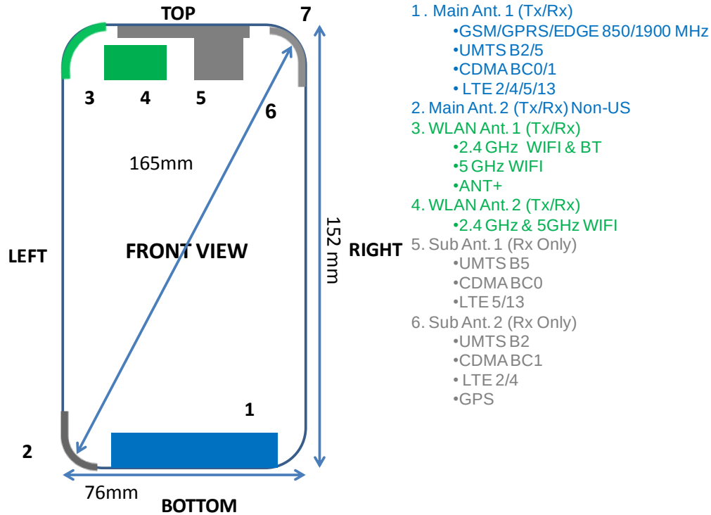
Figure F-1 DUT Antenna Locations
