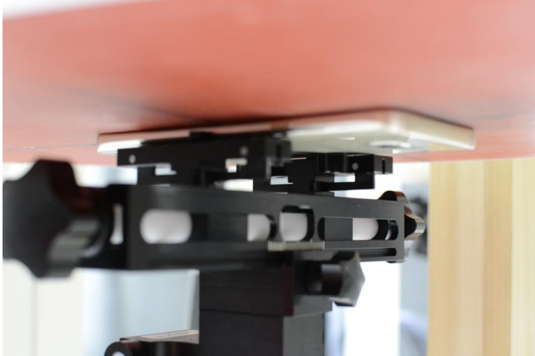
SAR Test Setup Photo 9— Front Side at 0.0 cm (Extremity)
