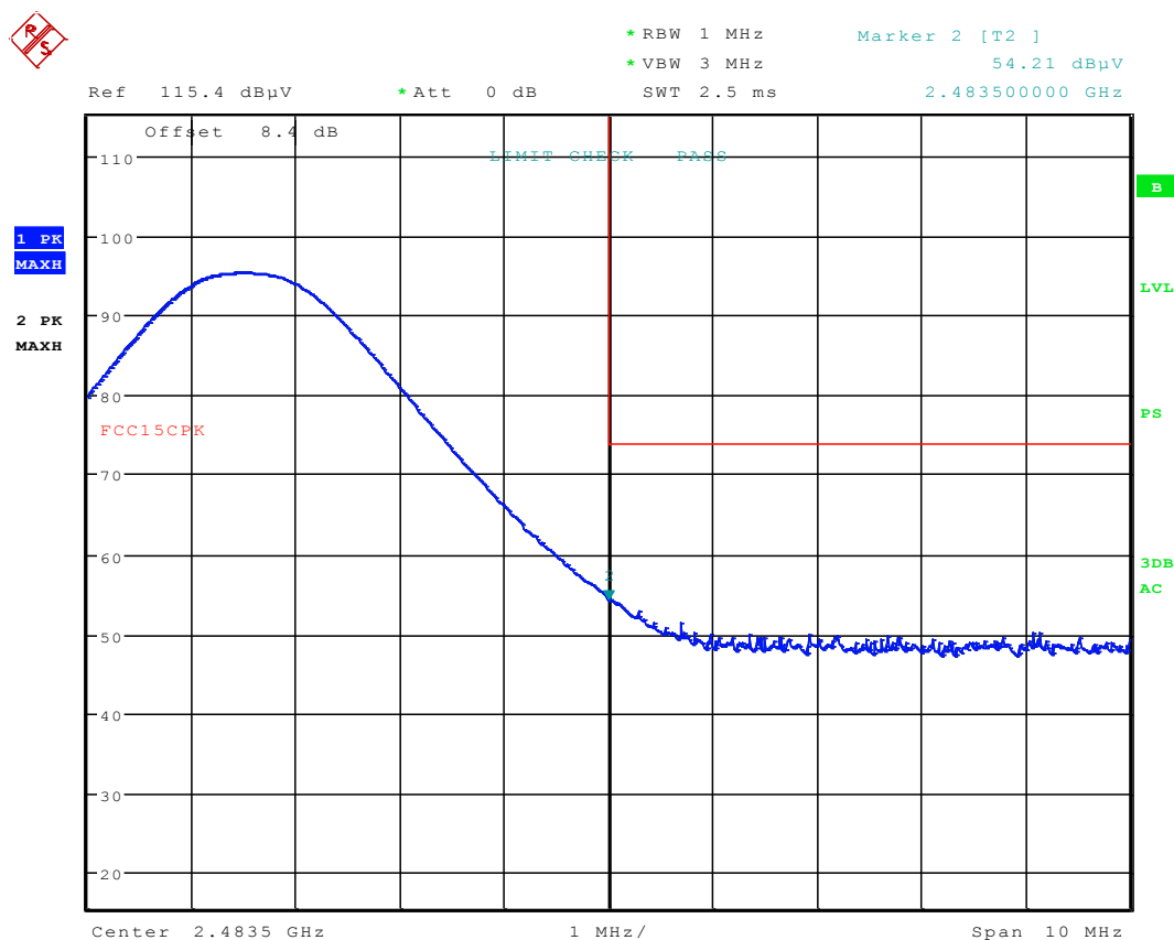
Plot 6-2. Radiated Restricted Upper Band Edge Measurement (Peak)
