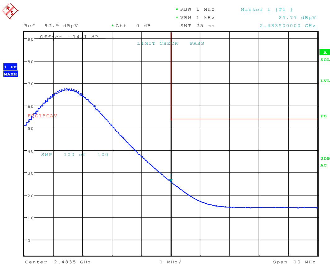
Plot 6-1. Radiated Restricted Upper Band Edge Measurement (Average)
