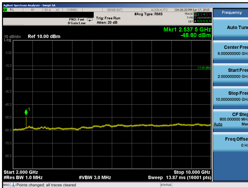
Plot 6-34. Conducted Spurious Plot (Cellular WCDMA Mode – Ch. 4233)
