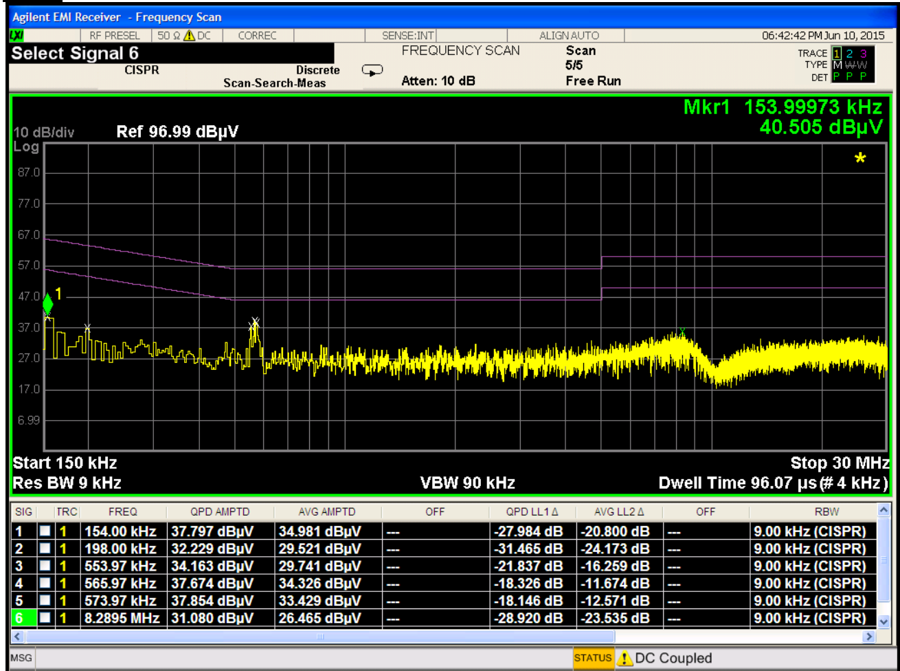
Plot 6-254. Line Conducted Plot with 802.11a UNII Band 3 (L1)
