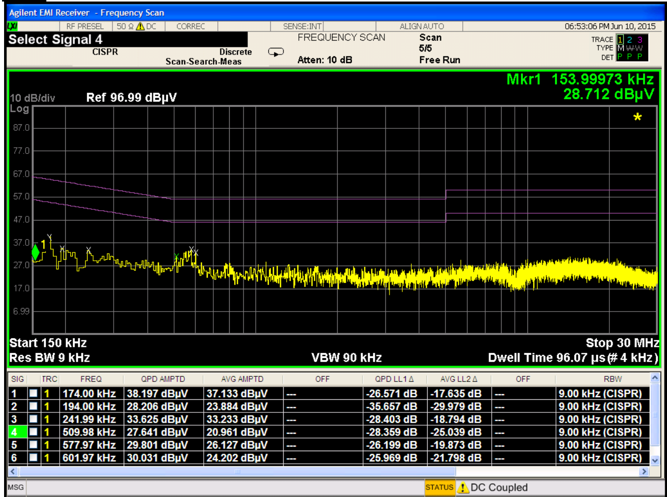
Plot 6-251. Line Conducted Plot with 802.11a UNII Band 2A (N)
