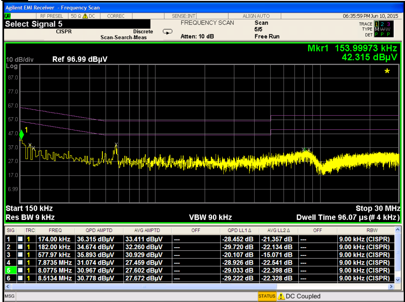
Plot 6-250. Line Conducted Plot with 802.11a UNII Band 2A (L1)
