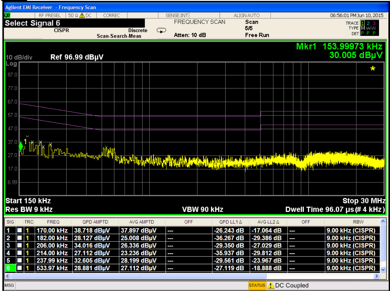
Plot 6-249. Line Conducted Plot with 802.11a UNII Band 1 (N)
