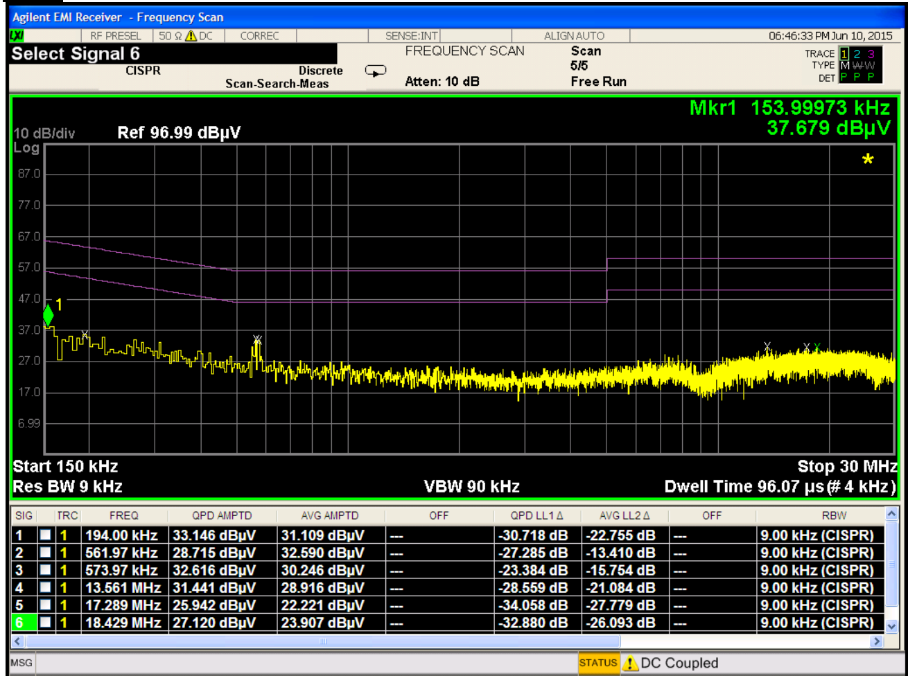
Plot 6-255. Line Conducted Plot with 802.11a UNII Band 3 (N)
