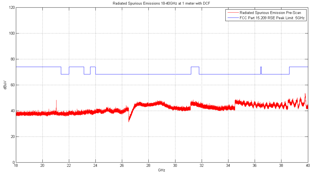
Plot 6-178. Radiated Spurious Plot above 18GHz (Config-1, Ant. Pol. V)
