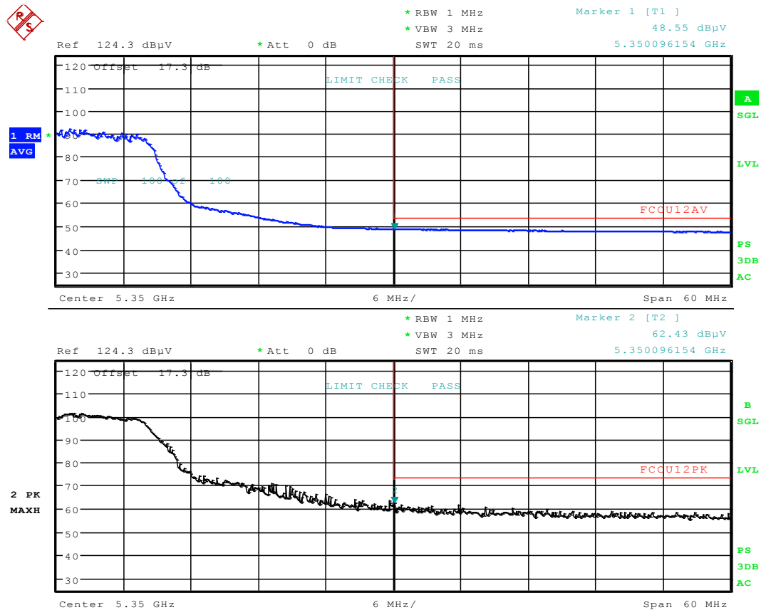
Plot 6-2. Radiated Restricted Upper Band Edge Plot (Average & Peak – UNII Band 2A)
