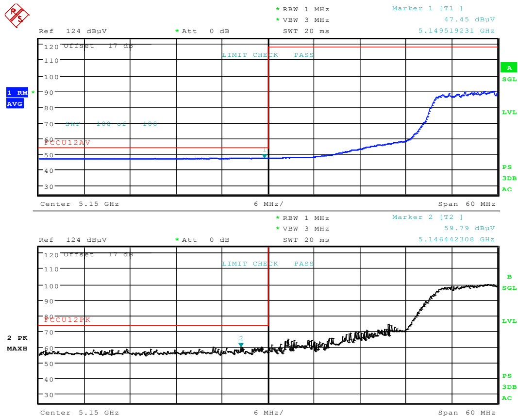
Plot 6-1. Radiated Restricted Lower Band Edge Plot (Average & Peak – UNII Band 1)
