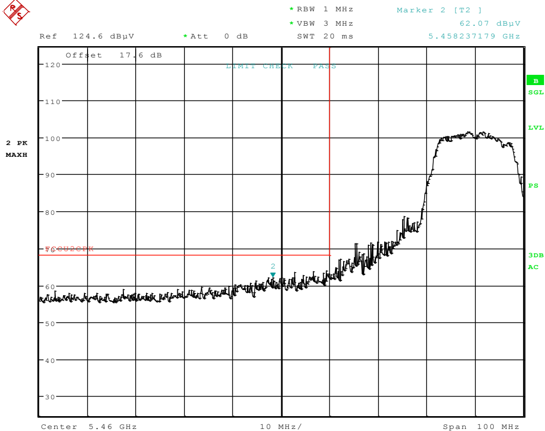
Plot 6-4. Radiated Restricted Lower Band Edge Plot (Peak – UNII Band 2C)
