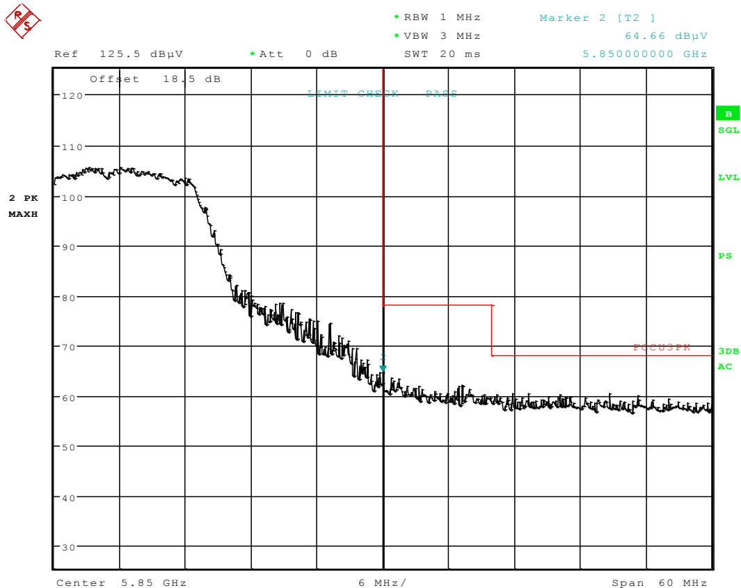
Plot 6-5. Radiated Upper Band Edge Plot (Peak – UNII Band 3)
