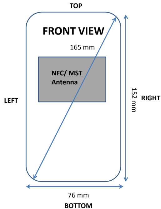
Figure F-2 NFC / MST Antenna Location
