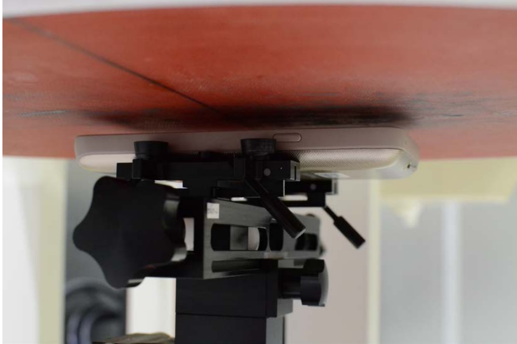
SAR Test Setup Photo 7— Front Side at 1.0 cm (Hotspot)
