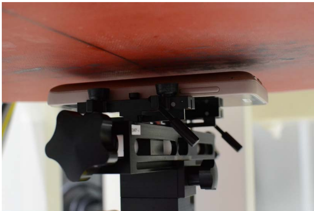
SAR Test Setup Photo 5– Back Side at 1.0 cm (Hotspot)
