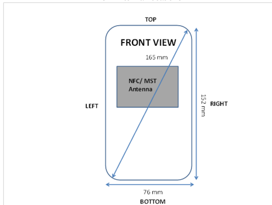
Figure F-2 NFC Antenna Location
