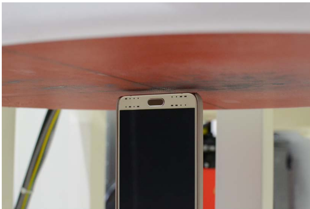
SAR Test Setup Photo 11— Bottom Edge at 0.3 cm (Phablet)
