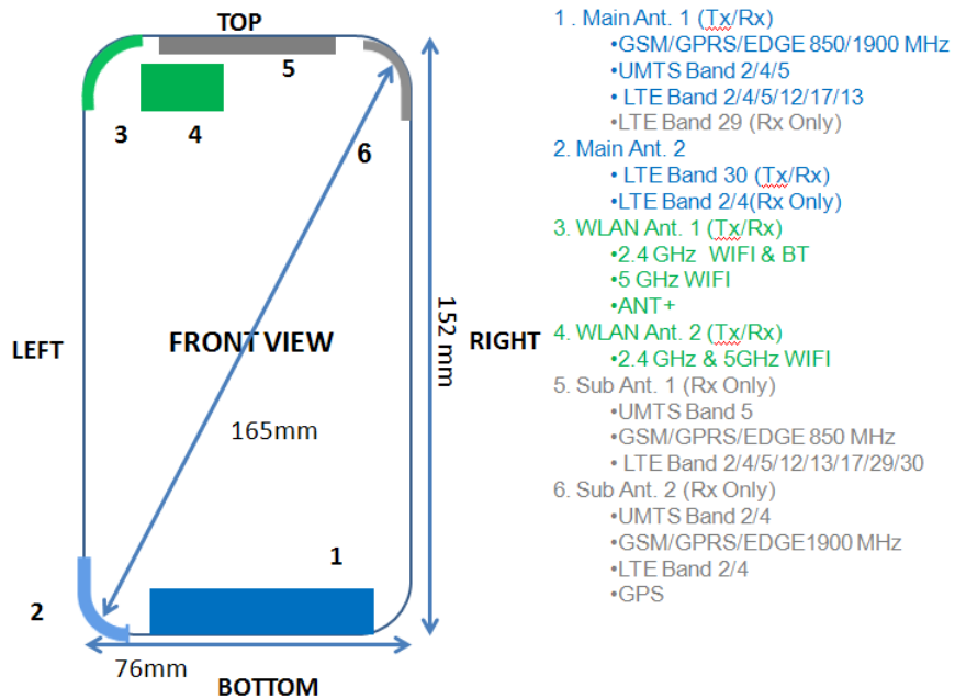
Figure F-1 DUT Antenna Locations
