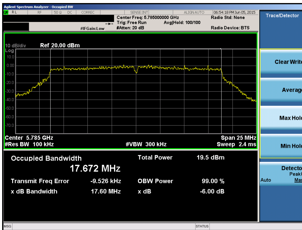
Plot 6-63. 6dB Bandwidth Plot (20MHz BW 802.11n (UNII Band 3) – Ch. 157)
