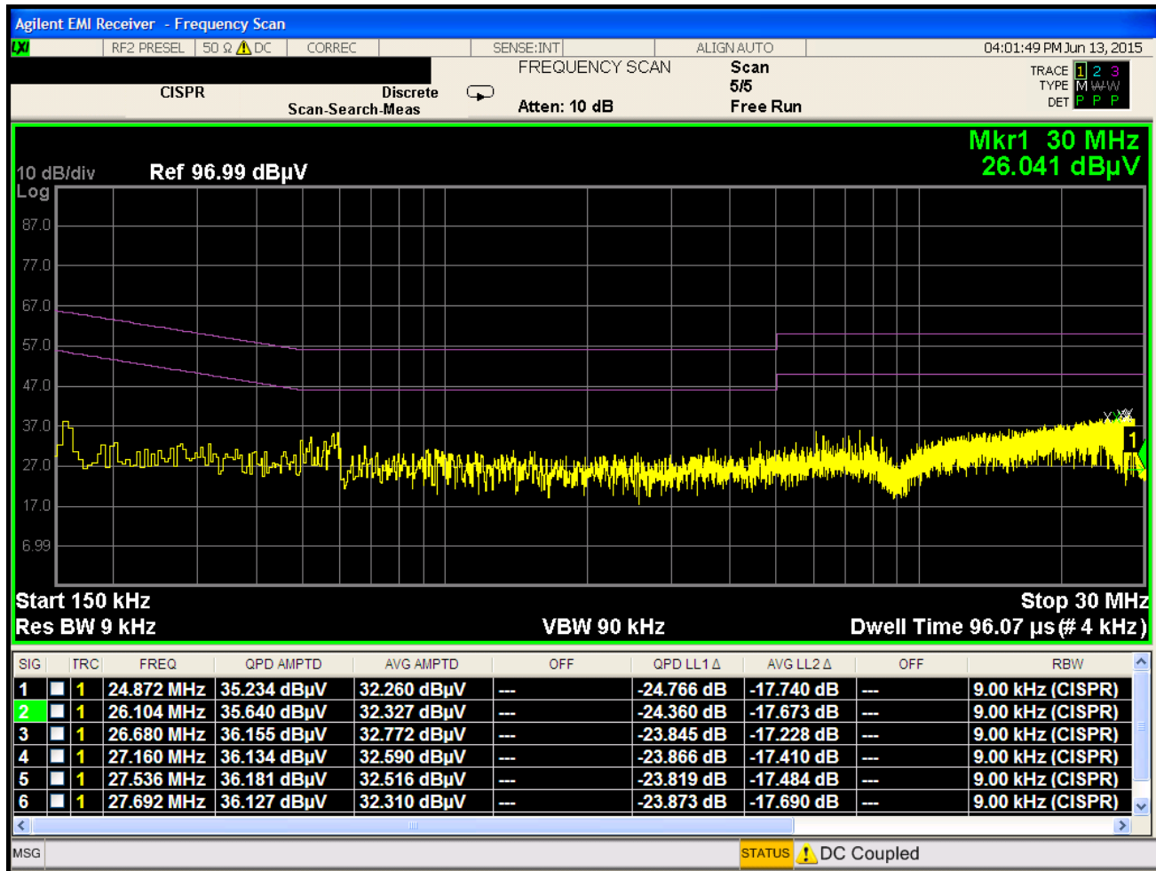
Plot 6-247. Line Conducted Plot with 802.11a UNII Band 1 (N)
