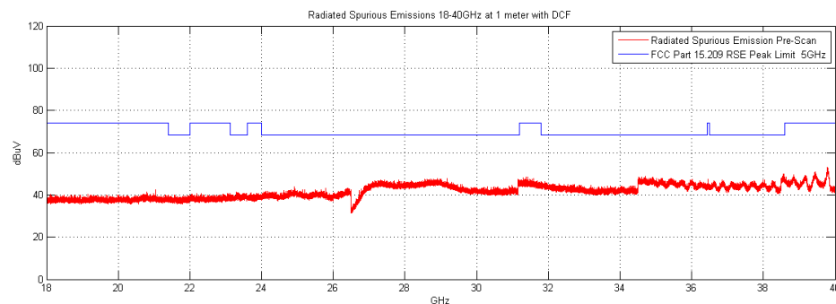
Plot 6-177. Radiated Spurious Plot above 18GHz (Simultaneous Tx Config-1, Pol. H)
