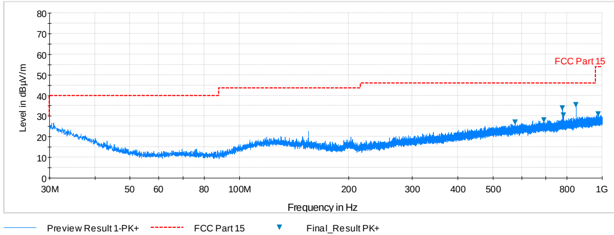
Plot 6-238. Radiated Spurious Plot below 1GHz (802.11a – U3 Ch. 157, Ant. Pol. H)
