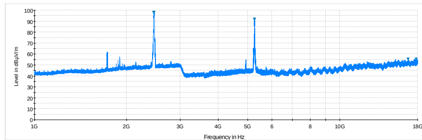
Plot 6-174. Radiated Spurious Plot above 1GHz (Simultaneous Tx Config-1, Pol. V)
