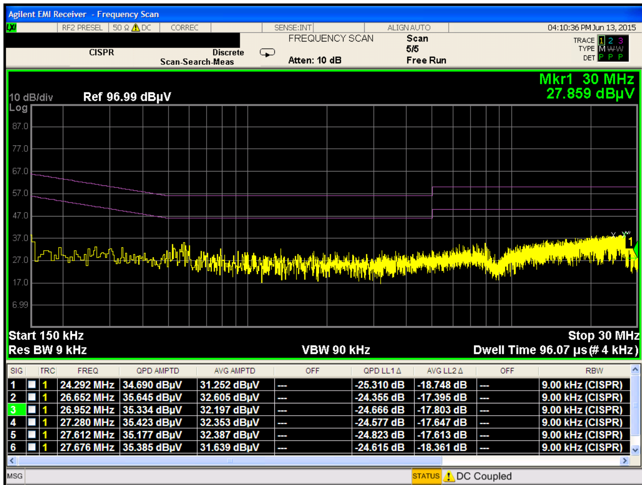
Plot 6-251. Line Conducted Plot with 802.11a UNII Band 2C (N)
