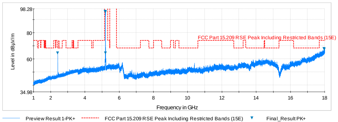
Plot 6-164. Radiated Spurious Plot above 1GHz (802.11a – U1 Ch. 40, Ant. Pol. V)
