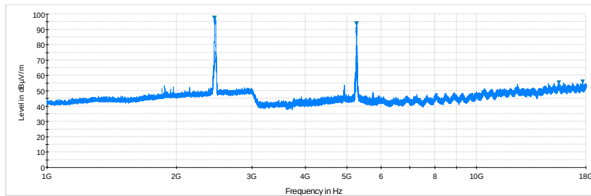
Plot 6-173. Radiated Spurious Plot above 1GHz (Simultaneous Tx Config-1, Pol. H)
