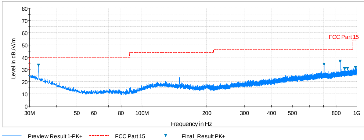
Plot 6-239. Radiated Spurious Plot below 1GHz (802.11a – U3 Ch. 157, Ant. Pol. V)
