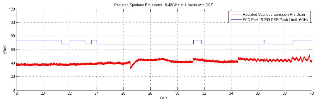
Plot 6-180. Radiated Spurious Plot above 18GHz (Simultaneous Tx Config-2, Pol. V)
