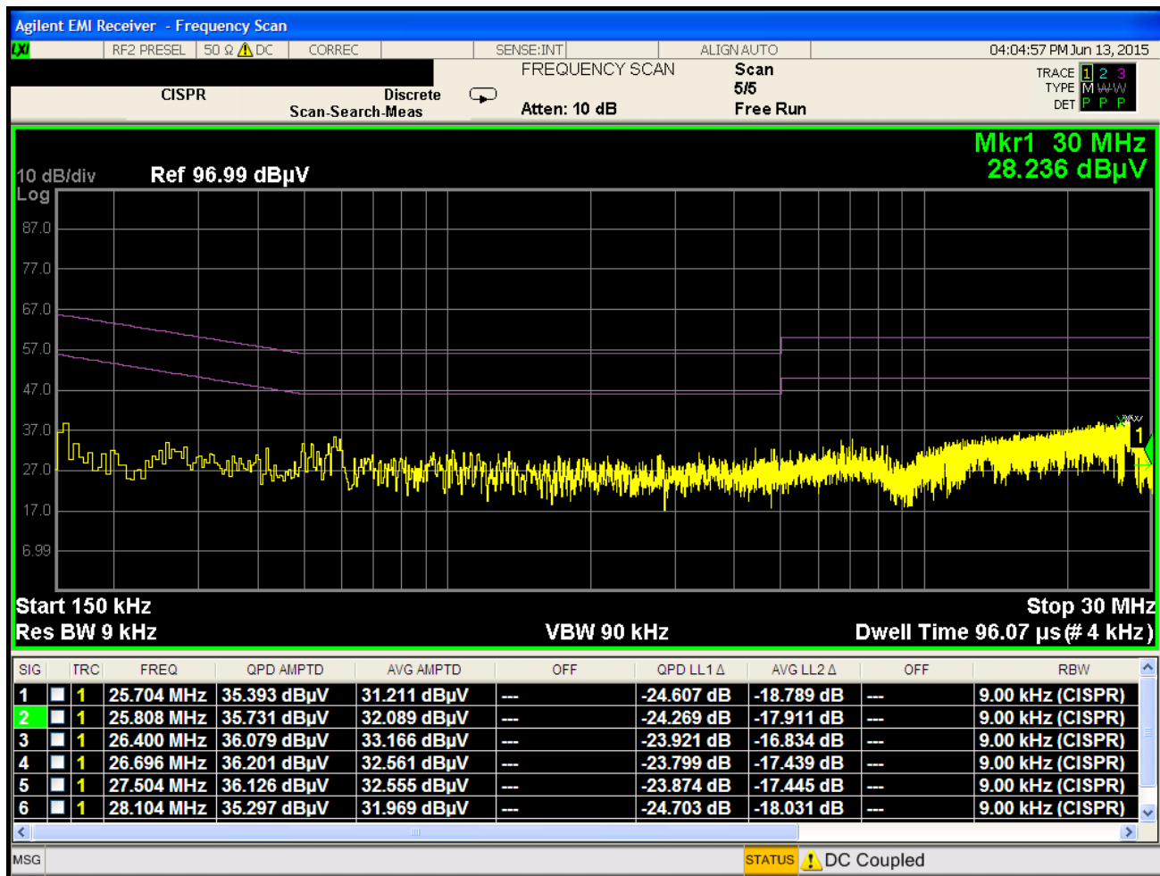
Plot 6-249. Line Conducted Plot with 802.11a UNII Band 2A (N)
