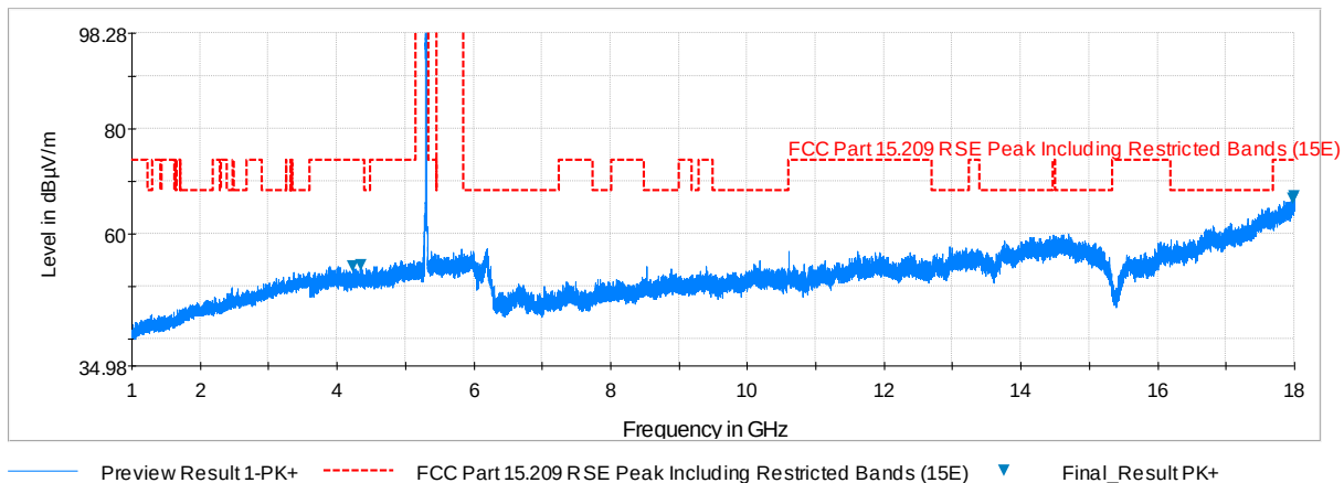
Plot 6-166. Radiated Spurious Plot above 1GHz (802.11a – U2A Ch. 56, Ant. Pol. V)
