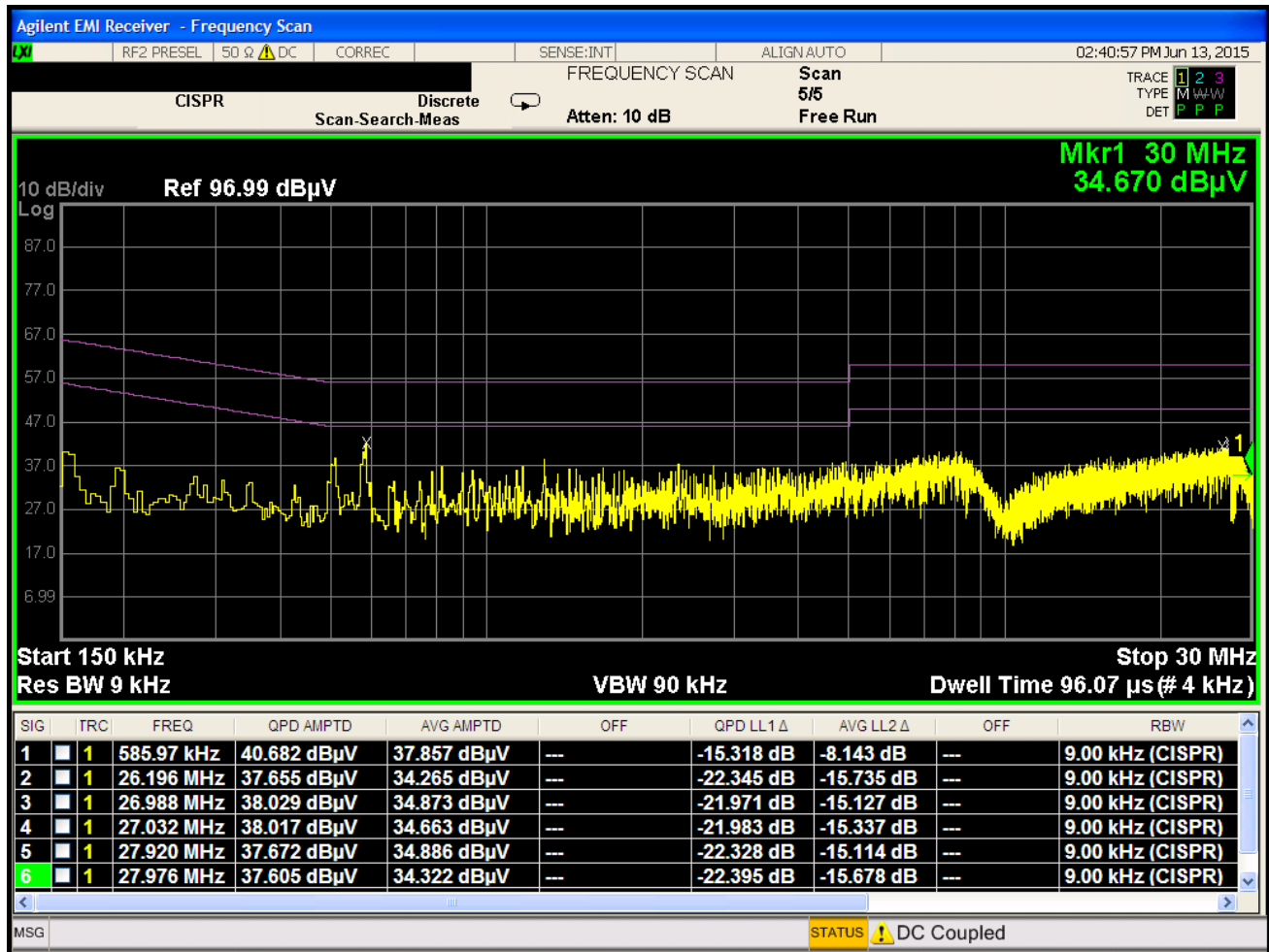
Plot 6-246. Line Conducted Plot with 802.11a UNII Band 1 (L1)
