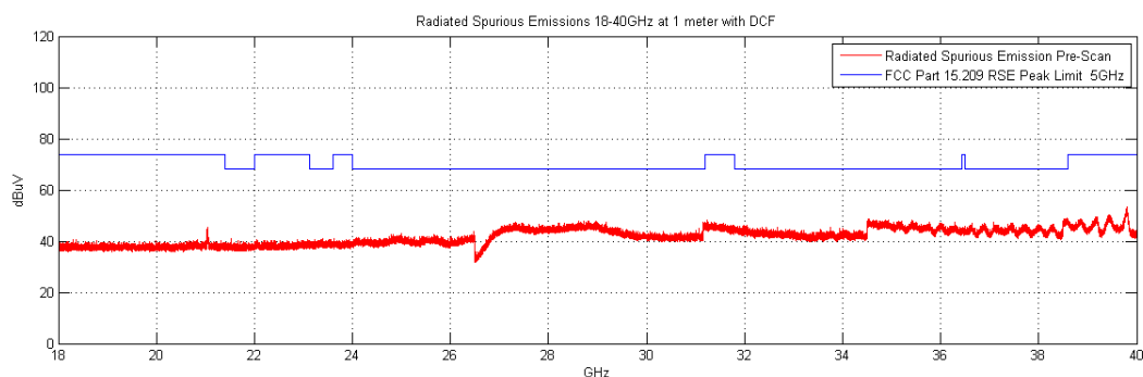
Plot 6-178. Radiated Spurious Plot above 18GHz (Simultaneous Tx Config-1, Pol. V)
