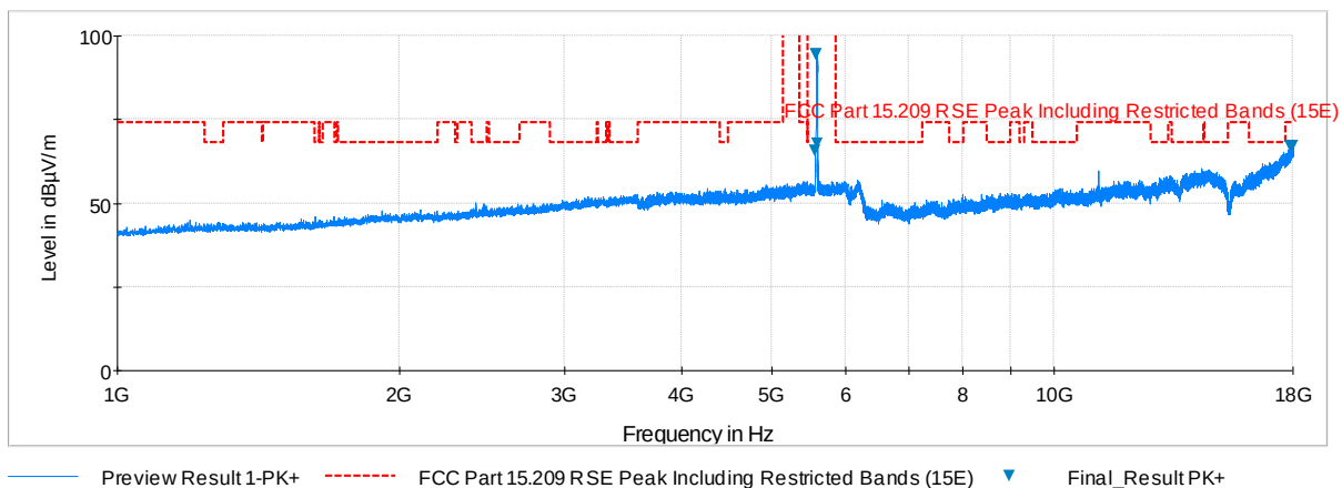
Plot 6-167. Radiated Spurious Plot above 1GHz (802.11a – U2C Ch. 116, Ant. Pol. H)
