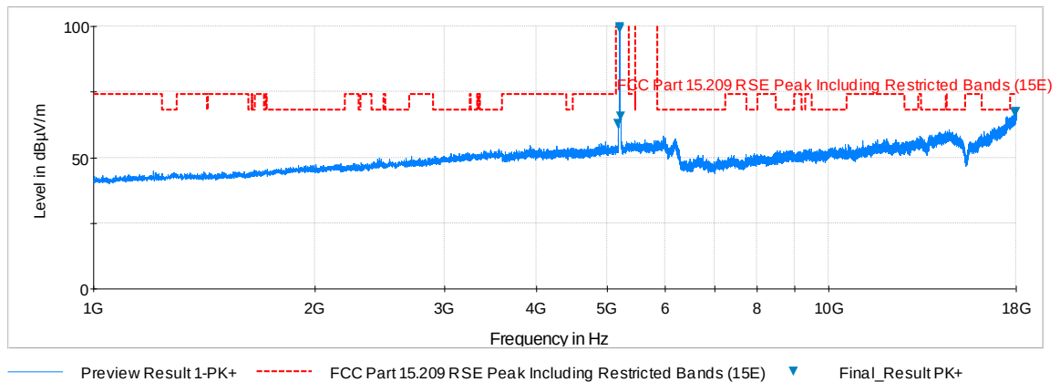
Plot 6-163. Radiated Spurious Plot above 1GHz (802.11a – U1 Ch. 40, Ant. Pol. H)
