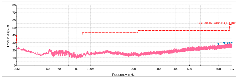
Plot 6-242. Radiated Spurious Plot below 1GHz (Ant. 1 – 2.4GHz, Ant. 2 – 5GHz, Pol. H)
