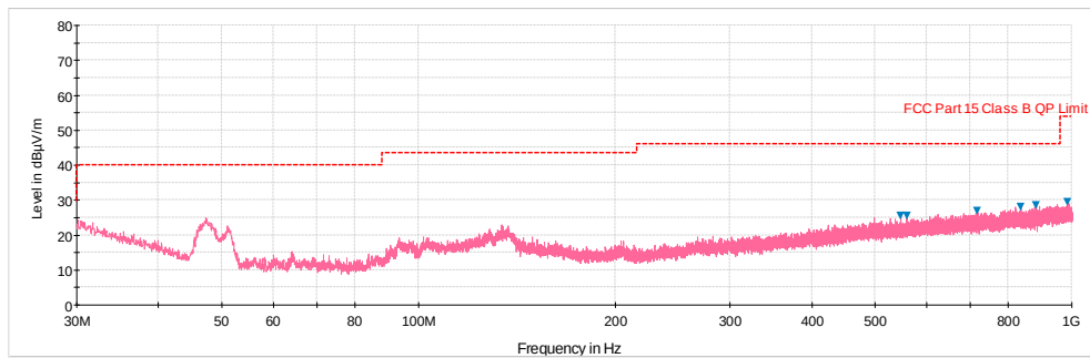
Plot 6-243. Radiated Spurious Plot below 1GHz (Ant. 1 – 2.4GHz, Ant. 2 – 5GHz, Pol. V)
