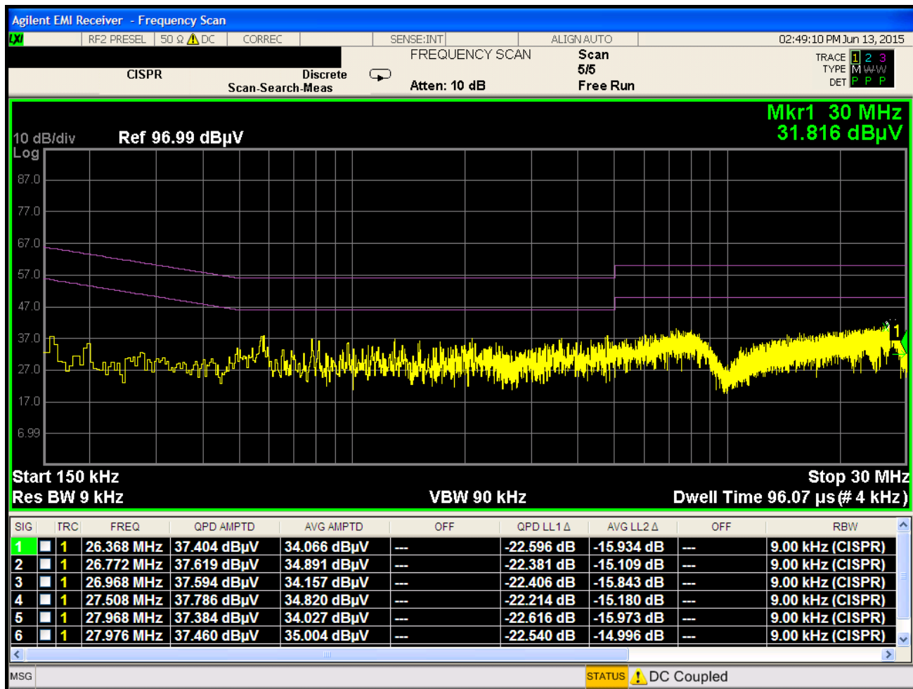
Plot 6-250. Line Conducted Plot with 802.11a UNII Band 2C (L1)
