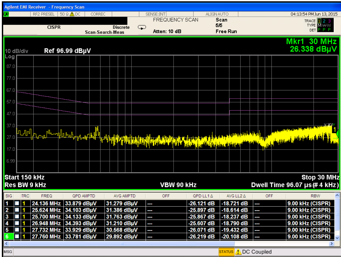
Plot 6-253. Line Conducted Plot with 802.11a UNII Band 3 (N)
