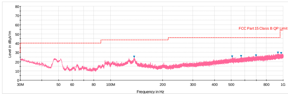
Plot 6-244. Radiated Spurious Plot below 1GHz (Ant. 1 – 5GHz, Ant. 2 – 2.4GHz, Pol. H)
