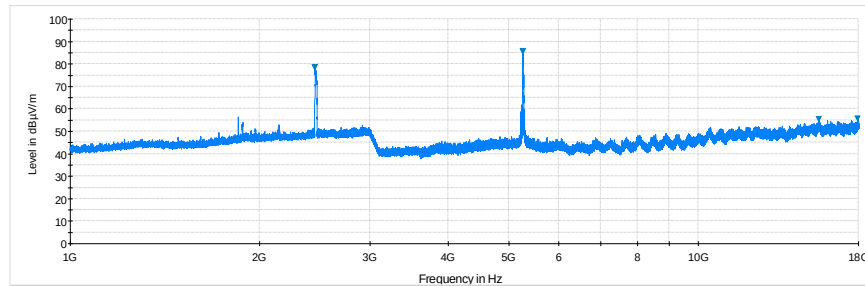
Plot 6-175. Radiated Spurious Plot above 1GHz (Simultaneous Tx Config-2, Pol. H)
