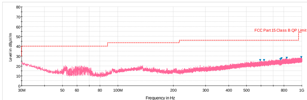
Plot 6-245. Radiated Spurious Plot below 1GHz (Ant. 1 – 5GHz, Ant. 2 – 2.4GHz, Pol. V)
