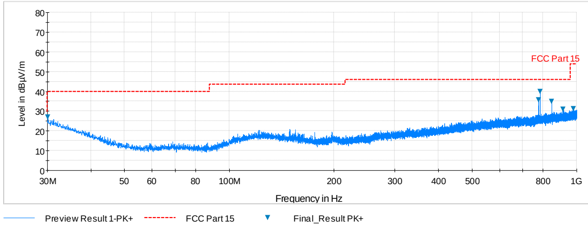
Plot 6-240. Radiated Spurious Plot below 1GHz (802.11a – U3 Ch. 157, Ant. Pol. H)
