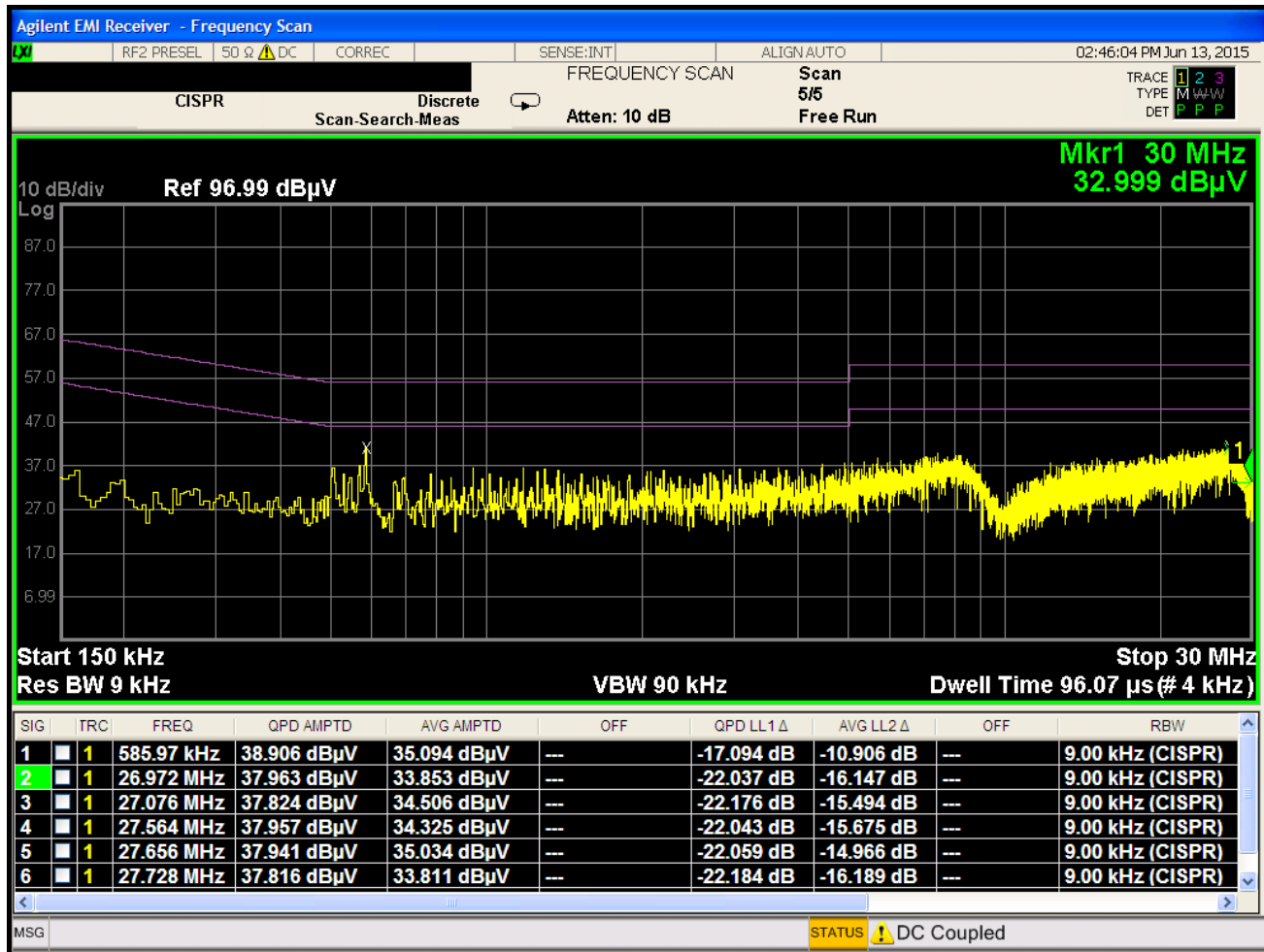
Plot 6-248. Line Conducted Plot with 802.11a UNII Band 2A (L1)
