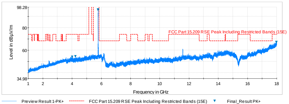
Plot 6-170. Radiated Spurious Plot above 1GHz (802.11a – U3 Ch. 157, Ant. Pol. V)
