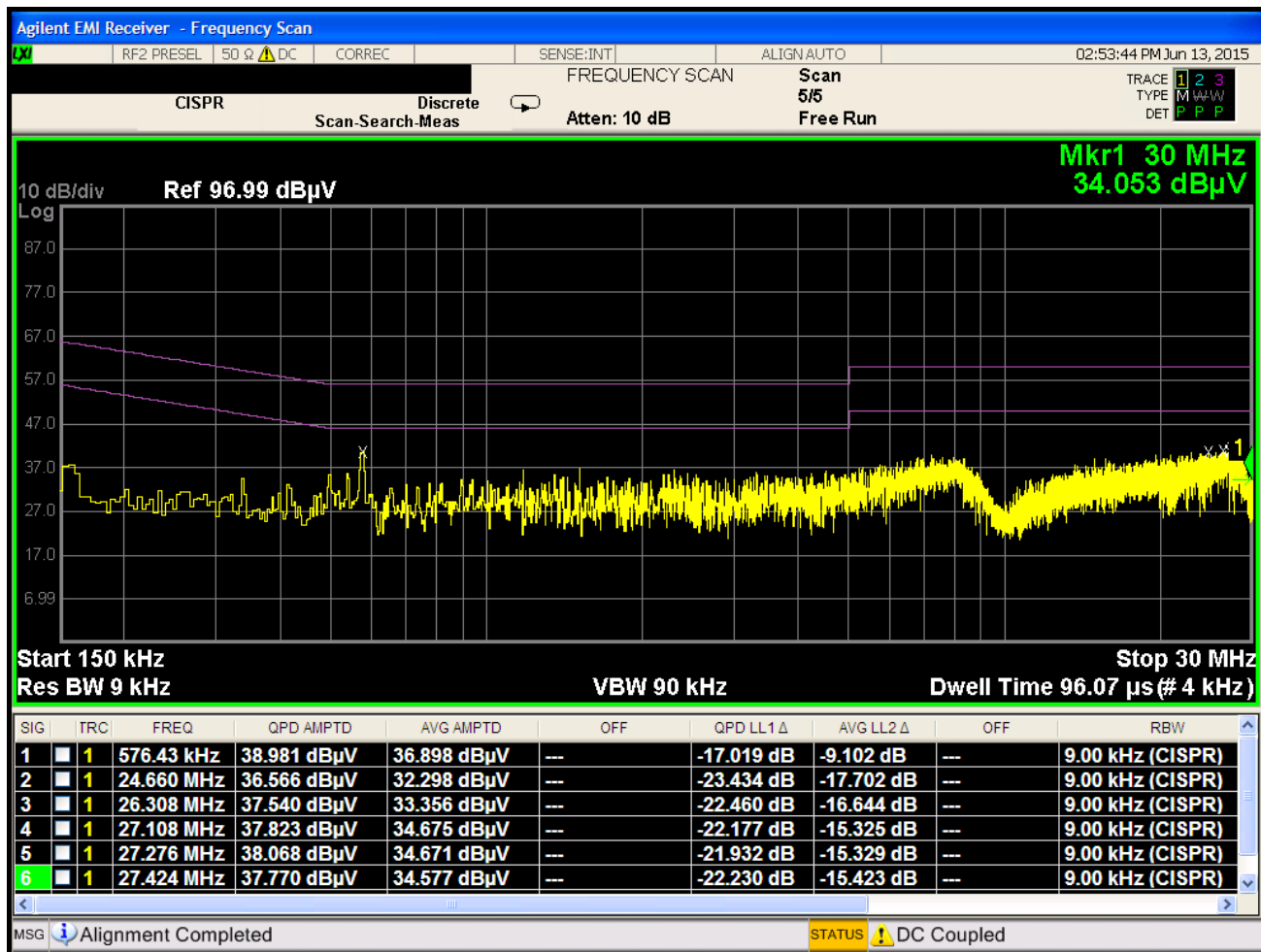
Plot 6-252. Line Conducted Plot with 802.11a UNII Band 3 (L1)
