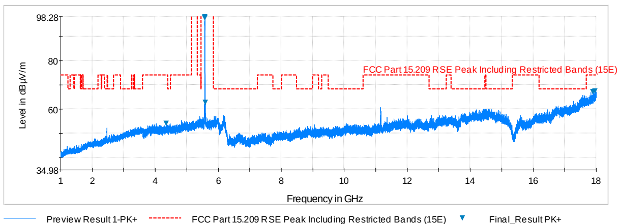
Plot 6-168. Radiated Spurious Plot above 1GHz (802.11a – U2C Ch. 116, Ant. Pol. V)
