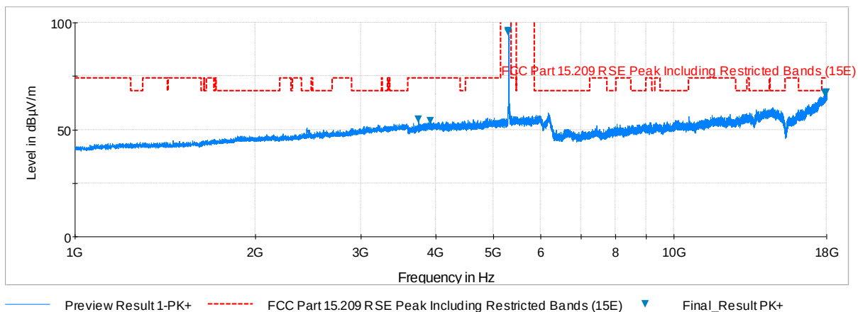
Plot 6-156. Radiated Spurious Plot above 1GHz (802.11a – U2A Ch. 56, Ant. Pol. V)
