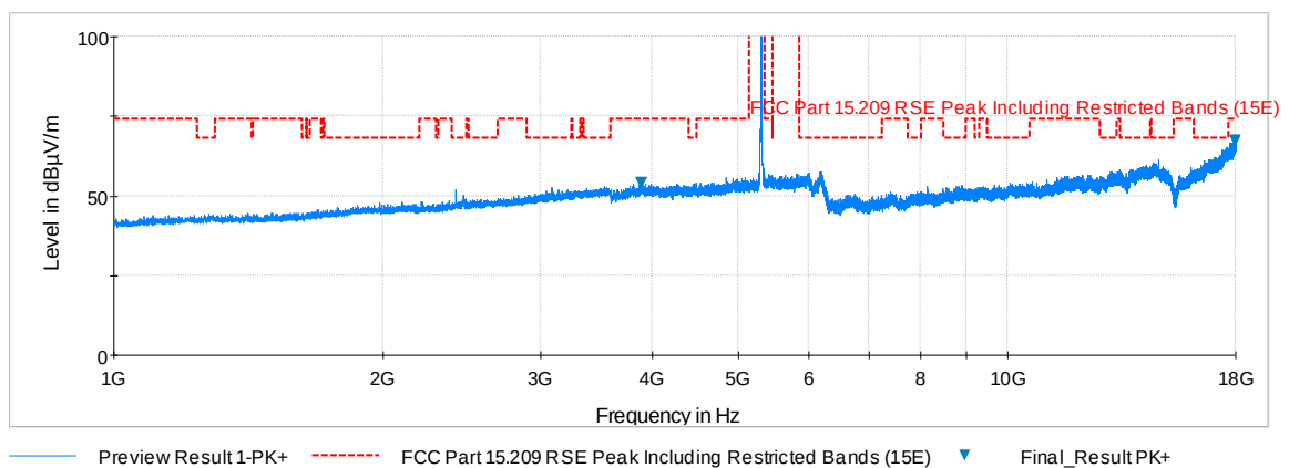
Plot 6-165. Radiated Spurious Plot above 1GHz (802.11a – U2A Ch. 56, Ant. Pol. H)
