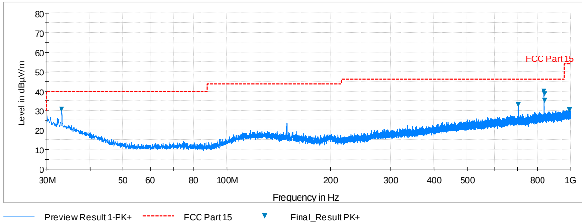
Plot 6-241. Radiated Spurious Plot below 1GHz (802.11a – U3 Ch. 157, Ant. Pol. V)
