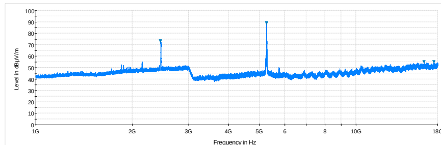
Plot 6-176. Radiated Spurious Plot above 1GHz (Simultaneous Tx Config-2, Pol. V)
