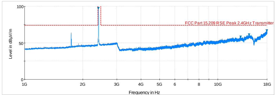
Plot 6-73. Radiated Spurious Plot above 1GHz (802.11b – Ch. 1, Ant. Pol. H)
