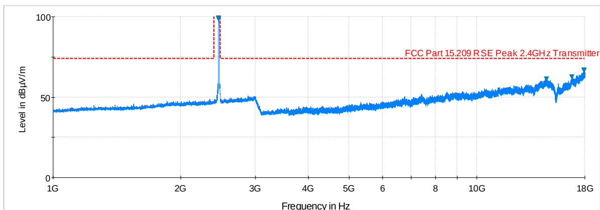
Plot 6-77. Radiated Spurious Plot above 1GHz (802.11b – Ch. 11, Ant. Pol. H)
