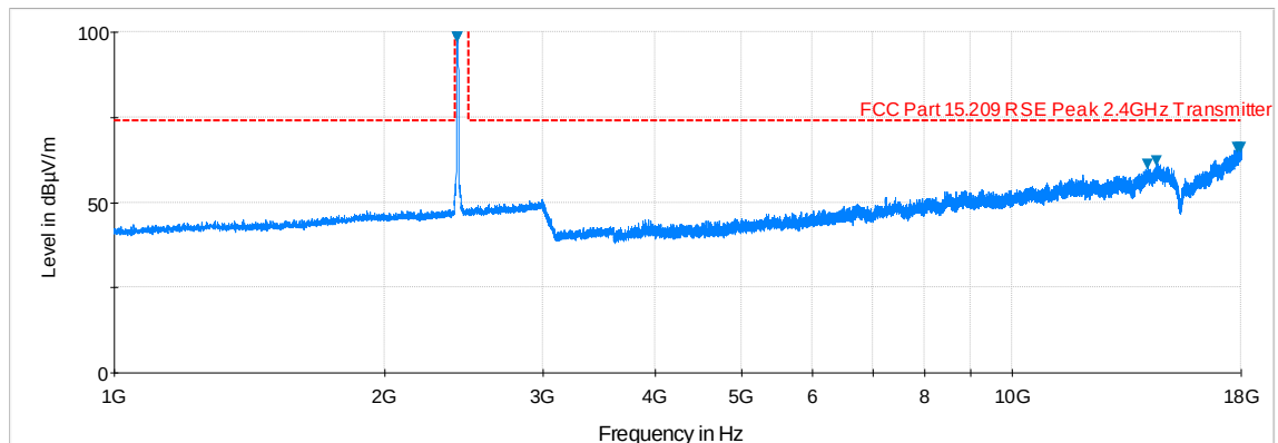
Plot 6-74. Radiated Spurious Plot above 1GHz (802.11b – Ch. 1, Ant. Pol. V)
