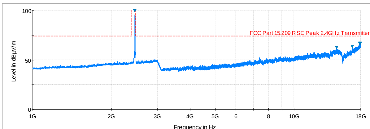
Plot 6-78. Radiated Spurious Plot above 1GHz (802.11b – Ch. 11, Ant. Pol. V)
