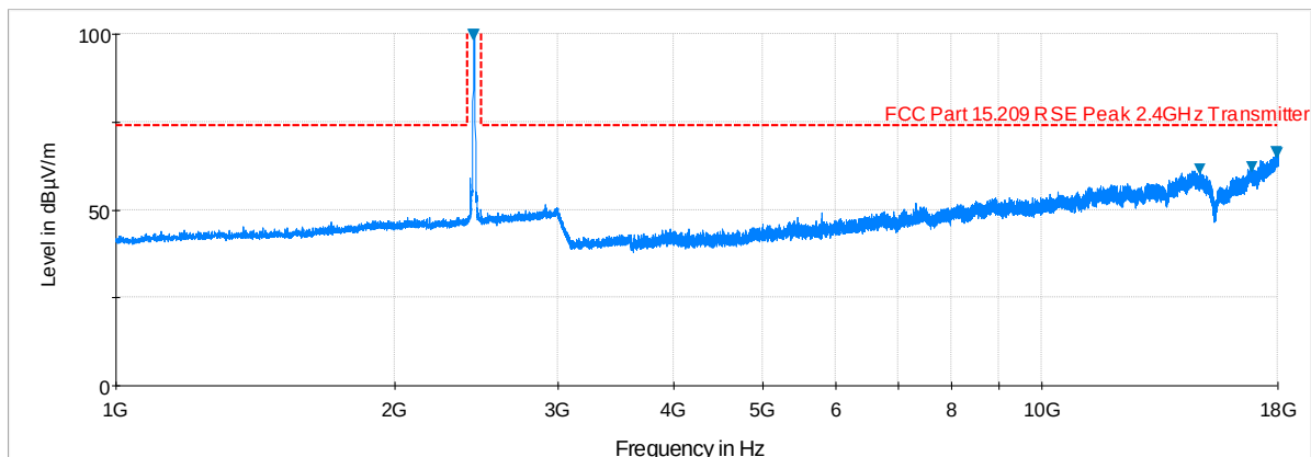
Plot 6-76. Radiated Spurious Plot above 1GHz (802.11b – Ch. 6, Ant. Pol. V)
