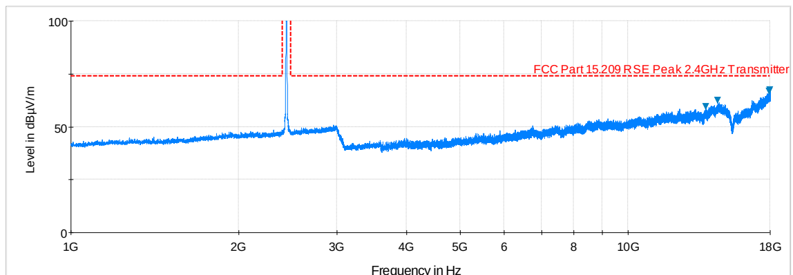
Plot 6-75. Radiated Spurious Plot above 1GHz (802.11b – Ch. 6, Ant. Pol. H)
