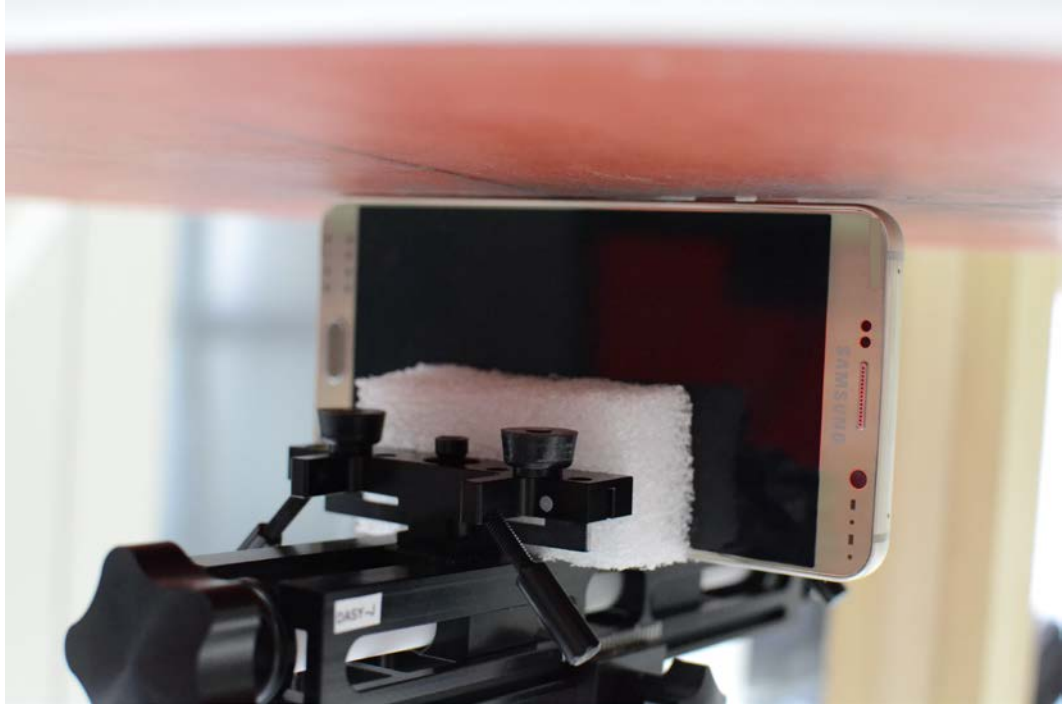
SAR Test Setup Photo 9– Left Edge at 0.0 cm (Extremity)
