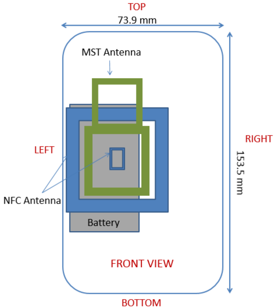
Figure F-2 NFC Antenna Locations
