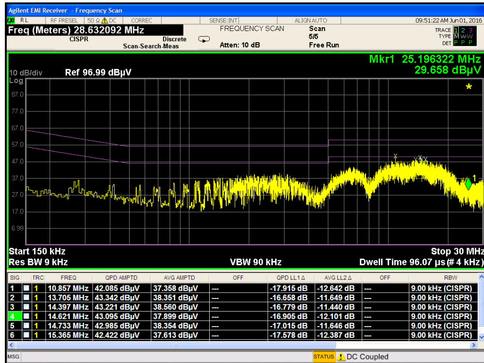
Plot 7-23. Line Conducted Plot with Bluetooth LE (N)
