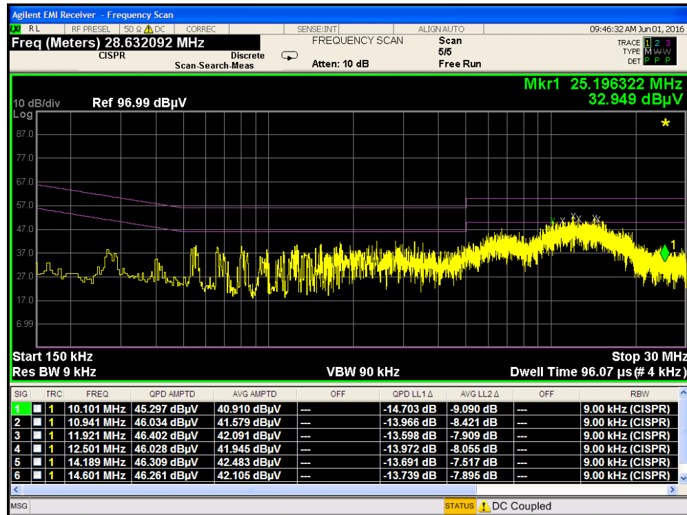
Plot 7-22. Line Conducted Plot with Bluetooth LE (L1)
