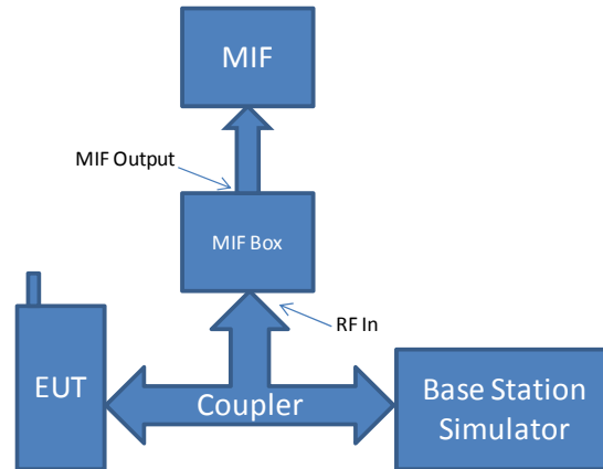
Figure 7-1 MIF Measurement Setup for licensed modes
