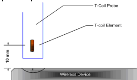
Figure 4-10 Measurement Distance
