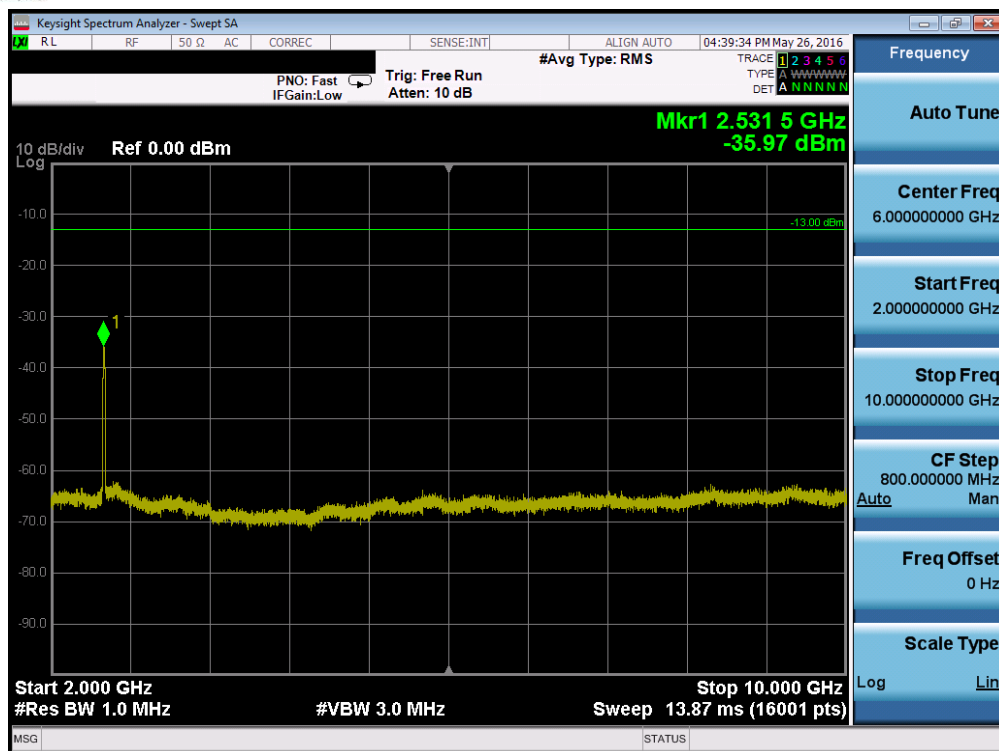
Plot 7-101. Conducted Spurious Plot (Band 5 – 3.0MHz QPSK – RB Size 1, RB Offset 0 – High Channel)
