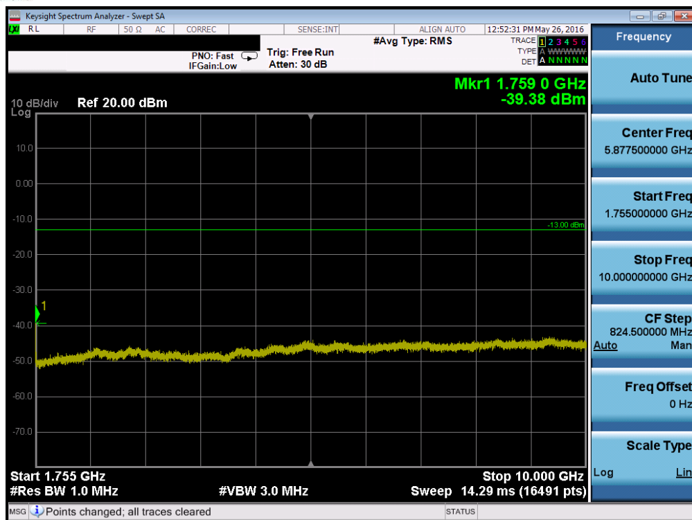
Plot 7-115. Conducted Spurious Plot (Band 4 – 3.0MHz QPSK – RB Size 1, RB Offset 0 – Mid Channel)
