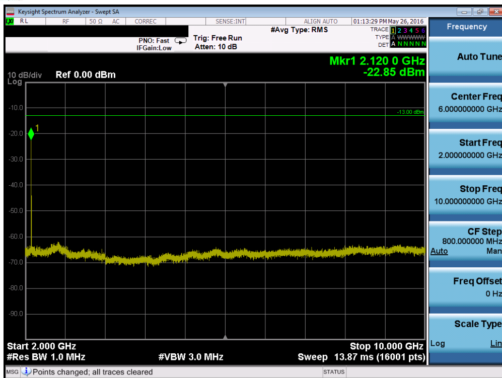
Plot 7-83. Conducted Spurious Plot (Band 12/17 – 5.0MHz QPSK – RB Size 1, RB Offset 0 – High Channel)
