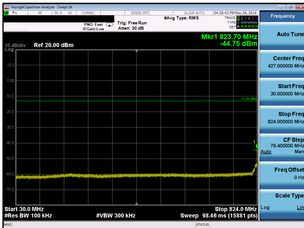
Plot 7-108. Conducted Spurious Plot (Band 26 – 3.0MHz QPSK – RB Size 1, RB Offset 0 – High Channel)
