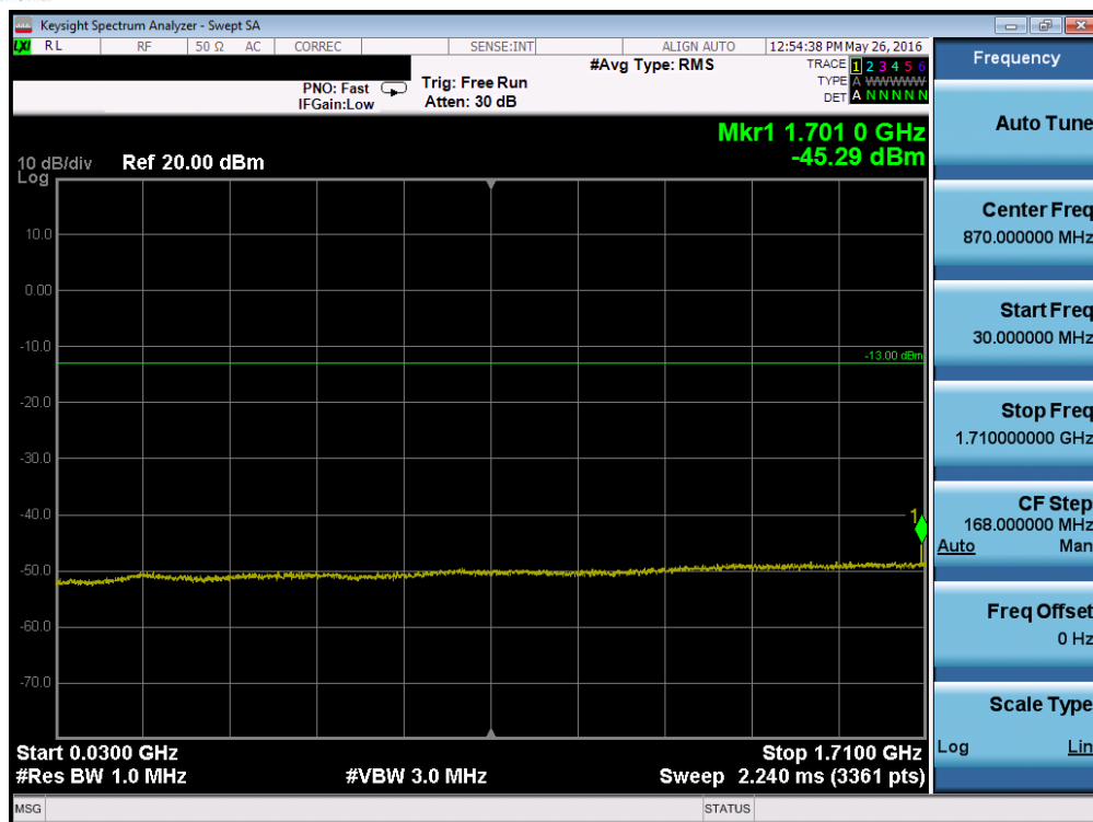
Plot 7-117. Conducted Spurious Plot (Band 4 – 3.0MHz QPSK – RB Size 1, RB Offset 0 – High Channel)
