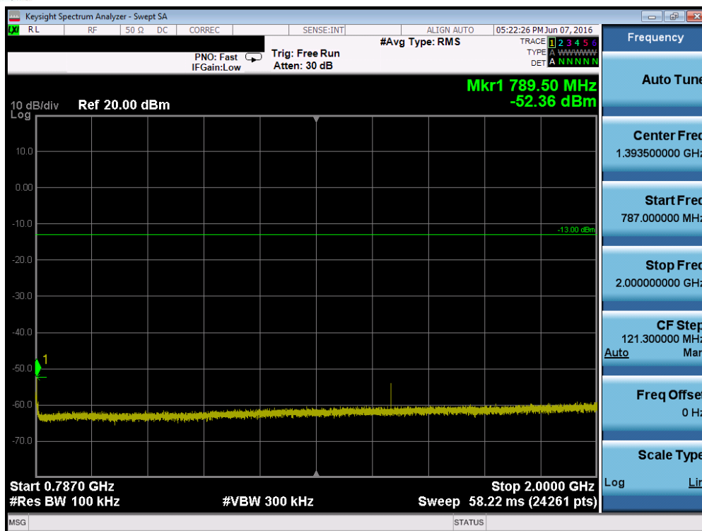
Plot 7-85. Conducted Spurious Plot (Band 13 – 5.0MHz QPSK – RB Size 1, RB Offset 0 – Low Channel)
