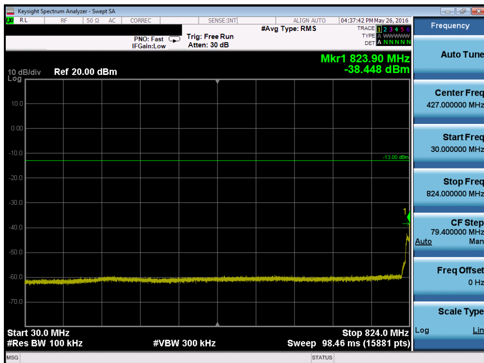
Plot 7-96. Conducted Spurious Plot (Band 5 – 3.0MHz QPSK – RB Size 1, RB Offset 0 – Mid Channel)
