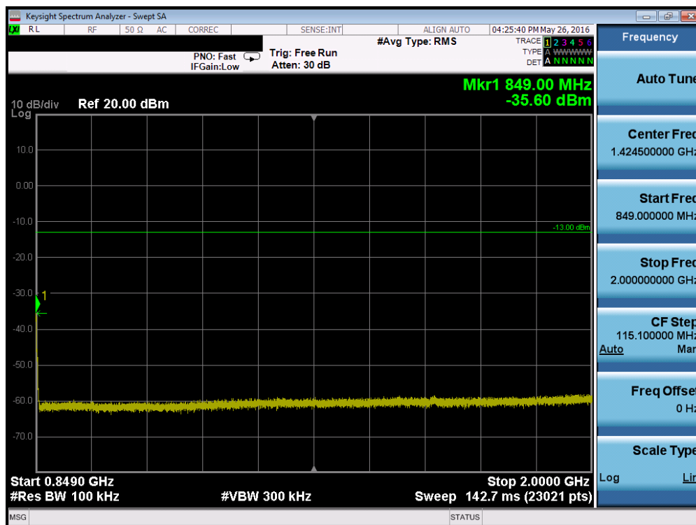
Plot 7-106. Conducted Spurious Plot (Band 26 – 3.0MHz QPSK – RB Size 1, RB Offset 0 – Mid Channel)
