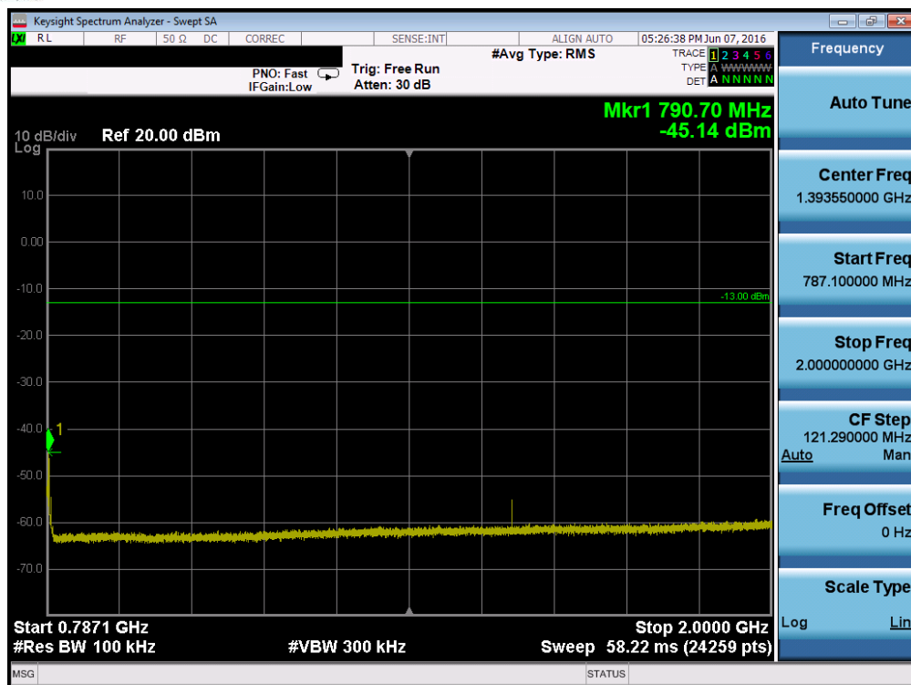
Plot 7-91. Conducted Spurious Plot (Band 13 – 5.0MHz QPSK – RB Size 1, RB Offset 0 – High Channel)
