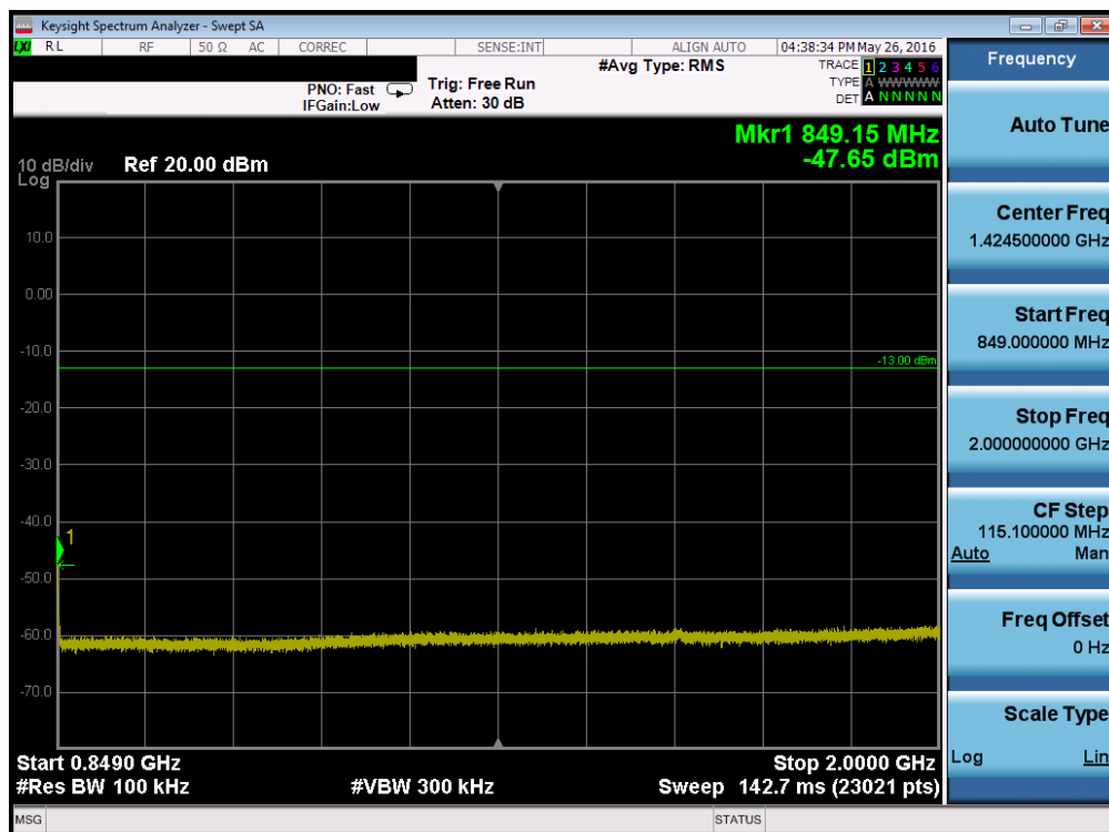
Plot 7-94. Conducted Spurious Plot (Band 5 – 3.0MHz QPSK – RB Size 1, RB Offset 0 – Low Channel)
