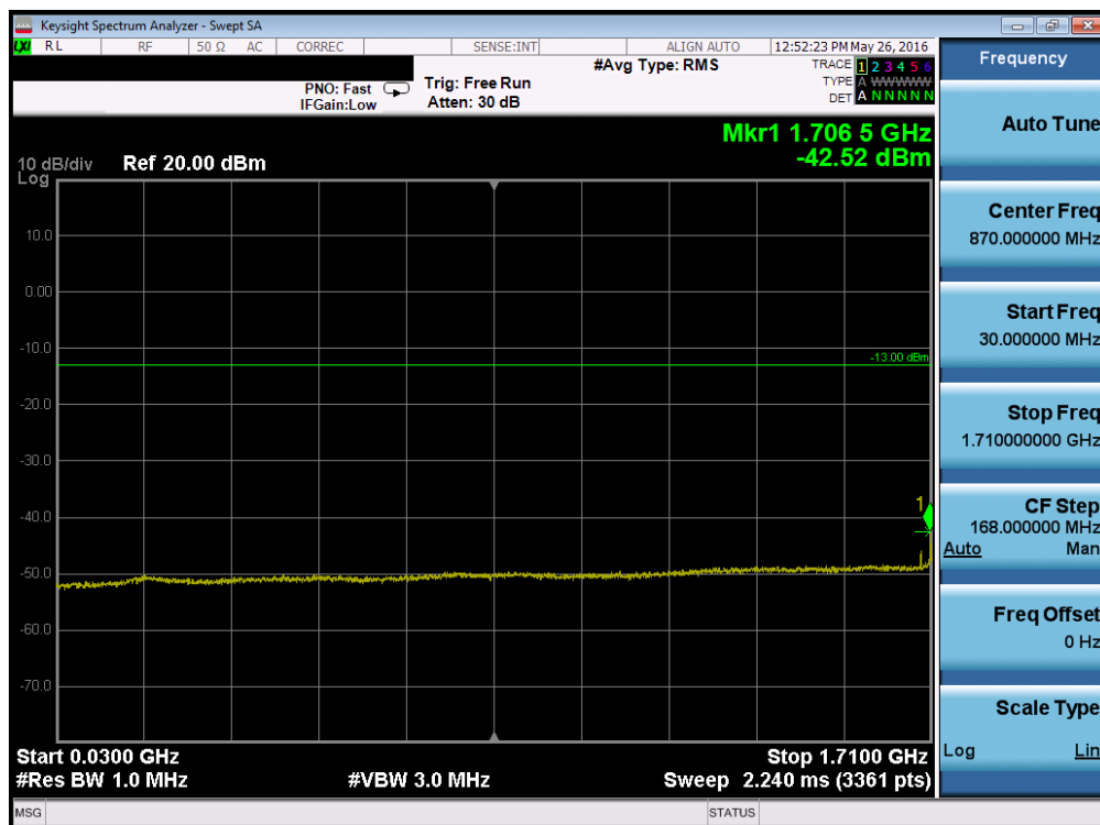
Plot 7-114. Conducted Spurious Plot (Band 4 – 3.0MHz QPSK – RB Size 1, RB Offset 0 – Mid Channel)
