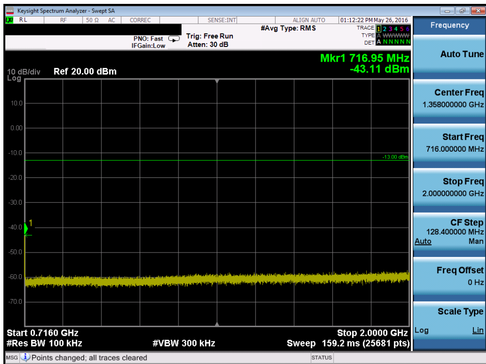
Plot 7-76. Conducted Spurious Plot (Band 12/17 – 5.0MHz QPSK – RB Size 1, RB Offset 0 – Low Channel)
