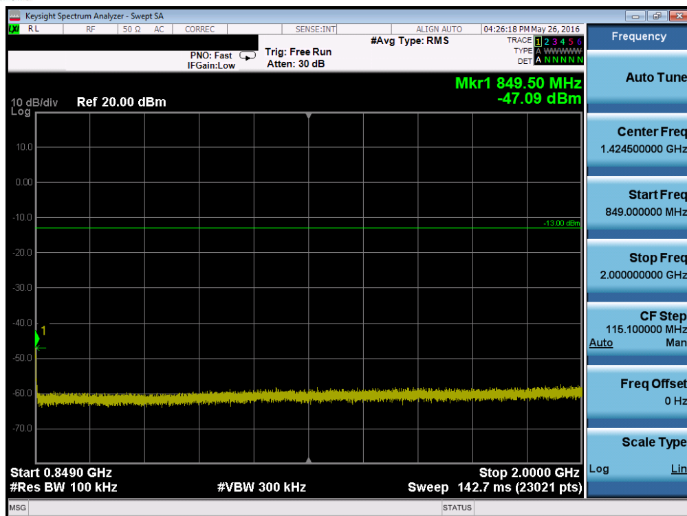
Plot 7-103. Conducted Spurious Plot (Band 26 – 3.0MHz QPSK – RB Size 1, RB Offset 0 – Low Channel)
