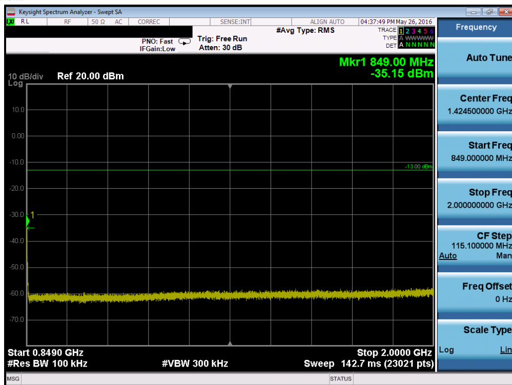
Plot 7-97. Conducted Spurious Plot (Band 5 – 3.0MHz QPSK – RB Size 1, RB Offset 0 – Mid Channel)
