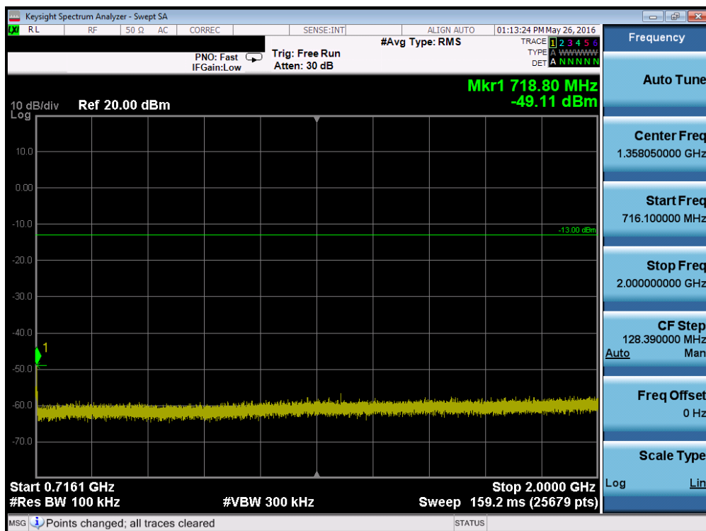
Plot 7-82. Conducted Spurious Plot (Band 12/17 – 5.0MHz QPSK – RB Size 1, RB Offset 0 – High Channel)
