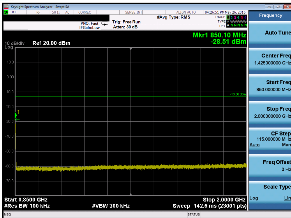
Plot 7-109. Conducted Spurious Plot (Band 26 – 3.0MHz QPSK – RB Size 1, RB Offset 0 – High Channel)
