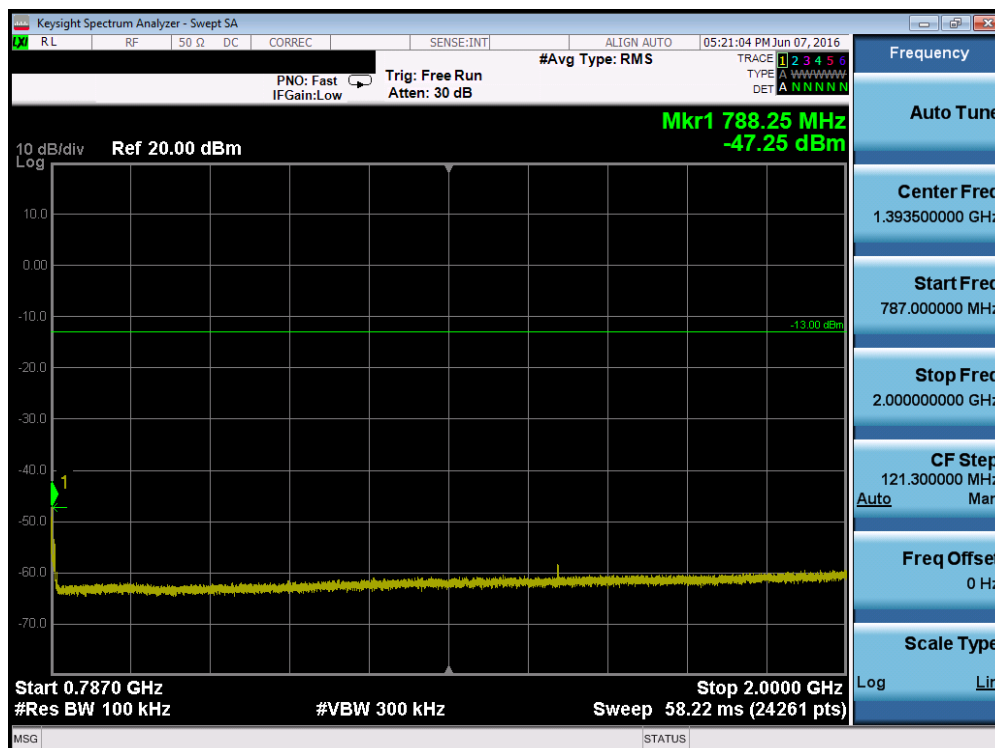
Plot 7-88. Conducted Spurious Plot (Band 13 – 5.0MHz QPSK – RB Size 1, RB Offset 0 – Mid Channel)
