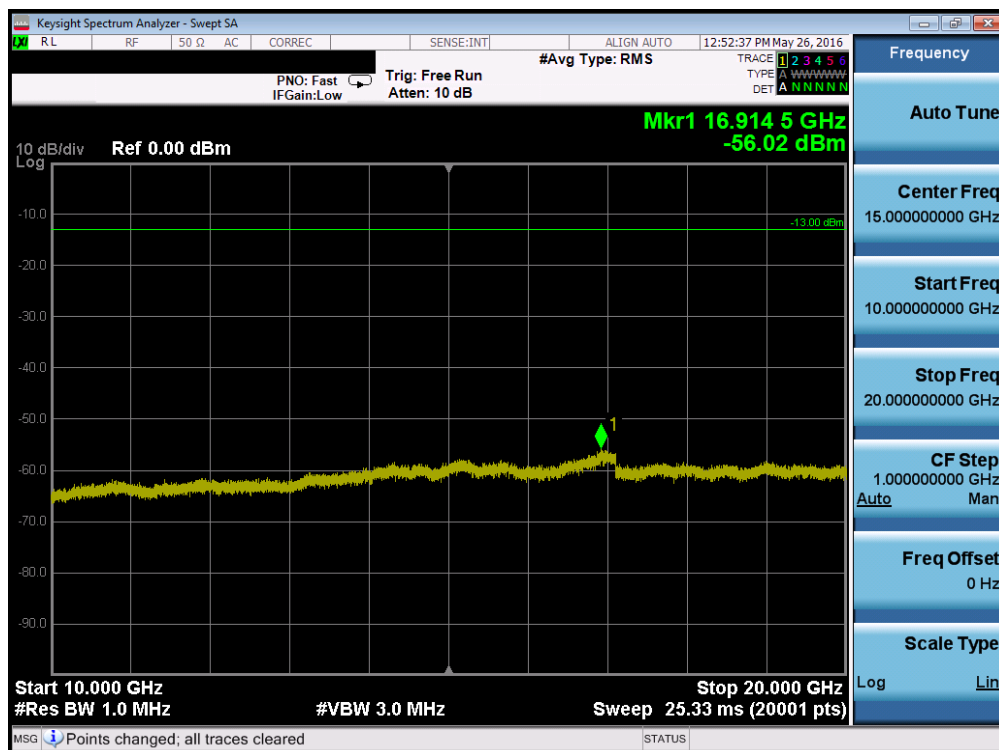
Plot 7-116. Conducted Spurious Plot (Band 4 – 3.0MHz QPSK – RB Size 1, RB Offset 0 – Mid Channel)
