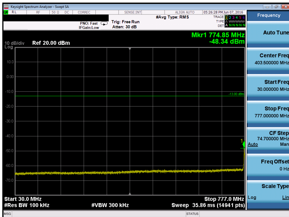
Plot 7-90. Conducted Spurious Plot (Band 13 – 5.0MHz QPSK – RB Size 1, RB Offset 0 – High Channel)
