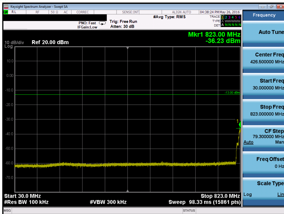
Plot 7-93. Conducted Spurious Plot (Band 5 – 3.0MHz QPSK – RB Size 1, RB Offset 0 – Low Channel)
