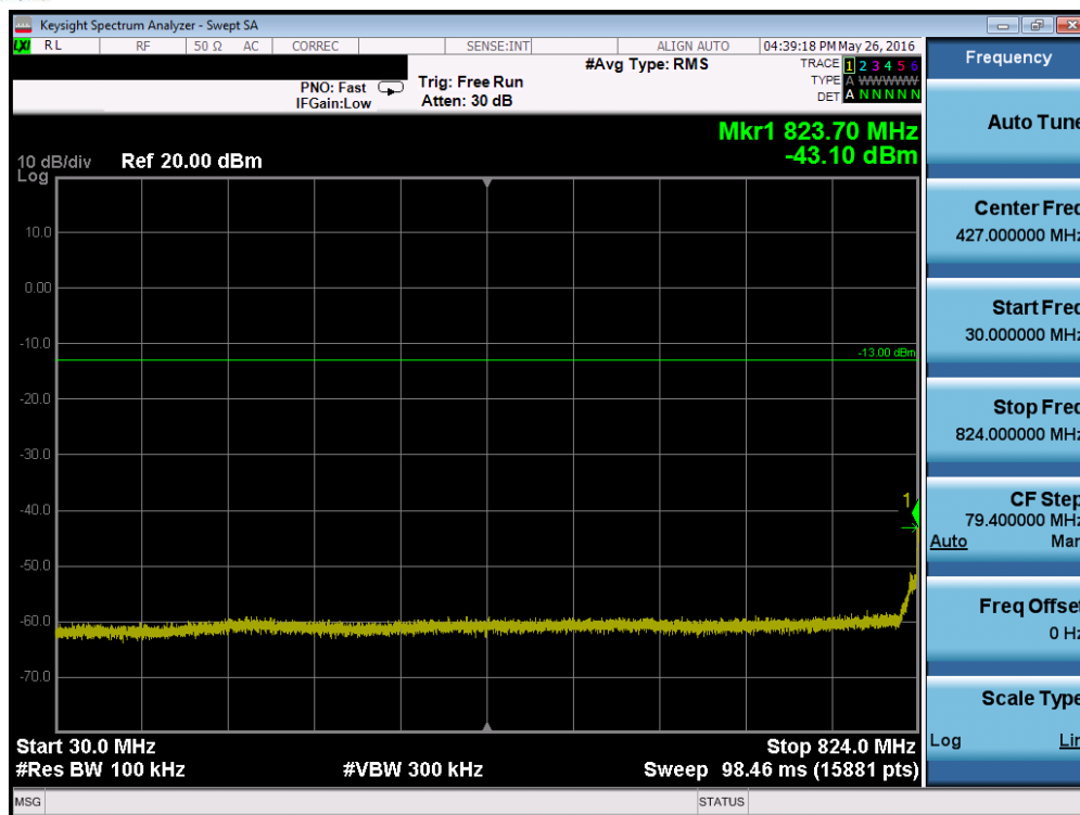
Plot 7-99. Conducted Spurious Plot (Band 5 – 3.0MHz QPSK – RB Size 1, RB Offset 0 – High Channel)
