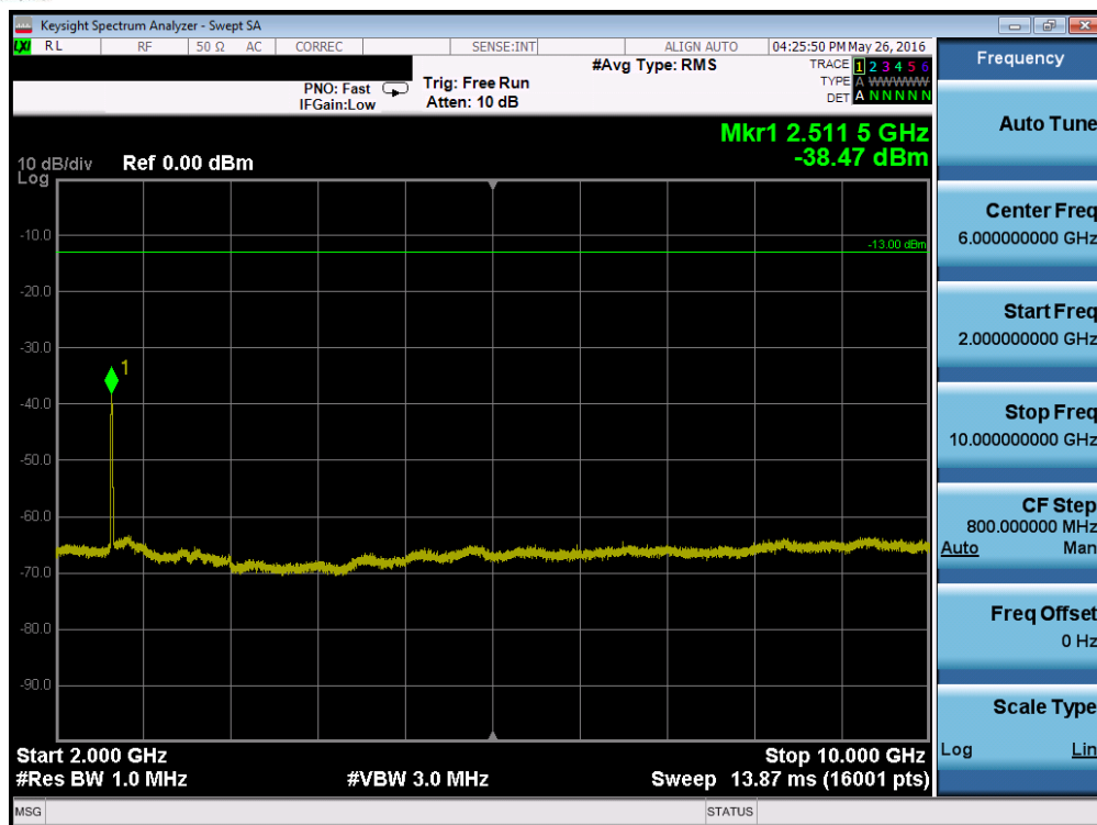
Plot 7-107. Conducted Spurious Plot (Band 26 – 3.0MHz QPSK – RB Size 1, RB Offset 0 – Mid Channel)
