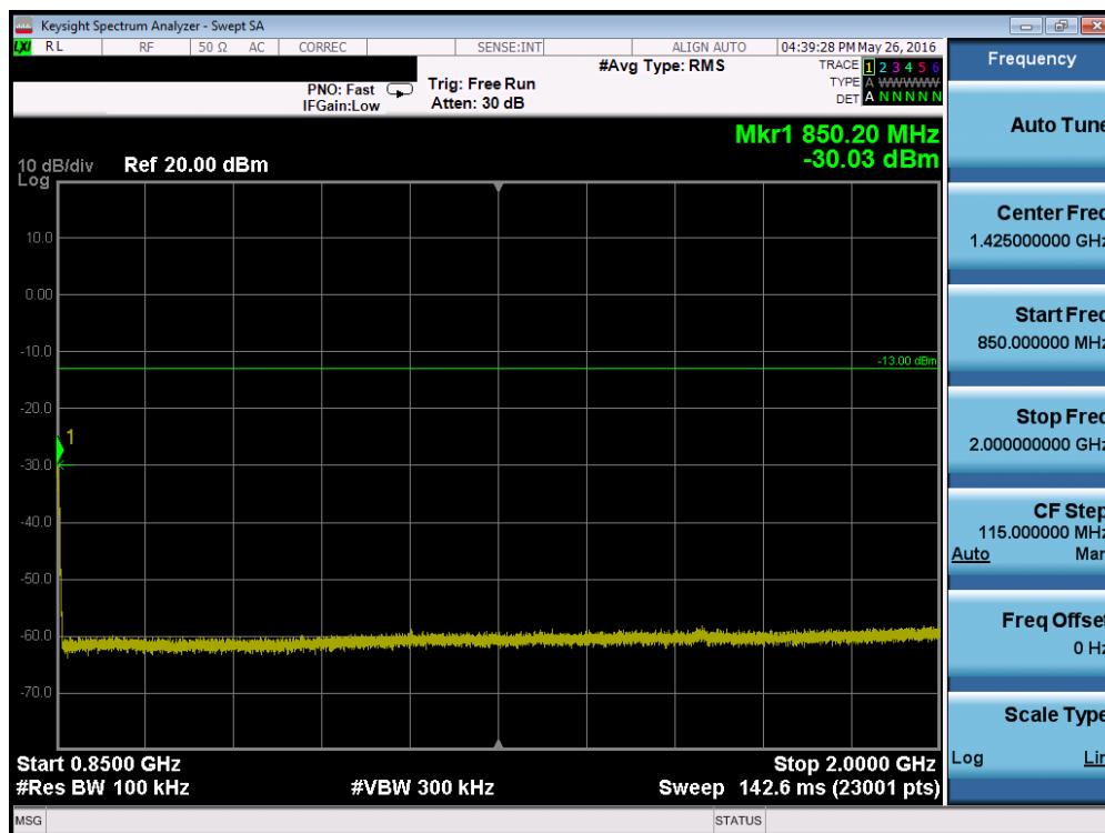
Plot 7-100. Conducted Spurious Plot (Band 5 – 3.0MHz QPSK – RB Size 1, RB Offset 0 – High Channel)
