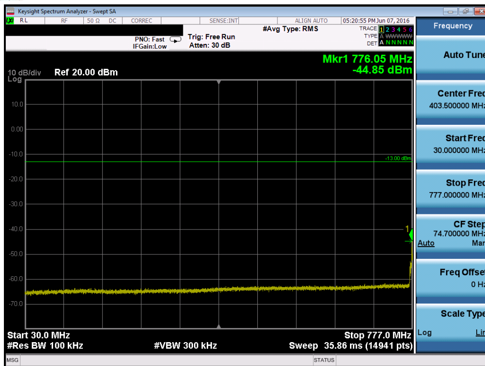
Plot 7-87. Conducted Spurious Plot (Band 13 – 5.0MHz QPSK – RB Size 1, RB Offset 0 – Mid Channel)
