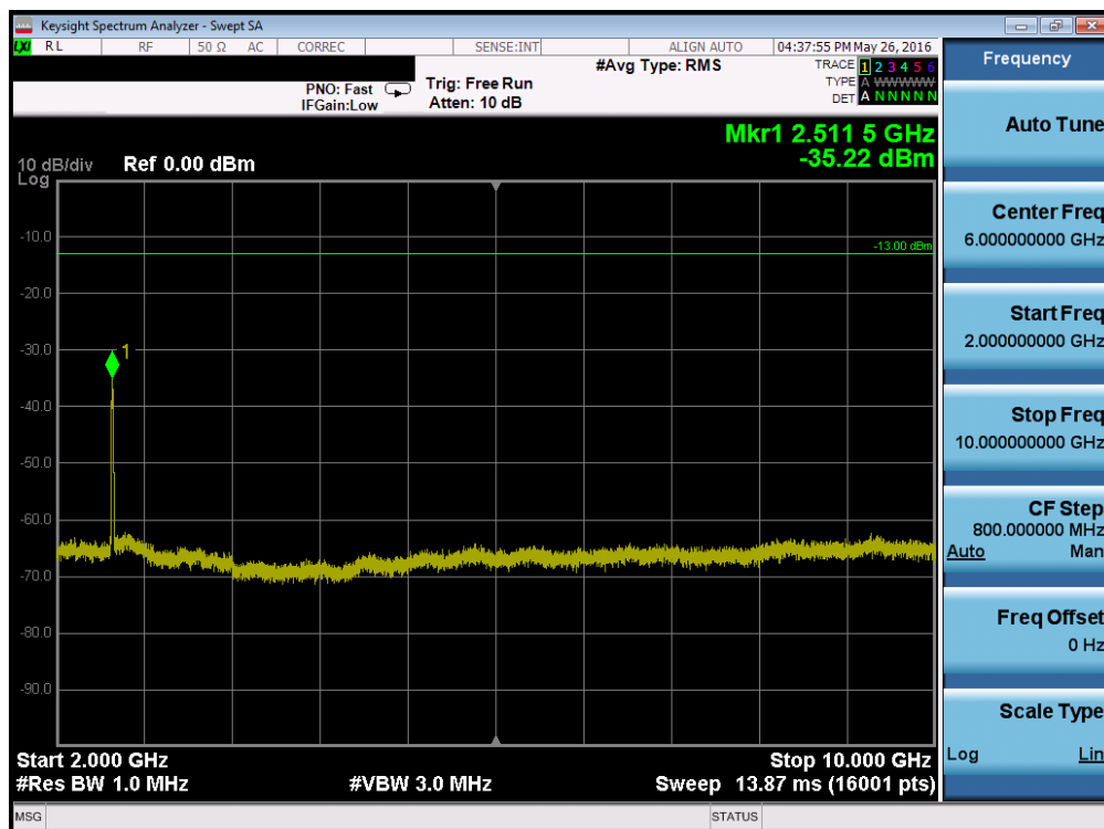
Plot 7-98. Conducted Spurious Plot (Band 5 – 3.0MHz QPSK – RB Size 1, RB Offset 0 – Mid Channel)
