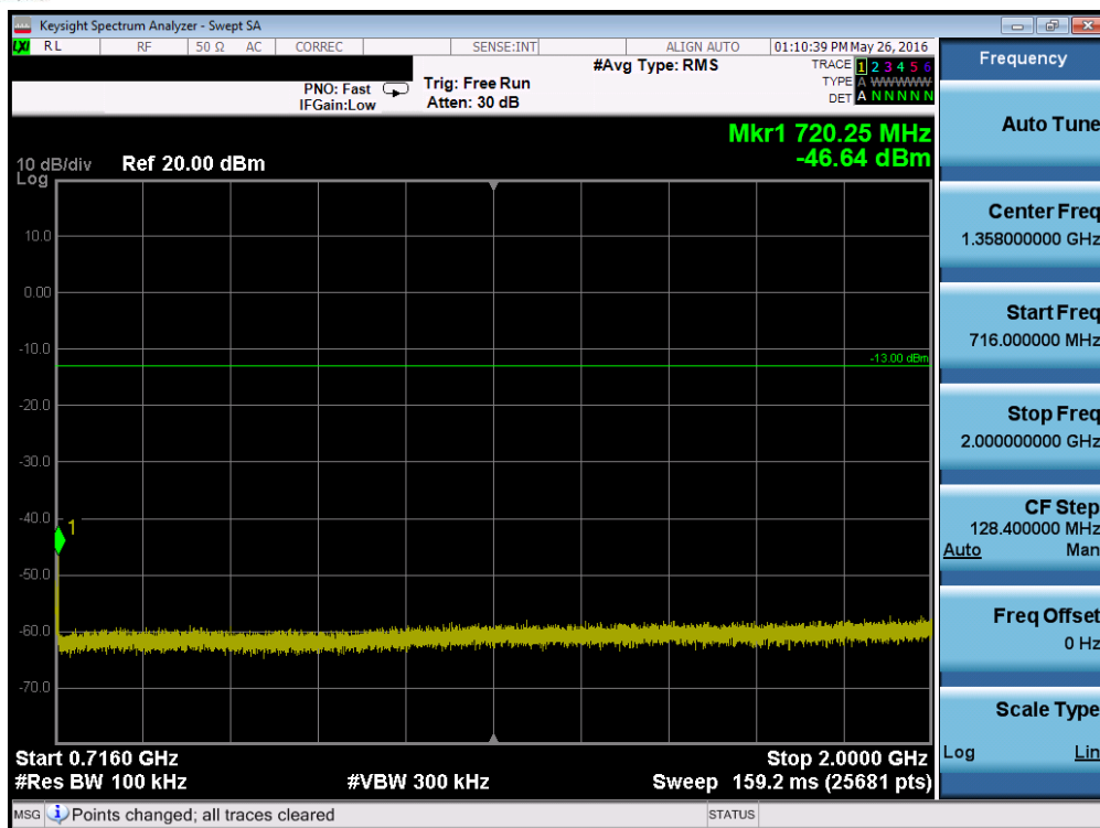
Plot 7-79. Conducted Spurious Plot (Band 12/17 – 5.0MHz QPSK – RB Size 1, RB Offset 0 – Mid Channel)
