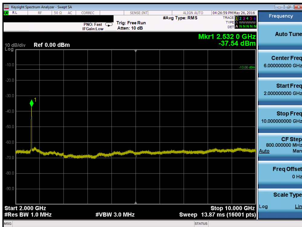
Plot 7-110. Conducted Spurious Plot (Band 26 – 3.0MHz QPSK – RB Size 1, RB Offset 0 – High Channel)
