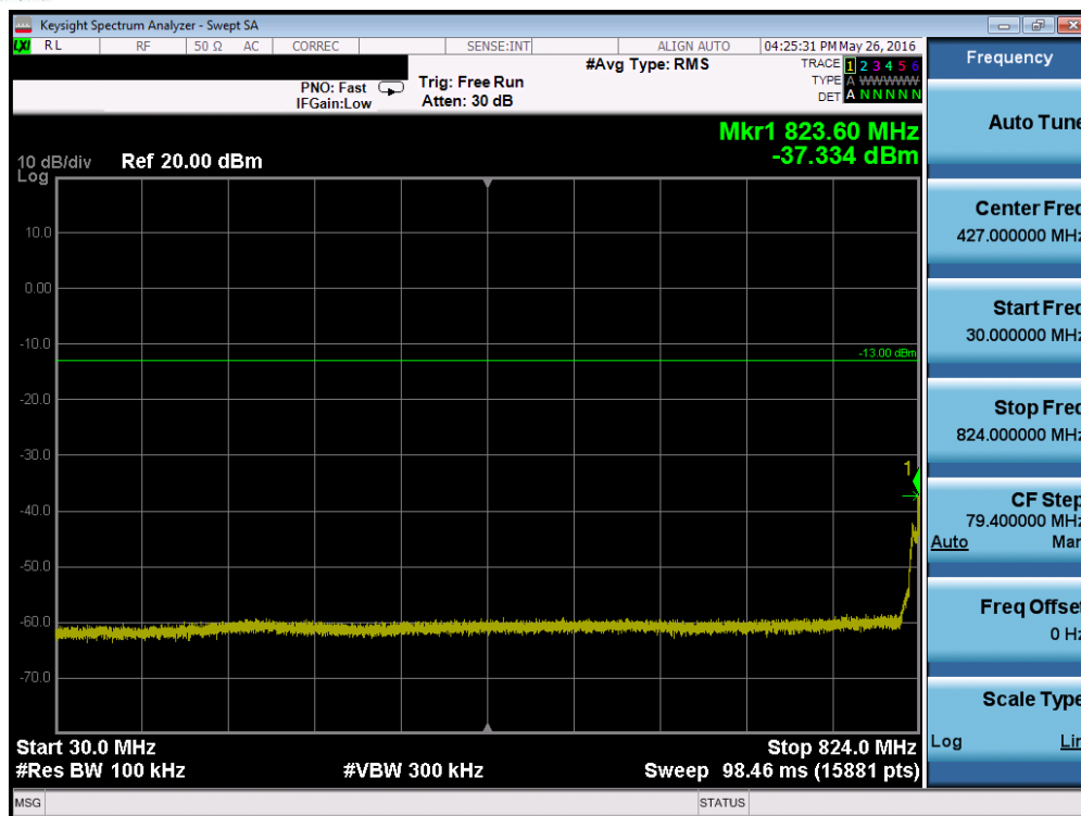
Plot 7-105. Conducted Spurious Plot (Band 26 – 3.0MHz QPSK – RB Size 1, RB Offset 0 – Mid Channel)
