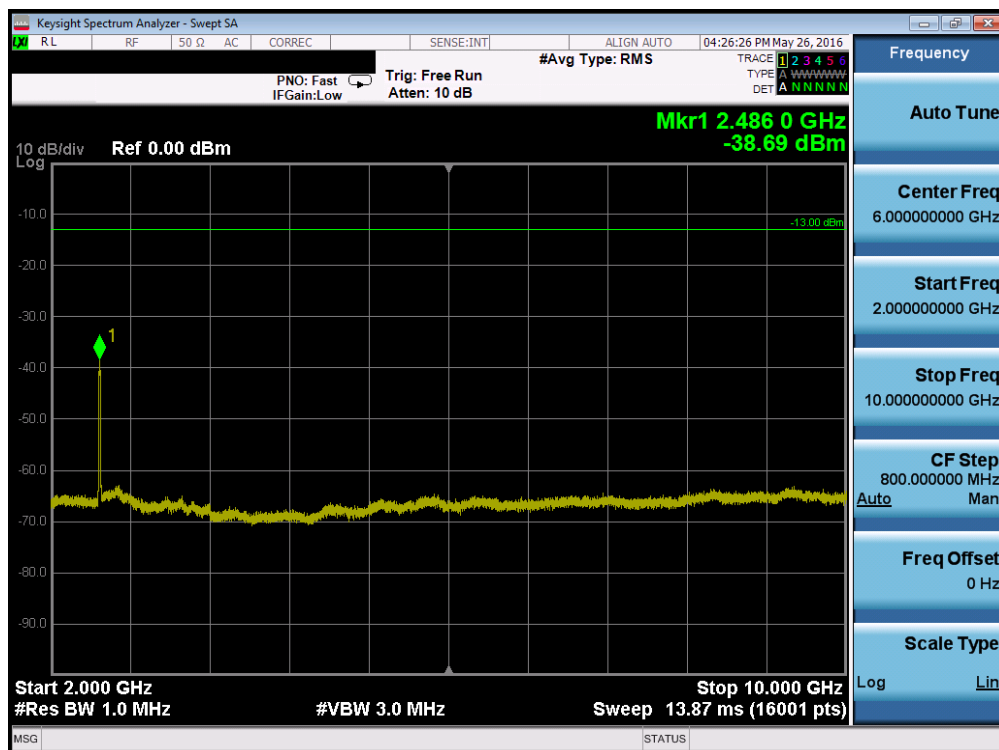
Plot 7-104. Conducted Spurious Plot (Band 26 – 3.0MHz QPSK – RB Size 1, RB Offset 0 – Low Channel)
