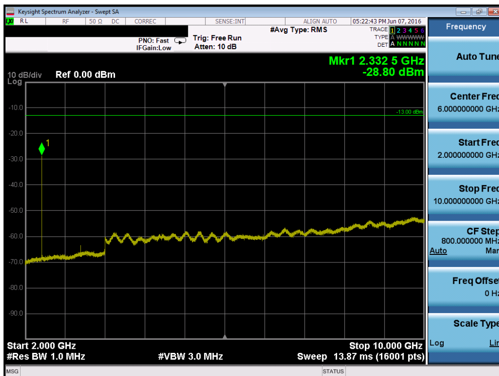
Plot 7-86. Conducted Spurious Plot (Band 13 – 5.0MHz QPSK – RB Size 1, RB Offset 0 – Low Channel)
