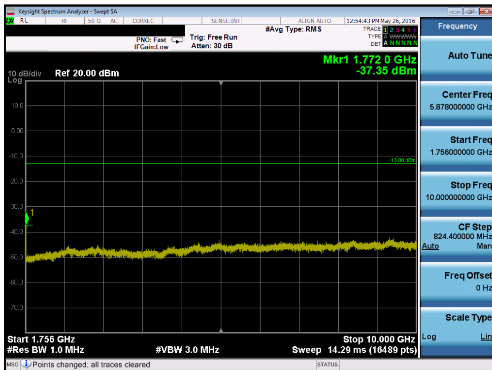
Plot 7-118. Conducted Spurious Plot (Band 4 – 3.0MHz QPSK – RB Size 1, RB Offset 0 – High Channel)
