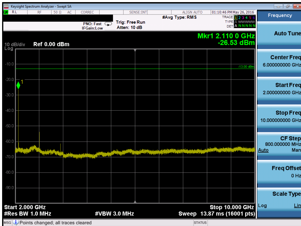
Plot 7-80. Conducted Spurious Plot (Band 12/17 – 5.0MHz QPSK – RB Size 1, RB Offset 0 – Mid Channel)
