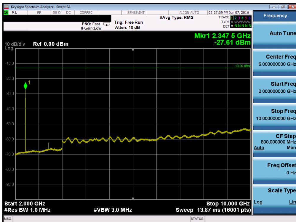
Plot 7-92. Conducted Spurious Plot (Band 13 – 5.0MHz QPSK – RB Size 1, RB Offset 0 – High Channel)
