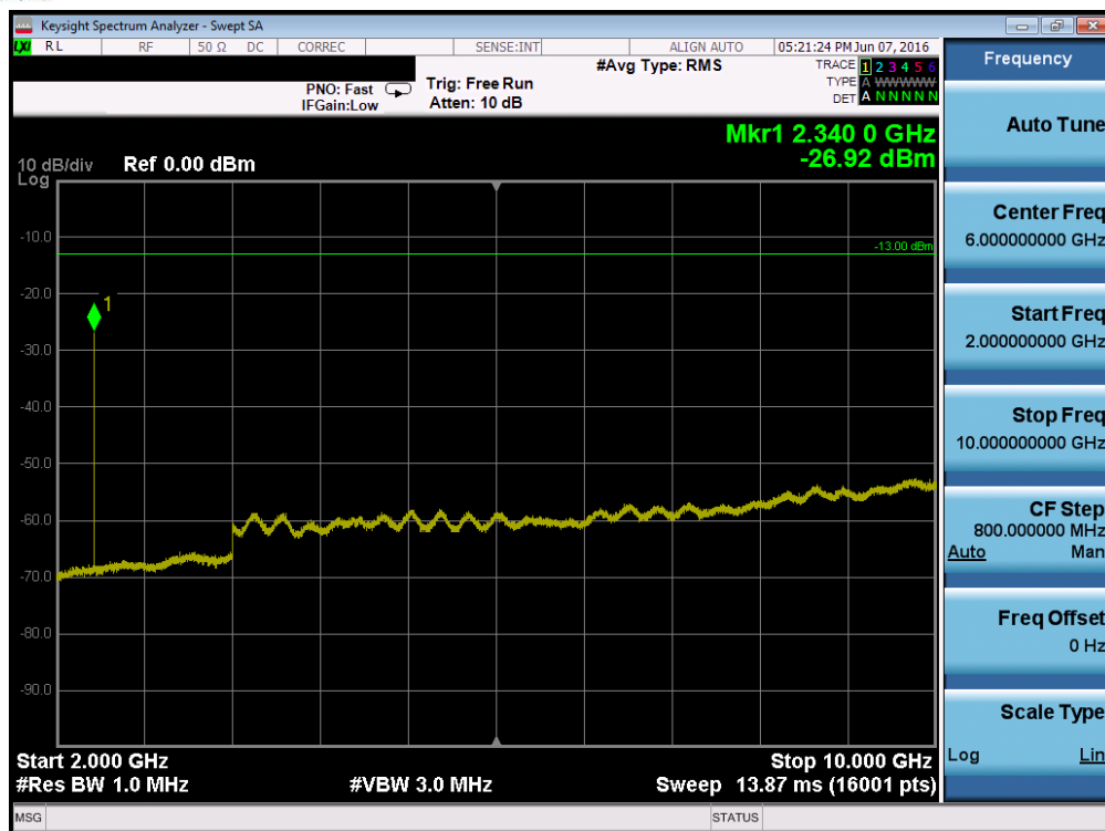
Plot 7-89. Conducted Spurious Plot (Band 13 – 5.0MHz QPSK – RB Size 1, RB Offset 0 – Mid Channel)
