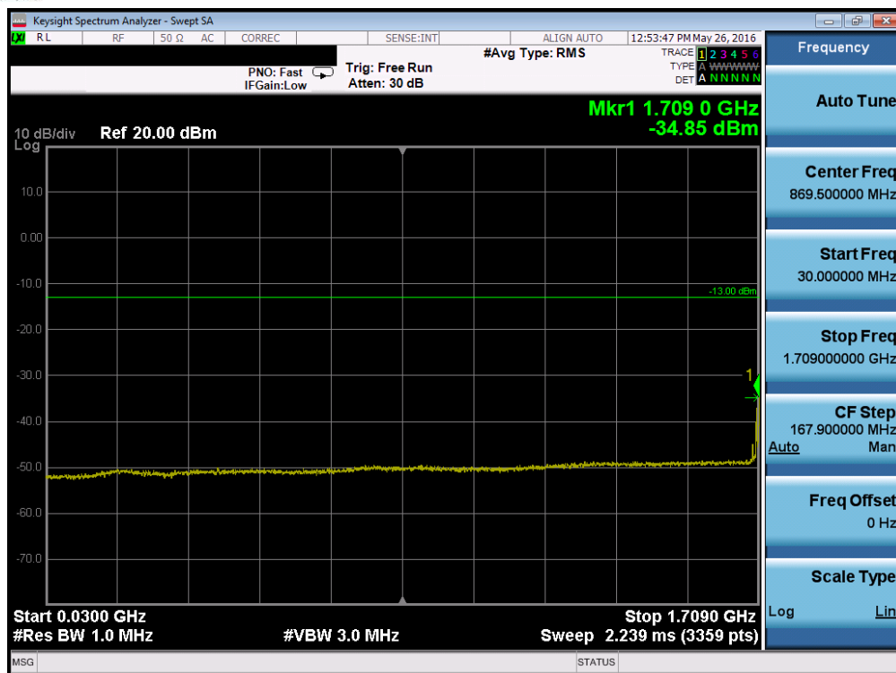
Plot 7-111. Conducted Spurious Plot (Band 4 – 3.0MHz QPSK – RB Size 1, RB Offset 0 – Low Channel)
