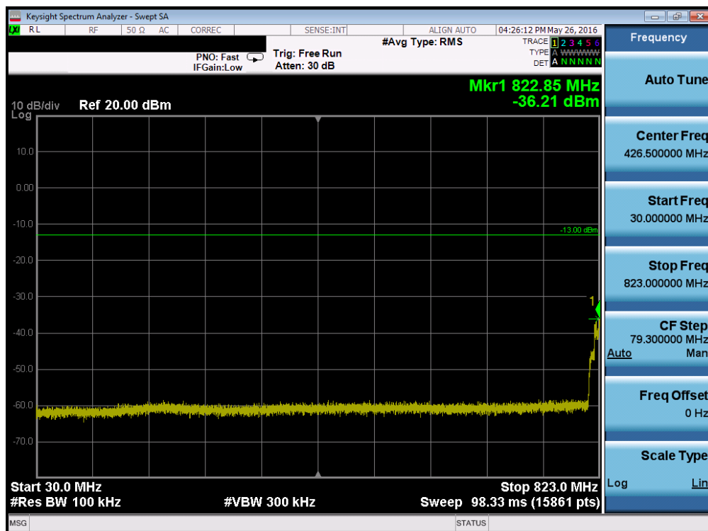
Plot 7-102. Conducted Spurious Plot (Band 26 – 3.0MHz QPSK – RB Size 1, RB Offset 0 – Low Channel)
