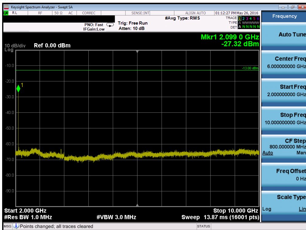
Plot 7-77. Conducted Spurious Plot (Band 12/17 – 5.0MHz QPSK – RB Size 1, RB Offset 0 – Low Channel)
