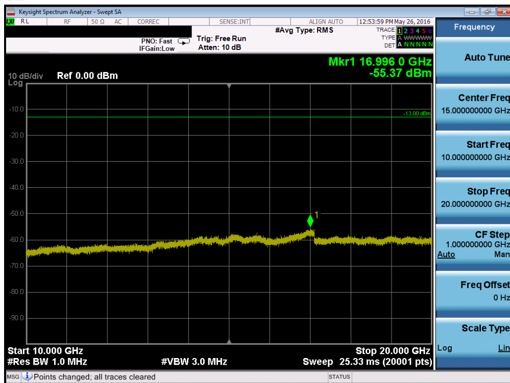
Plot 7-113. Conducted Spurious Plot (Band 4 – 3.0MHz QPSK – RB Size 1, RB Offset 0 – Low Channel)
