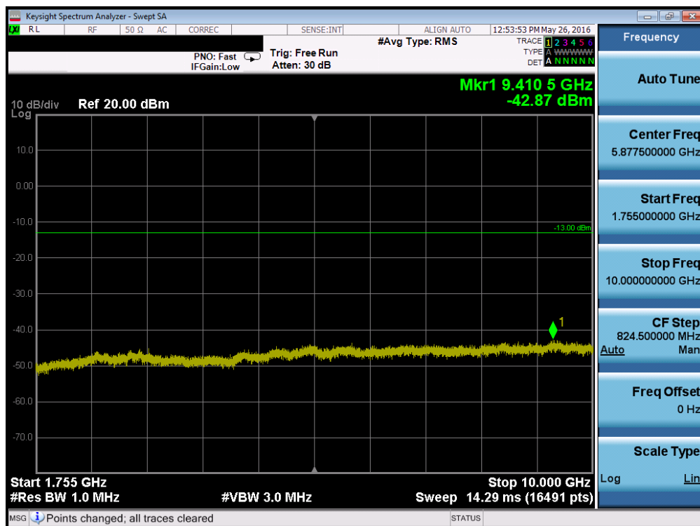
Plot 7-112. Conducted Spurious Plot (Band 4 – 3.0MHz QPSK – RB Size 1, RB Offset 0 – Low Channel)
