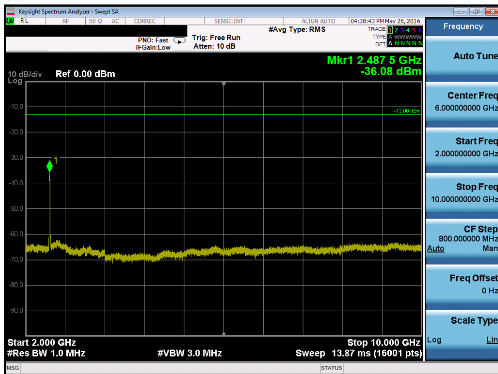
Plot 7-95. Conducted Spurious Plot (Band 5 – 3.0MHz QPSK – RB Size 1, RB Offset 0 – Low Channel)
