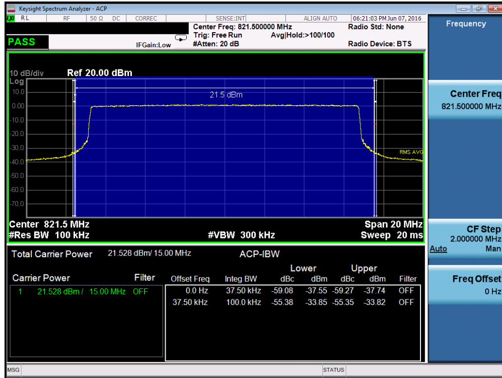
Plot 7-23. Channel Edge Plot (15MHz QPSK – RB Size 75)
