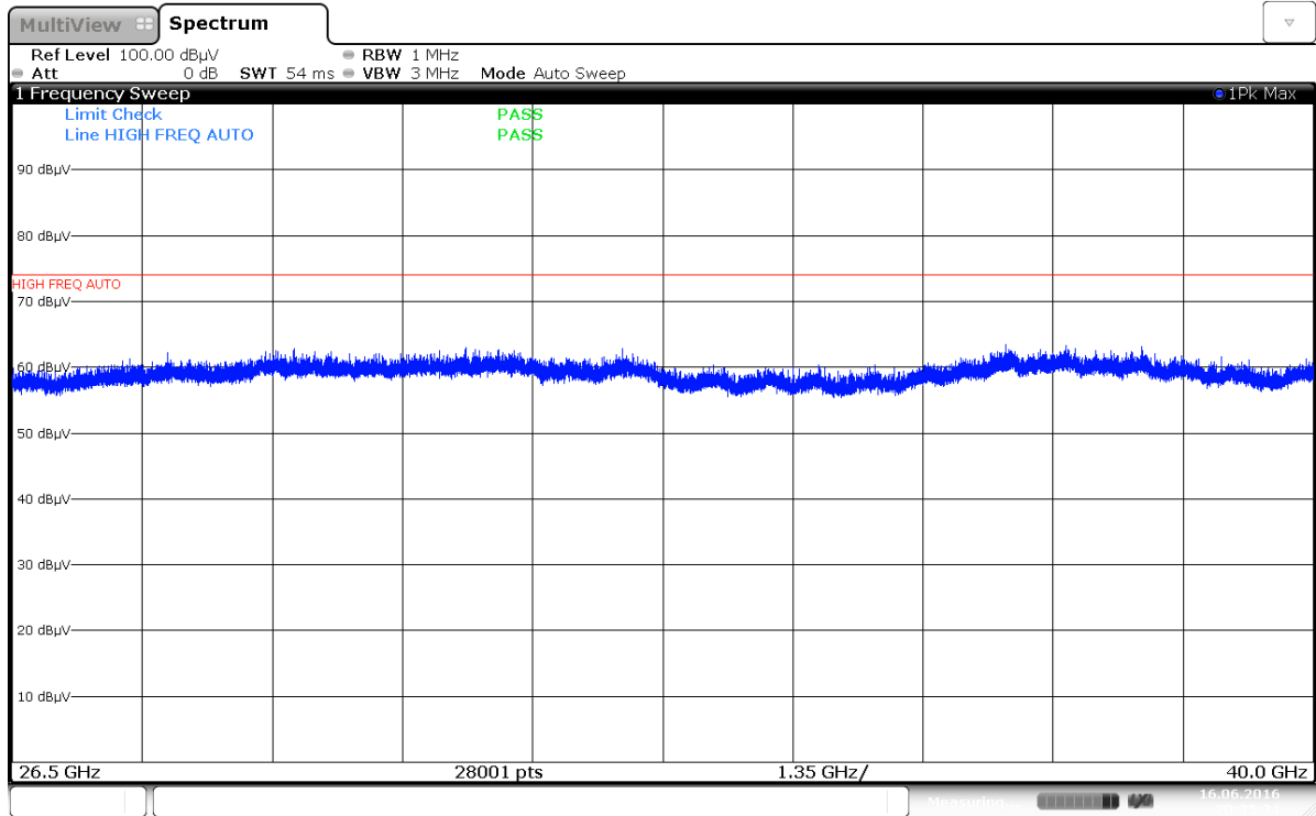
Plot 7-190. Radiated Spurious Plot above 18GHz (5 GHz – 2.4 GHz, Ant. Pol. H)
