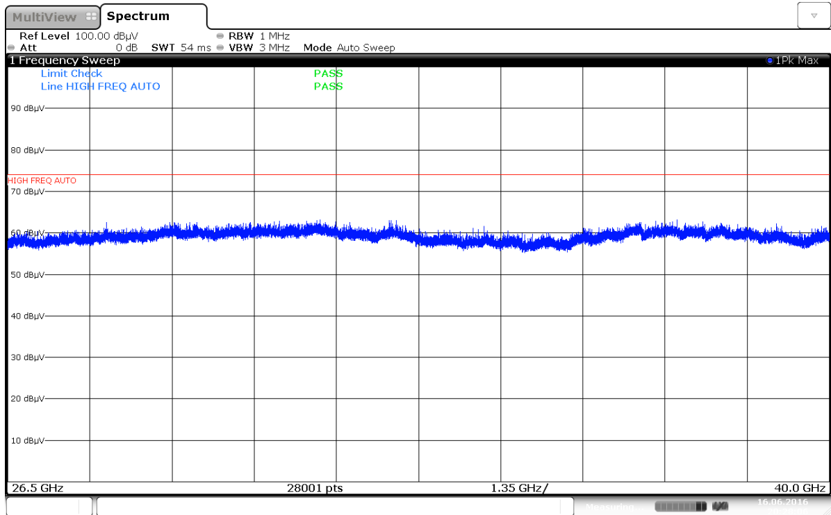
Plot 7-186. Radiated Spurious Plot above 18GHz (2.4 GHz – 5 GHz, Ant. Pol. H)
