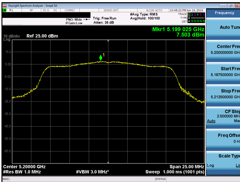
Plot A3-14. Power Spectral Density Plot (802.11a (UNII Band 1) – Ch. 40)
