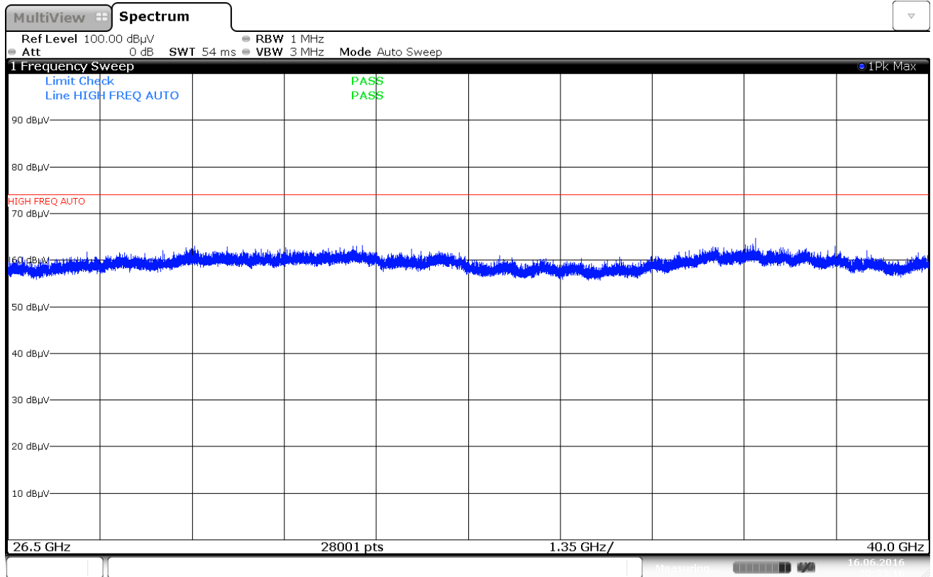
Plot 7-192. Radiated Spurious Plot above 18GHz (5 GHz – 2.4 GHz, Ant. Pol. V)
