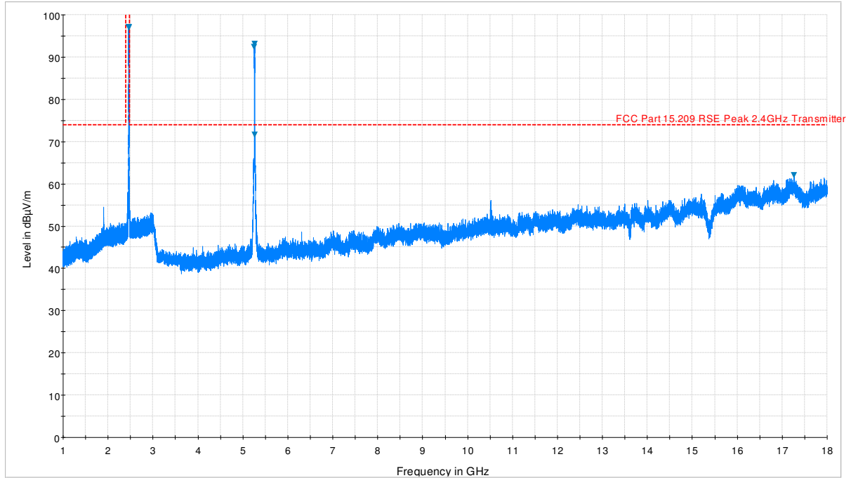
Plot 7-182. Radiated Spurious Plot above 1GHz (2.4GHz – 5GHz, Ant. Pol. V)
