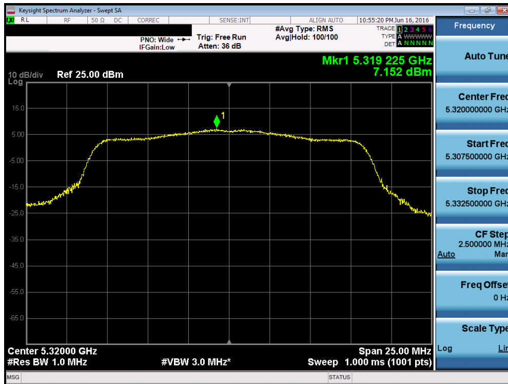
Plot A3-18. Power Spectral Density Plot (802.11a (UNII Band 2A) – Ch. 64)
