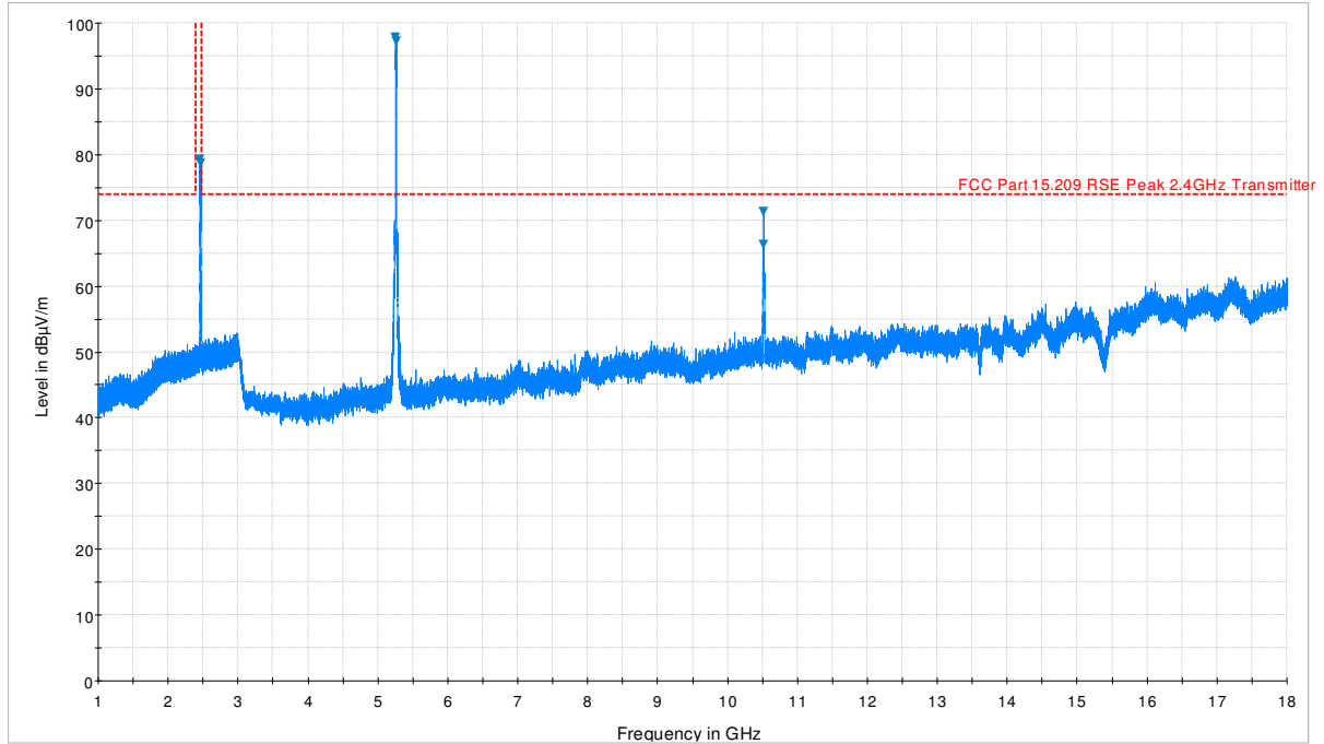
Plot 7-184. Radiated Spurious Plot above 1GHz (5GHz – 2.4 GHz, Ant. Pol. V)
