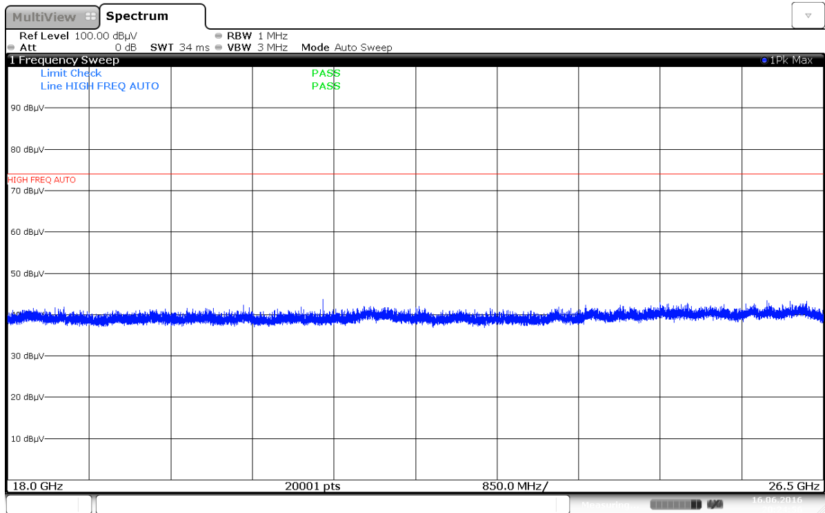
Plot 7-191. Radiated Spurious Plot above 18GHz (5 GHz – 2.4 GHz, Ant. Pol. V)
